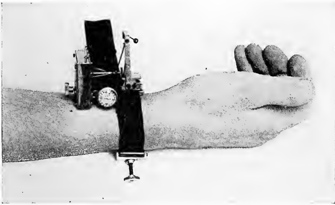
Fig. 15—Dudgeon's sphygmograph.
