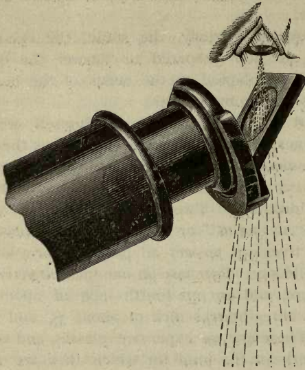
Fig. 4. Camera Lucida, or Neutral Tint Reflector. (Bausch & Lomb.)
