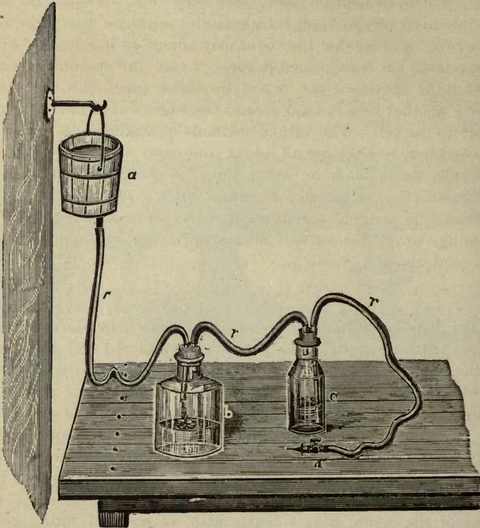
Fig. 7. Injecting Apparatus.
