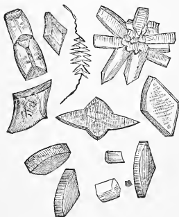
Uric acid in various forms.
