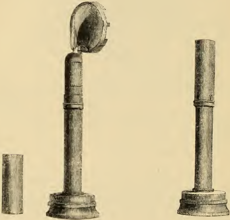
MILLER'S LAMP OPEN.
