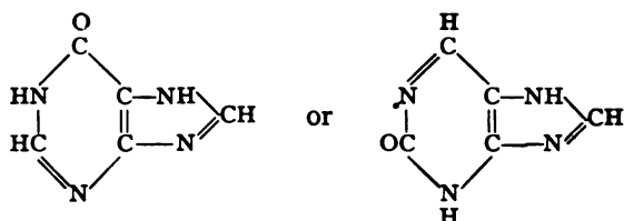
Hypoxanthine
