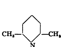
\alpha\alpha' -Dimethylpyridine B.P. 142°-143°; is converted by oxidation into dipicolinic acid.
