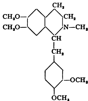
Laudanosine
