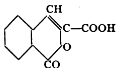
Isocoumarin carboxylic acid
