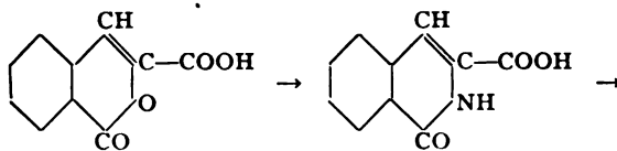
Isocoumarin carboxylic acid
