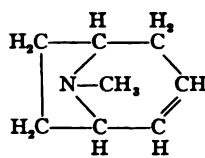
Tropidine (Tropene)
