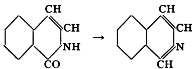
Isocarbostyryl
