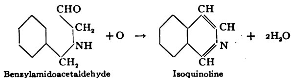
Benzylamidoacetaldehyde
