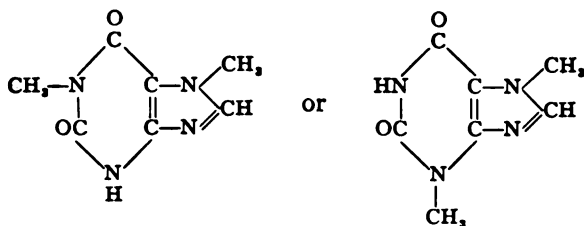
Theobromine
