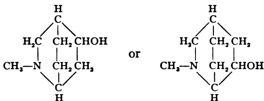
Tropine
