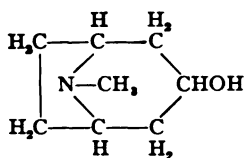
Tropine and Pseudotropine (Tropanol)
