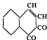
\beta -Naphthoquinone
