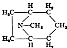
Hydrotropidine (Tropane)
