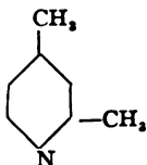
\alpha\gamma -Dimethylpyridine B.P. 156-157°; is converted by oxidation into lutidinic acid.
