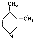
\beta\gamma -Dimethylpyridine B.P. 164°; is converted by oxidation into cinchomeronic acid.
