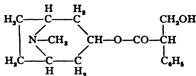
Atropine and Hyoscyamine
