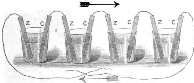
FIG. 28. Voltaic Battery.
