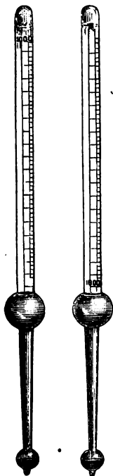
FIG. 31. Hydrometer for liquids heavier than water.
