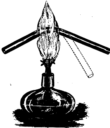
FIG. 18. Bonding Glass Tubing.
