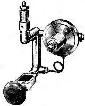
FIG. 96.—Reducing valve.
