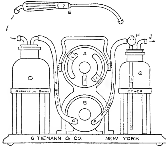
FIG. 132.—Electrical aspirator.
