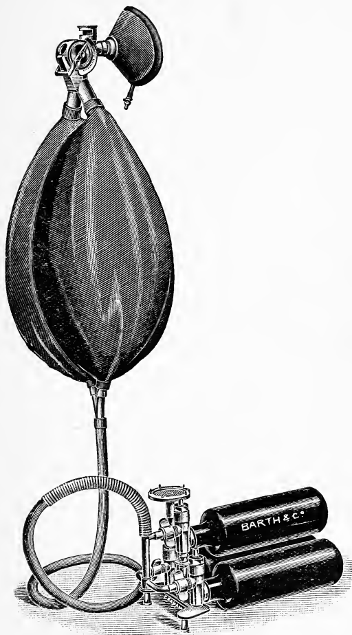
FIG. 9.—DR. HEWITT'S NITROUS OXIDE AND OXYGEN APPARATUS.
