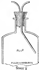
FIG. 15.—THE AUTHOR'S ETHER BOTTLE STOPPER FOR USE WITH ORDINARY EIGHT-OUNCE DISPENSING BOTTLE.
