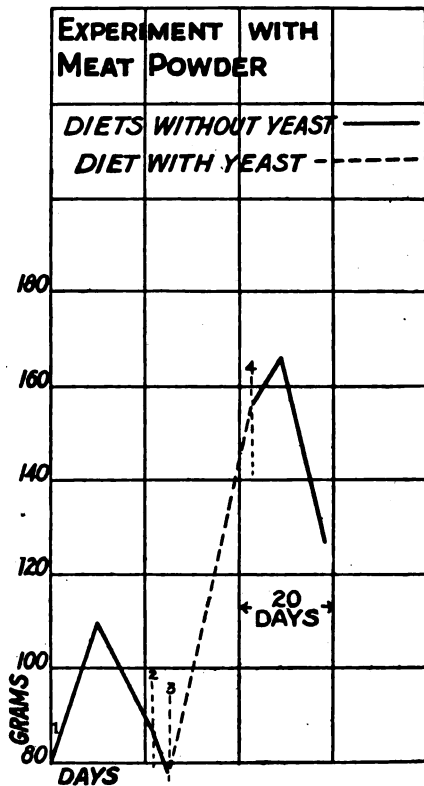
FIG. 174.—GROWTH CURVE OF ALBINO RAT SHOWING IMPORTANCE OF WATER-SOLUBLE "B".
