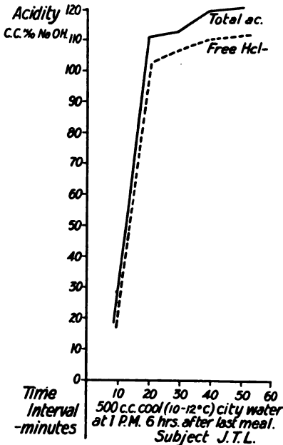
FIG. 41.—CURVES SHOWING STIMULATORY POWER OF WATER. (Bergeim, Rehfuß and Hawk: Journal Biological Chemistry , 19, 345, 1914.)
