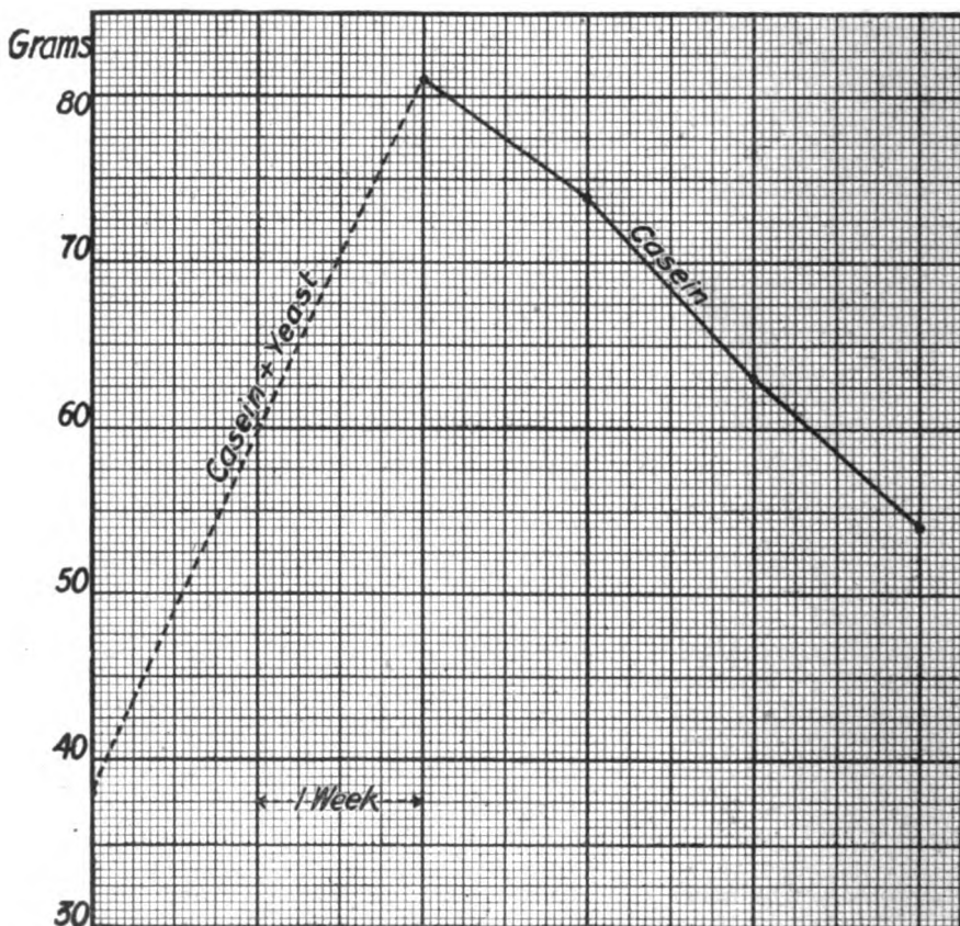
FIG. 171.—GROWTH CURVE OF ALBINO RAT SHOWING IMPORTANCE OF WATER-SOLUBLE "B".
