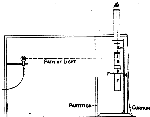
FIG. 95.—NEPHELOMETER IN POSITION, SHOWING RELATION TO SOURCE OF LIGHT.
