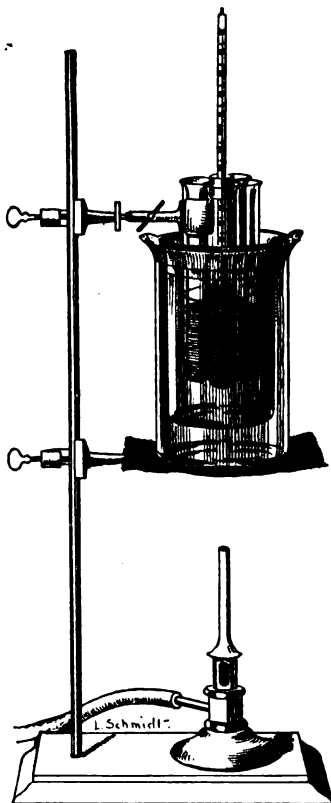
FIG. 36.—COAGULATION TEMPERATURE APPARATUS.
