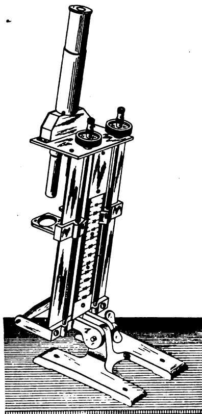
FIG. 96.—KOBBER'S NEPHELOMETER COLORIMETER. (From Journal of Biological Chemistry , 29, 155, 1917.)
