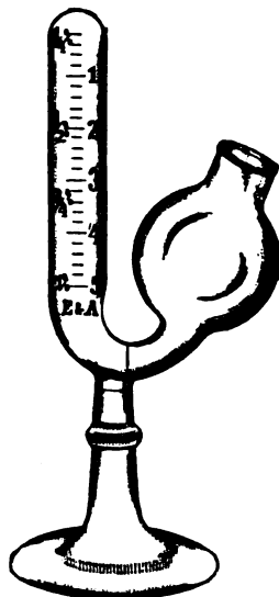
FIG. 5.—EINHORN'S SACCHAROMETER.
