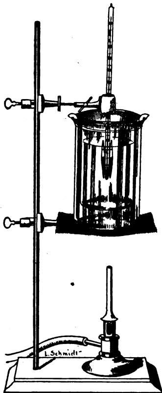
FIG. 60.—MELTING-POINT APPARATUS.
