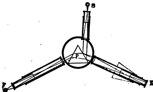
FIG. 99.—DIAGRAM OF ANGULAR-VISION SPECTROSCOPE. (Long.)
