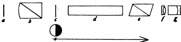
FIG. 7.—DIAGRAMMATIC REPRESENTATION OF THE COURSE OF THE LIGHT THROUGH THE LAURENT POLARISCOPE. (The direction is reversed from that of Fig. 6, p. 31.)
