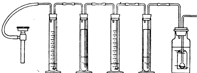
FIG. 90.—ASPIRATION APPARATUS FOR UREA DETERMINATION.
