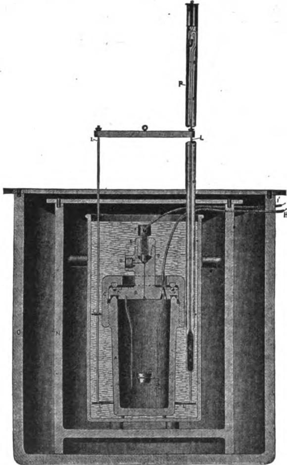
FIG. 192.—BERTHELOT-ATWATER BOMB CALORIMETER.
