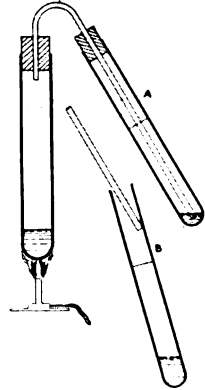
FIG. 88.—APPARATUS FOR DISTILLATION OF AMMONIA FROM UREA. A, FIRST POSITION. B, SECOND POSITION.
