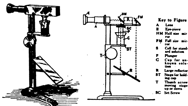
FIG. 161.—BOCK BENEDICT COLORIMETER ILLUSTRATIONS FROM MYERS, "PRACTICAL CHEMICAL ANALYSIS OF BLOOD," ST. LOUIS, 1921.
