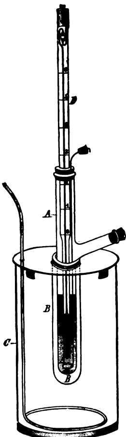
FIG. 122.—BECKMANN-HEIDENHAIN FREEZING-POINT APPARATUS. (Long.)
