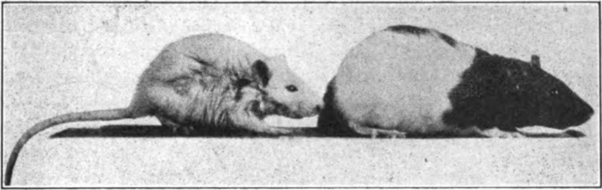
FIG. 175.—RAT FED A DIET DEFICIENT IN FAT-SOLUBLE A (LEFT) AND RAT FED AN ADEQUATE DIET (RIGHT). (From McCollum "The Newer Knowledge of Nutrition.")
