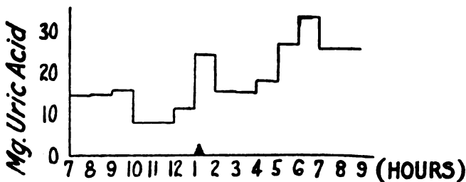
FIG. 190.—INFLUENCE OF PROTEIN INGESTION ON ENDOGENOUS URIC ACID OUTPUT. GLUTEN (130 GRAMS) INGESTED AT 1 P.M. ( Mendel & Stehle: Jour. Biol. Chem. , 22, 215, 1915.)
