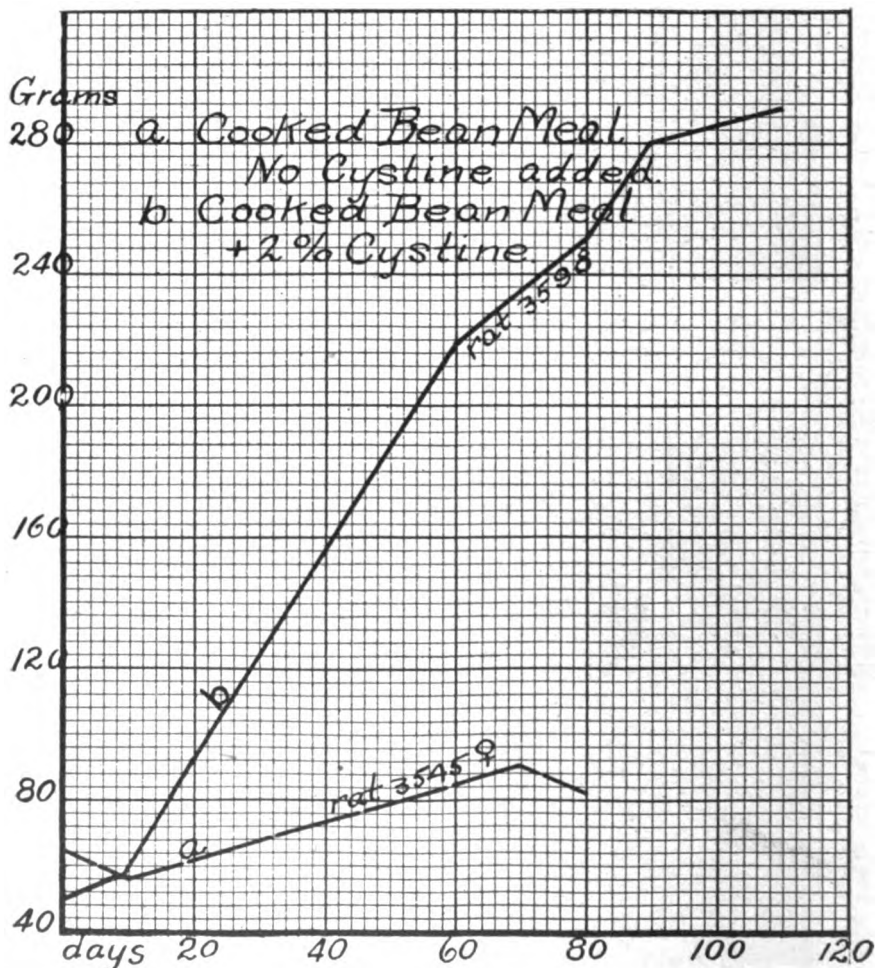
FIG. 183.—CURVE SHOWING INFLUENCE OF A DEFICIENCY OF CYSTINE IN THE DIET. (Johns and Finks: Journal of Biological Chemistry , 41, 379, 1920.)
