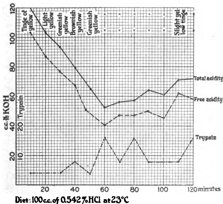
FIG. 49.—INFLUENCE OF ACID INTRODUCED INTO THE NORMAL HUMAN STOMACH. (Spencer, Meyer, Rehffuss and Hawk: American Journal of Physiology , March, 1916.)
