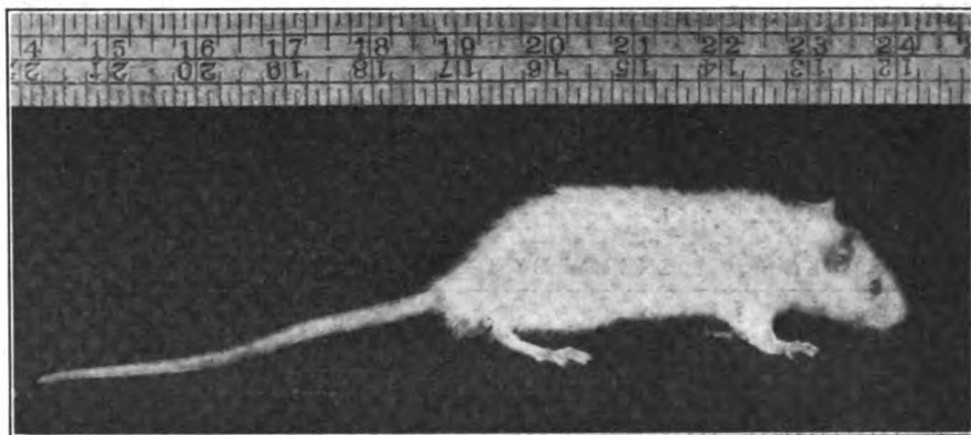
FIG. 186.—RAT RECEIVING WHEAT PROTEIN ONLY. THIS DIET WAS DEFICIENT IN Lysine . COMPARE FIG. 185.
