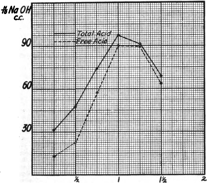
FIG. 43.—CURVES SHOWING STIMULATORY POWER OF BEEF EXTRACT (Plotted from unpublished data collected in the author's laboratory by Professor Chester C. Fowler.)
