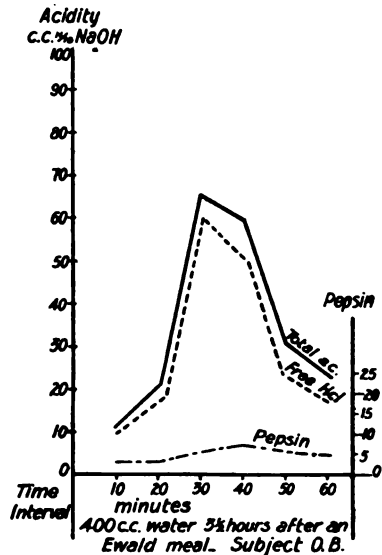
FIG. 42.—CURVES SHOWING STIMULATORY POWER OF WATER. (Bergeim, Rehfuß and Hawk: Journal Biological Chemistry , 19, 345, 1914.)
