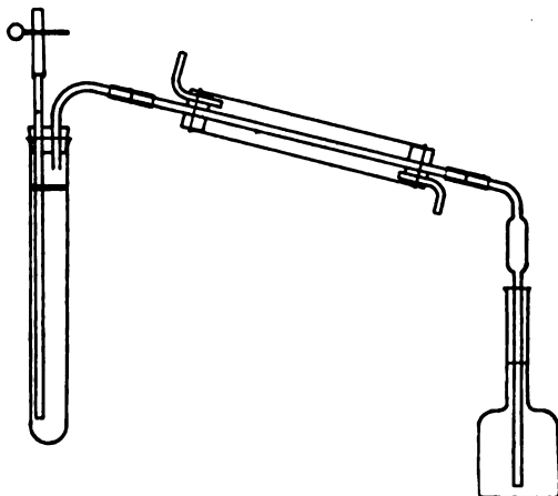
FIG. 165.—BOCK AND BENEDICT APPARATUS.
