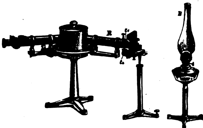
FIG. 98.—ANGULAR-VISION SPECTROSCOPE ARRANGED FOR ABSORPTION ANALYSIS.
