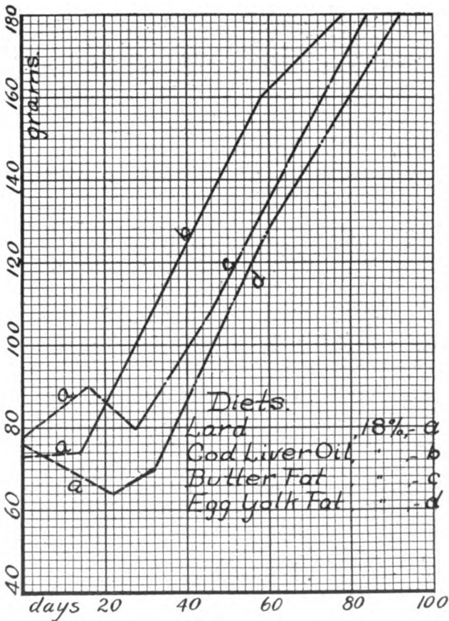
FIG. 176.—THE FAT-SOLUBLE VITAMINE AND GROWTH. THE DIET CONTAINING LARD WAS DEFICIENT IN FAT-SOLUBLE A, WHILE COD LIVER OIL, BUTTER FAT, AND EGG YOLK FAT ARE RICH IN THIS SUBSTANCE. (Osborne and Mendel: Journal of Biological Chemistry , 16, 434, 1913; 17, 405, 1914.)
