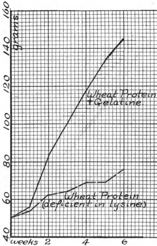
FIG. 184.—CURVE SHOWING INFLUENCE OF A DEFICIENCY OF LYSINE IN THE DIET. (Hawk, Smith and Bergeim: Unpublished data.)
