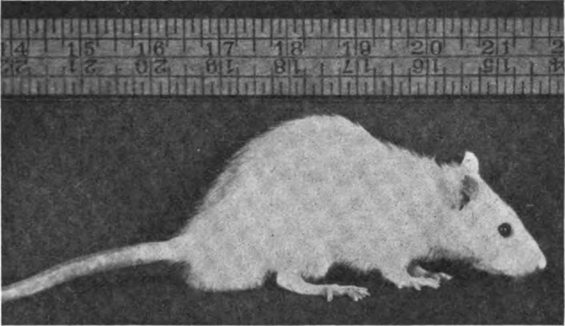
FIG. 172.—RAT (NO. 14) FED A DIET CONTAINING SUFFICIENT WATER-SOLUBLE "B." COMPARE FIG. 173.
