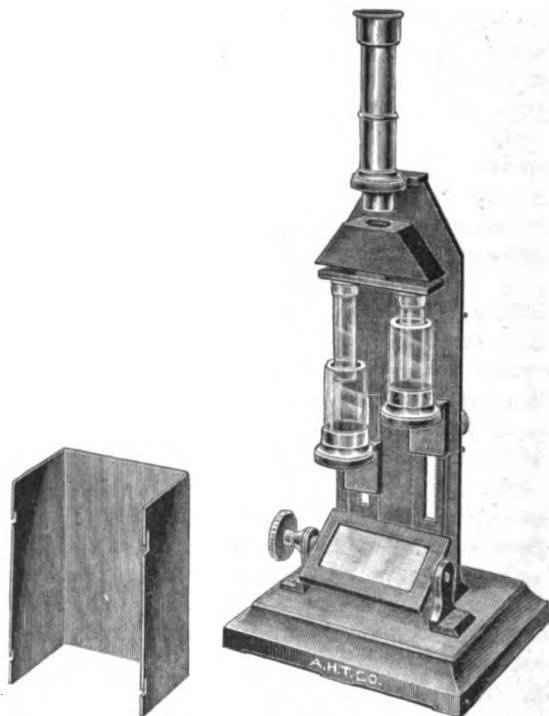
FIG. 160.—DUBOSCQ COLORIMETER.
