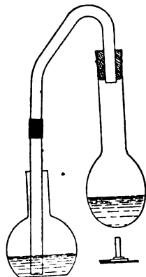
FIG. 159.—FOLIN WRIGHT DISTILLATION APPARATUS. 1
