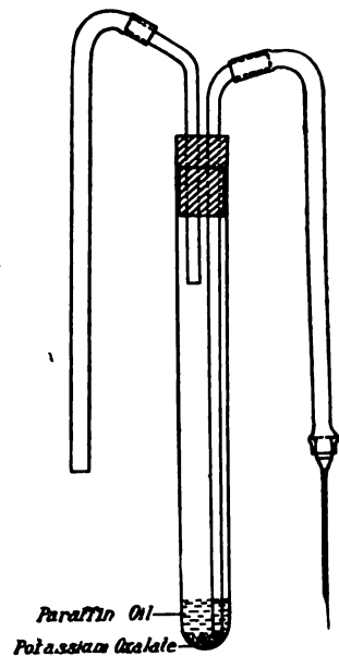
FIG. 101.—TUBE USED IN COLLECTING BLOOD. ( Journal Biological Chemistry , 30, 289, 1917.)
