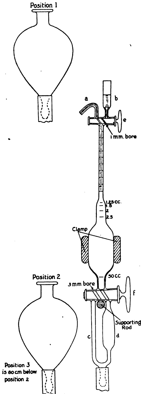
FIG. 100.—VAN SLYKE CARBON DIOXIDE APPARATUS. ( Journal Biological Chemistry , 30, 289, 1917; 30, 347, 1917.)
