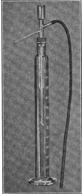
FIG. 112.—CROLL'S FAT APPARATUS
