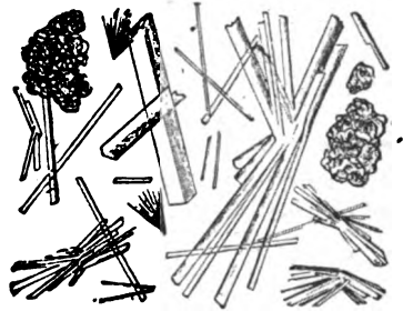
FIG. 133.—CALCIUM SULPHATE. (Hensel and Weil.)
