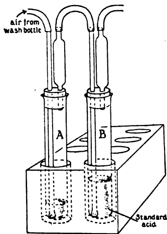
FIG. 166.—VAN SLYKE AND CULLEN APPARATUS.
