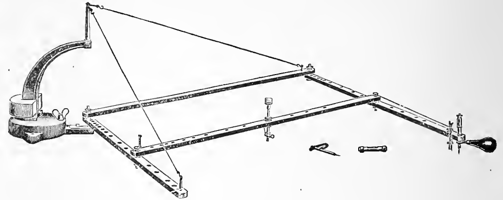
Fig. 52. Pantograph.
