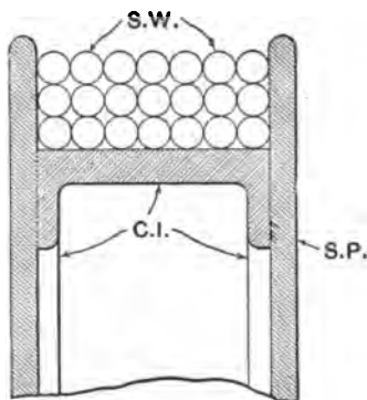
CROSS SECTION S.W. — Steel Wire S.P. — Steel Plates C.I. — Cast Iron
