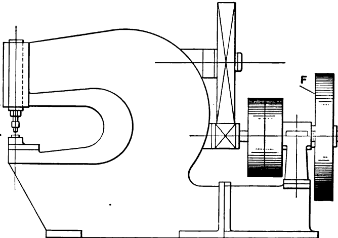
Fig. 29. Single-ended Punch
