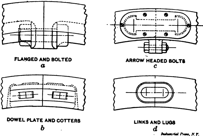
Fig. 16. Additional Types of Rim Joints
