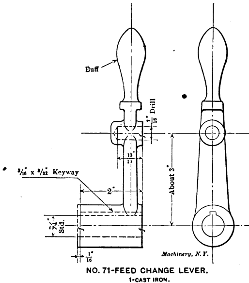
Fig. 8. Detail Drawing
