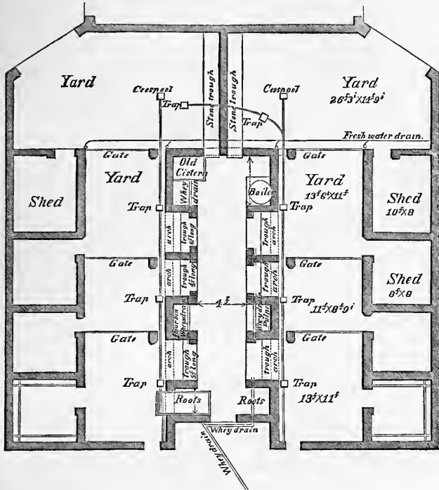
Fig. 44.—GROUND PLAN OF TATTENHALL PIGGERY.
