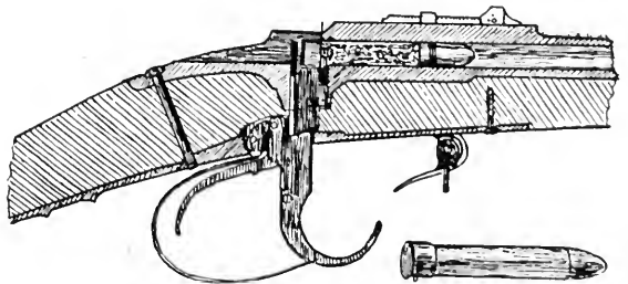
Early French Military Breech-loader.
