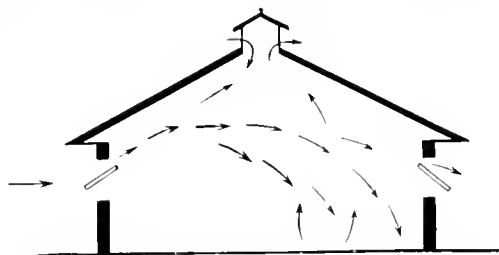
Fig. 467.—Direction taken by Air-currents when opposite Windows are half-open
