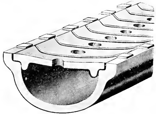
Fig. 471.—Covered Surface-drain
