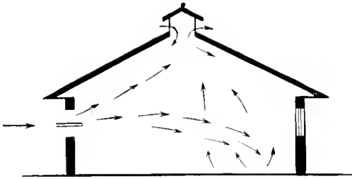
Fig. 464.—Direction taken by Air-currents with the Windward Windows open
