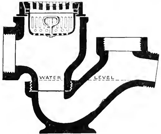
Fig. 475.—Winser's Stoneware Gully
