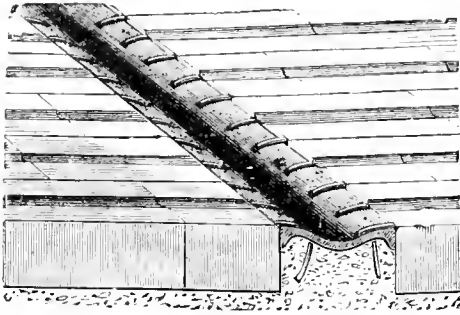
Fig. 470.—Wrought-iron Open Gutter (St. Pancras Ironworks Co.)
