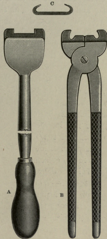
Fig. 389.—Tools for Clamping Sand Crack
