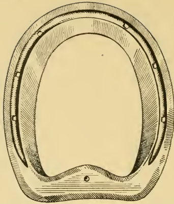
Front Shoe, Wide Web, Heavy Bevel and Crease, Flat Wide Bar—10 Ounces. For Scalper.
