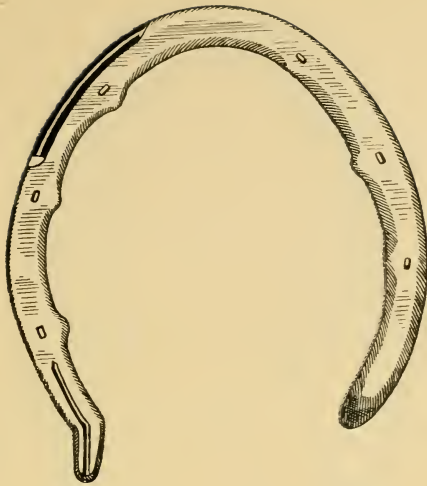
Another Pattern Cross-fire Shoe, Brazed Outside Grab and Heel Calk, Plain Inside— 3\frac{1}{2} Ounces.
