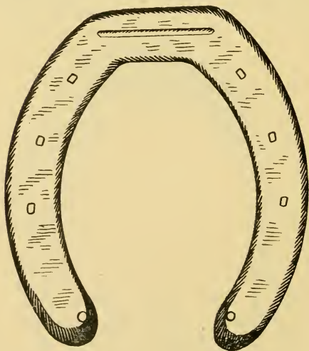
Square-Toed Front Shoe, Creased Toe, Beveled Edges—7½ Ounces.
