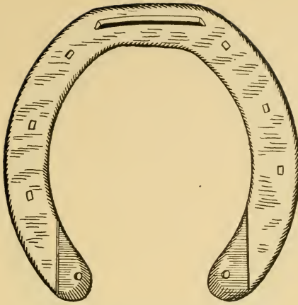
Front Shoe, Creased Toe, Set-Calks, Slightly Rounded Edges and Toe Squared— 6\frac{1}{2} Ounces.
