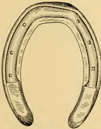
Heavily Grooved Front Shoe, Rolled Off at Outside Toe, Flat Heels, Beveled Sides and Heels—5½ Ounces.
