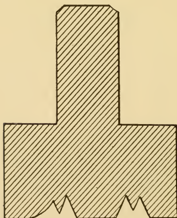
Double Swedge for Light Front and Heavy Hind Shoe.
