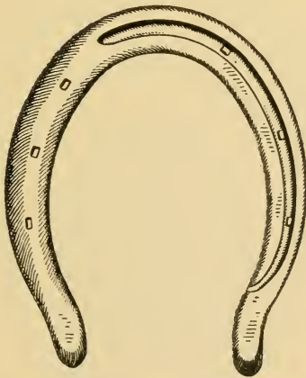
Outside-Swedged Cross-firing Shoe, Inside Half-Oval, No Heel Calks. For Trotters and Pacers—5 Ounces.
