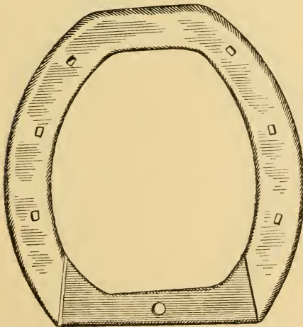
Front Bar-Shoe, Square Toe, Beveled Sides, Toe Broke Over, Long Fine Set-Calks—5 Ounces.
