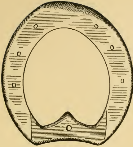
Front Shoe, Wide Web and Bar, Fine Set-Calks, Rolled Outside Toe and Sides—10 Ounces.
