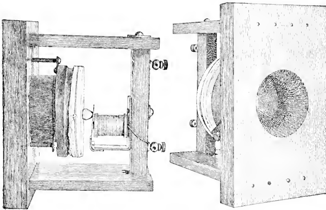
Side and front views of Bell's first Telephone The instrument shown at the Centennial Exposition
