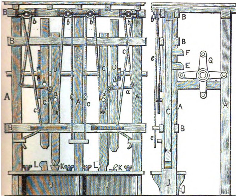
Wedge Press—Front and Side Elevation.
