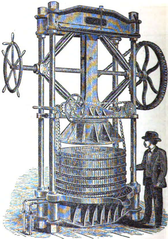
Fig. 31.—Elbow Press.
