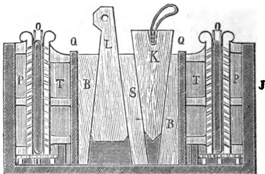
Fig. 37.—Wedge Press—Longitudinal Section of Lower Portion.
