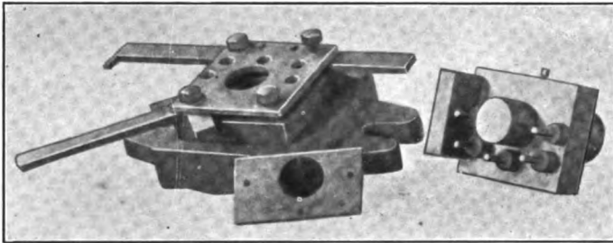
FIG. 153. — A piercing and cutting-off die
