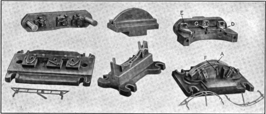
FIG. 372. — Dies for forming the universal bar
