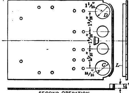
SECOND OPERATION PIERCING HOLES C-D AND FORMING UP LIP L AT END
