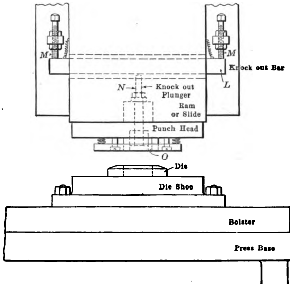
Fig. 134. — Application of positive “knock out”
