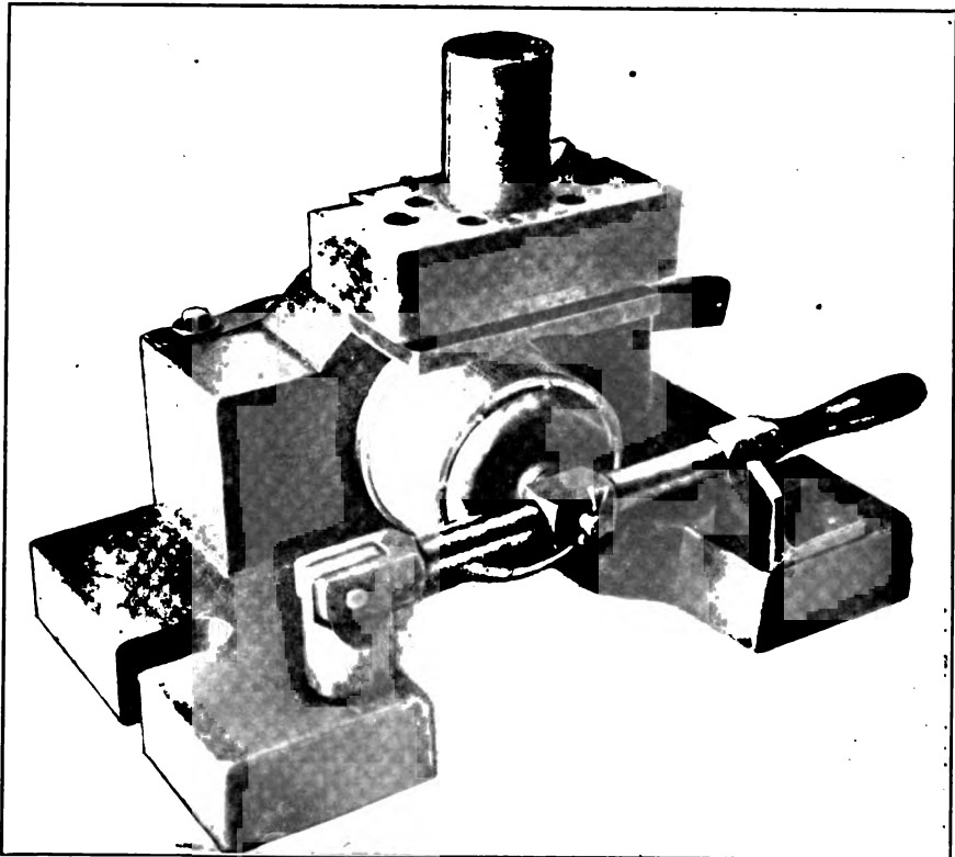
FIG. 460. — Indexing die with work in place
