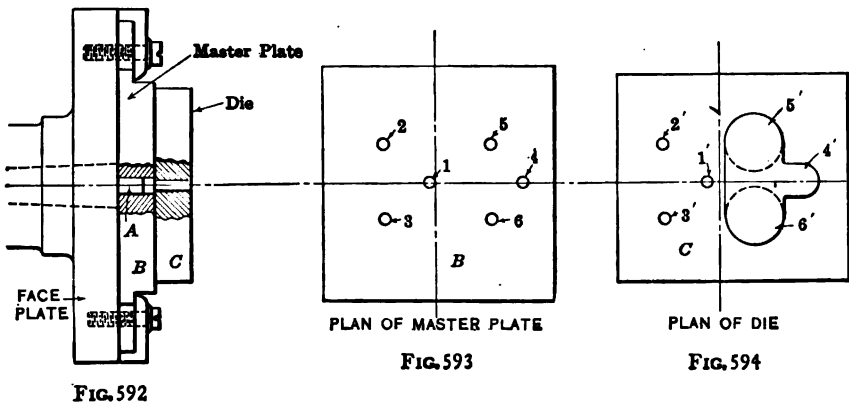
FIGS. 592-594. — The use of the master plate
