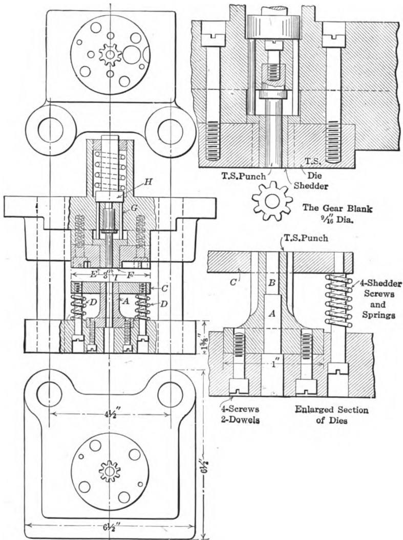
FIG. 136. — Compound dies for making a small gear
