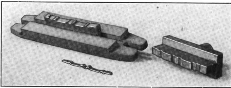
FIG. 336. — The first operation forming tools
