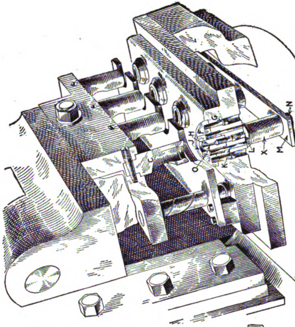
Figs. 263-265. — Gang drawing dies
