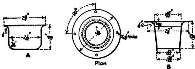
FIG. 307. — Brass coupling, No. 20 gage
