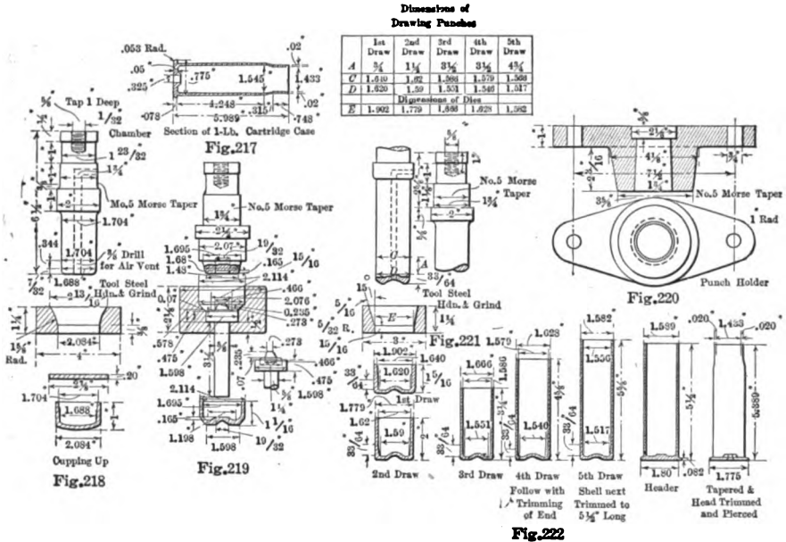
FIGS. 217-222. — Tools for drawing 1 lb. cartridge cases
