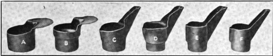
FIG. 251. — Steps in making an oil can spout
