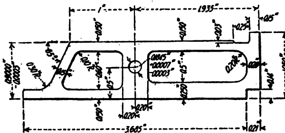
FIG. 440. — Detail of type bar
