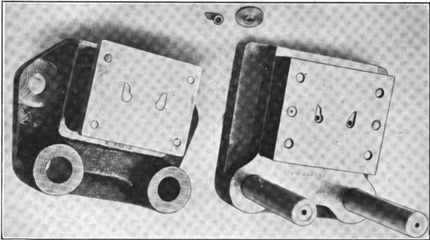
FIG. 185. — Dies for trimming cams from a disk
