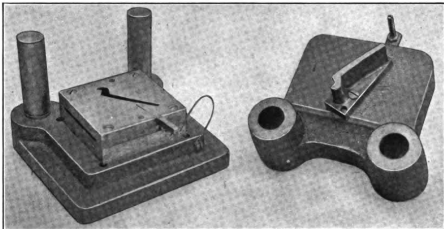
FIG. 48. — Dies made with diagonally placed opening
