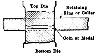
FIG. 26. — Coining dies
