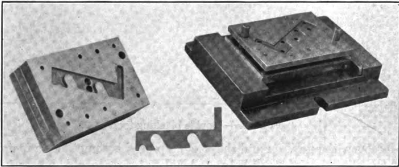
Fig. 67. — Another blanking die with combined pressure pad and close fitting stripper
