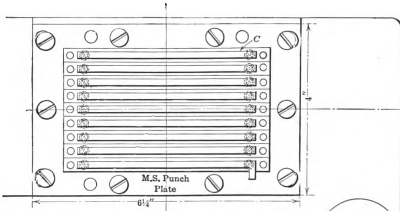
PLAN OF PUNCH FIG. 116
