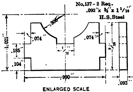
FIG. 447. — Spacing piece for a coin wheel
