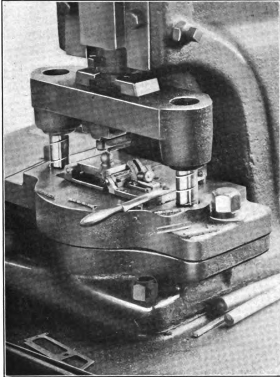
FIG. 446. — Piercing for type rivets
