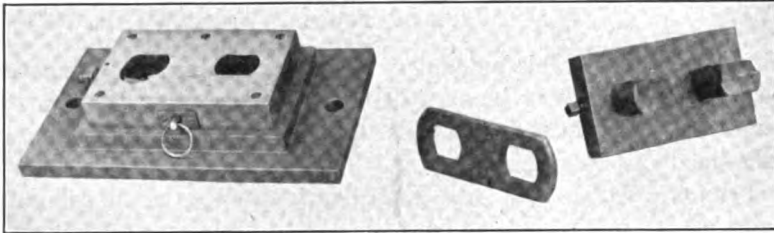
FIG. 85. — Double tools for piercing a link
