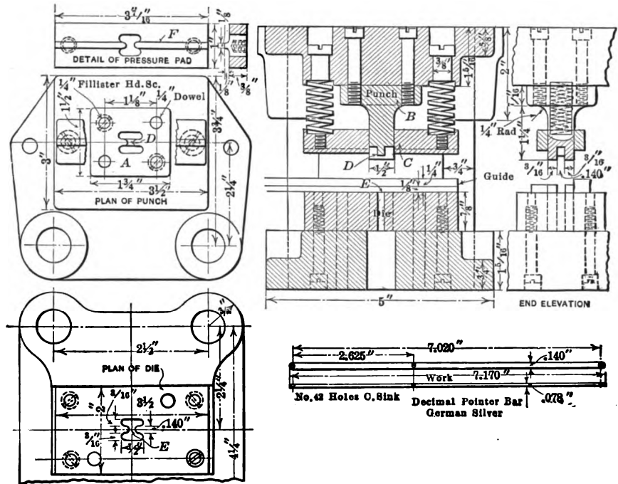
FIGS. 159-160. — Details of parting dies shown in Fig. 158
