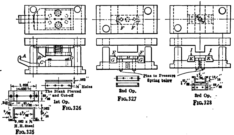
FIGS. 325-328. — Dies for double bending operation
