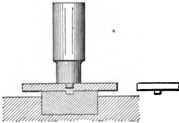
FIG. 28. — Extruding tools
