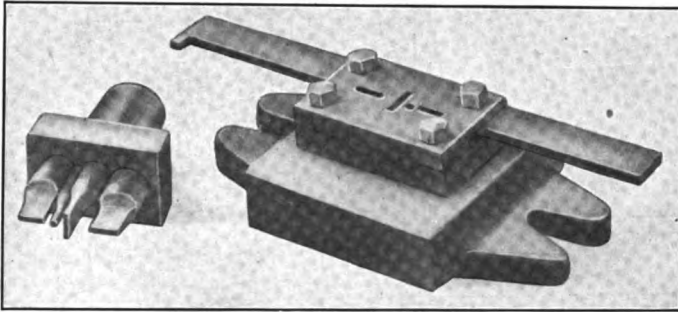
FIG. 156. — Slotting and cutting-off tools.
