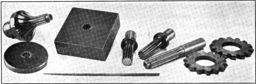
FIG. 600. — The punch, the die, the broaches and lap
