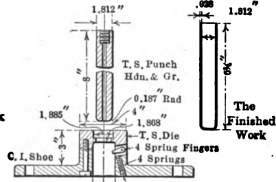
FIG. 262 4th Operation 3rd Redraw
