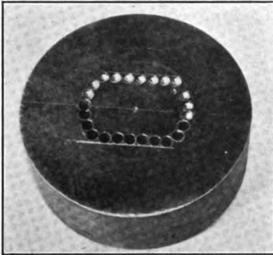
FIG. 556. — Series of holes in drilling out a die opening
