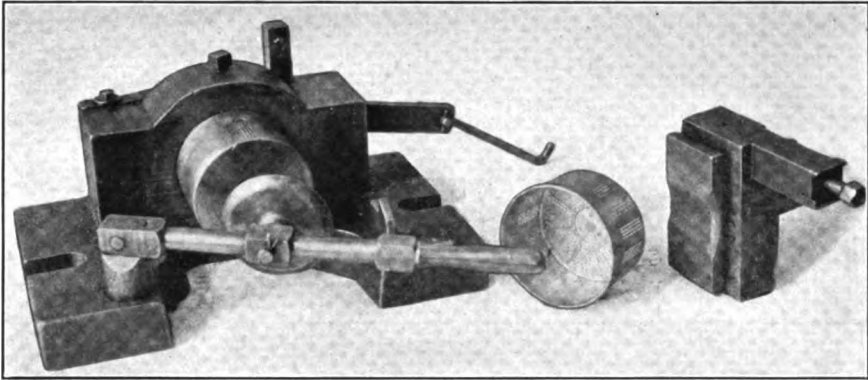
FIG. 459. — An indexing perforating die
