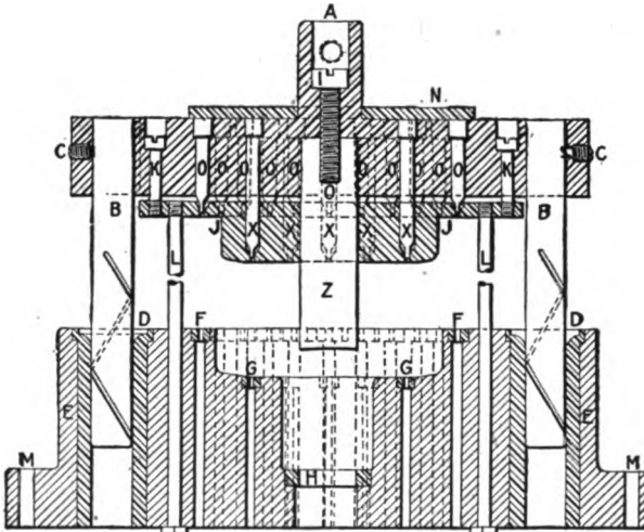
FIG. 271. — Eighth operation
