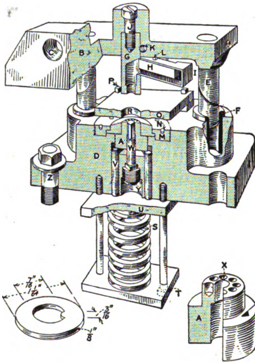
FIG. 152. — Lock washer tools
