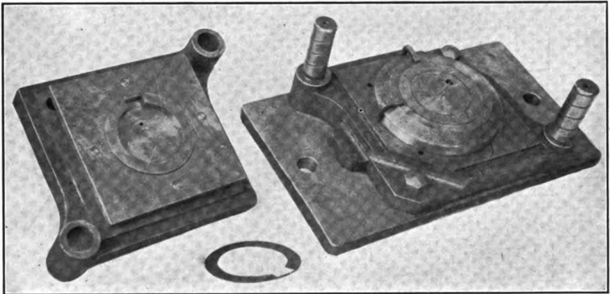
FIG. 137. — Dies for thin washer with keyway punched out
