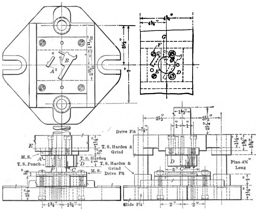
FIG. 104. — Piercing and blanking tools for a typewriter part
