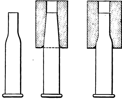
FIG. 18. — Reducing dies
