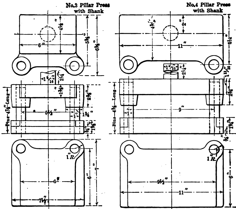
FIGS. 485-486. — Standard parts for pillar dies
