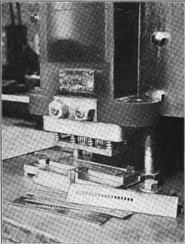
FIG. 390. — Piercing dies in the press
