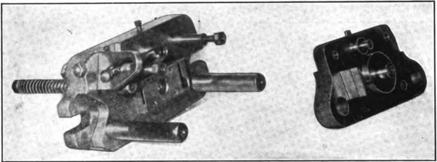
FIG. 468. — Transfer device for compound die
