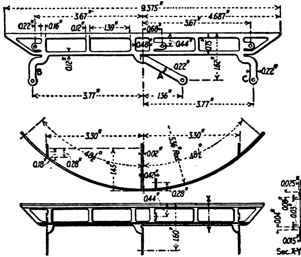
FIG. 368. — Details of universal bar for typewriter
