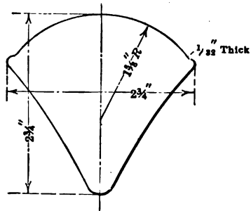
FIG. 32. — The blank produced in the tools in Fig. 31
