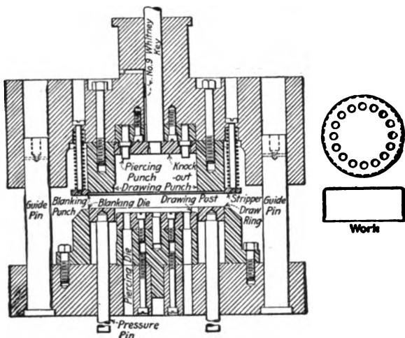
FIG. 306. — Blanking, drawing, forming, and piercing die
