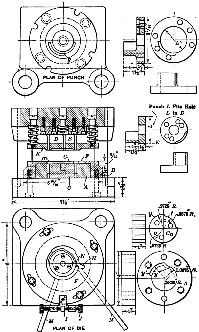
FIG. 178. — Details of slot shaving die
