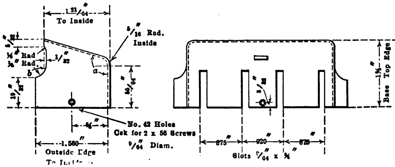
FIG. 405. — Detail of carriage cover for calculating machine
