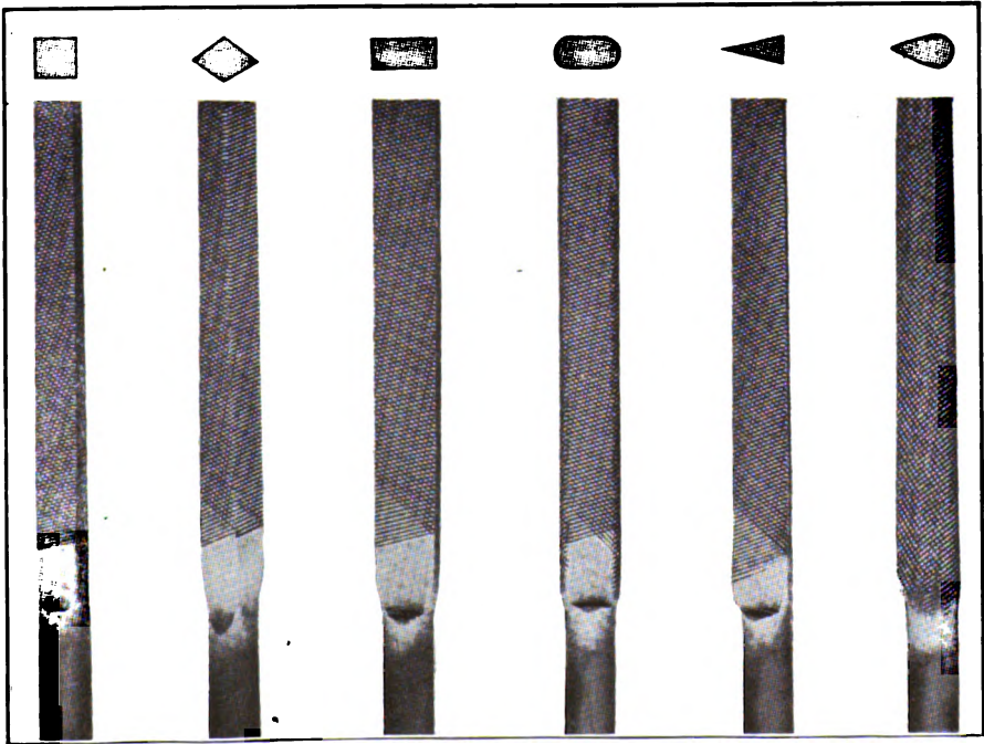
FIG. 570. — Bench filing machine files (Disston)
