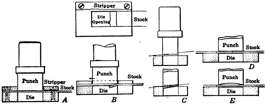
FIG. 7. — Action of punch and die on the stock
