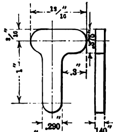
Fig. 45. — A three lobe blank
