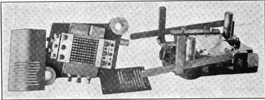
FIG. 437. — Dies for stamping numerals
