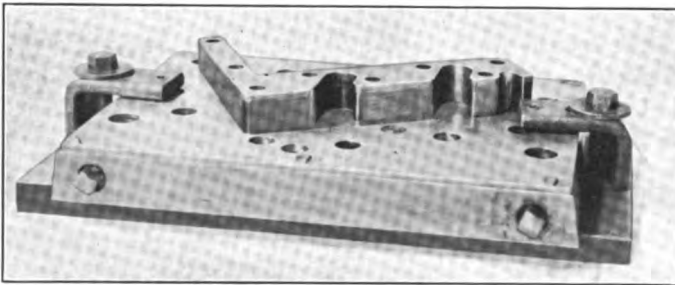
FIG. 563. — Adaptor for grinding shear on blanking punch
