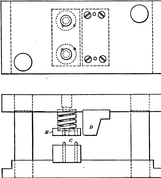
FIG. 330. — Bending dies for a light bracket
