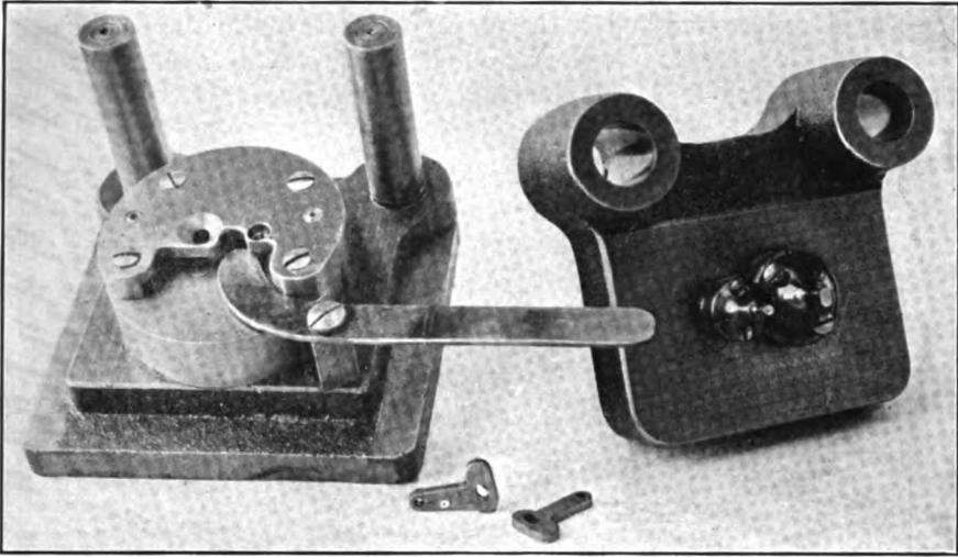
FIG. 94. — Piercing tools for blank with two holes
