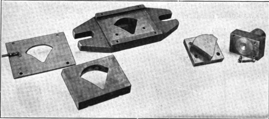
FIG. 31. — Blanking tools taken apart
