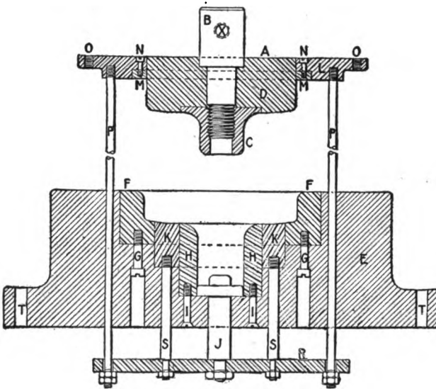
FIG. 269. — Sixth operation
