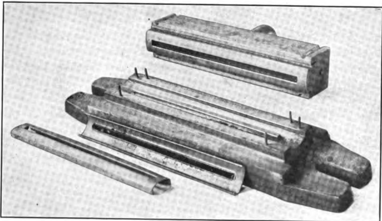
FIG. 362. — Forming tools that follow the slitting die
