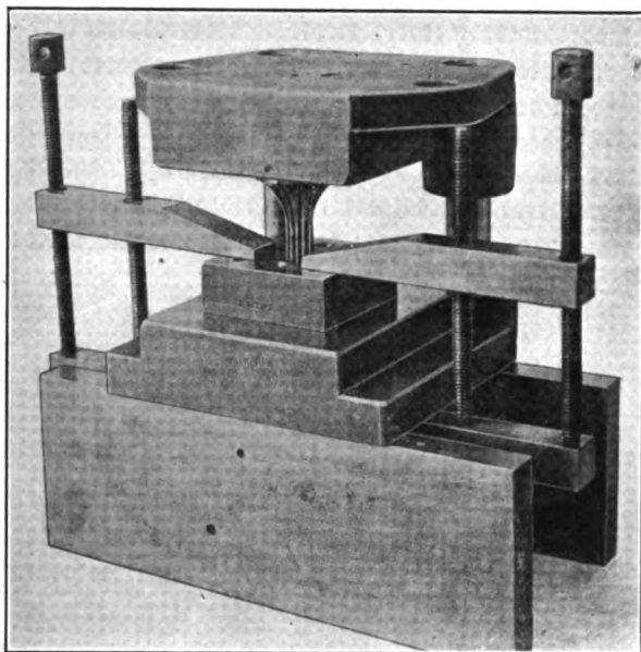
FIG. 604. — Clamping the die in line with the punch for drilling holes in base
