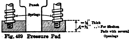
FIGS. 487-490. — Pressure pad and nest details
