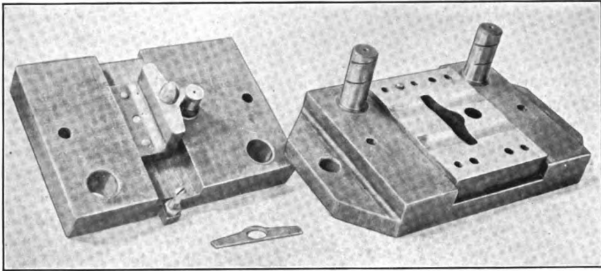
FIG. 103. — Progressive tools with sheared die face
