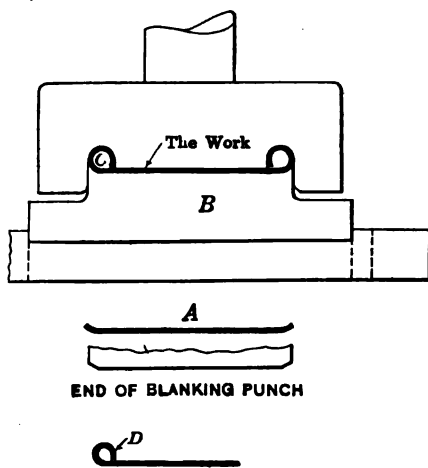
FIG. 367. — Curling operation
