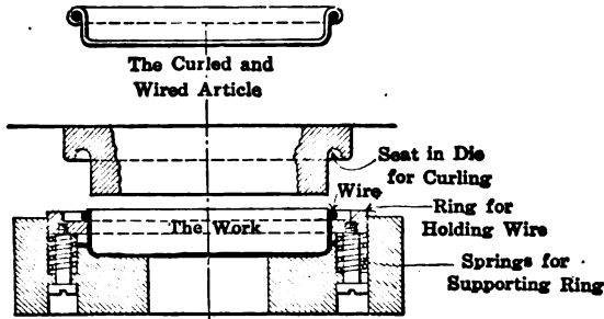
FIG. 23. — Curling and wiring dies
