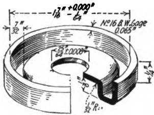
FIG. 304. — The spring cup to be made
