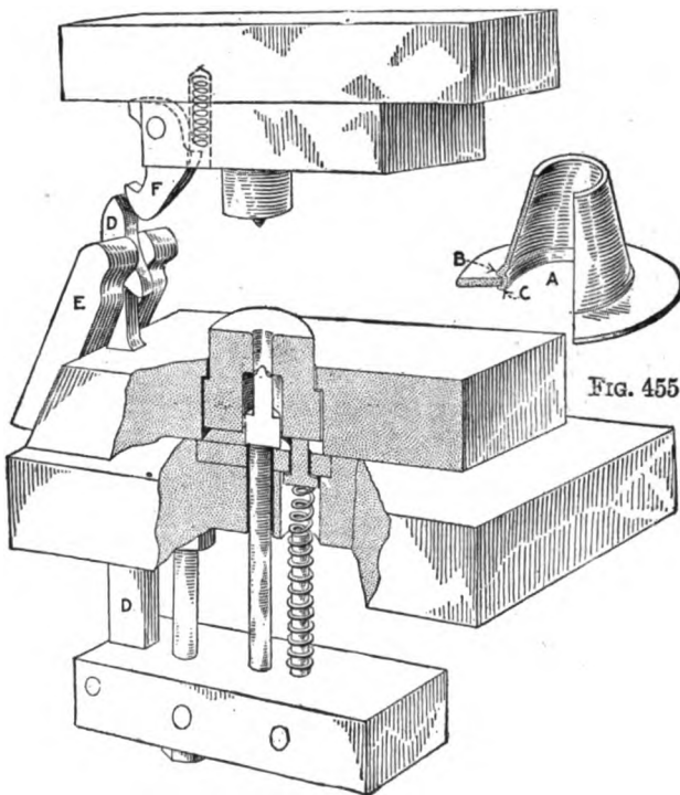
FIGS. 454-455. — Swaging dies
