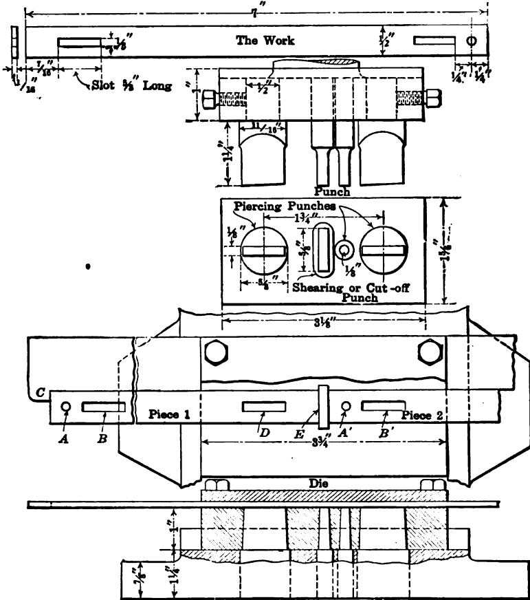
FIG. 157. — Slotting and cutting-off tools
