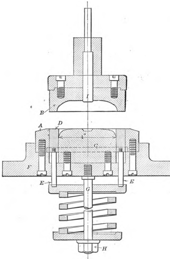
FIG. 286. — Section through combination die
