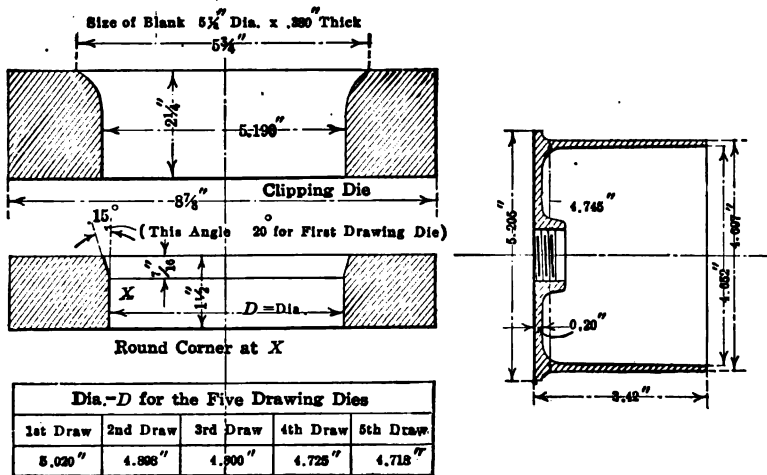
FIG. 230. — Drawing dies for 4.5 Howitzer cases
