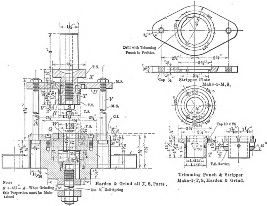
FIG. 314. — Construction of trimming dies
