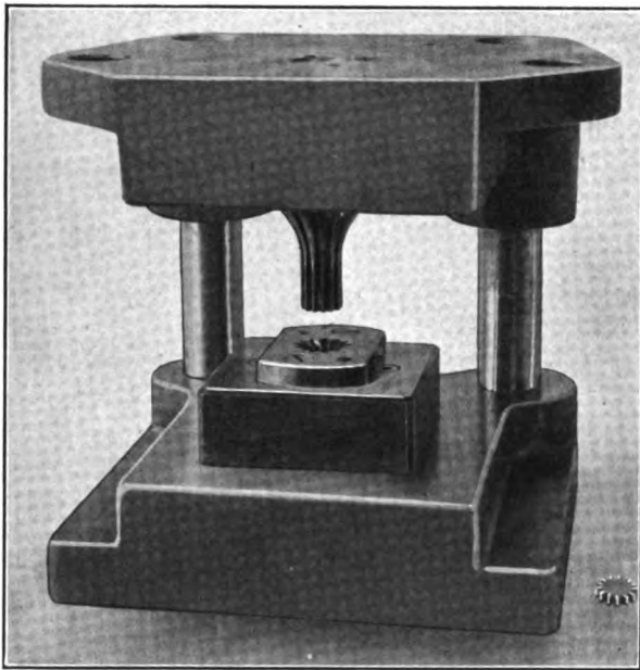
FIG. 596. — The shaving tools
