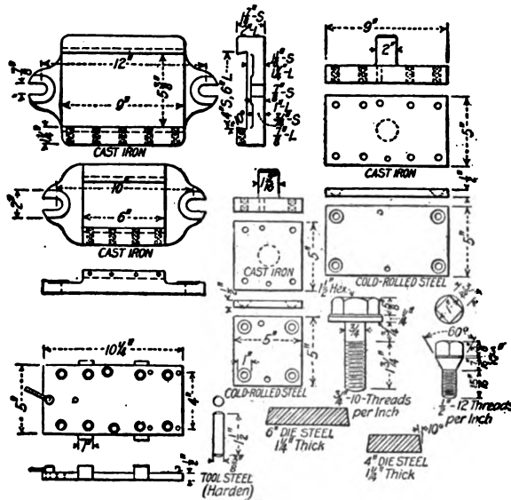
FIG. 537. — Die shoe, punch holder and drill jig
