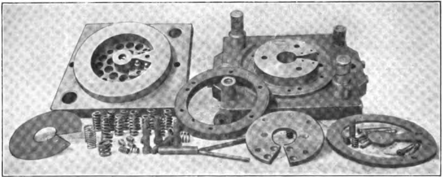
FIG. 140. — The dies taken apart
