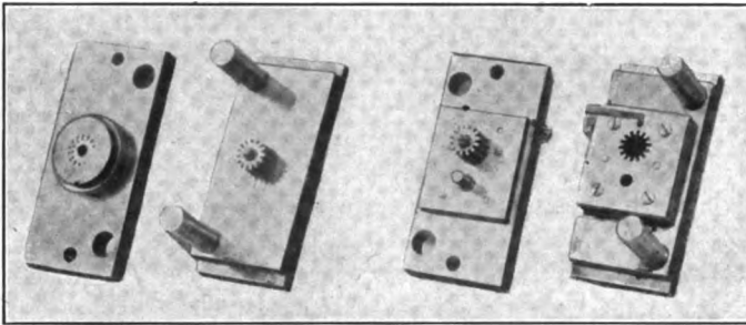
FIG. 170. — Dies for making a gear wheel
