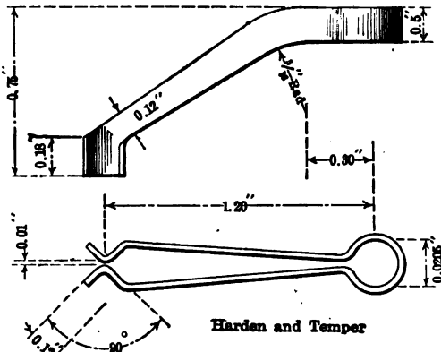
Fig. 382. — Detail of small spring
