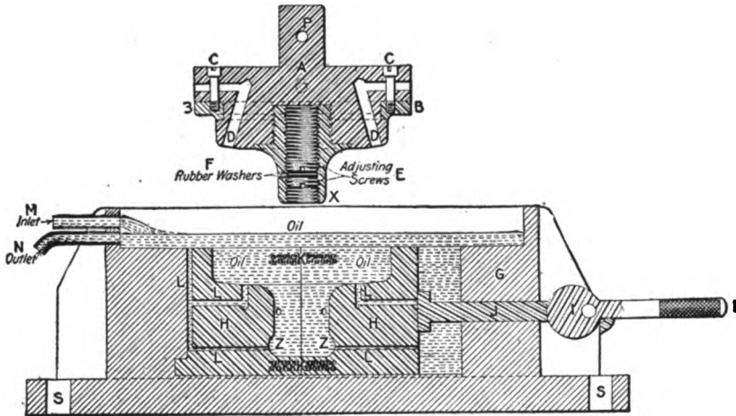
FIG. 270. — Seventh operation
