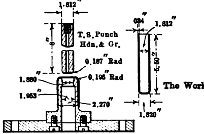
FIG. 261 3rd Operation 2nd Redraw Die
