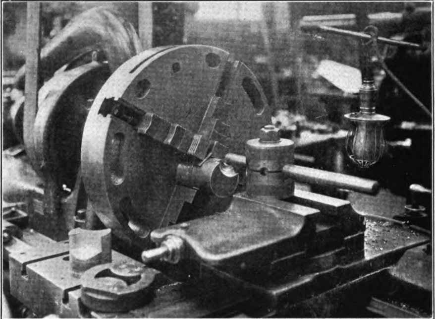
FIG. 577. — Making a punch in the lathe
