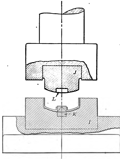
FIG. 363. — End view of forming die
