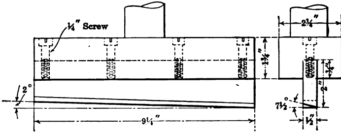
FIG. 184. — Trimming tools
