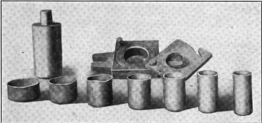
FIG. 278. — Shells drawn with cast iron punches and dies
