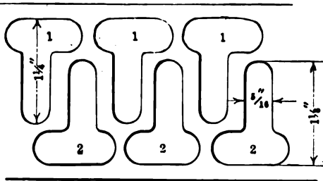
FIG. 47. — Blanking in double run through the press
