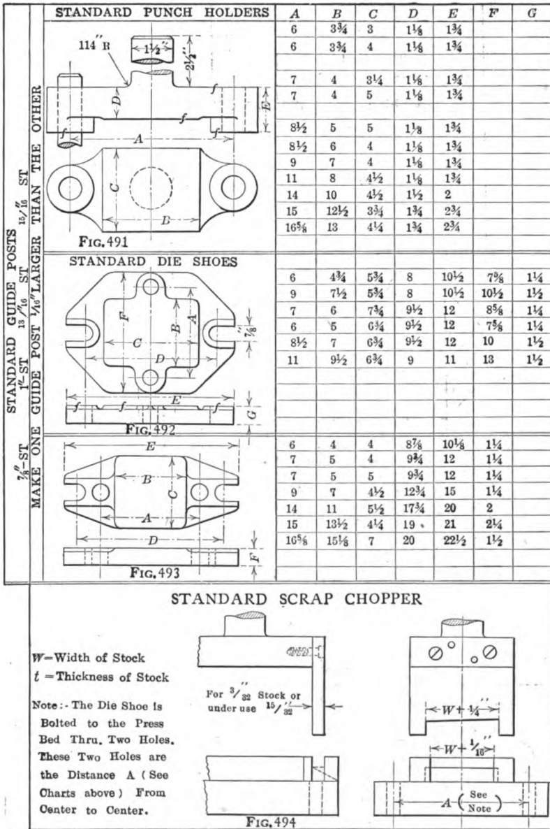
Figs. 491-494. — Standard die shoes and punch holders
