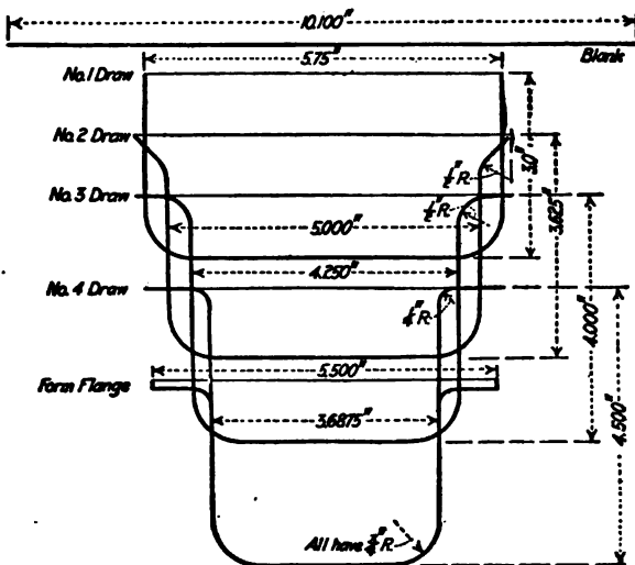
FIG. 238. — Drawing a flanged shell
