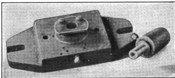
FIG. 80. — Simple piercing tools
