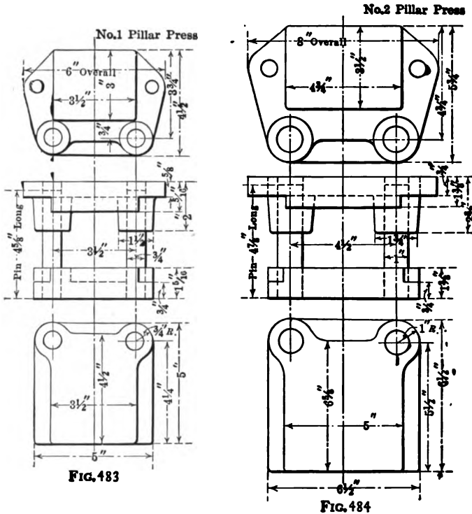
Figs. 483-484. — Standard parts for pillar dies
