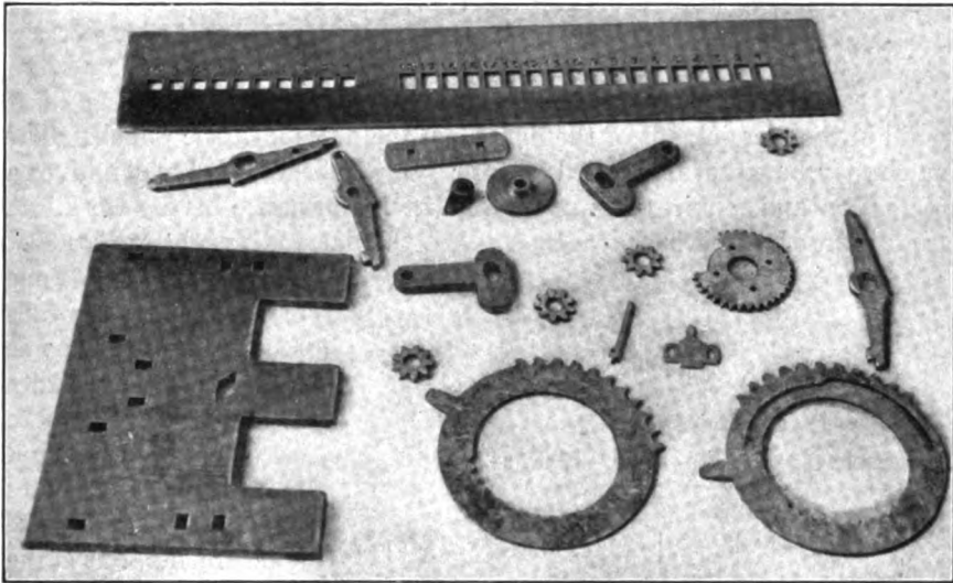
FIG. 79. — Examples of blanked and pierced work
