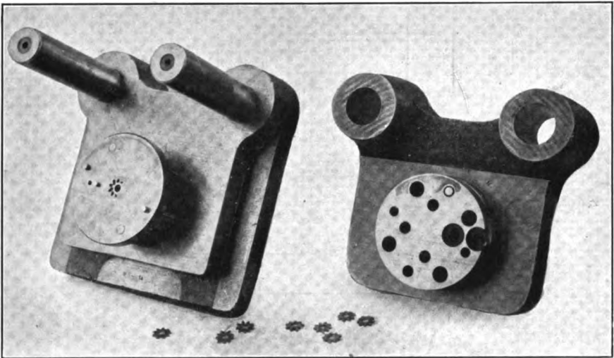
Fig. 135. — Compound dies for making a small gear
