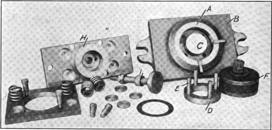
FIG. 132. — Showing details of tools in Fig. 131
