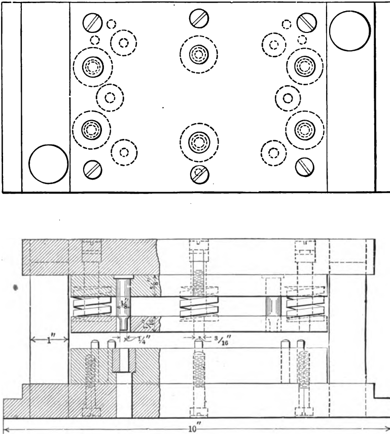
FIG. 110. — Multiple piercing tools for a sheared plate
