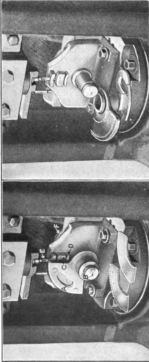
FIG. 463 FIGS. 463-464. — Indexing die for notching a typewriter comb
