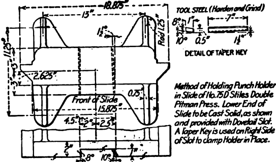
Fig. 528. — Punch holder for No. 75-D press
