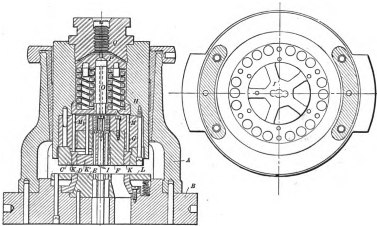
Fig. 478. — Construction of sub press with compound clock wheel dies
