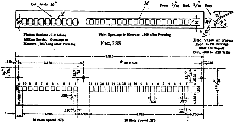
FIGS. 387-388. — Detail of cover plate
