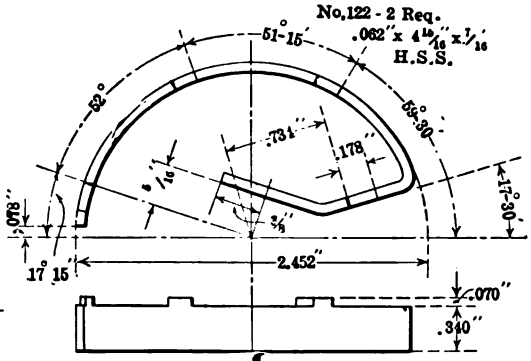
FIG. 448. — Coin wheel member
