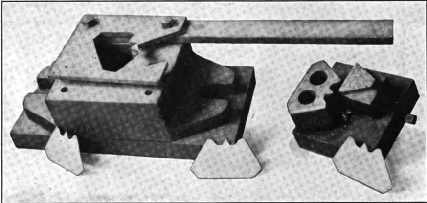
FIG. 341. — Progressive stamping and blanking dies
