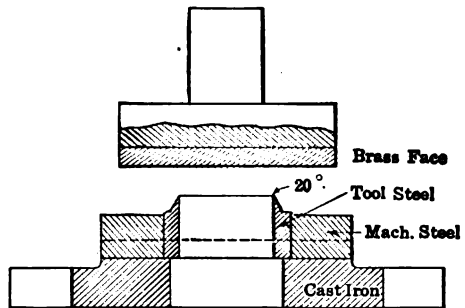
FIG. 16. — Dies for blanking fiber
