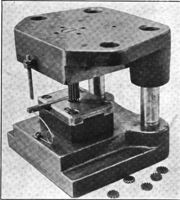
FIG. 33. — A wheel blanking die of the sub-press type
