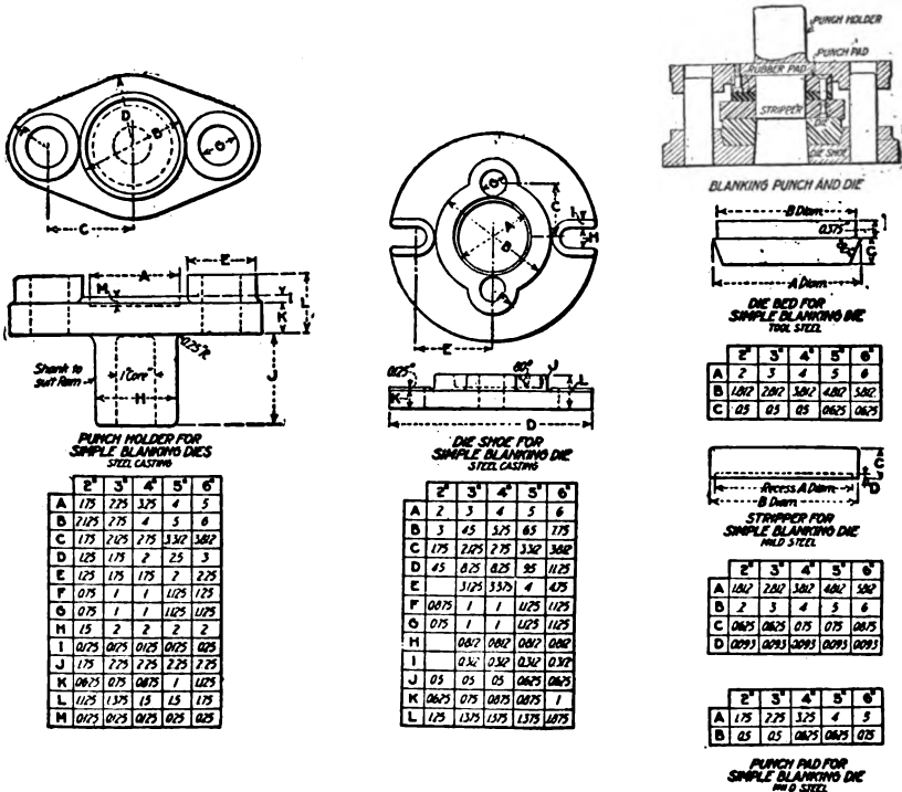
Fig. 532. — Simple blanking punch holder, die shoe and details
