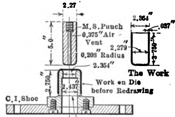
FIG. 260 2nd Operation 1st Redraw Die
