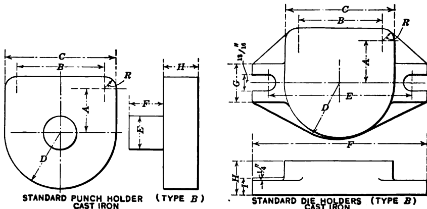
FIG. 495. — Punch and die standards
