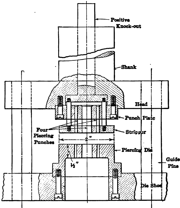
FIG. 301. — The piercing tools
