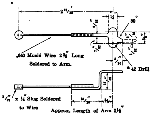
FIG. 320. — The piece bent in the dies Fig. 319
