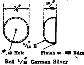
FIG. 296. — Detail of bell
