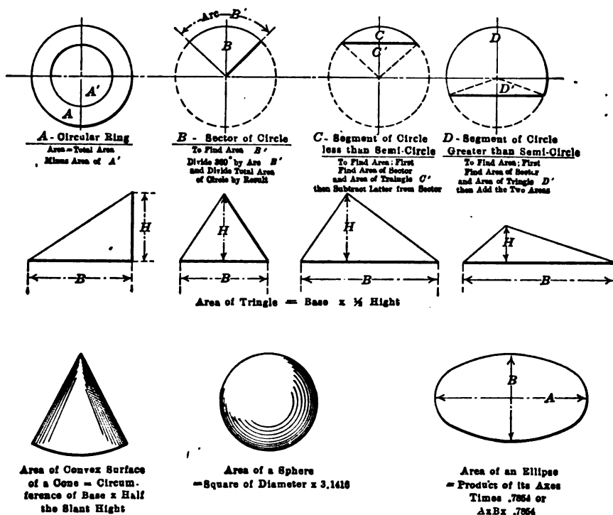
FIG. 538. — Plane surfaces, and cones and spheres
