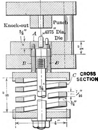
FIG. 169 FIGS. 168-169. — Sectional view of shaving dies
