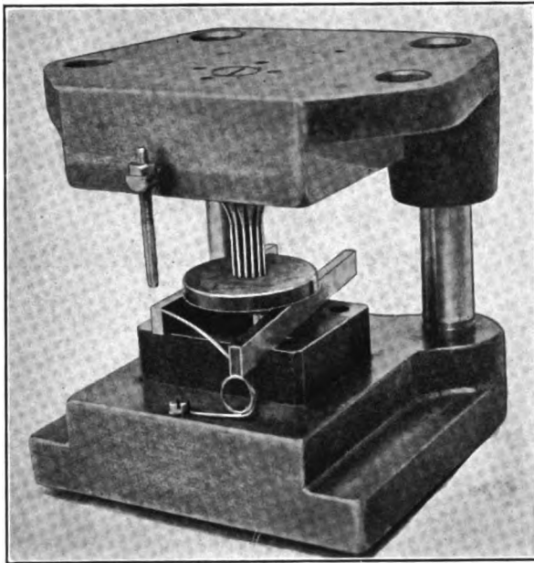
FIG. 609. — Broaching out the nest
