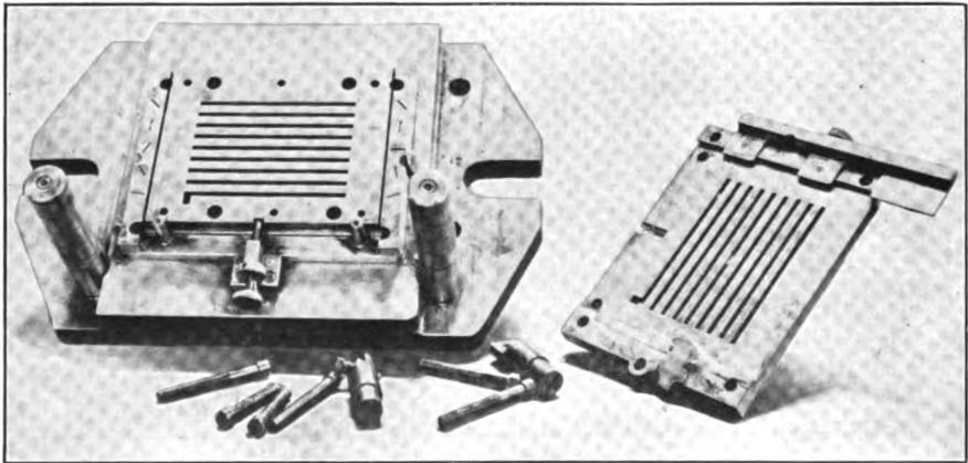
FIG. 114. — Sectional slot die details
