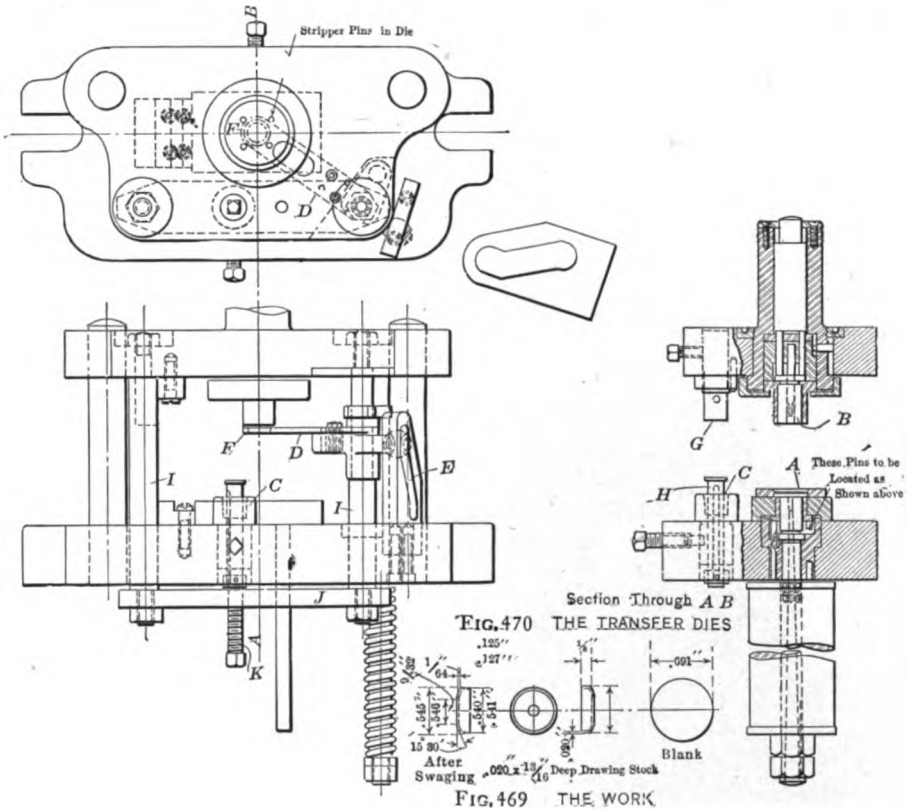
Figs. 469-470. — Transfer dies for a cup
