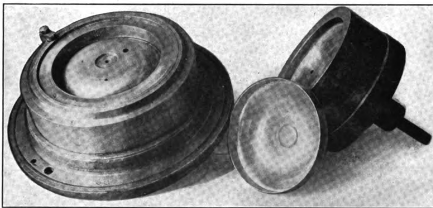
FIG. 285. — Combination dies for blanking and forming a shallow cover
