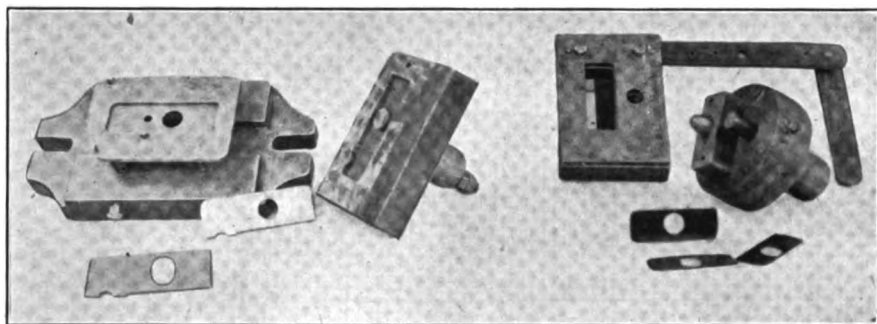
Fig. 128. — Compound piercing and blanking dies
