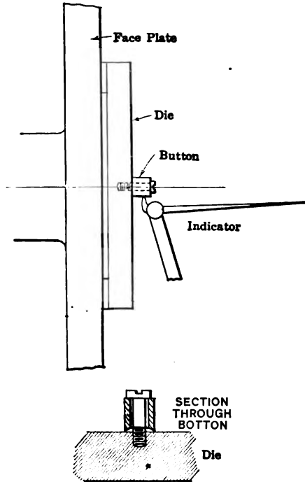
FIG. 583. — Application of the locating button and test indicator
