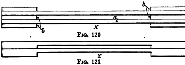
Figs. 120-121. — Other possible forms of die sections
