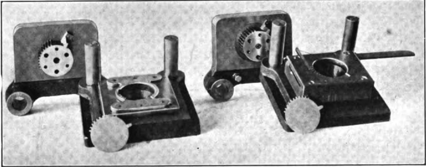
FIG. 173. — Blanking die and a shaving die for outside of work
