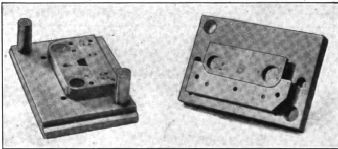
FIG. 419. — Tools for forming flange at end of work
