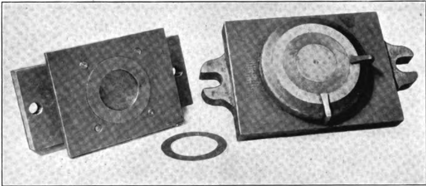
FIG. 131. — Dies for thin ring or washer
