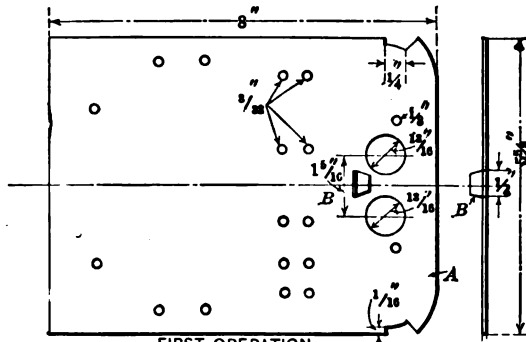
FIG. 417 FIRST OPERATION TRIMMING END A AND PIERCING HOLES AND FORMING TONGUE B
