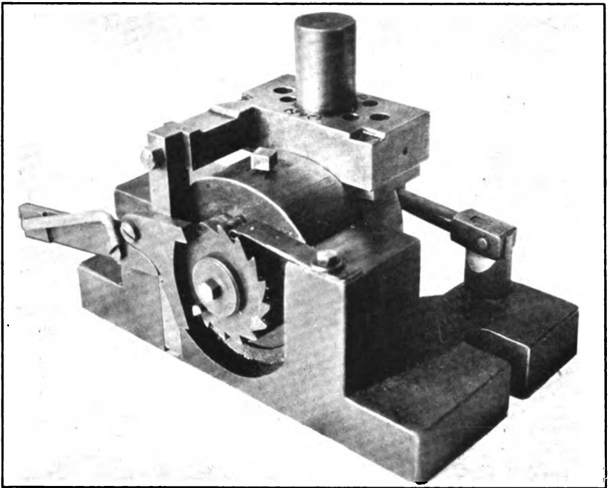
FIG. 461. — Mechanism at rear of indexing die
