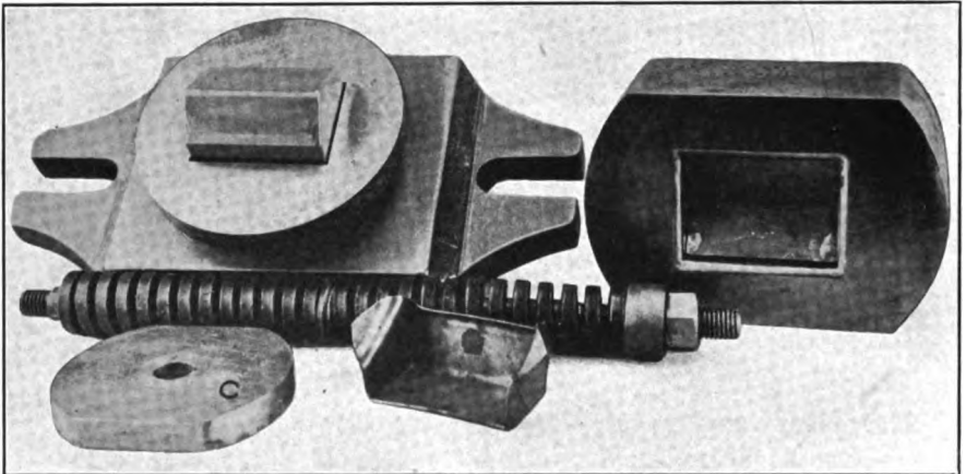
FIG. 407. — Tools for second draw
