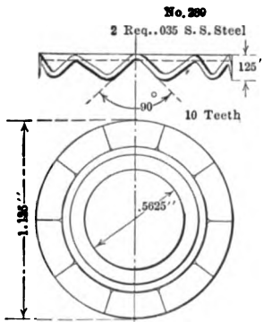
FIG. 433. — Embossed disk
