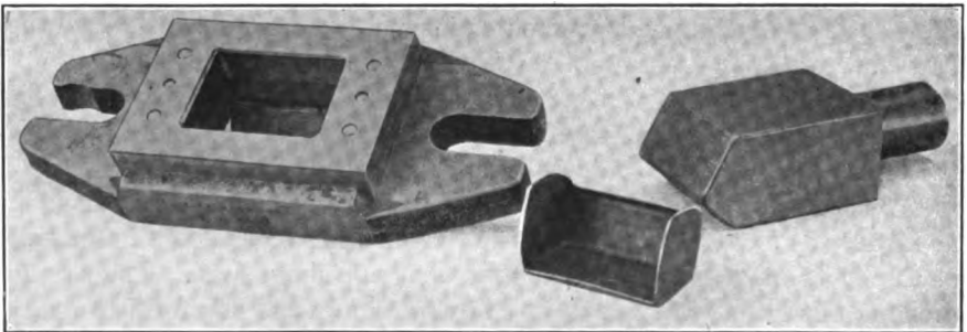
FIG. 408. — "Push through" dies for third draw
