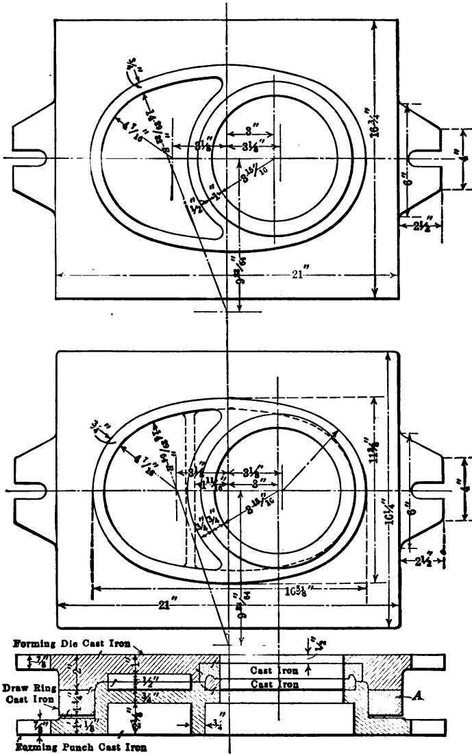
Fig. 281. — Tools for large metal cover
