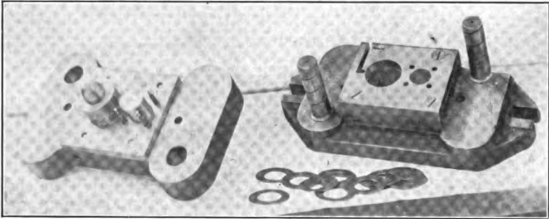
FIG. 96. — Progressive piercing and blanking dies for a special washer
