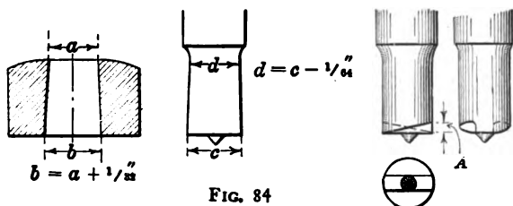
FIGS. 81-84. — Punch dies for plate work
