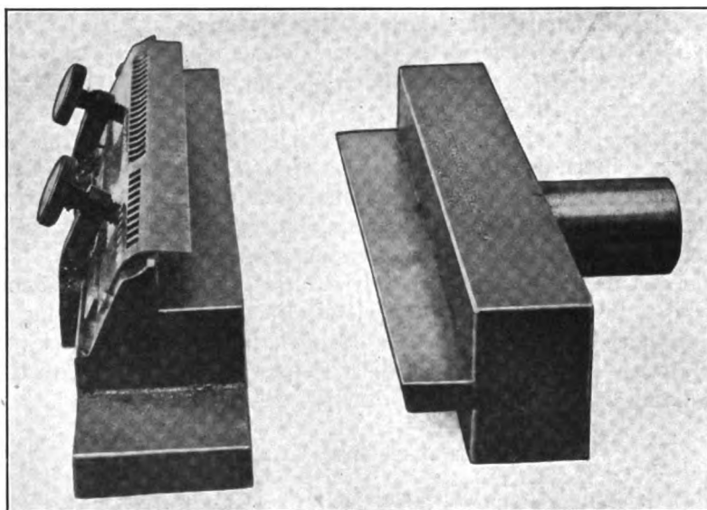
FIG. 183. — Trimming tools
