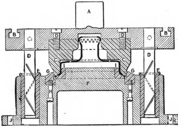
FIG. 272. — Ninth operation
