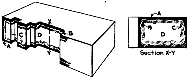
FIG. 616. — Diagrammatic section of a solid die, showing areas and lines of hardness must be uniformly hard from top to bottom. That this condition did not exist in many dies as ordinarily made has been proved time and again.
