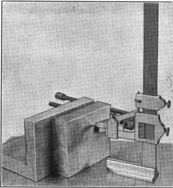
FIG. 551. — Vernier height gage used in laying out dies
