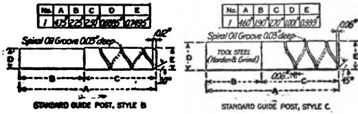
Figs. 530-531. — Standard guide posts
