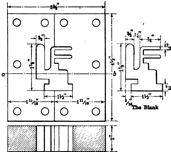
FIG. 6. — Sectional die made in halves
