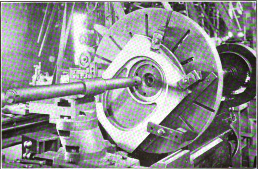
FIG. 580. — Making large dies
