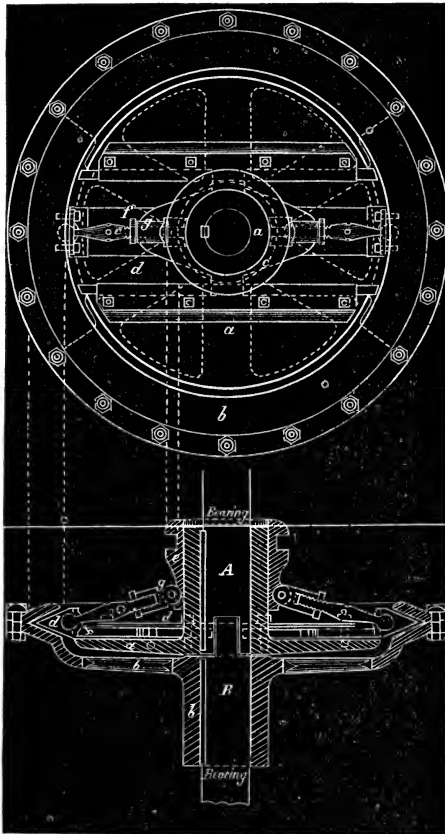
FIG. 117.—Thirty-six inch Friction Coupling, one-twelfth size.
