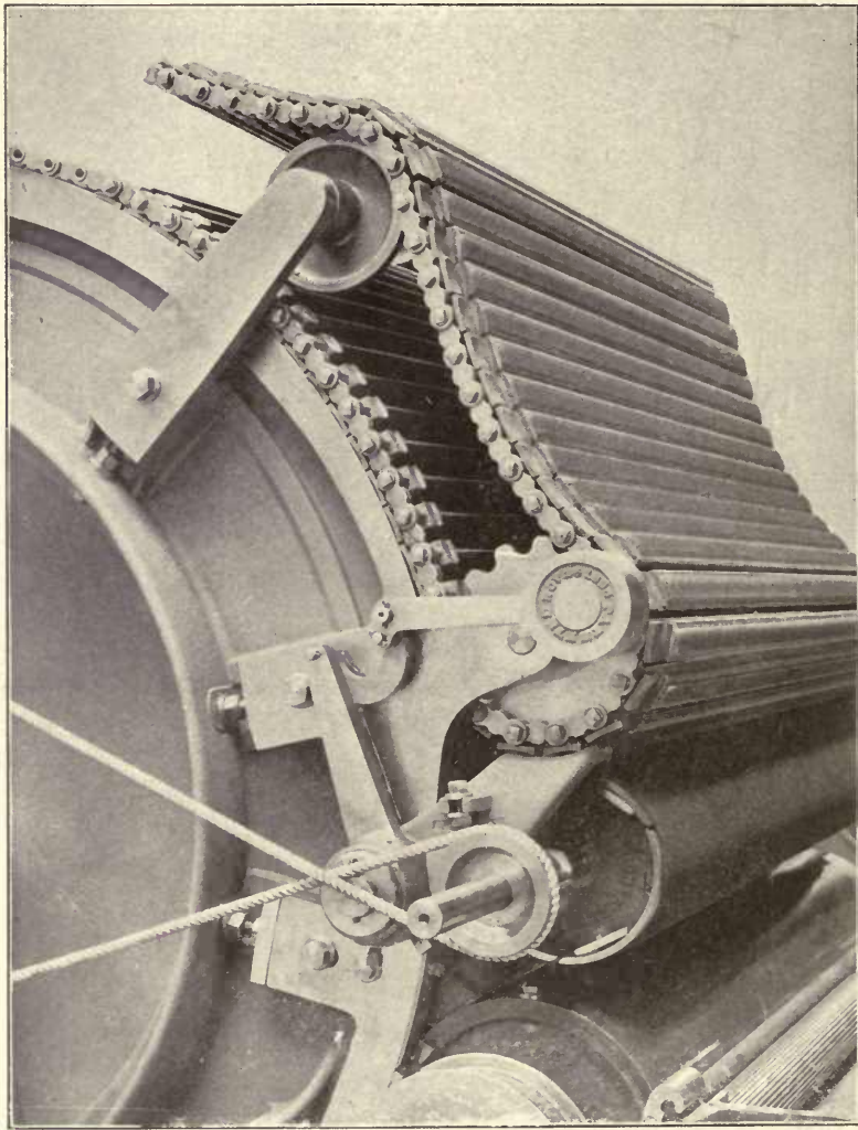
APPARATUS FOR GRINDING FLATS FROM THEIR WORKING SURFACES Mason Machine Works.
