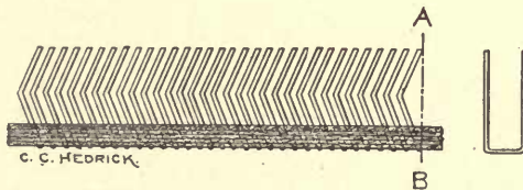
Fig. 75. Clothing for cylinder, doffer and flats.
