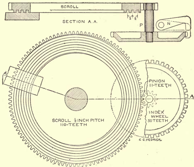
Fig. 71. Section and elevation of scroll.
