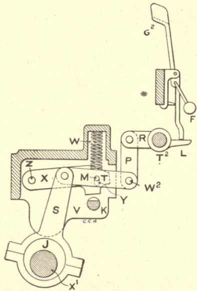
Fig. 178. Back Stop Motion.
