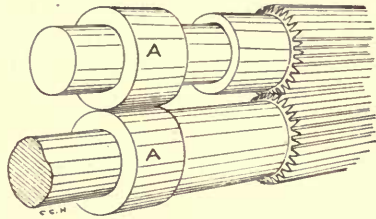
Fig. 156. Perspective View of Metallic Top Rolls.
