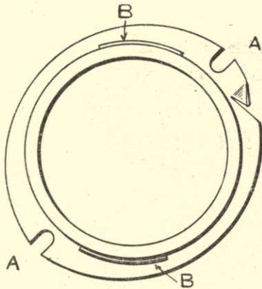
Fig. 205. Oval Plate Holder and Ring.
