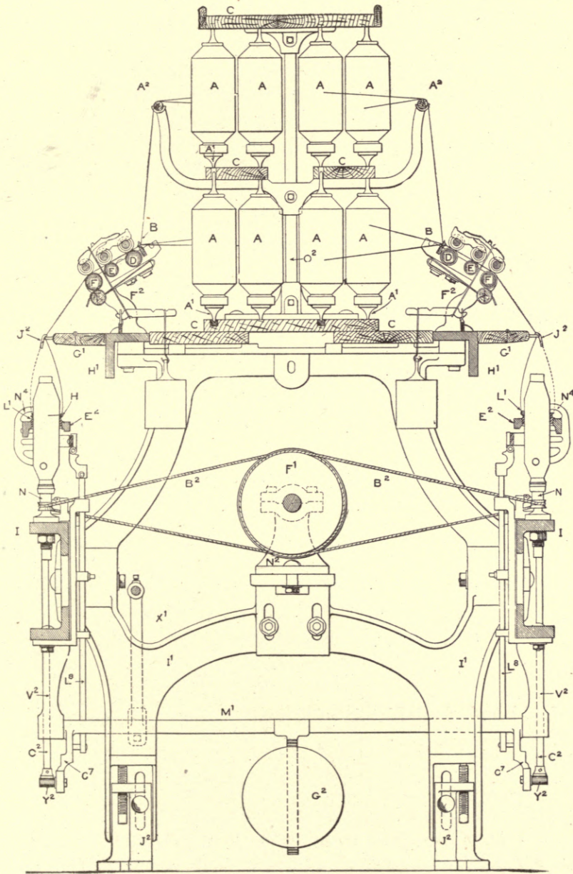
Fig. 192. Sectional Elevation of Ring Frame.
