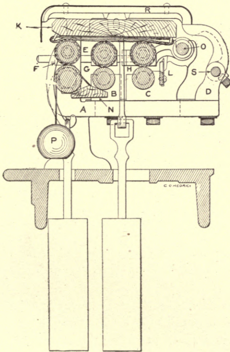
Fig. 179. Roll Stand.
