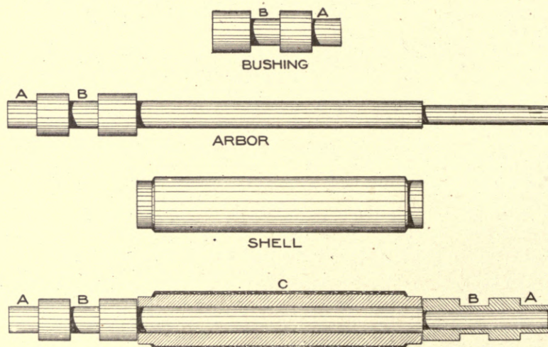
Fig. 155. Shell Top Roll.
