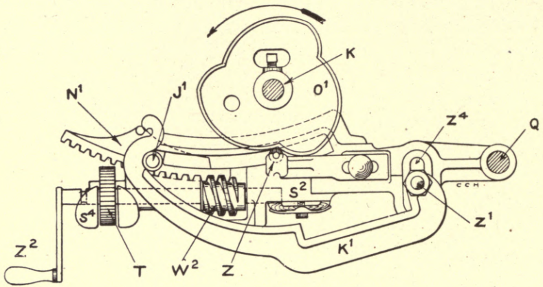
Fig. 215. Combination Builder.
