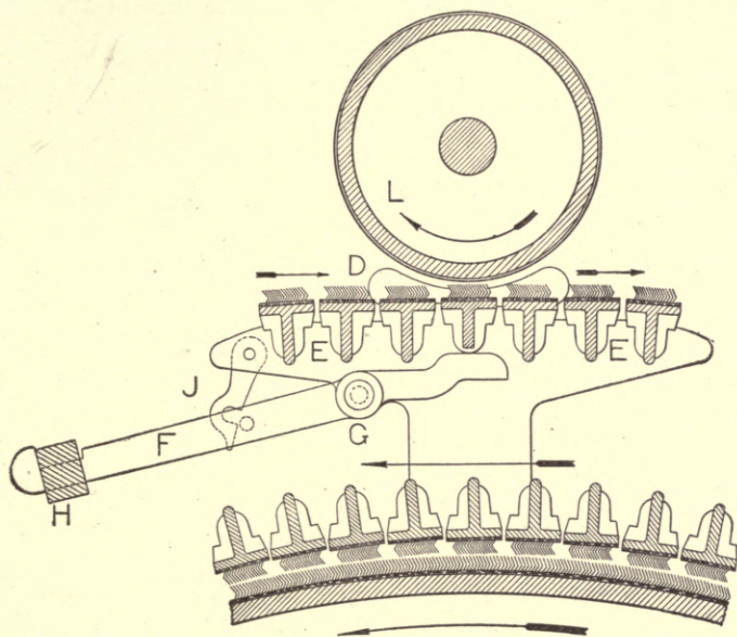
Fig. 95. Section Showing Flat Grinder.
