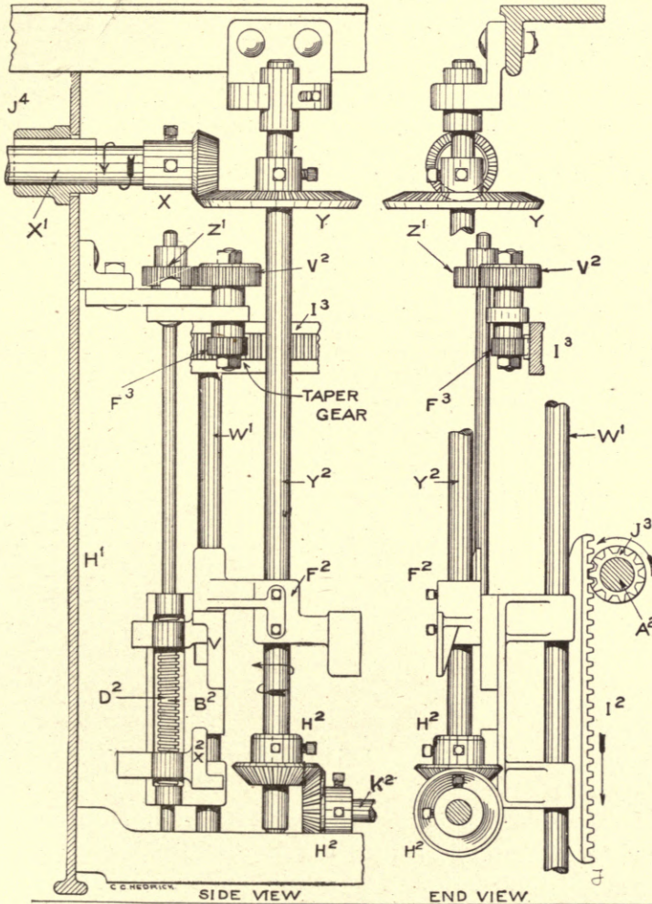
Fig. 170. Builder.
