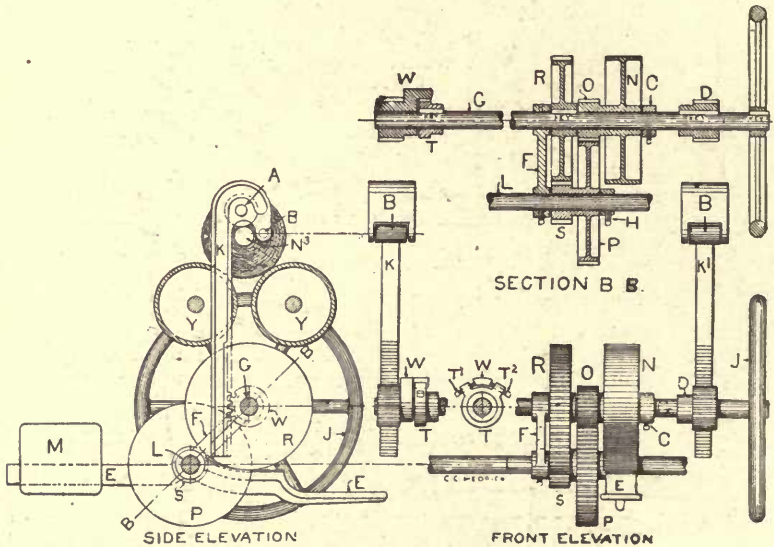
Fig. 43. Friction Let-off.
