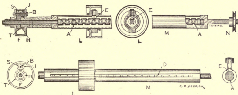
Fig. 89. Traverse Grinder.
