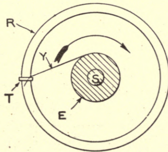
Fig. 208. Diagram Showing Principle of Traveler.
