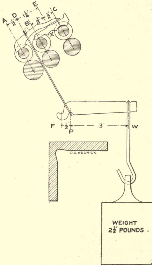
Fig. 195. Diagram of Weighing.
