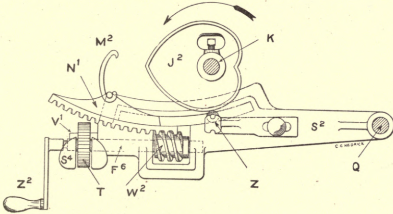
Fig. 210. Warp Builder.
