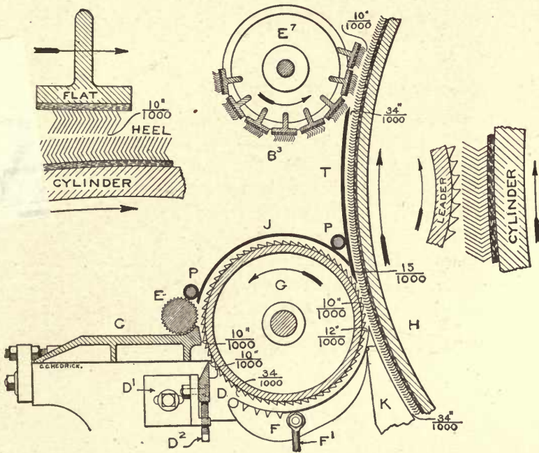
Fig. 57. Section of cylinder, leader and flat.
