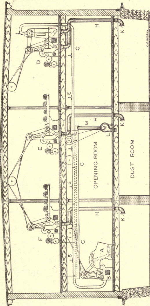
Fig. 8. Sectional Elevation.
