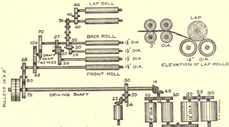
Fig. 111. Diagram of Gearing of Ribbon Lapper.
