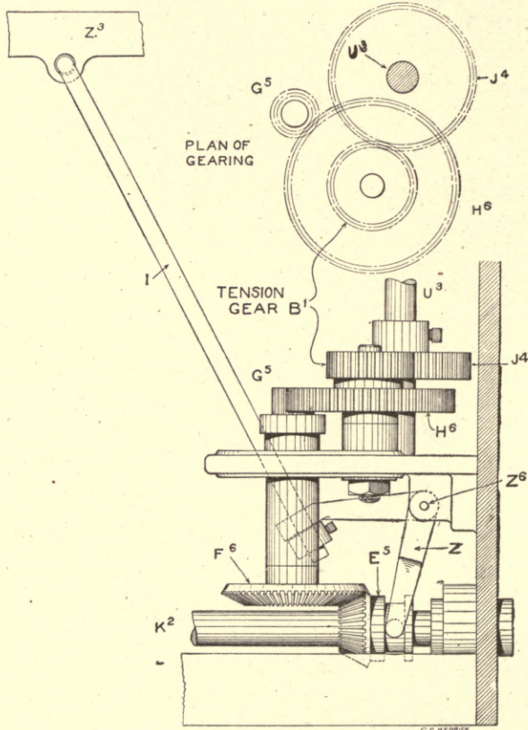
Fig. 173. Tension Gearing.
