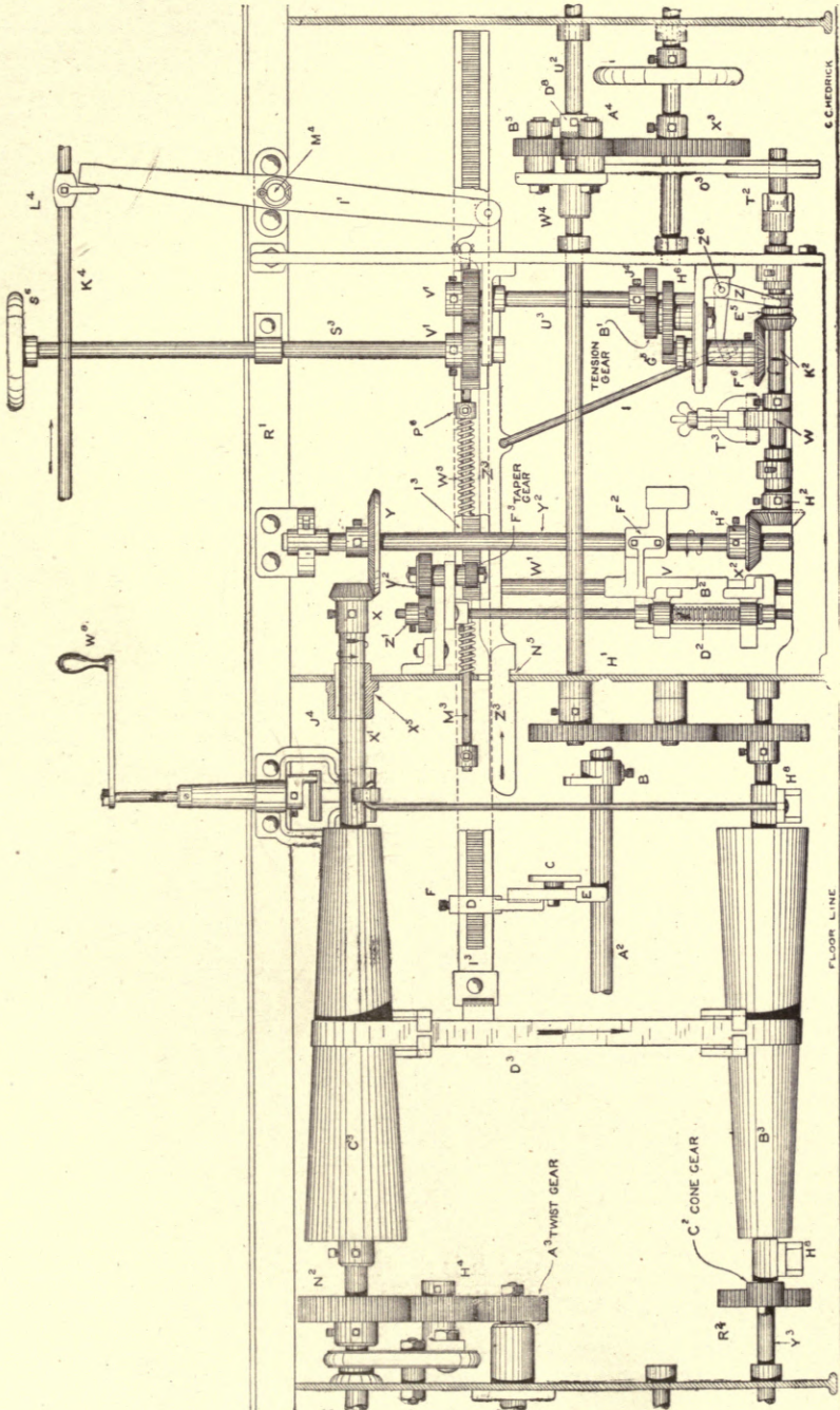
Fig. 168. Reversing Motion and Builder.
