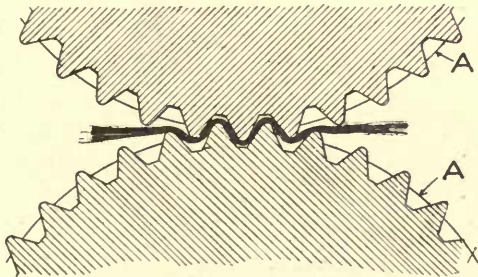
Fig. 157. Enlarged Section of Metallic Top Rolls.
