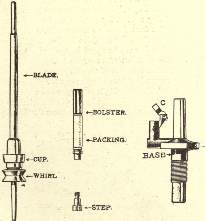
Fig. 201. Spindle Parts.
