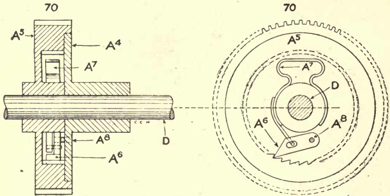
Fig. 240. Roller Motion.
