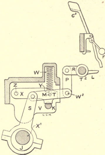
Fig. 177. Back Stop Motion.
