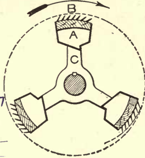
Fig. 10. Carding Beater.
