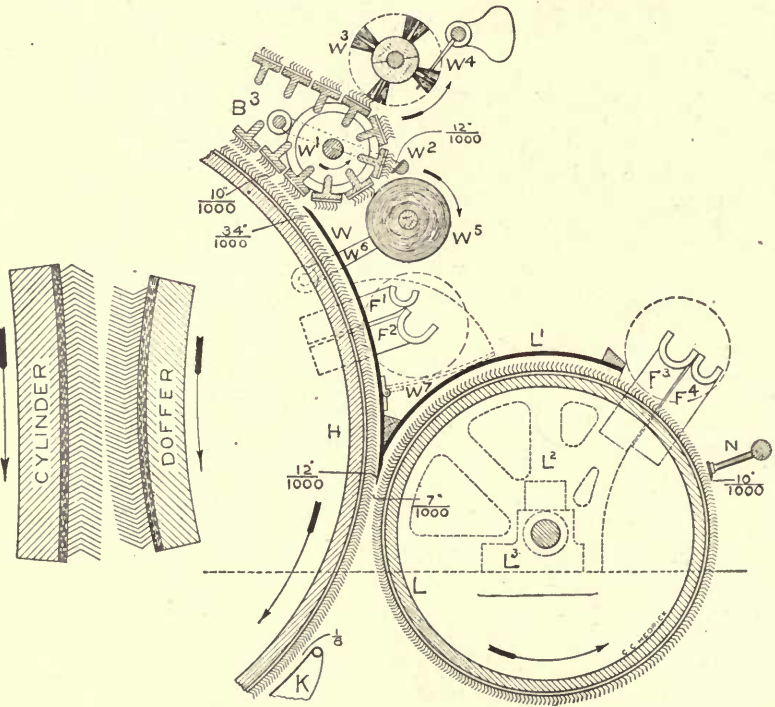
Fig. 58. Section of cylinder and doffer.
