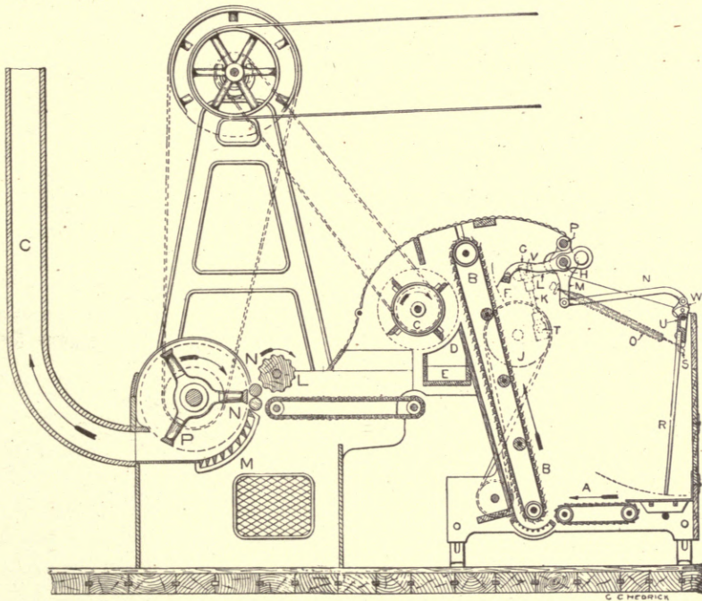
Fig. 28. Automatic Feeder with Evenner Attached.
