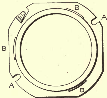
Fig. 206. Square Plate Holder and Ring.
