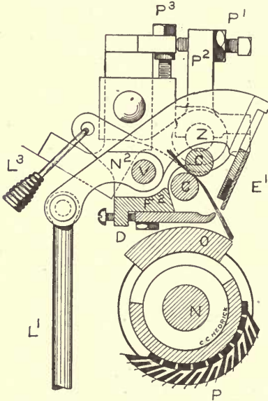
Fig. 117. Section showing Nipper and Cushion Plate.
