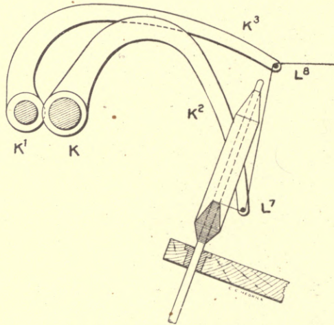
Fig. 229. Elevation Showing Fallers.
