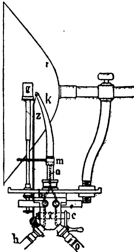
FIG. 3.—BURNER OF WOLTERS AND ROSLIN.
