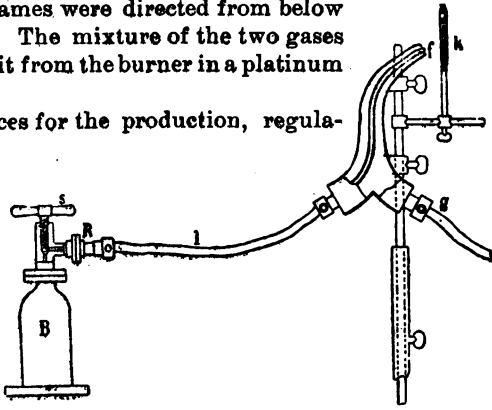
FIG. 2. SCHILTSKY'S BURNER.
