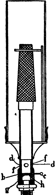
FIG. 45. BURNER OF WEIL AND ROSENTHAL.
