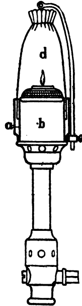
FIG. 65. PINTSCH'S BURNER-HEAD.
