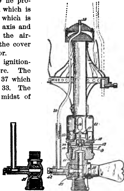
FIG. 44.—BELL'S BURNER.
