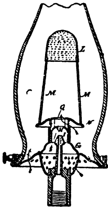
FIG. 19.—REQUA'S BURNER.
