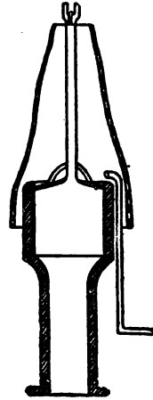
FIG. 48. SCHLESINGER'S IGNITER.
