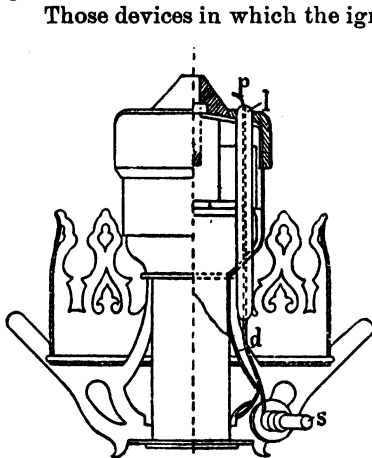
FIG. 49. REIDLINGER'S IGNITER.
