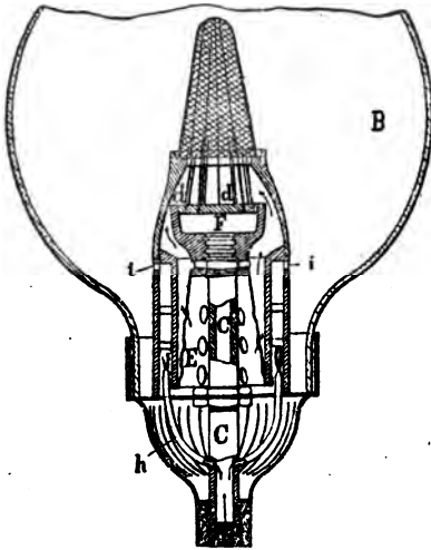
Fig. 4.—CLAMOND'S BURNER.
