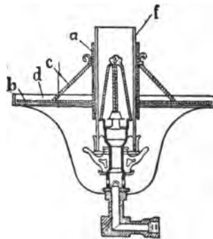
FIG. 63. OHLEN'S GUIDE.
