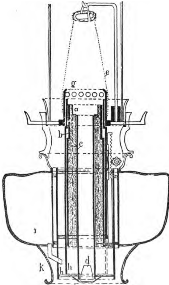
FIG. 34. LINTZMEYER'S BURNER.
