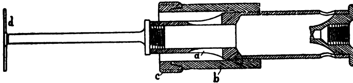
FIG. 25A.—SEEGRUEN'S BURNER.*
