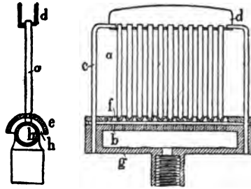
FIG. 25. STEWART'S BUNSEN FLAME.
