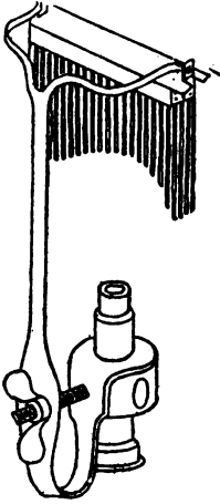
FIG. 8. FAHNEHJELM'S MANTLE.
