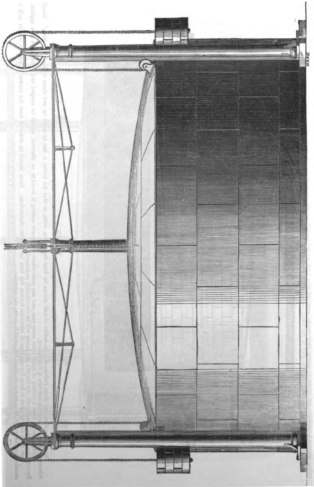
ELEVATION OF GAS-HOLDER COUNTER-BALANCED.
