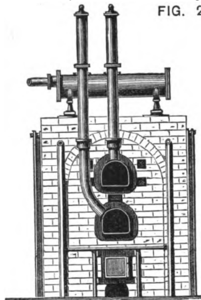
SETTING OF 2 IRON D RETORTS.
