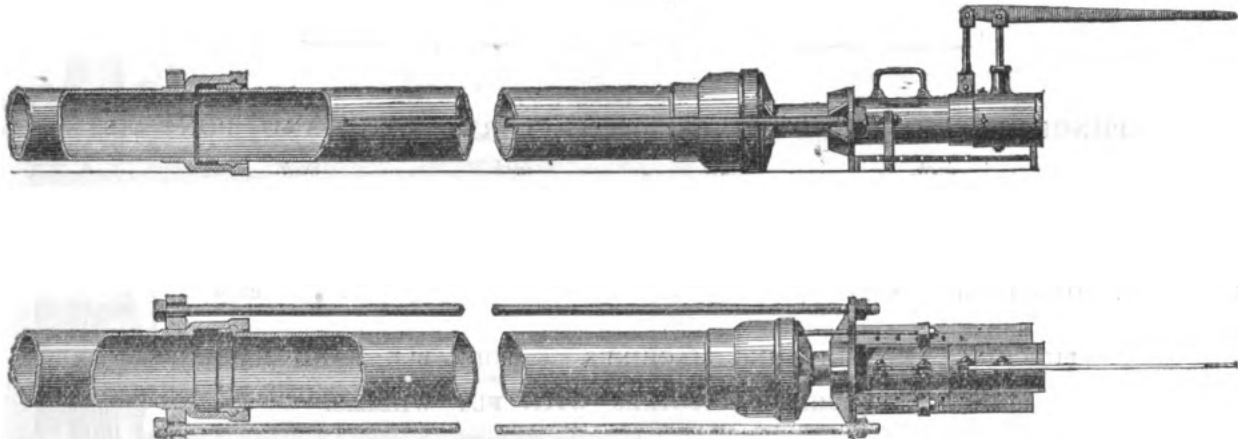
PLAN and ELEVATION OF HYDRAULIC JACK, as used in making joints with Robbin's Patent Pipes. This Jack is also applicable to pipes having turned and bored joints.
