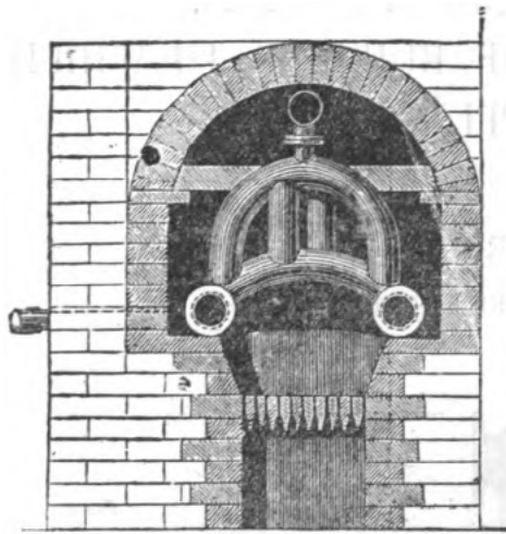
TRANSVERSE SECTION.
