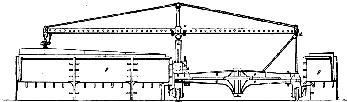
HYDRAULIC LIFTING APPARATUS AND TRAVELLER FOR PURIFIER LIDS.
