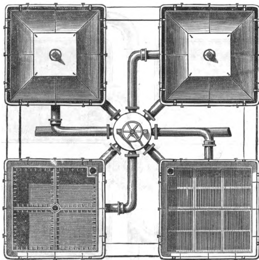
PLAN AND ELEVATION SHEWING TYPE OF SQUARE PURIFIERS MANUFACTURED BY GEORGE BOWER; ALSO, ARRANGEMENT OF INLET AND OUTLET PIPES, AND DRY CENTRE CHANGE VALVE, FOR WORKING ONE, TWO, THREE, OR FOUR PURIFIERS, AS DESIRED.
