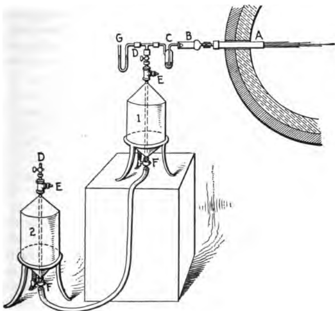
FIG. 2.—Apparatus for aspirating a sample of gas from a flue.
