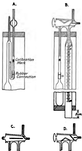
FIG. 19.—Details of gas burette with automatic compensator for temperature and pressure.
