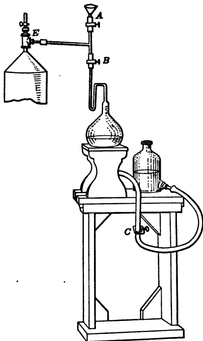
FIG. 4.—Glass gas holder for storing samples.
