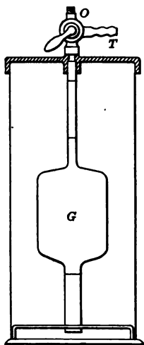
Fig. 42.—Bureau of Standards form of simple specific gravity apparatus.
