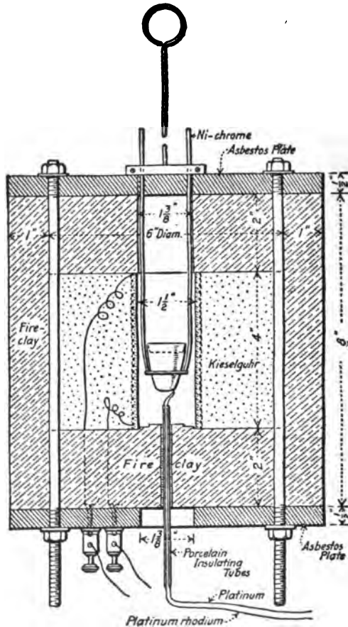
FIG. 54.—Electric tube furnace for determining volatile matter in coal.
