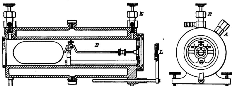
FIG. 43.—Edwards specific gravity balance for gases.
