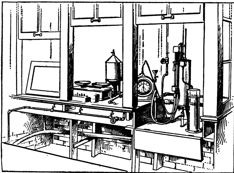
FIG. 23.—Gas calorimeter and accessories.
