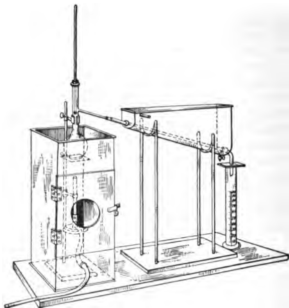
FIG. 46.—Apparatus for distillation of petroleum.
