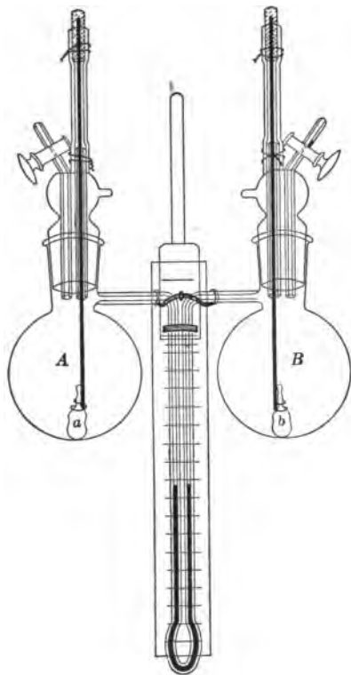
FIG. 37.—Davis differential pressure apparatus for benzene in gas.
