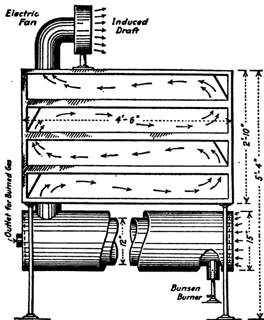
FIG. 50.—Air-drying oven.
