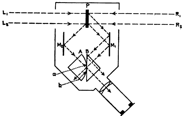
FIG. 31.—Diagram of Lummer-Brodhun photometric screen.
