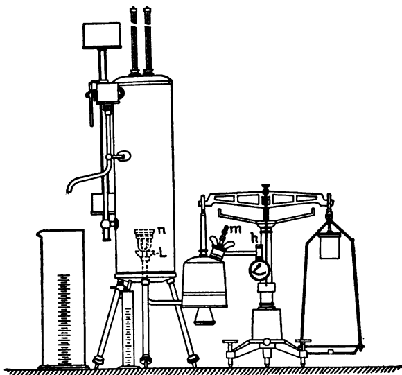
FIG. 44.—Calorimeter for heating value of oils.
