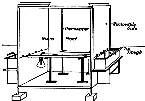
FIG. 40.—Oven for naphthalene determinations.
