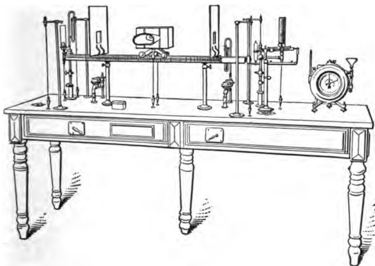
FIG. 34.—Photometer bench.
