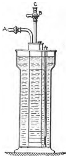
FIG. 41.—Schilling's specific gravity apparatus.
