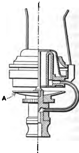
FIG. 30.—Metropolitan No. 2 Argand burner.
