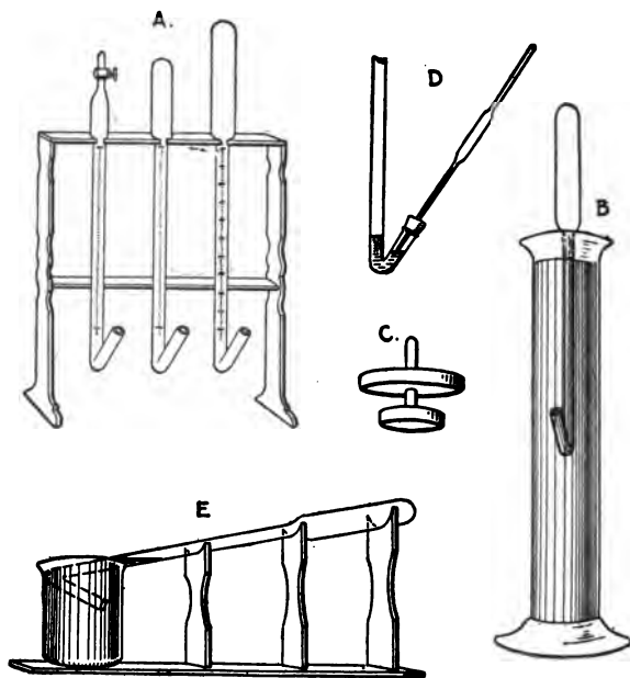
FIG. 18.—Chollar tubes for gas analysis.
