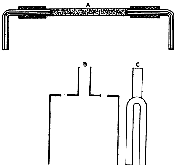
FIG. 13.—Quartz combustion tube filled with copper oxide.
