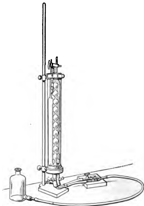
FIG. 21.—Burette for exact gas analysis.
