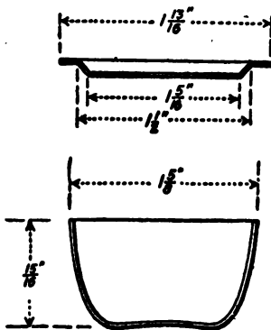
FIG. 53.—Porcelain capsule with flat aluminium cover.
