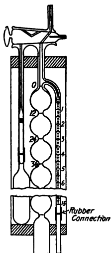
FIG. 20.—Details of bulbed gas burette for exact gas analysis.
