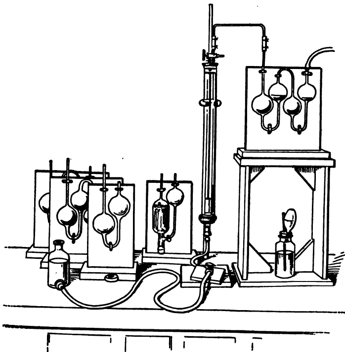
FIG. 9.—Assembled apparatus for gas analysis.
