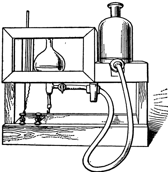
FIG. 11.—Explosion pipette and stand with protecting screen.
