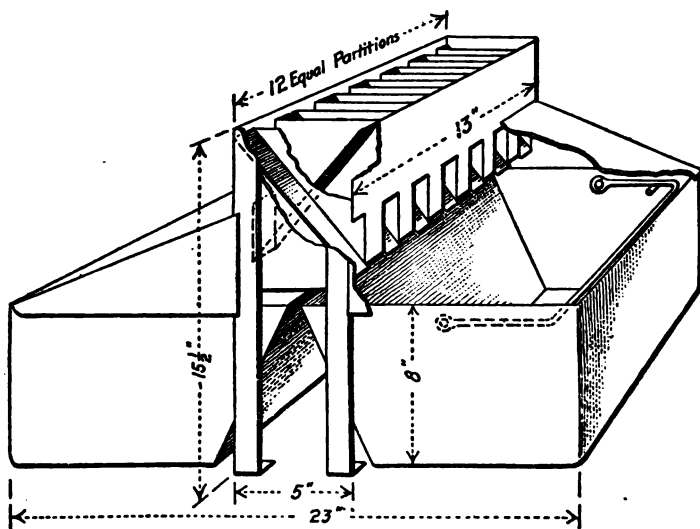
FIG. 51.—Riffle sampler.
