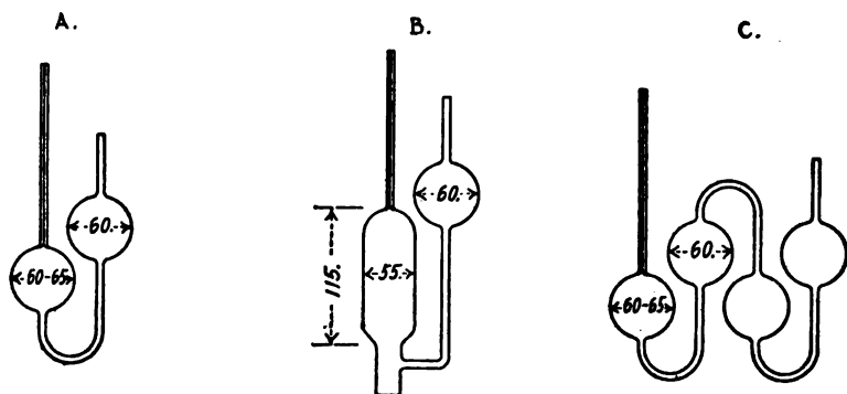
Fig. 8.—Details of gas pipettes.
