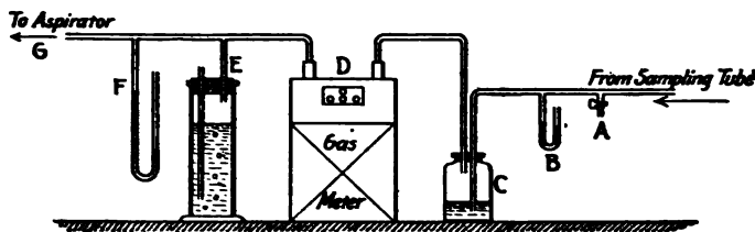
FIG. 3.—Continuous gas sampling apparatus.
