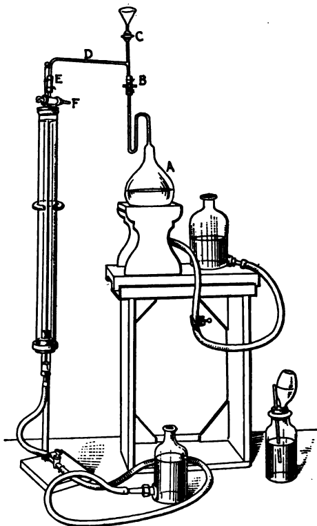
FIG. 7.—Gas burette and gas holder.
