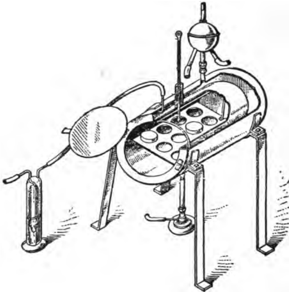
FIG. 52.—Moisture oven for coal, to contain toluene or glycerine and water
