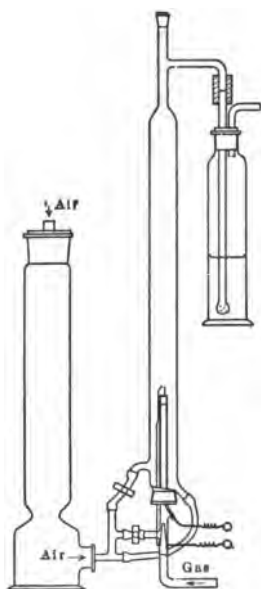
FIG. 38.—Bureau of standards form of sulphur apparatus.
