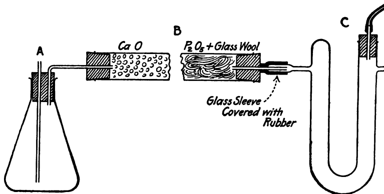
FIG. 39.—Details of naphthalene train.
