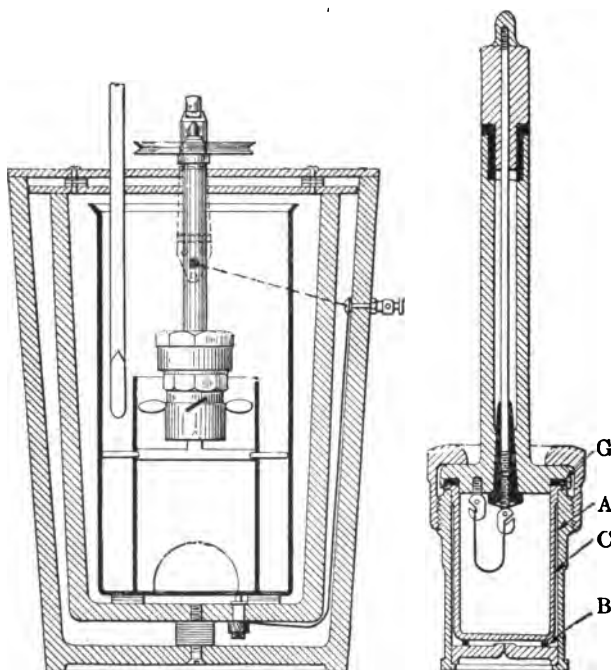
FIG. 58.—Parr calorimeter. FIG. 59.—Details of Parr calorimeter.
