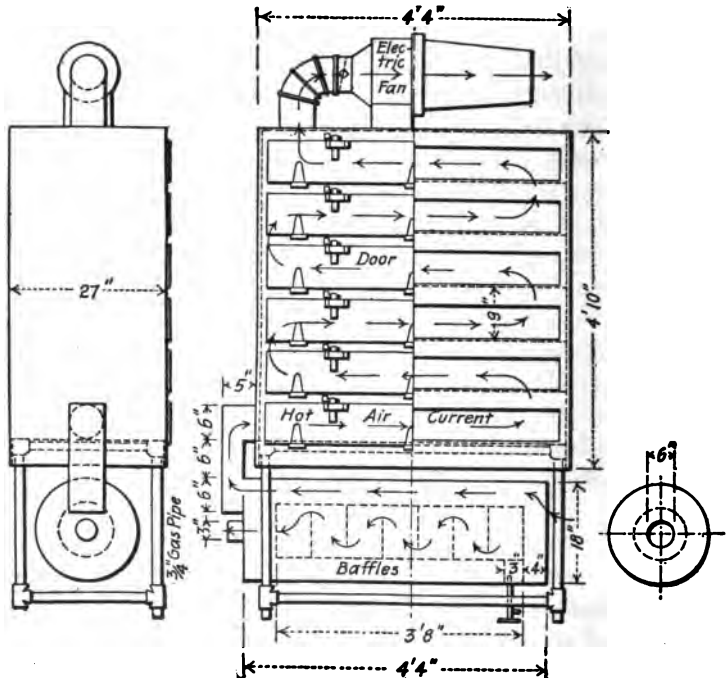
FIG. 48.—Oven for air-drying coal samples
