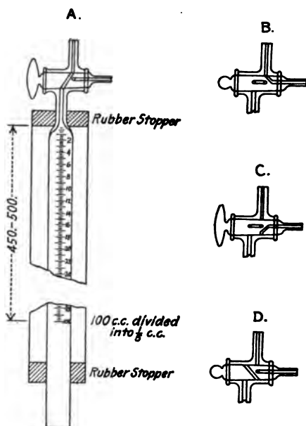
FIG. 6.—Details of gas burette.
