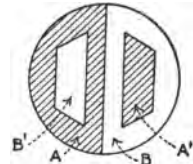
FIG. 33.—Field of Lummer-Brodhun contrast photometric screen.
