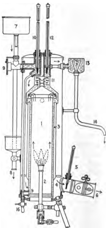
FIG. 22b.—Section of gas calorimeter.
