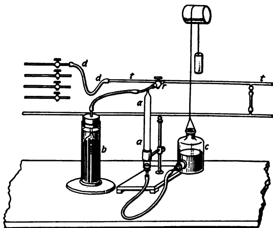
FIG. 14.—Schlösing and Rolland's apparatus.
