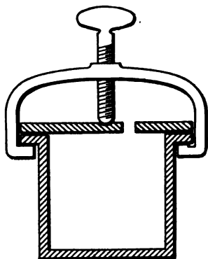
FIG. 49.—Crucible for peroxide fusion.
