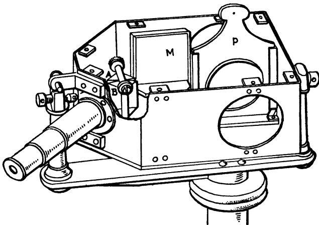
FIG. 32.—Lummer-Brodhun photometric screen.
