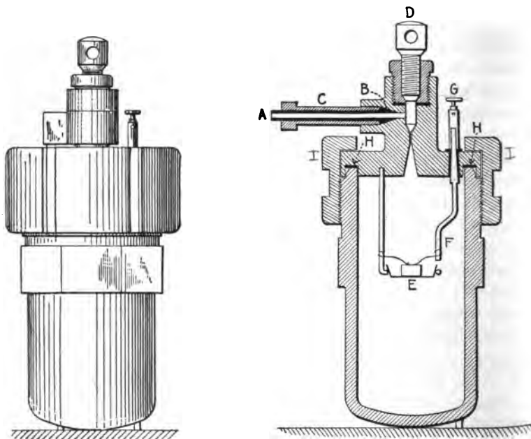
FIG. 55.—Details of calorimetric bomb.
