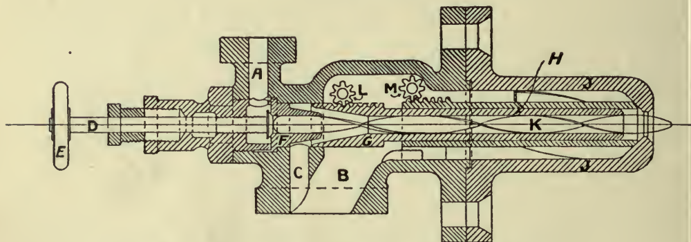
Fig. 69. ATOMIZER. KERMODES HOT AIR SYSTEM.
