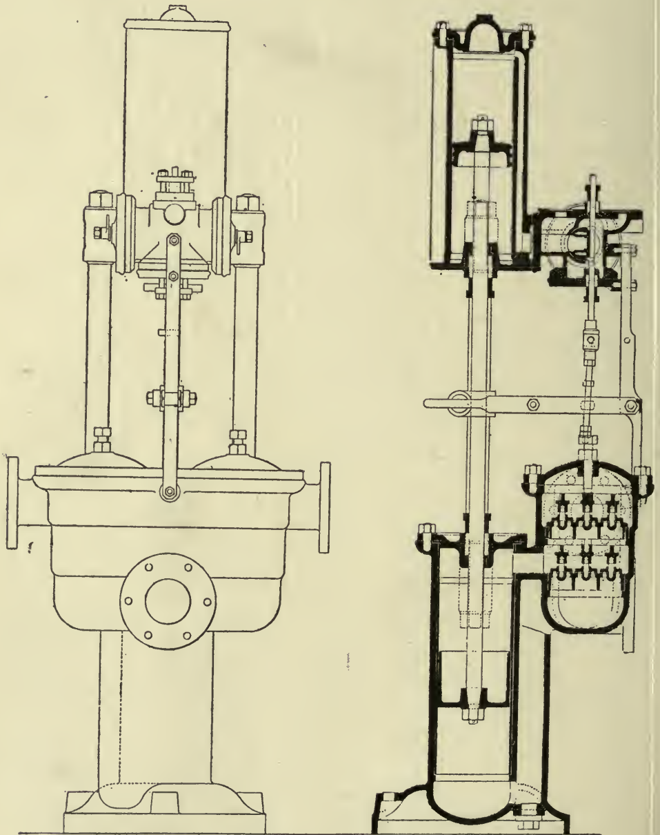
Fig. 62. WEIR'S OIL PUMP.
