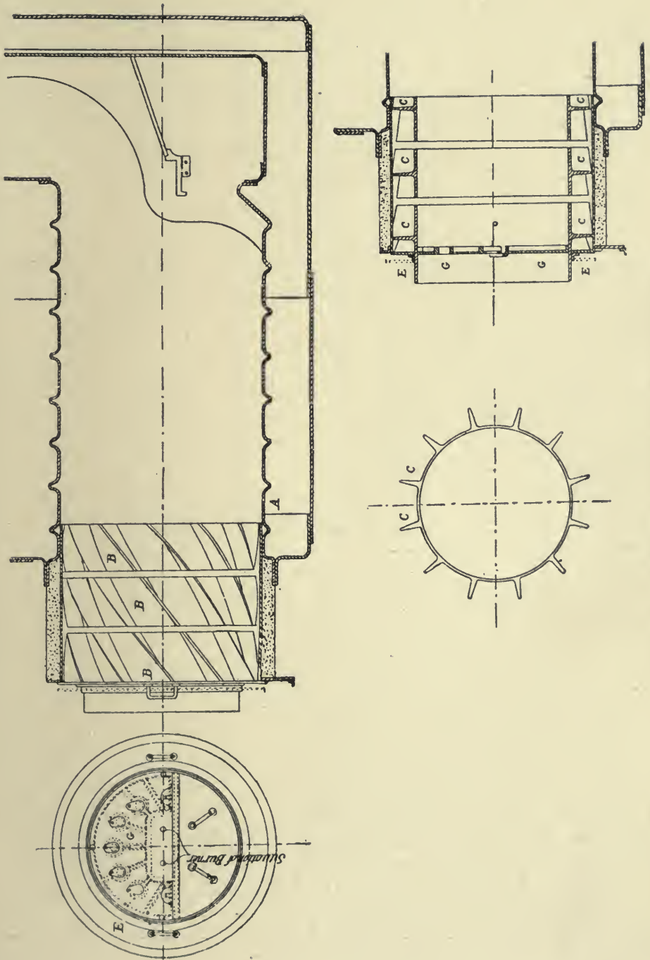
Fig. 33. MARINE FURNACE, MEYER SYSTEM.
