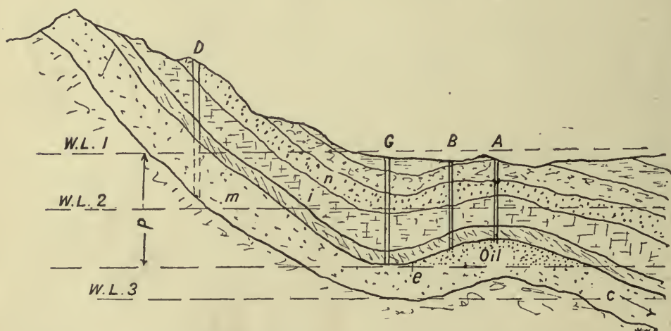
Fig. 0.—HYPOTHETICAL SECTION OF OIL-BEARING STRATIFICATION.
