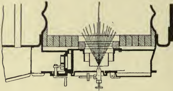
Fig. 17a. HAWDEN'S FORCED DRAUGHT.
