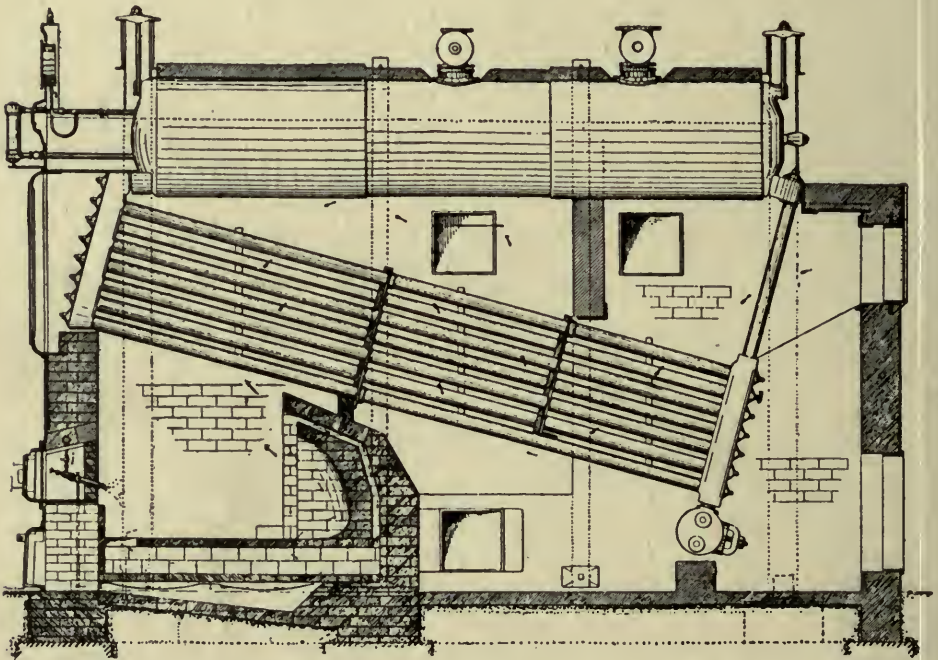
Fig. 51. WATER-TUBE BOILER. BILLOW SYSTEM.
