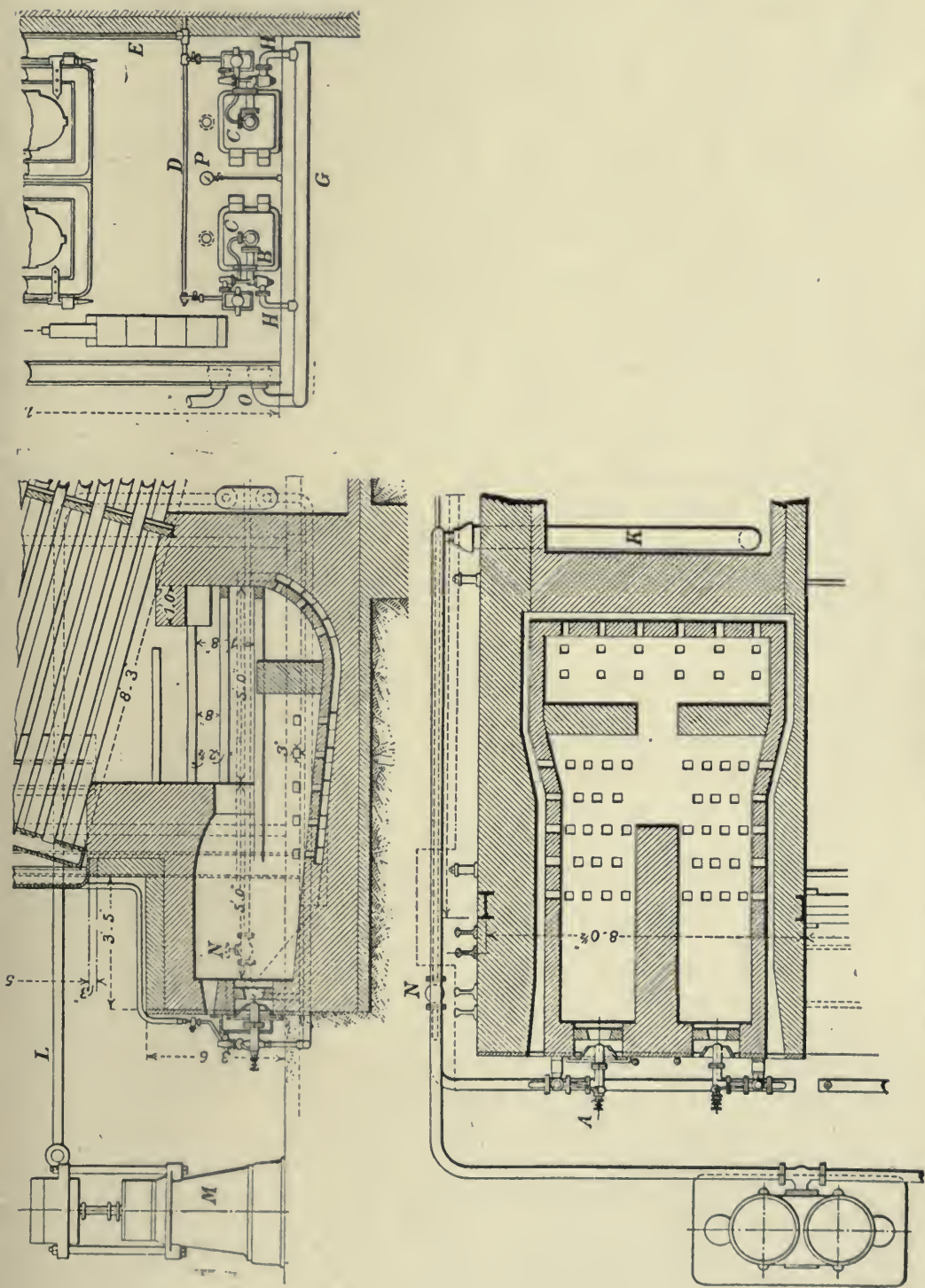
Fig. 54. BABCOCK BOILER WITH KERMODE'S OIL-BURNING SYSTEM.
