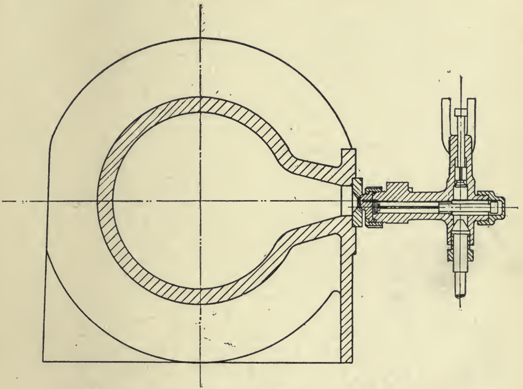
Fig. 84. ENLARGED CROSS SECTION OF VAPORIZER.
