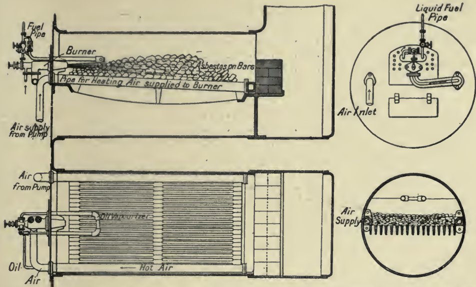
Fig. 53. LIQUID FUEL FURNACE. KERMODE'S SYSTEM. ALTERNATIVE ARRANGEMENT.
