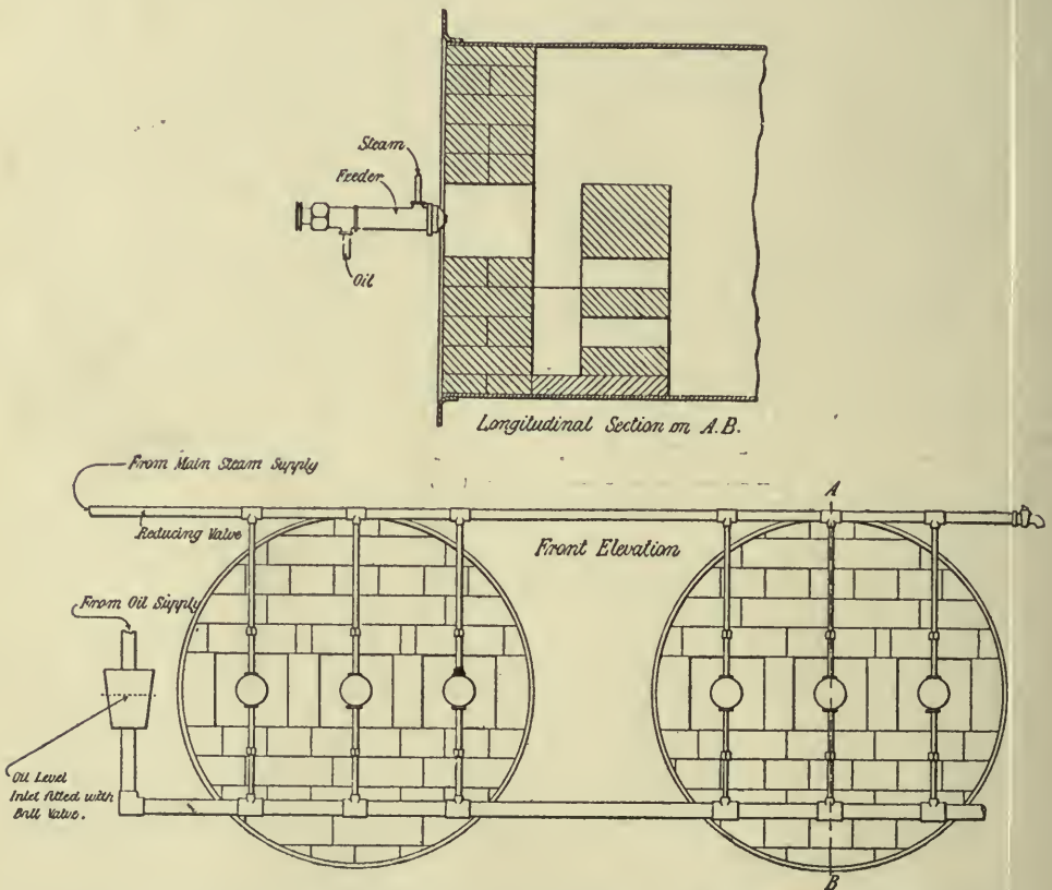
Fig. 56. HYDROLEUM LIQUID FUEL SYSTEM. MARINE BOILER DESIGN.
