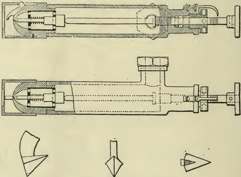
Fig. 73. SWENSSON ATOMIZER.
