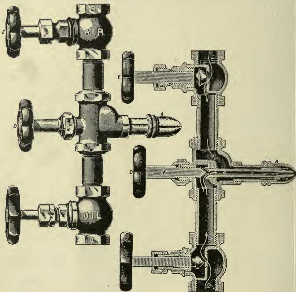
Fig. 67. ATOMIZER. AERATED FUEL SYSTEM.
