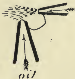
Fig. 81. SOLIANI BURNER.
