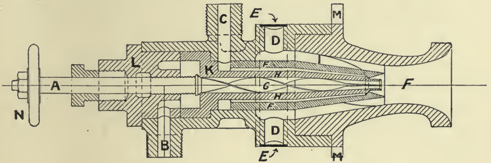
Fig. 70. ATOMIZER. KERMODE'S STEAM SYSTEM.
