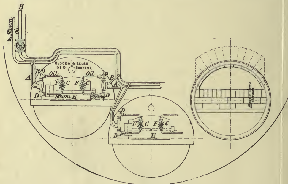
Fig. 9. FURNACE FRONTS OF S.S. "MUREX."
