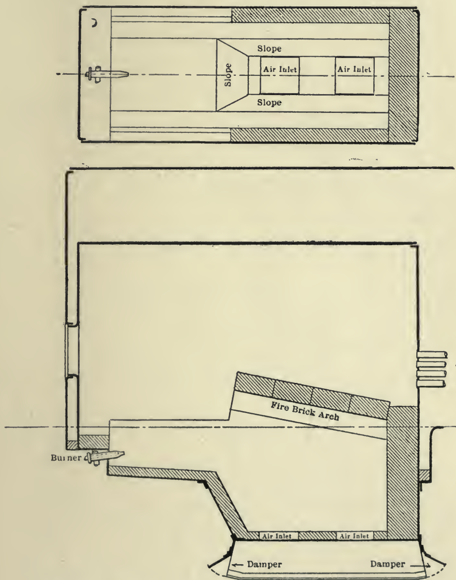
Fig. 27. FIREBOX OF AMERICAN OIL-BURNING LOCOMOTIVE.
