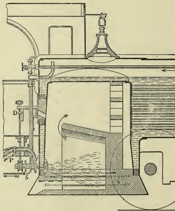
Fig. 38. GOODS LOCOMOTIVE, URQUHART SYSTEM, GRAZI-TSARITZIN RAILWAY.
