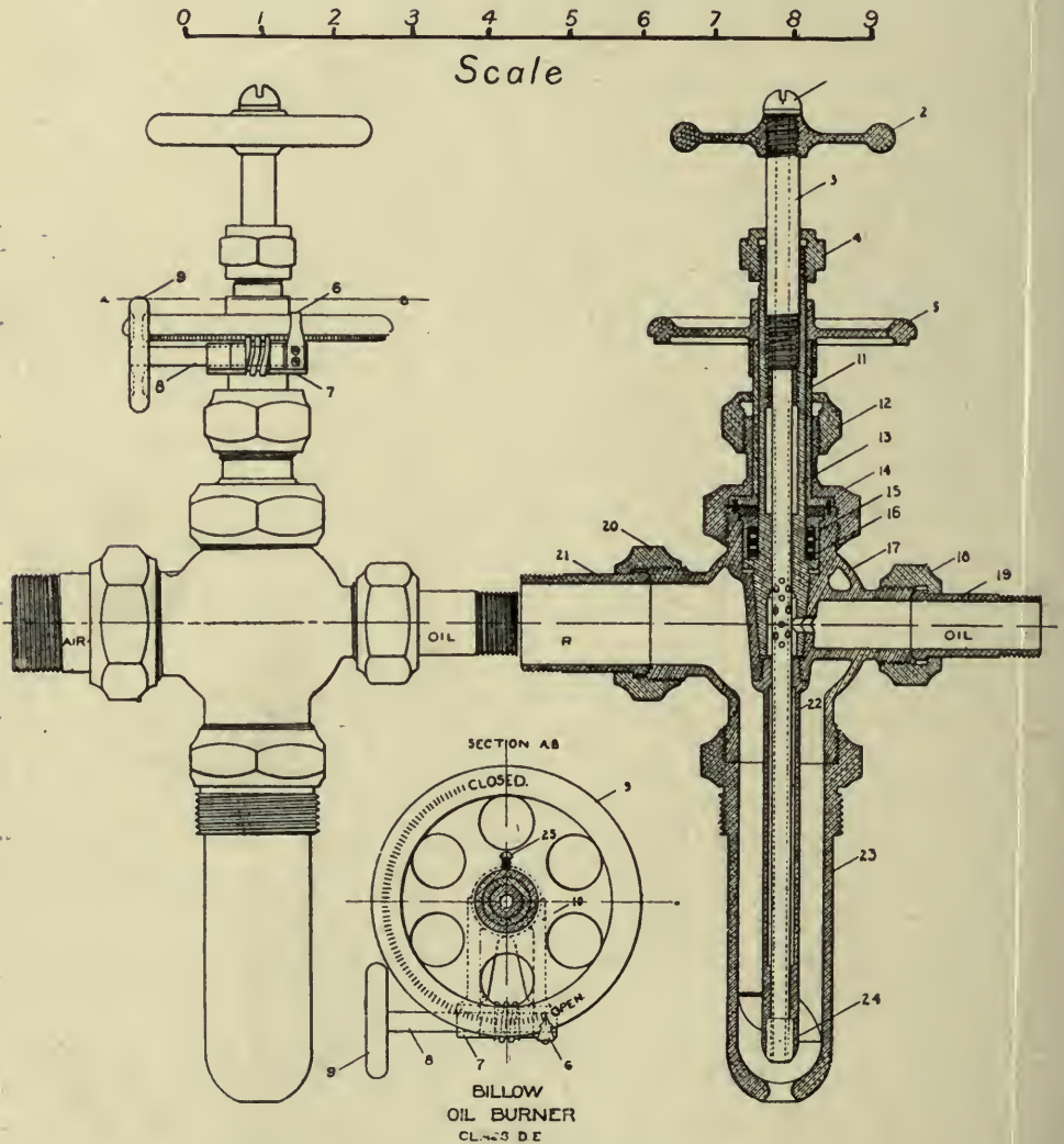
Fig. 44. ATOMIZER. BILLOW SYSTEM.
