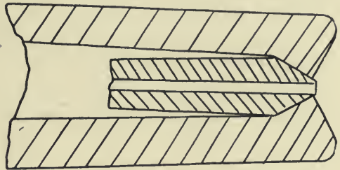
Fig. 76. NOZZLE OF GUYOT ATOMIZER. INCORRECT FORM.
