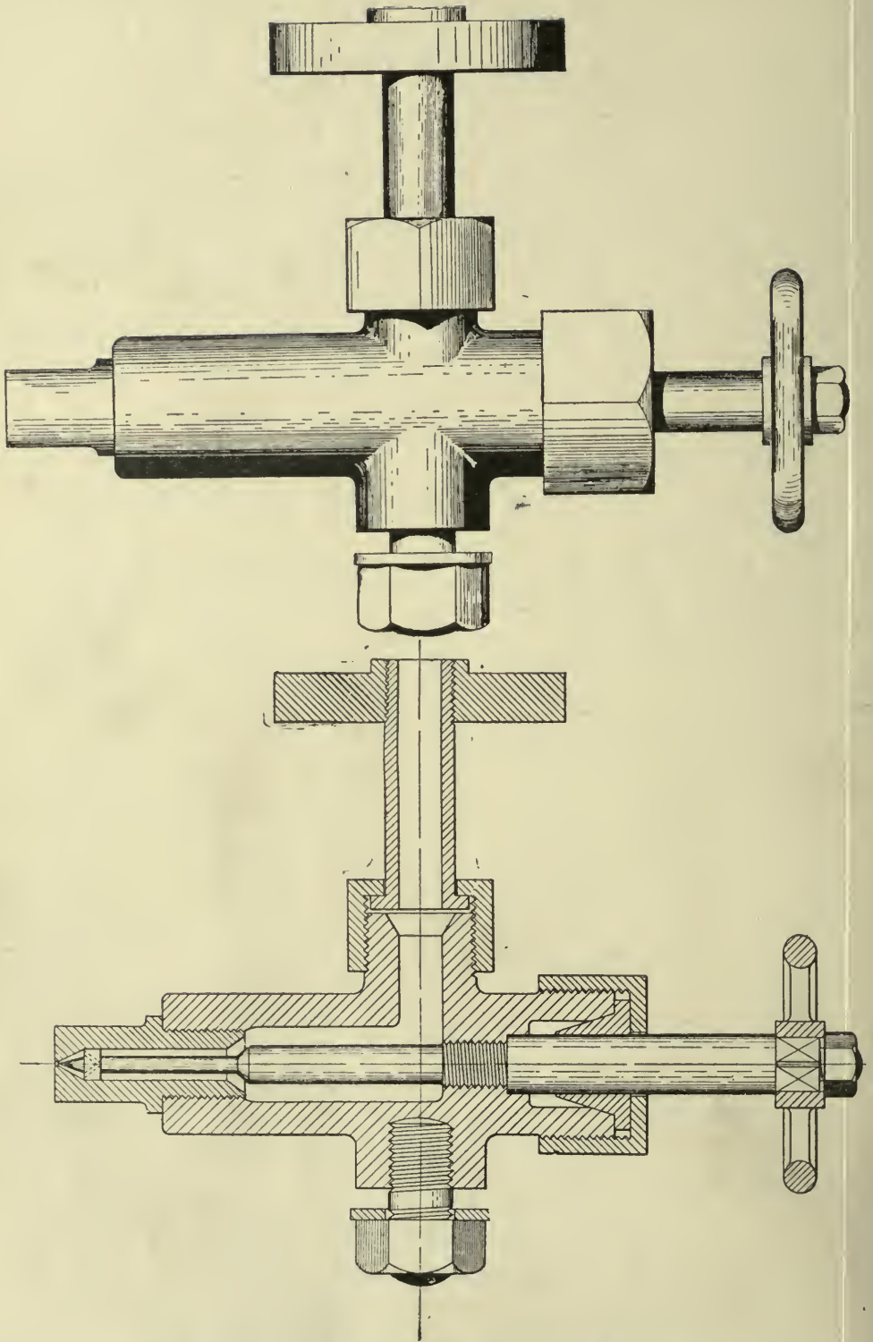
Fig. 18. THE WALLSEND PRESSURE BURNER.
