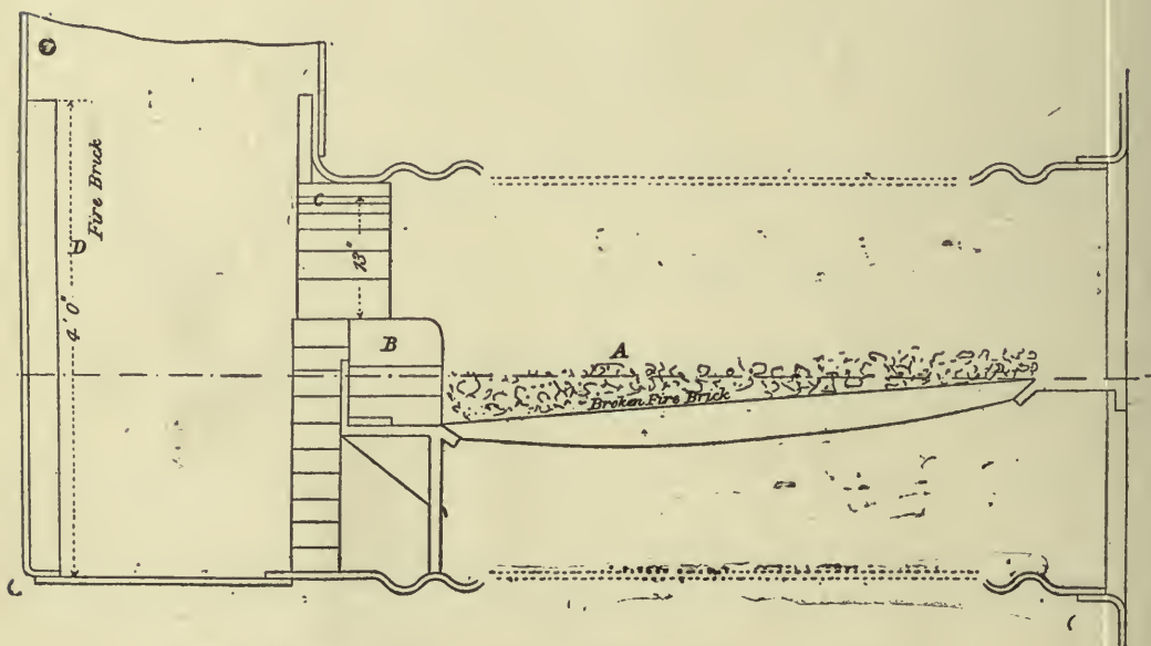
Fig. 11. FURNACE ARRANGEMENT OF S.S. "TROCAS."
