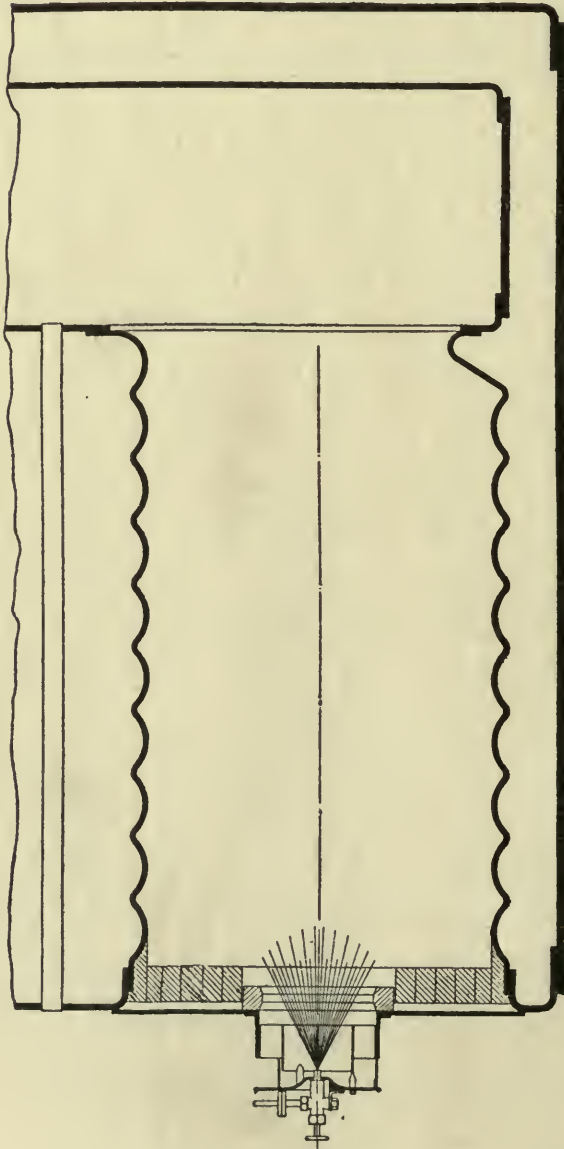
Fig. 17. FURNACES WITH WALLSEND OIL BURNING APPARATUS NATURAL DRAUGHT.
