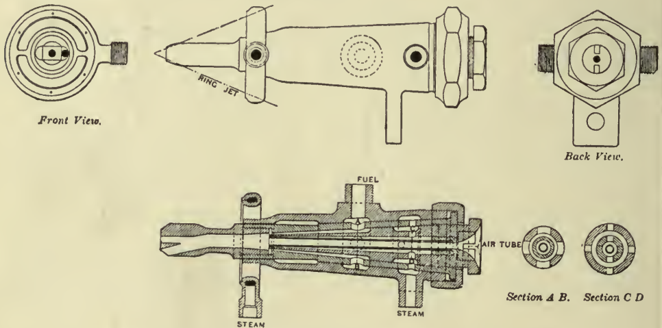
Fig. 25. ATOMIZER. OLD FORM, HOLDEN SYSTEM.
