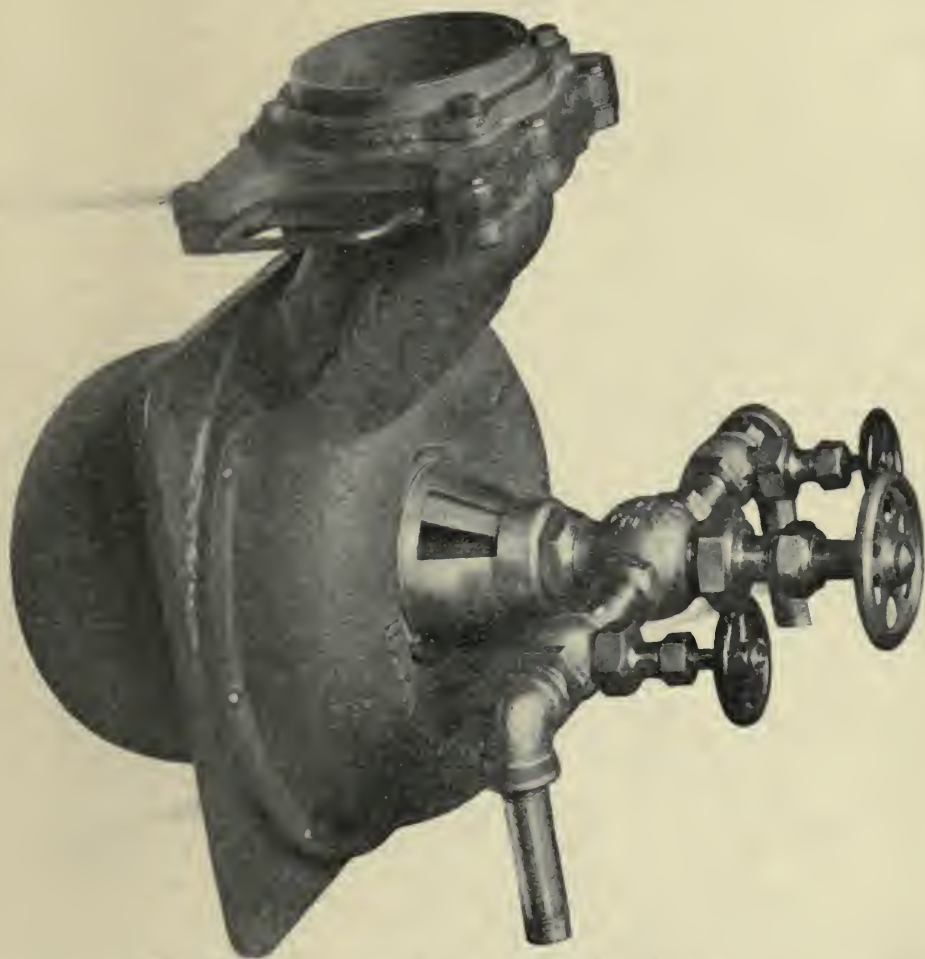
Fig. 46. COMPOUND TUYERE FOR AIR ADMISSION.
