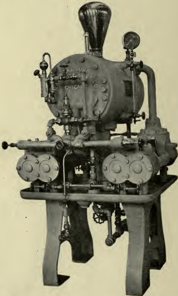
Fig. 45. DOUBLE PUMPING SYSTEM. CAPACITY, 1_ to 5,000 BOILER H.P.
