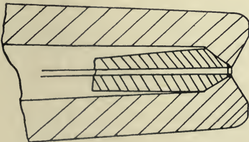
Fig. 77. NOZZLE OF GUYOT ATOMIZER. CORRECT FORM.
