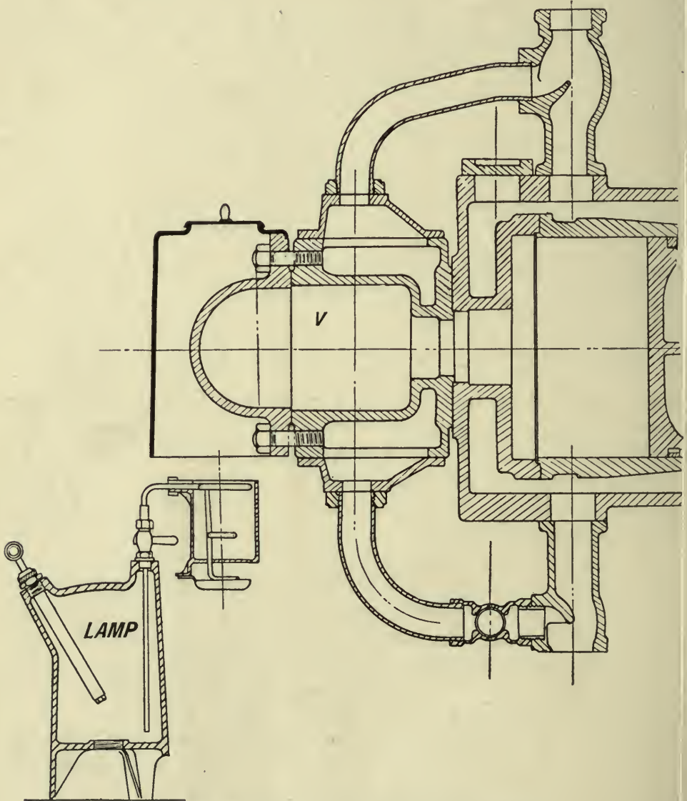
Fig. 83. HORNSBY OIL ENGINE VAPORIZER.
