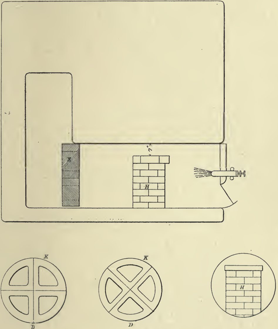
Fig. 10. ARRANGEMENT OF FURNACE BRICKWORK, S.S. "MUREX."
