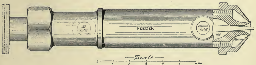
Fig. 71. ATOMIZER. HYDROLEUM SYSTEM.
