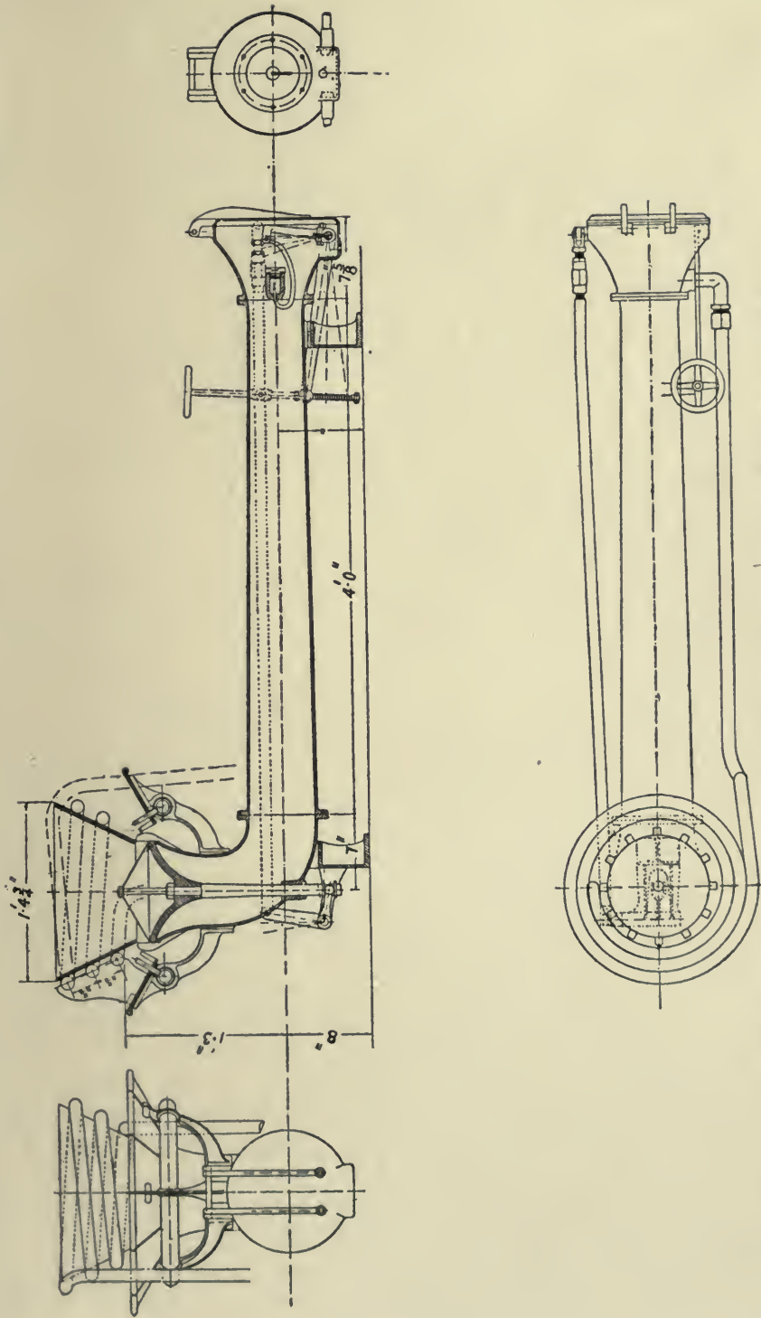
Fig. 57. CLARKSON-CAPEL VAPORIZING BURNER, 200 H.P. FOR FIRE FLOAT.
