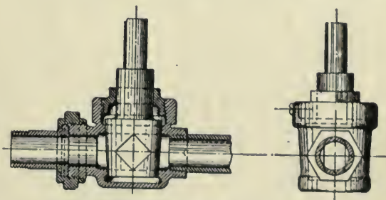
Fig. 35. OIL REGULATING COCK. BALDWIN LOCOMOTIVE CO.
