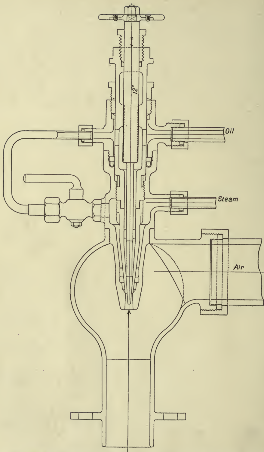
Fig. 15. ORDE AND SODEAU'S ATOMIZER, ARMSTRONG WHITWORTH & CO.
