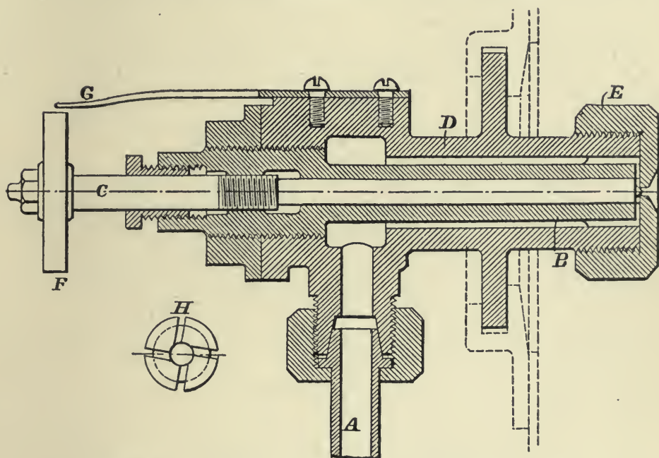
Fig. 68. ATOMIZER. KERMODE'S PRESSURE SYSTEM.
