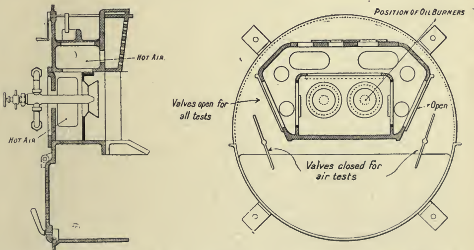
Fig. 60. ELLIS AND EAVES SYSTEM, FURNACE DOOR ARRANGEMENT.
