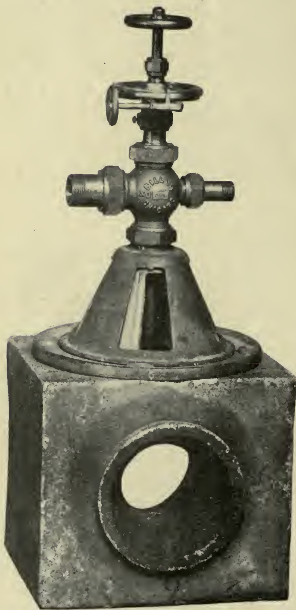
Fig. 47. AIR REGULATOR, ATOMIZER AND TUYERE BLOCK FOR FURNACE FRONT.
