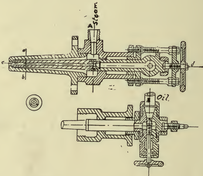
Fig. 75. GUYOT ATOMIZER.
