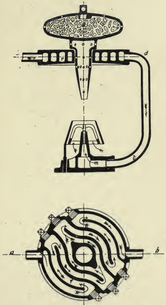
Fig. 74. SYMON-HOUSE BURNER AND VAPORIZER.
