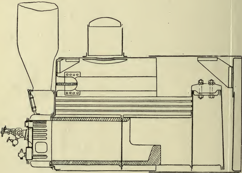
Fig. 78. BOILER OF FRENCH TORPEDO-BOAT No. 22.
