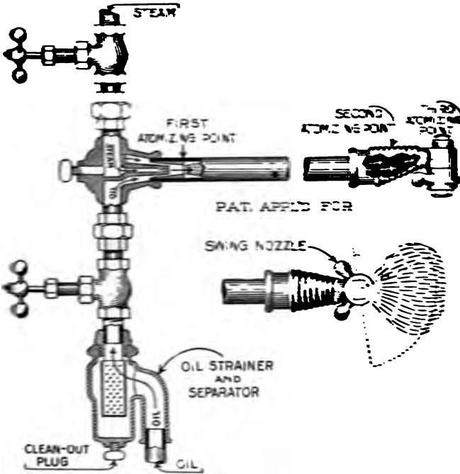
Fig. 26. Schur's Oil Burner.
