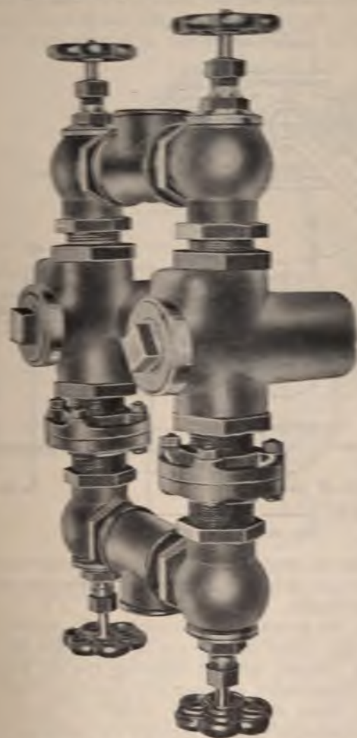
FIG. 39. Method of Connecting Bucket Heaters.
