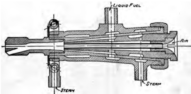
Fig. 31. Holden Oil Burner.
