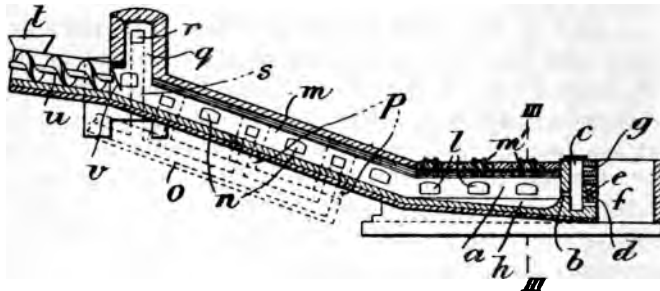
Fig. 69. Buchholtz Furnace.
