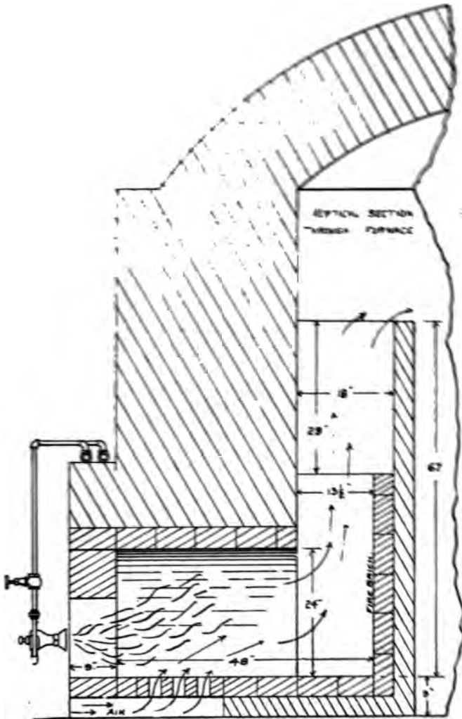
Fig. 49. Down-Draft Kiln.
