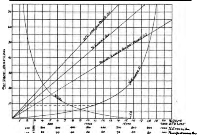
Fig. 106. \text{CO}_2 Curve Showing Heat Loss Due to Excess Air.
