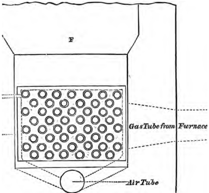
Fig. 26.—Gas furnace at Treveray.
