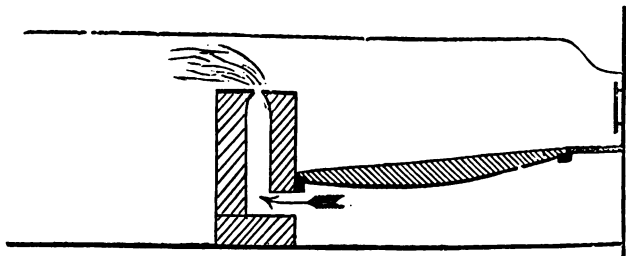
Fig. 33.—Parkes' Split Bridge.
