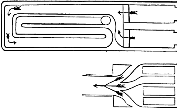
Fig. 27.—Equalising the supplies of gas and air.
