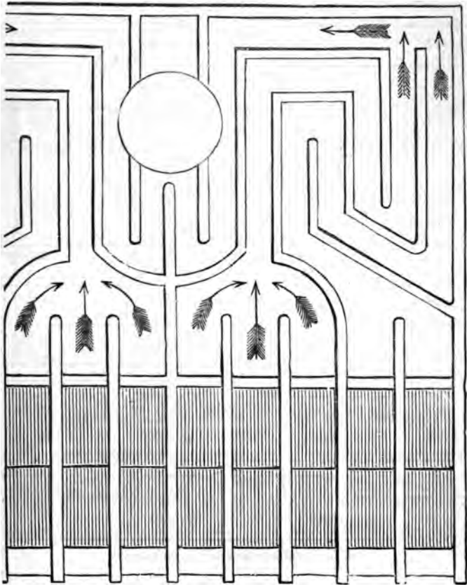
Fig. 98.—Boiler of the " Great Liverpool ."
