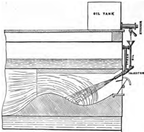
Fig. 118.—Liquid Fuel for Steam Boiler.
