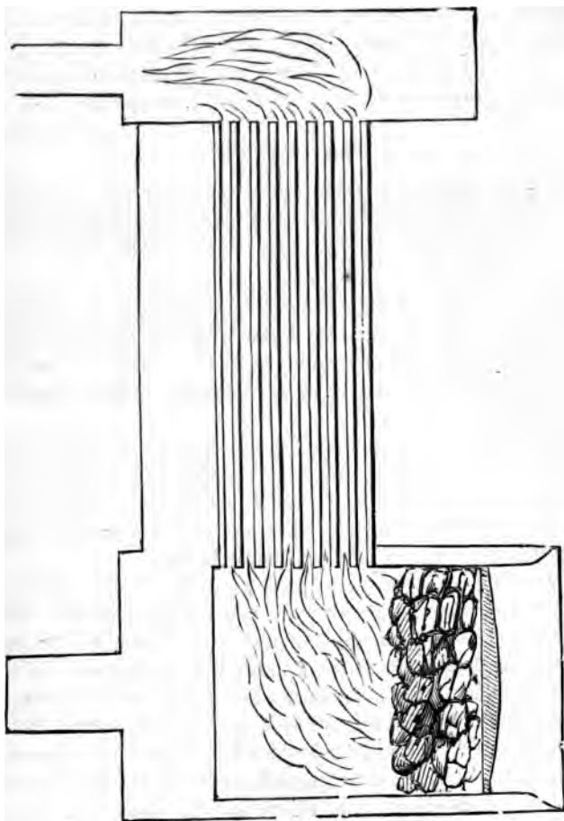
Fig. 99.—Locomotive Boiler.
