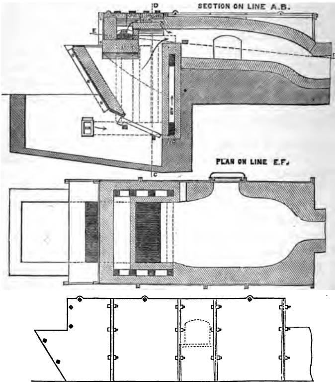
Figs. 125.—The Boetius Heating Furnace.
