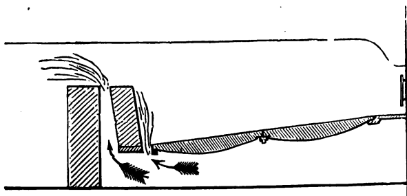
Fig. 85.—Split Bridge and Air at the Grate.
