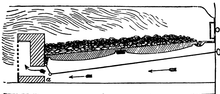
Fig. 63.—Proper Firing.
