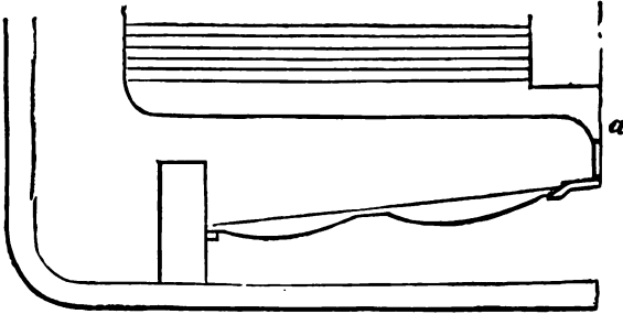
Fig. 60.—Common Furnace.
