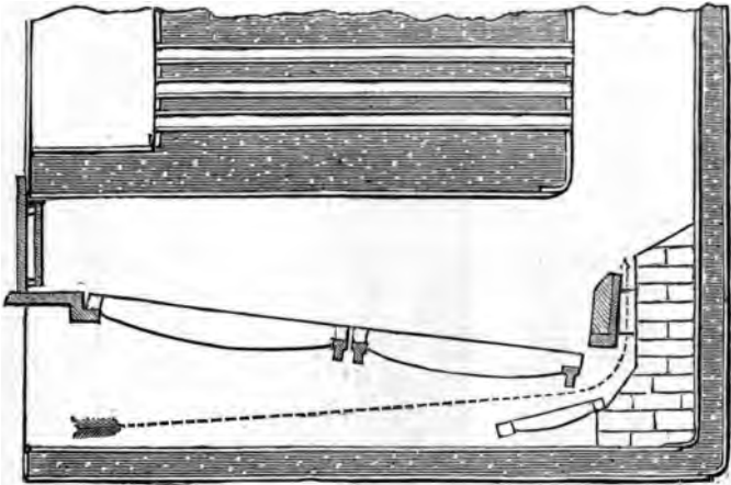
Fig. 56.—Hot Air at the Bridge.
