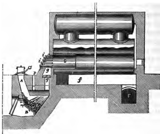
Fig. 123.—Gas-furnace for an Internally Fired Boiler.
