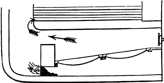
Fig. 43.—Air-box at Bridge.
