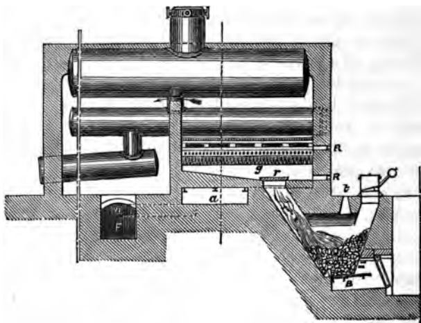
Fig. 122.—Gas-furnace for Steam Boiler.
