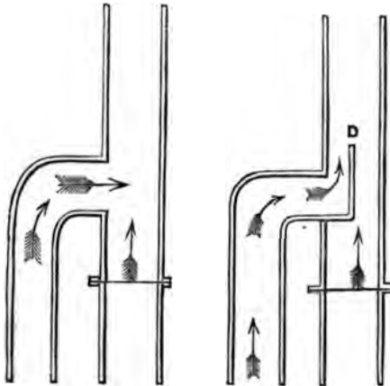
Figs. 87 and 88.—Draught in Flues.
