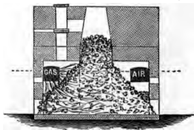
Fig. 136.—The Ponsard Gas-Furnace.—Superheated Gazogene.
