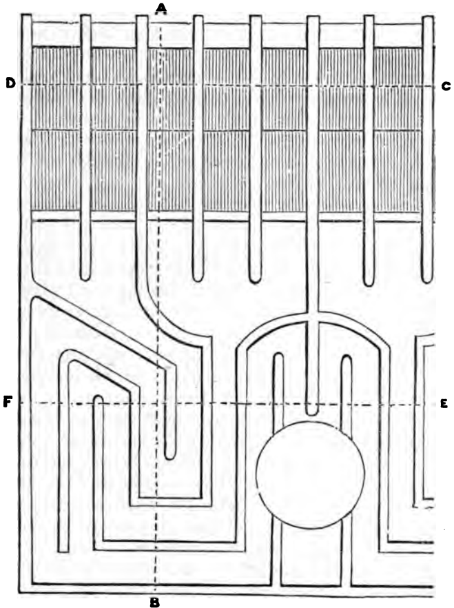
Fig. 81.—Boiler of the "Liverpool."
