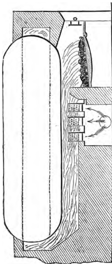
Fig. 10.-Air and Fuel Inlet.
