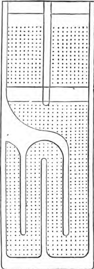
Fig. 113.—Boiler of the "Royal William."
