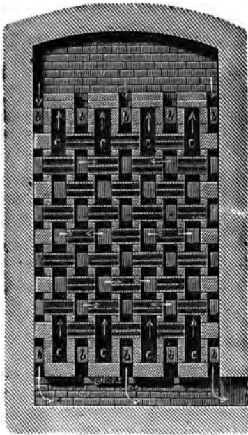
Fig. 138.—The Ponsard Gas-furnace.—Transverse Section of Recuperator.
