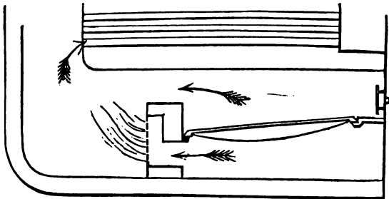
Fig. 44.—Argand Furnace.
