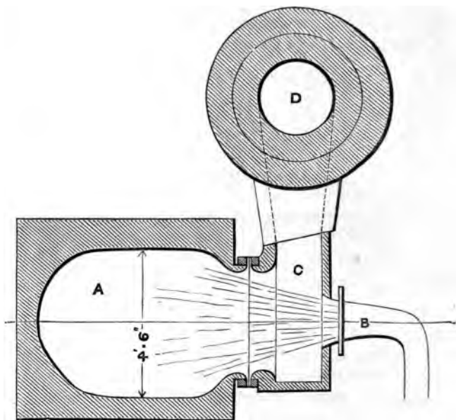
Fig. 142.—Crampton's Powdered Fuel Revolving Puddling Furnace—Single Chamber.
