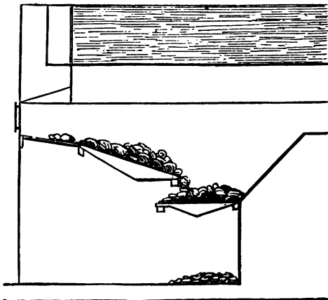
Fig. 55.—Chanter's System.
