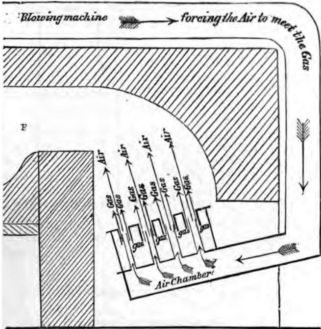
Fig. 25.—Gas furnace at Treveray.
