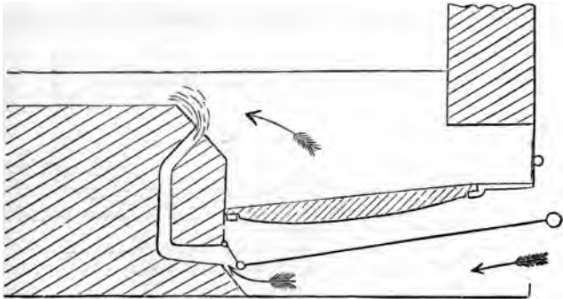
Fig. 54.—Hot Air at the Bridge.
