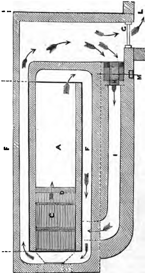
Fig. 58.—Blast of Smoke and Air.
