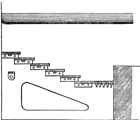
Fig. 117.—Step-Grate.
