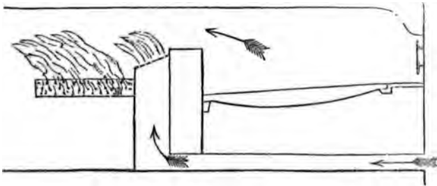
Fig. 42.—Argand Furnace.
