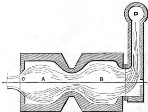
Fig. 141.—Crampton's Powdered Fuel Revolving Puddling Furnace.
