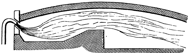
Fig. 140.—Crampton's Powdered Fuel Furnace.
