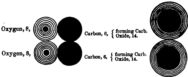
Fig. 9.—Carbonic Oxide.
