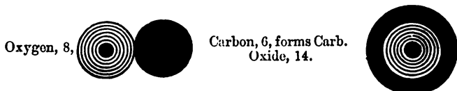
Fig. 7.—Carbonic Oxide.
