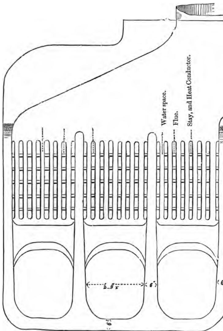
Fig. 114.—Lamb and Summers' Boiler.
