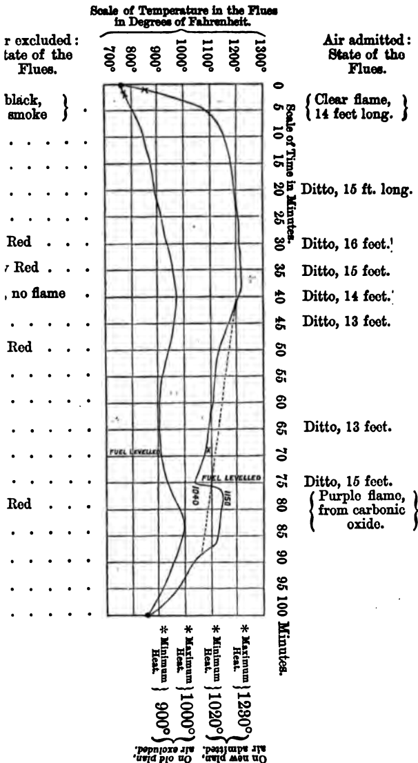
Fig. 16.—Diagrams of temperature in boiler-flue.
