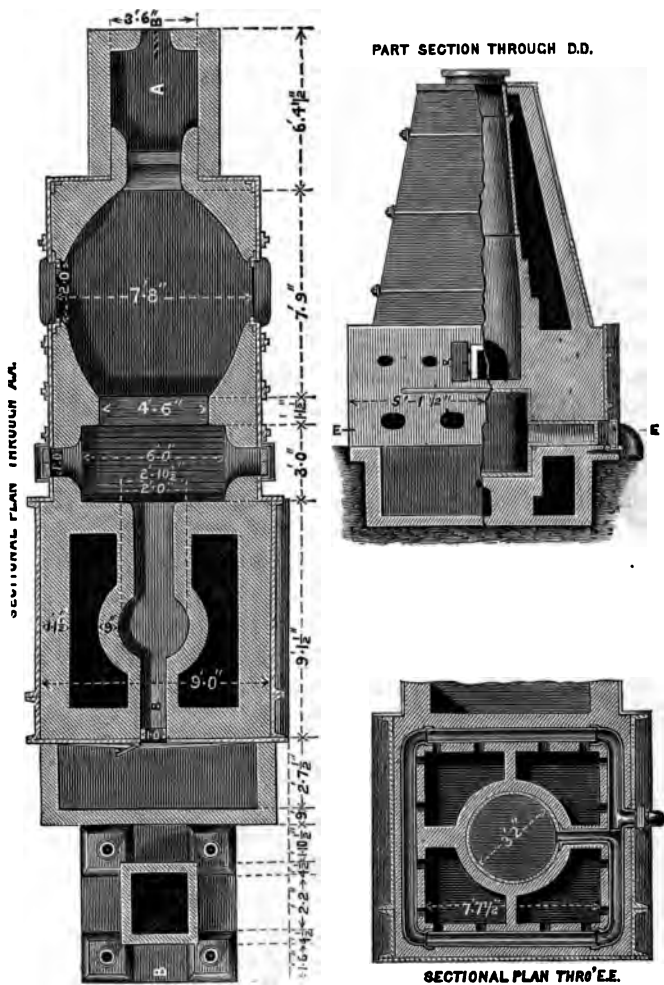
Figs. 180.—Price's Retort Furnace.
