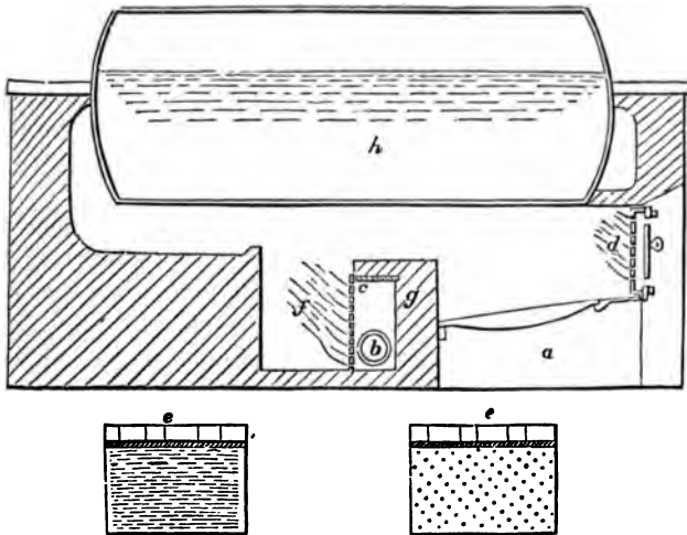
Fig. 31.—Argand Furnace.
