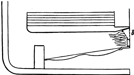
Fig. 61.—Argand Furnace.
