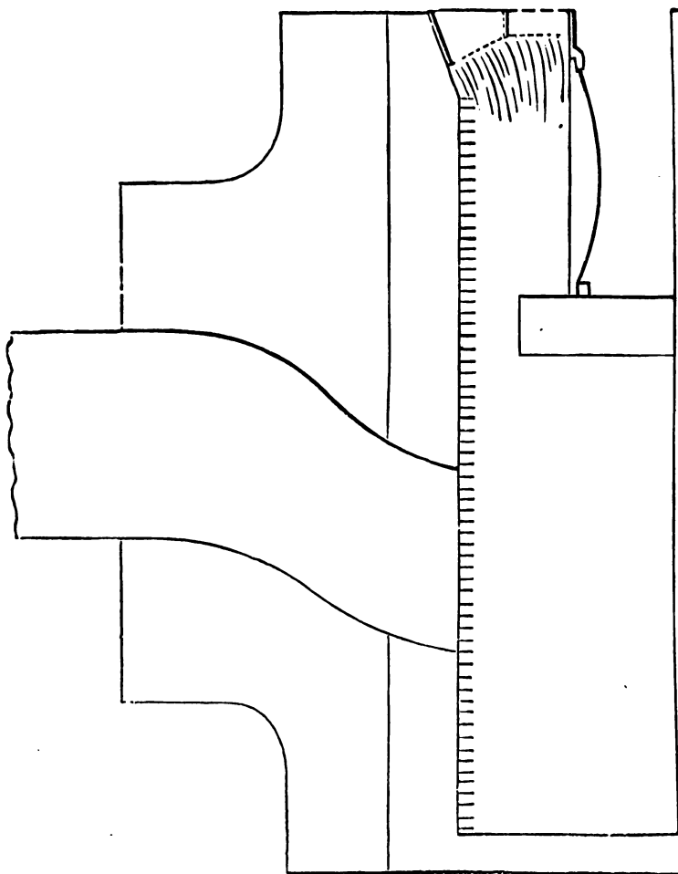
Fig. 112.—Boiler of the " Royal William ."
