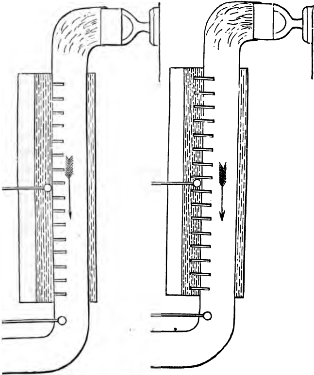
Fig. 109.—Evaporated 7 lbs. 14 oz.
