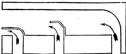
Fig. 89.—Draught in Flues.
