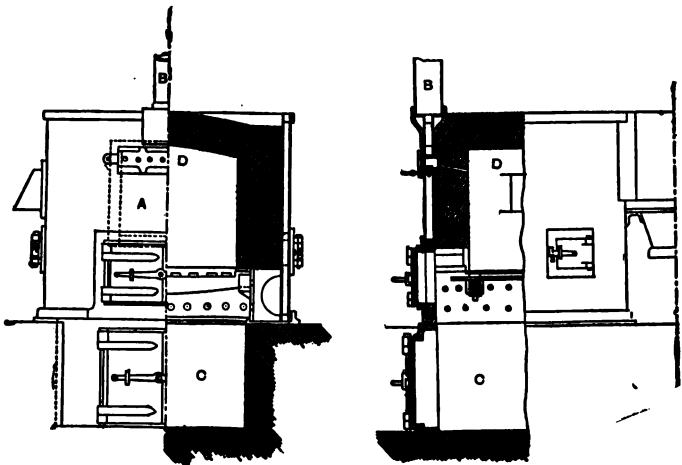
Fig. 181.—Caddick and Mabery's Furnace.
