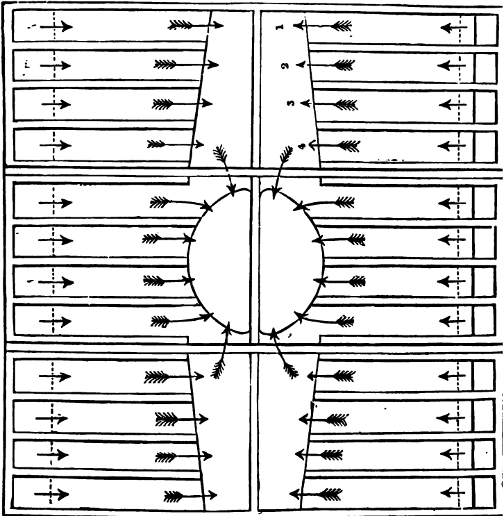
Fig. 92.—First Boilers of the "Great Britain."
