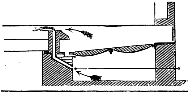
Fig. 53.—Hot-air expedient and Split Bridge.
