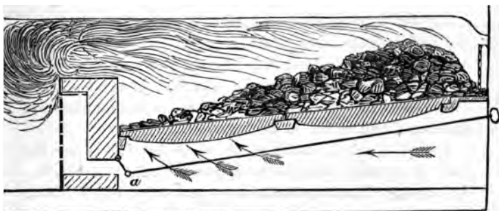
Fig. 63a.—Improper Firing.
