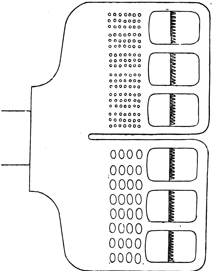
Fig. 102.—Boiler of the "Leeds."
