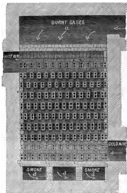
Fig. 137.—The Ponsard Gas-Furnace.—Longitudinal Section through Recuperator.
