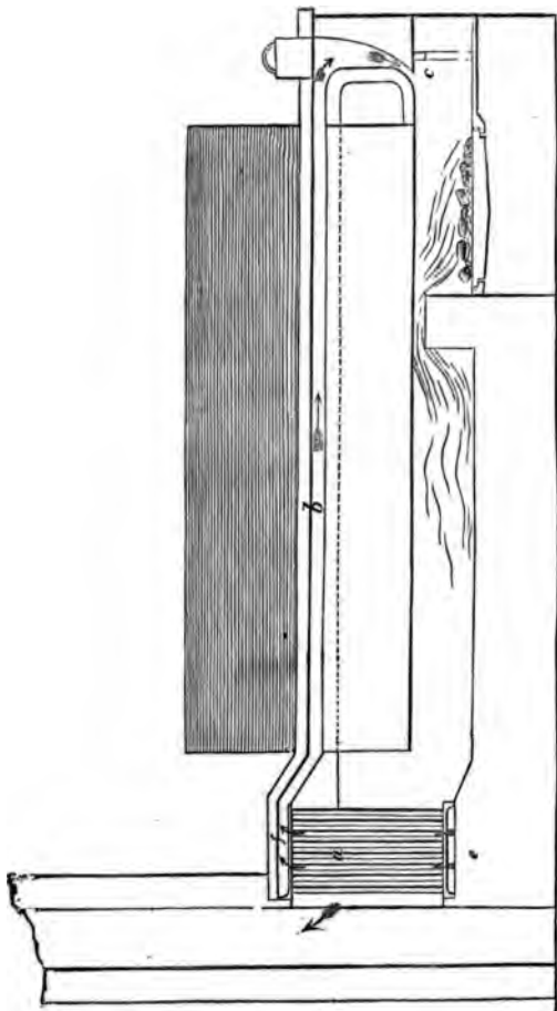
Fig. 57.—Hot Air from the Flues.
