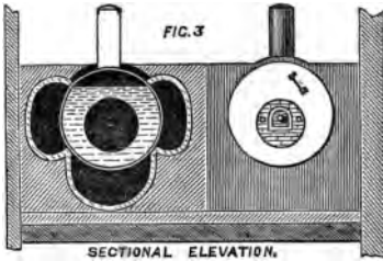
Fig. 144.—Stevenson's Coal-Dust Furnace.
