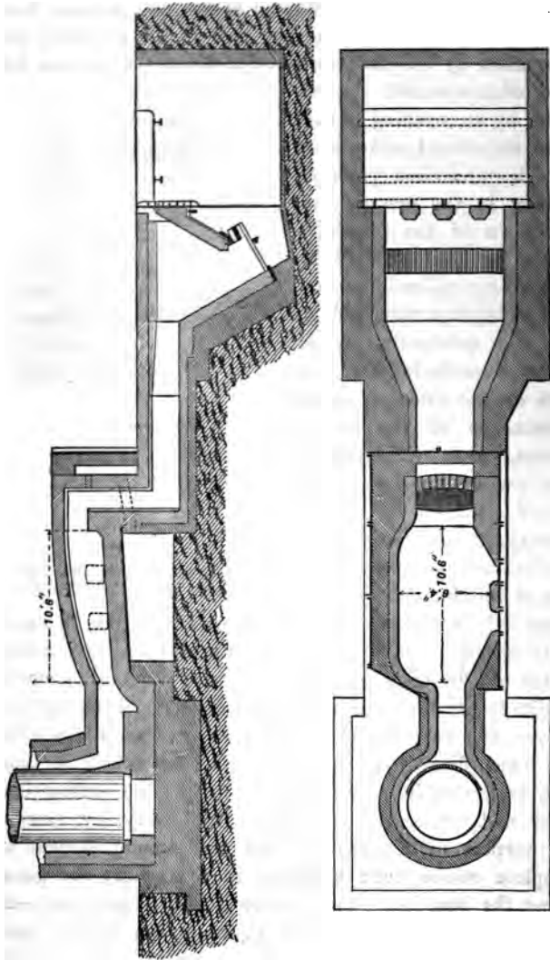
FIG. 127.—The Bessemer Pudding Furnace.
