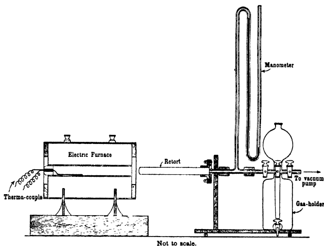
FIG. 7a.—Distillation Apparatus used by Burgess and Wheeler.
