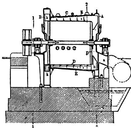
FIG. 71.—Theissen Washer (Side Elevation.)
