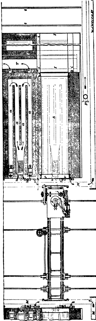
FIG. 42.—Pernolet's Coke Oven (Horizontal Section at Different Heights). (From Phillips and Bauerman's Elements of Metallurgy .)
