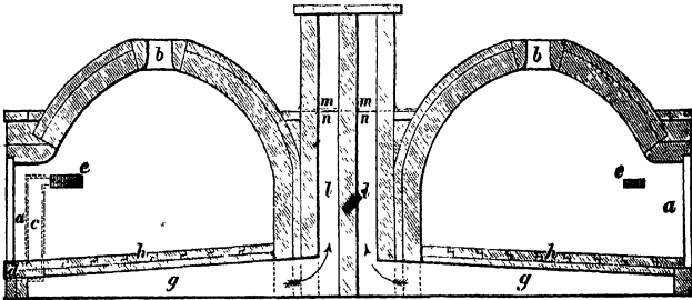
FIG. 40.—Breckon and Dixon's Coke Ovens (Sectional Elevation).
