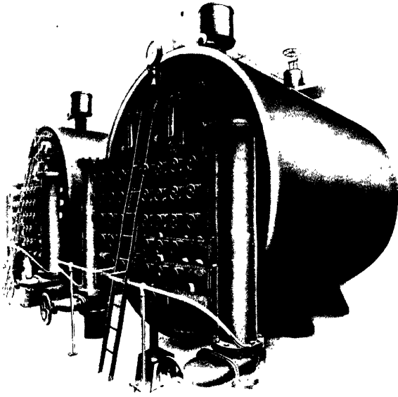
FIG. 91.—Front View of Bonecourt Surface Combustion Boiler
