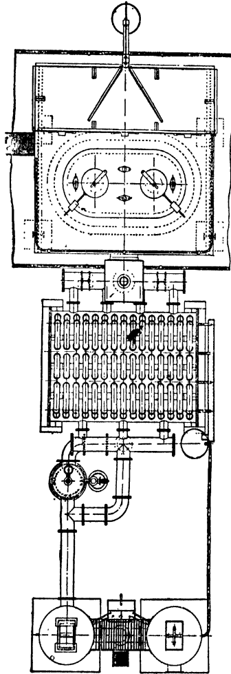
FIG. 58.—“Moore,” Water-jacketed Producer with By-product Recovery (Plan).
