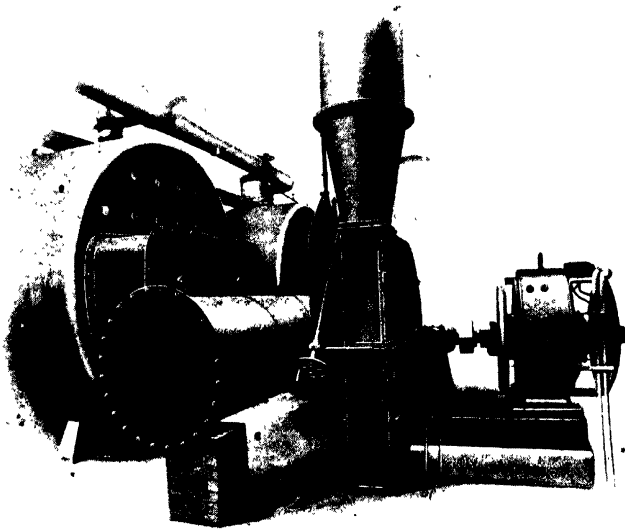
FIG. 92.—Back View of Bonecourt Surface Combustion Boiler.
