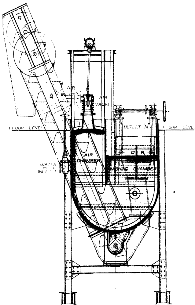
PLATE 11 — Baum Washer Box (End Elevation).
