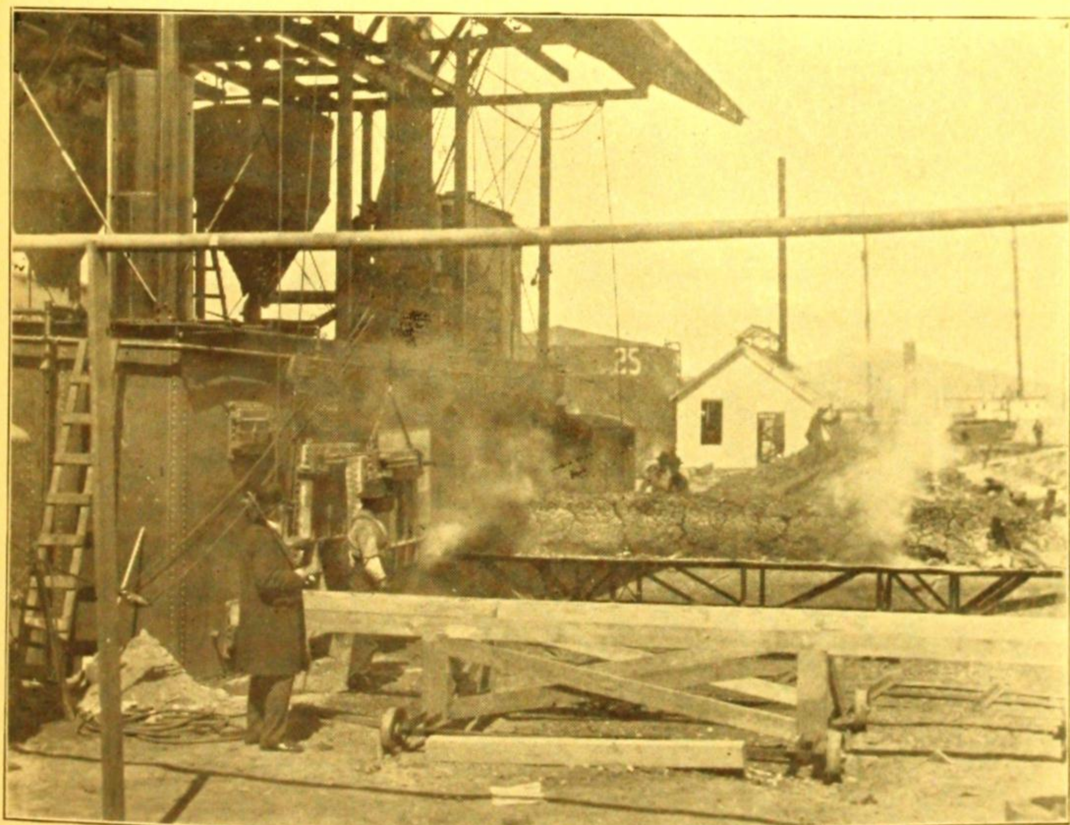
FIRST BLOCK OF LOWE ANTHRACITE COKE DRAWN FROM EXPERIMENTAL OVENS AT SAN FRANCISCO, APRIL, 1901.
