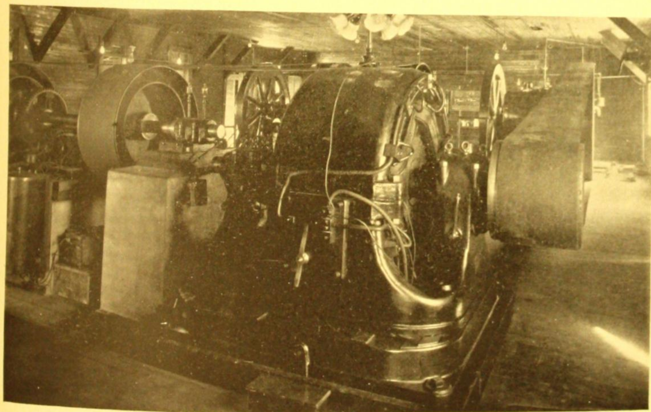
LARGE 500 VOLT ELECTRIC GENERATORS, BELT DRIVEN BY GAS ENGINES, FOR ELECTRIC STREET RAILWAYS.
