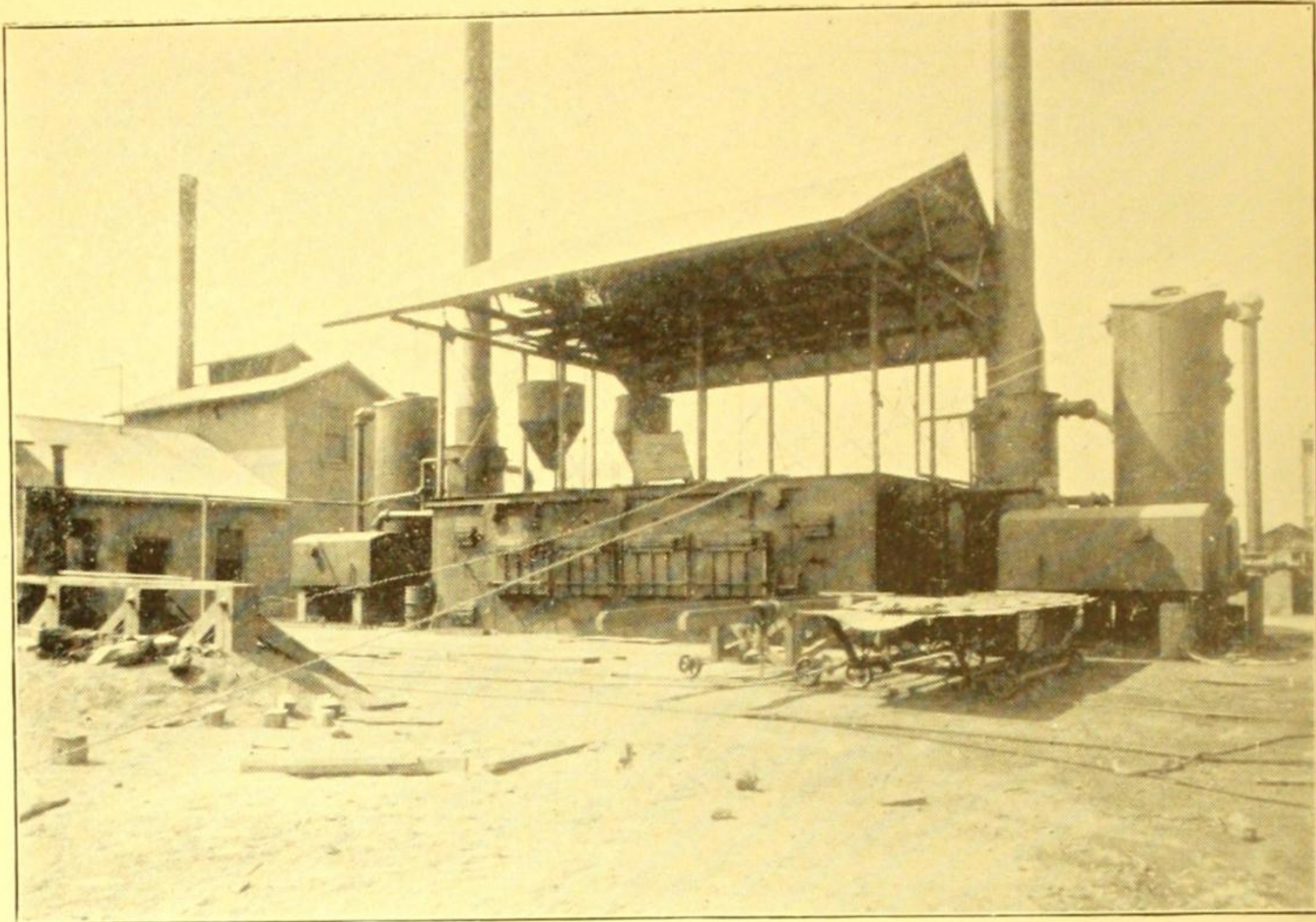
GENERAL VIEW OF EXPERIMENTAL LOWE ANTHRACITE COKE OVENS, AT SAN FRANCISCO.
