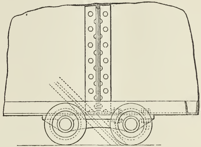
Elevation of Carriage.
