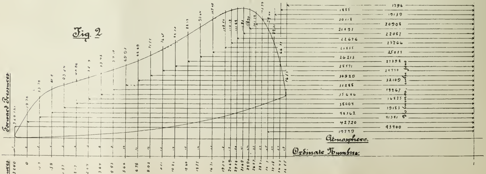
Indicator Diagram of Otto Gas Engine. Mean of 42 Cards. Scale, 25 lbs = 1" 3/16 in. ft = 1' Speed, 161.6 Revolutions per minute. Area card = 22 sq. in. Mean effective pressure = 59 lbs.
