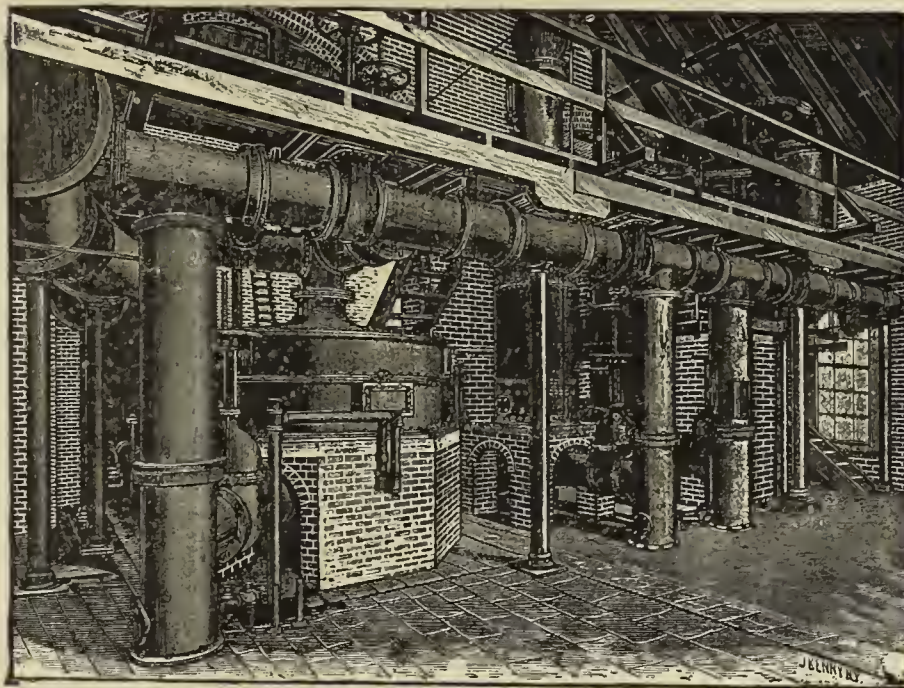
Purifying Machine erected at Cleveland Gas Works, No. 2. Capacity, 1,250,000 Cu. Ft.
