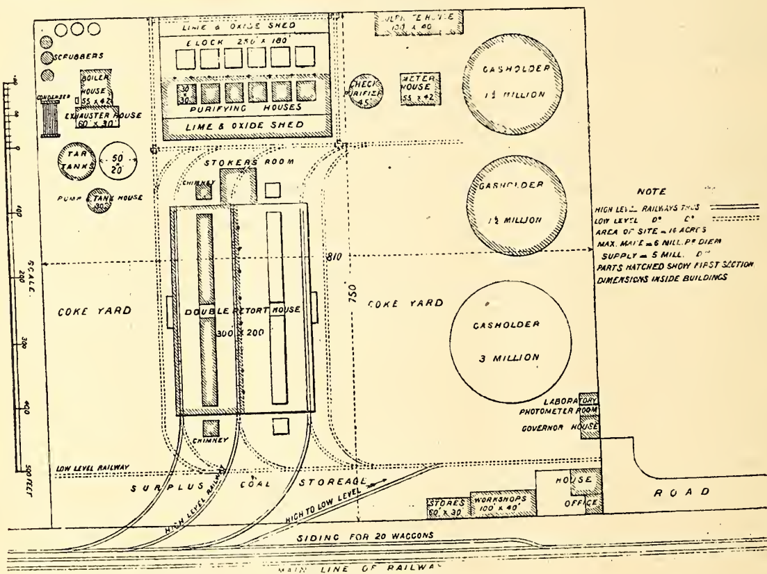
Sketch Plan of Gas Works.
