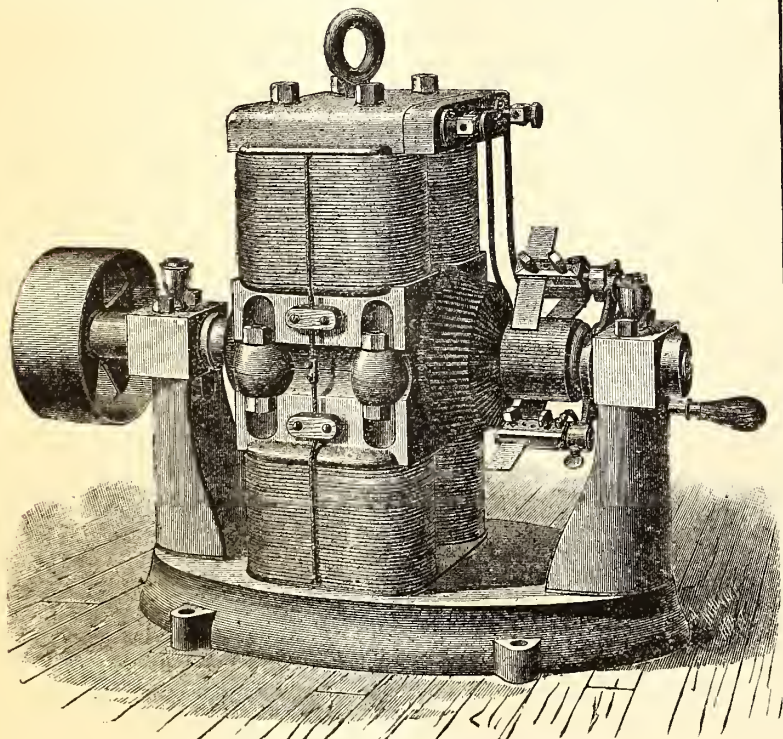
No. 3 Dynamo, Waterhouse System.
