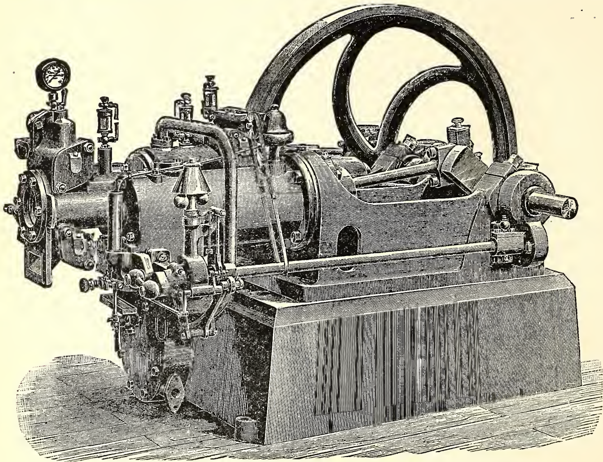
Combined Gas Engine and Refrigerator.
