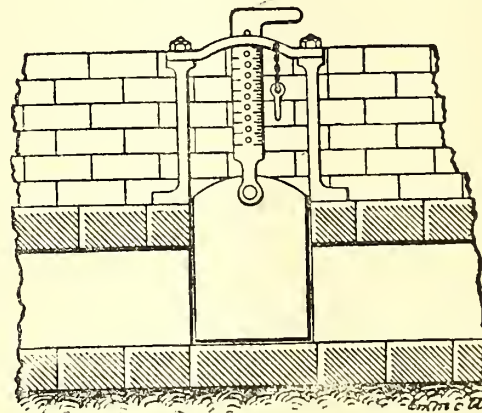
Humphrys' Patent Damper Frame for Furnaces.
