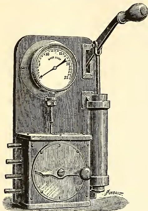
Pneumatic Hydrometer.
