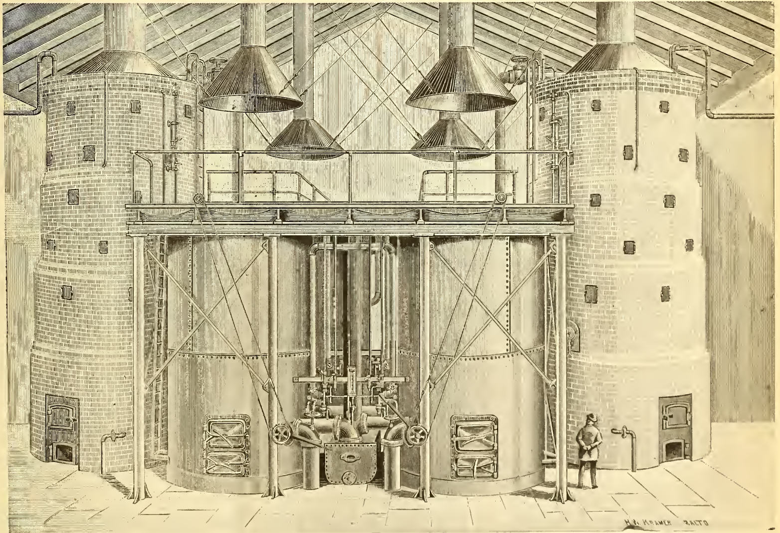
The Wilkinson Water Gas Process.
