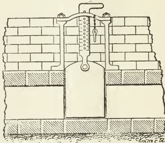
Humphrys' Patent Damper Frame for Furnaces.
