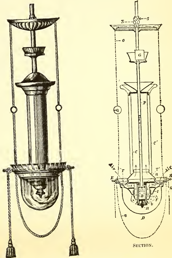
The New Lungren Lamp.
