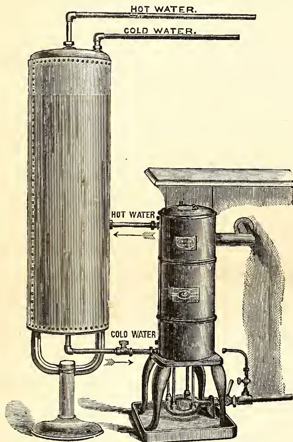
I.—Safety Hot Water Generator and Boiler.
