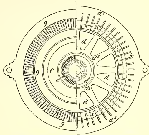
Fig. 2.—Horizontal Half-Sections.
