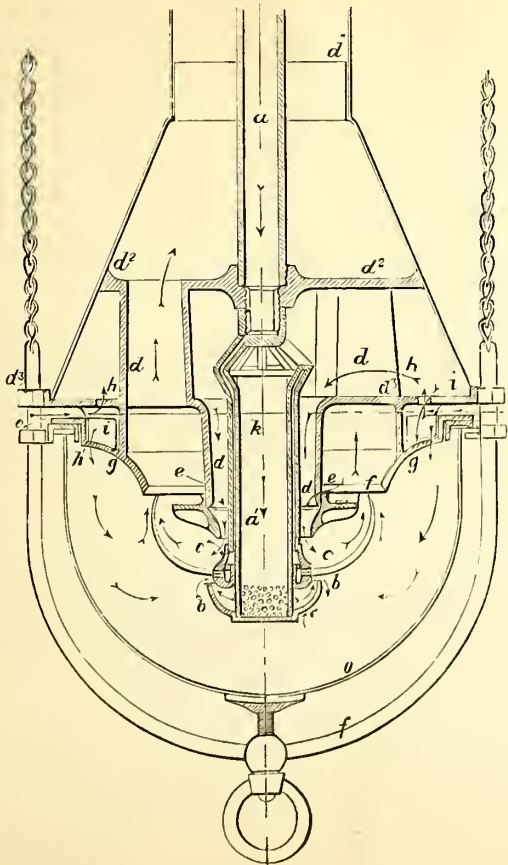
Fig. 1.—Vertical Section.
