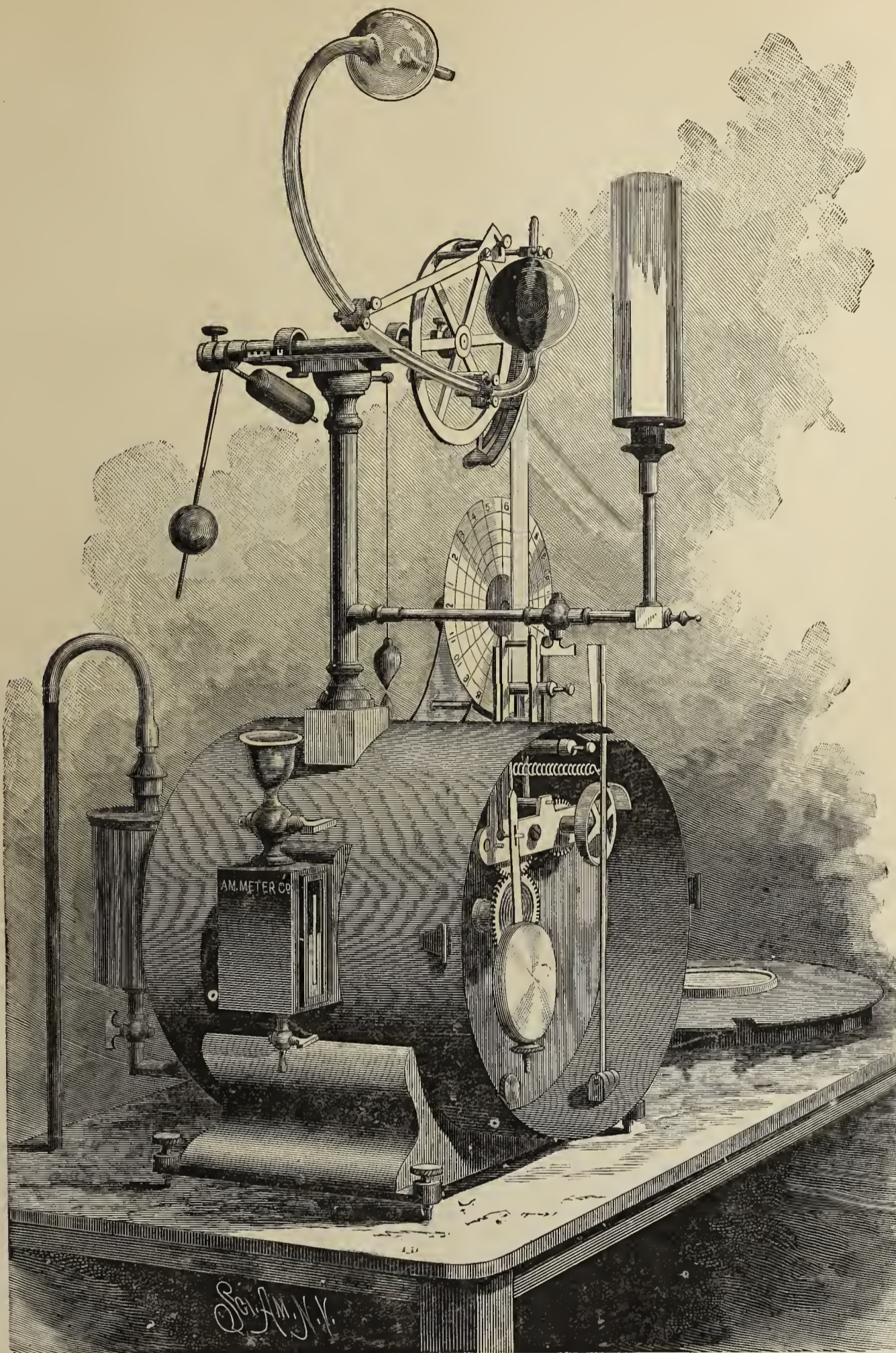
THE THERMOPHOTE, OR SELF-REGISTERING PHOTOMETER.
