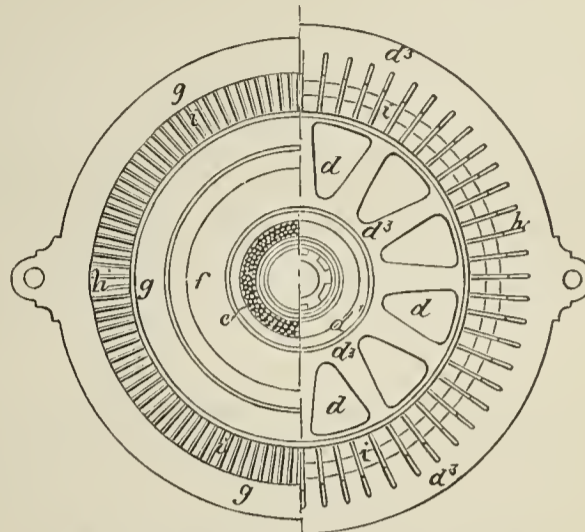
Fig. 2.—Horizontal Half-Sections.
