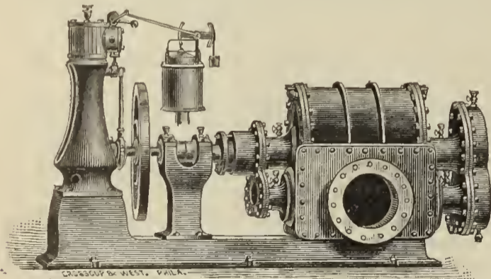
The Wilbraham Gas Exhauster.
