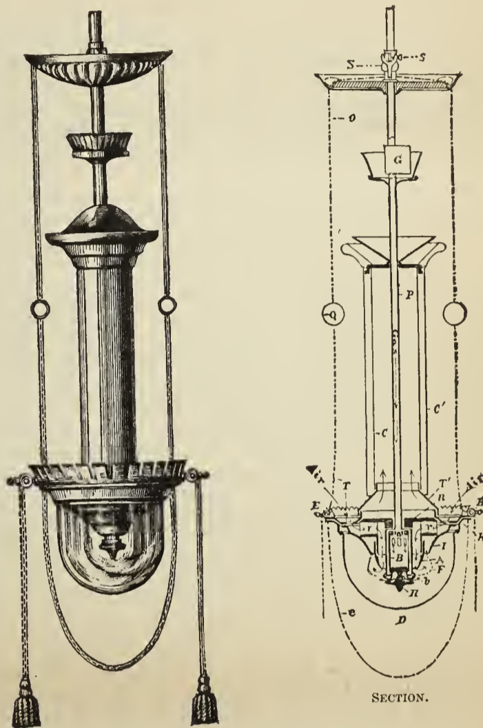
The New Lungren Lamp.
