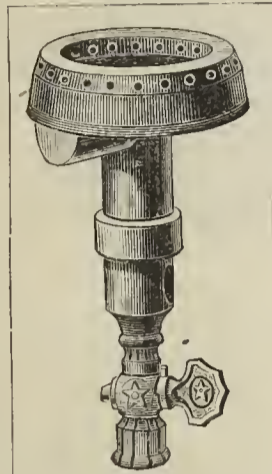
BURNER, by use of which Gasoline Stove is changed to Gas Stove.
