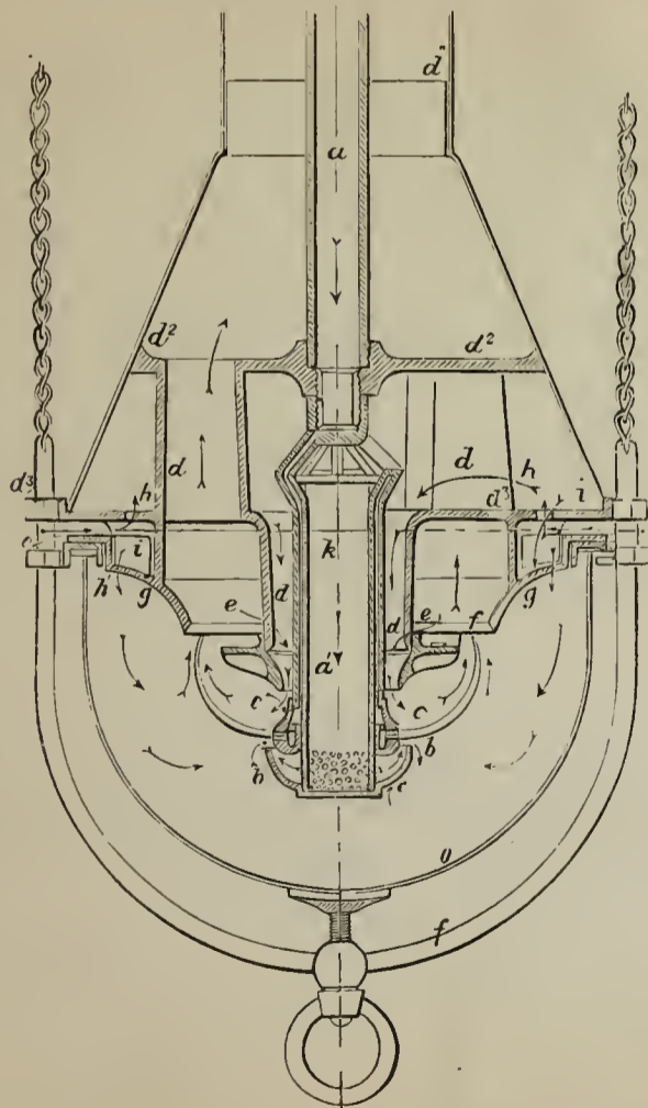
Fig. 1.—Vertical Section.
