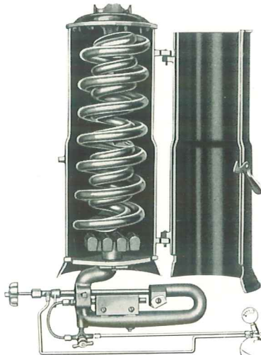
No. 9 Pressure Gasoline Water Heater
