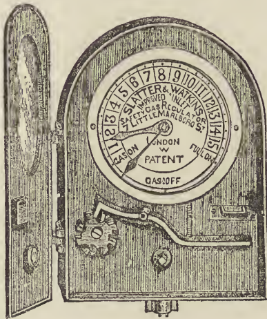
INLET SAFETY DOUBLE CHECK GAS REGULATOR.
