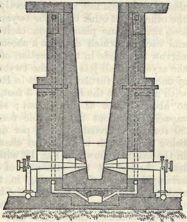
Fig. 18.—Sectional Elevation of the Rchette Furnace.
