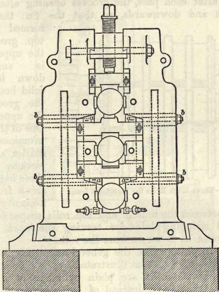
Fig. 63.—End Elevation of Housing for Three High Rolls.
