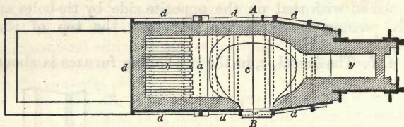
Fig. 44.—Horizontal Section showing Plan of Bed of Puddling Furnace.
