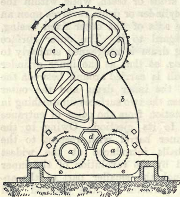
Fig. 53.—End Elevation of the Danks-Winslow Squeezer.
