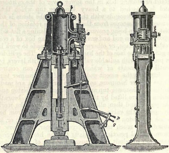
Fig. 55.—Front Elevation of Double-Acting Steam Hammer, for Shingling of Puddled Balls and Cogging of Steel Ingots, showing the Steam Cylinder, Valves, and Hammer tup in section.
