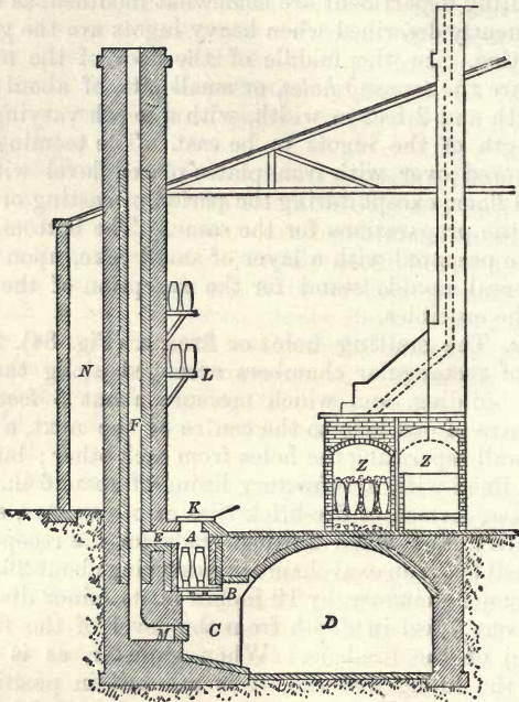
Fig. 84.—Crucible Cast-steel Melting Furnace.
