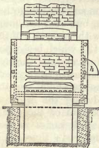
Fig. 45.—End Elevation of Puddling Furnace.
