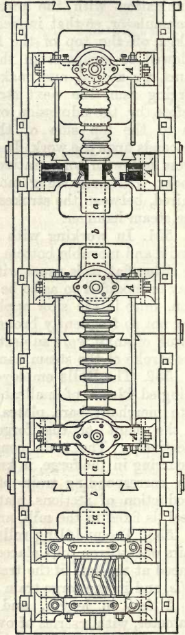
Fig. 60.—Plan of Mill Rolls with one Standard in Section.
