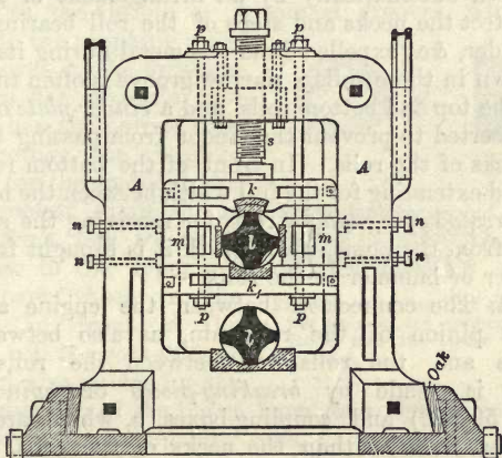
Fig. 61.—End Elevation of Roll Housing, or Standard for the Mill Rolls.
