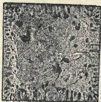
Fig. 95.—Cross Section towards the Top End of a Bessemer Steel Ingot showing Honeycombs.
