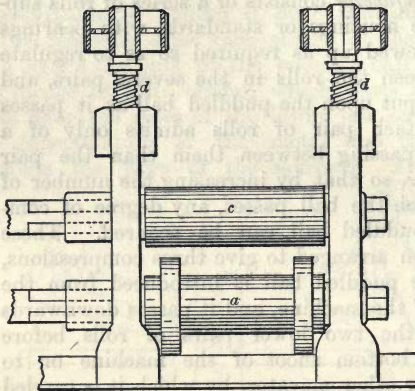
Fig. 51.—Front Elevation of Squeezer for Puddled Balls.
