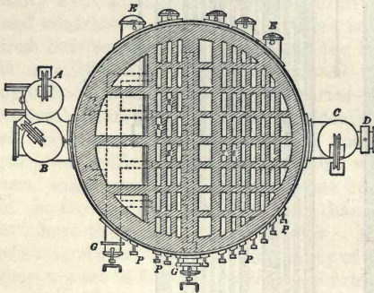
Fig. 28.—Sectional Plan of the Whitwell Hot-blast Stove.
