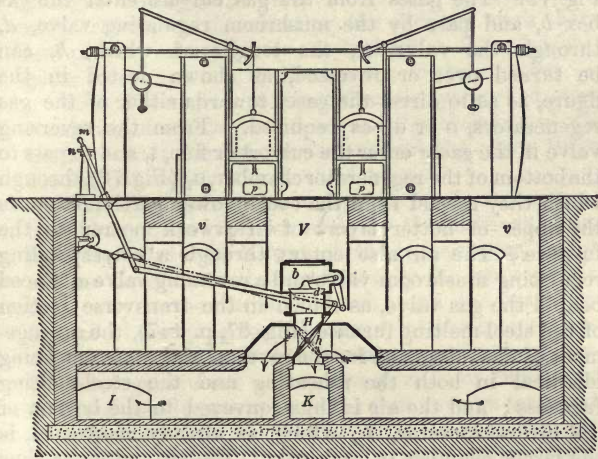
Fig. 79.—Front Elevation of Siemens Mill or Reheating Furnace, with Section through the Cave and Reversing Valve.
