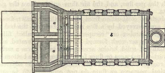
Fig. 81.—Plan of the Bicheroux Reheating Furnace, on the line A B C D. (Fig. 80.)
