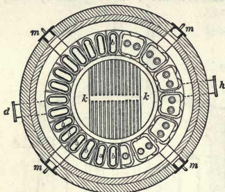
Fig. 23.—Horizontal Section of Circular Hot-blast Pipe Stove on line A B C D , Fig. 22.
