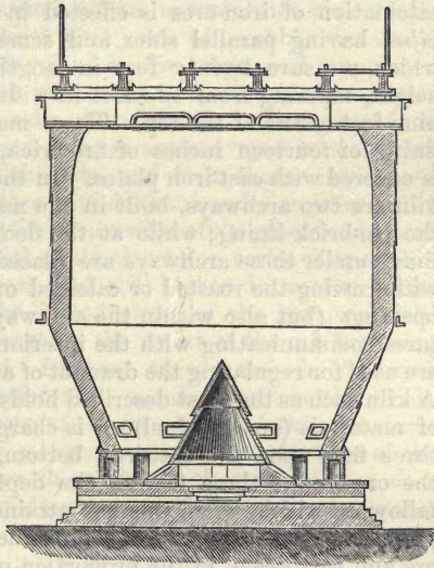
Fig. 7.—Vertical Section of Gjers' Calcining Kiln.
