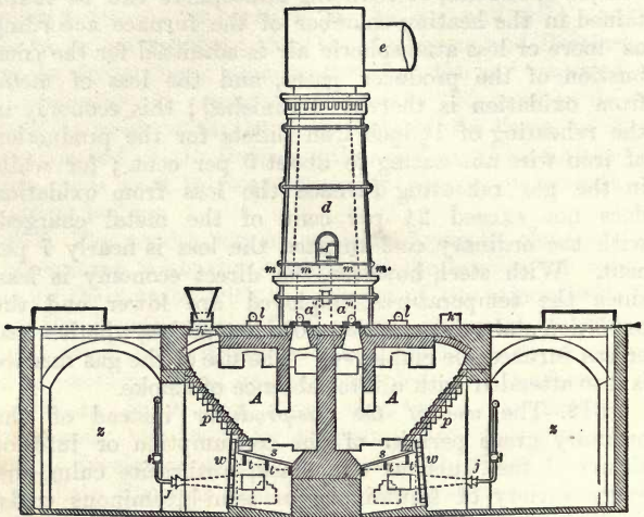
Fig. 74.—Vertical Section through Two of Siemens Gas-producers.
