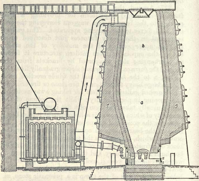
Fig. 11.—Vertical Section of the Older Type of Close-topped Blast furnace, with Rectangular Hot-blast Stoves.
