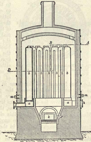
Fig. 22.—Sectional Elevation of Circular Hot-blast Pipe Stove.
