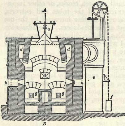
Fig. 77.—Vertical Section of the Brook and Wilson Gas Producer.
