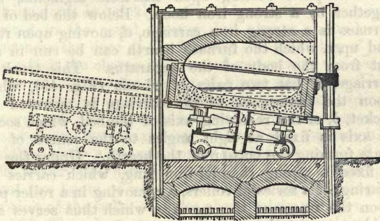
Fig. 49.—Longitudinal Cross-Sectional Elevation of the Pernot Revolving Puddling Furnace.
