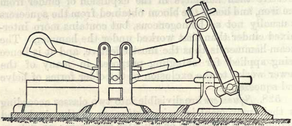
Fig. 50.—Front Elevation of Double-acting Crocodile Squeezer.
