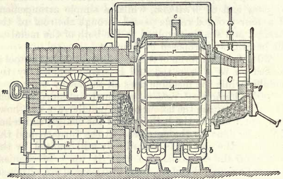
Fig. 47.—Vertical Section through the revolving Chamber and the Flue of the Danks Puddling Furnace.
