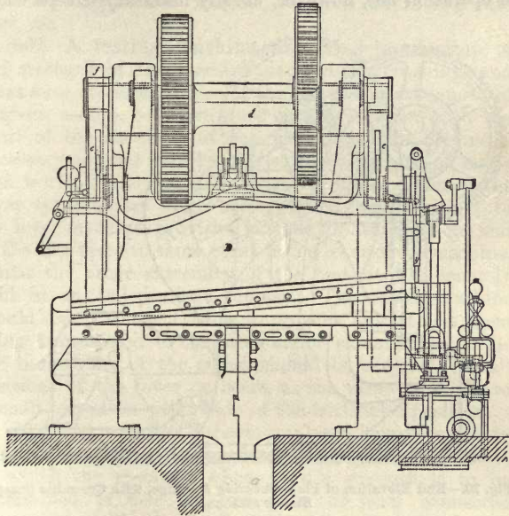
Fig. 69.—Front Elevation of Plate-Shearing Machine
