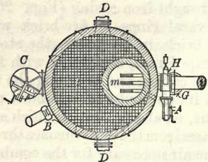
Fig. 26.—Plan of the Cowper Hot-blast Stove.
