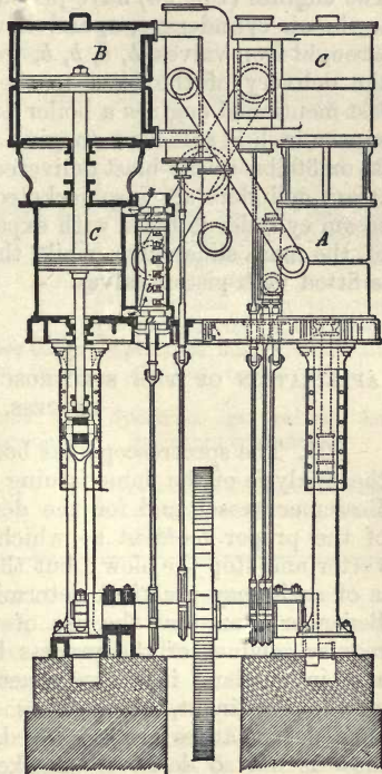
Fig. 93.—Elevation of Vertical Compound Bessemer Blowing Engines.
