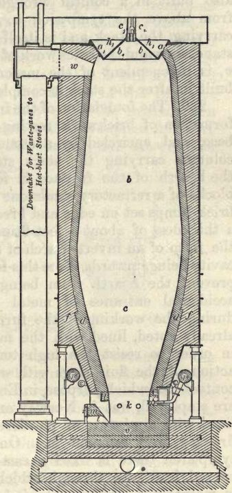
Fig. 12.—Vertical Section of the Cupola Blast furnace.
