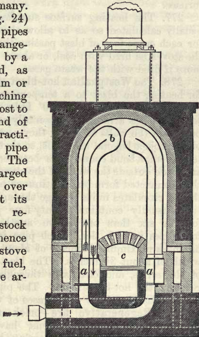
Fig. 24.—Vertical Section of Pistol-pipe Hot-blast Stove.
