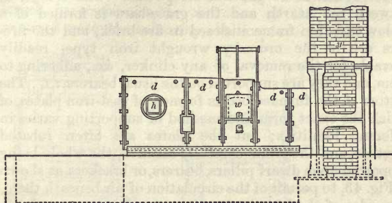
Fig. 42.—Front Elevation of Puddling Furnace.
