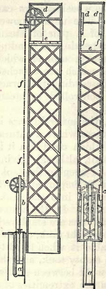
Fig. 31. — Side and End Elevation of Hydraulic Hoist.
