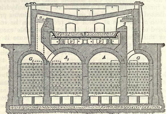
Fig. 78.—Sectional Elevation of Siemens Reheating or Mill Furnace.
