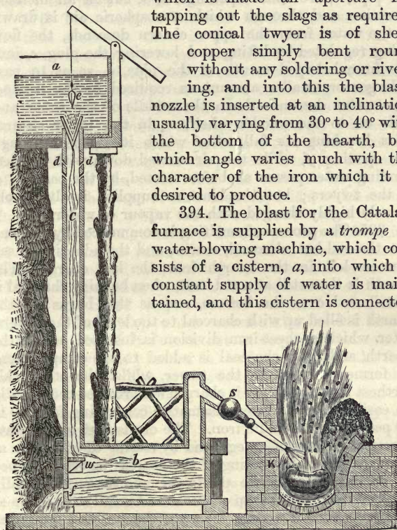
Fig. 38.—Vertical Section of Catalan Furnace and Blowing Apparatus.
