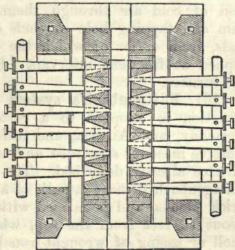
Fig. 19.—Plan of the Rchette Furnace.
