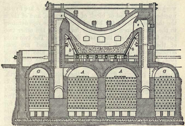
Fig. 86.—Longitudinal Section of the Siemens Open-Hearth Steel-Melting Furnace.
