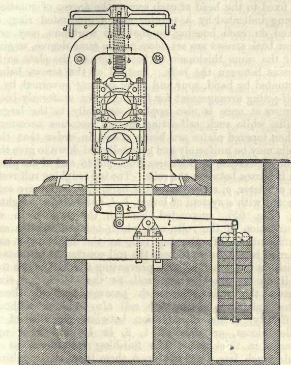
Fig. 65.—End Elevation of Plate Mill Housing, showing Balance Weights for Top Roughing Roll.
