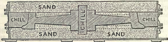
Fig. 37.—Section of Mould for Chilling Tread of Wheel.
