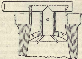
Fig. 14.—Sectional Elevation of Furnace Throat, showing arrangement for Drawing off Waste Gases by a central tube.
