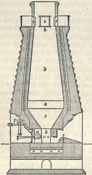
Fig. 10.—Sectional Elevation of a Staffordshire Open-topped Blast furnace.
