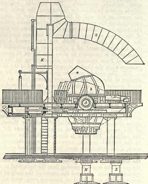
Fig. 90.—Arrangement of the Bessemer Converter.
