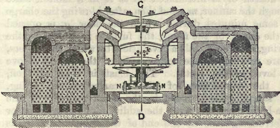
Fig. 88.—Vertical Section of the Ponsard Steel-Melting Furnace.
