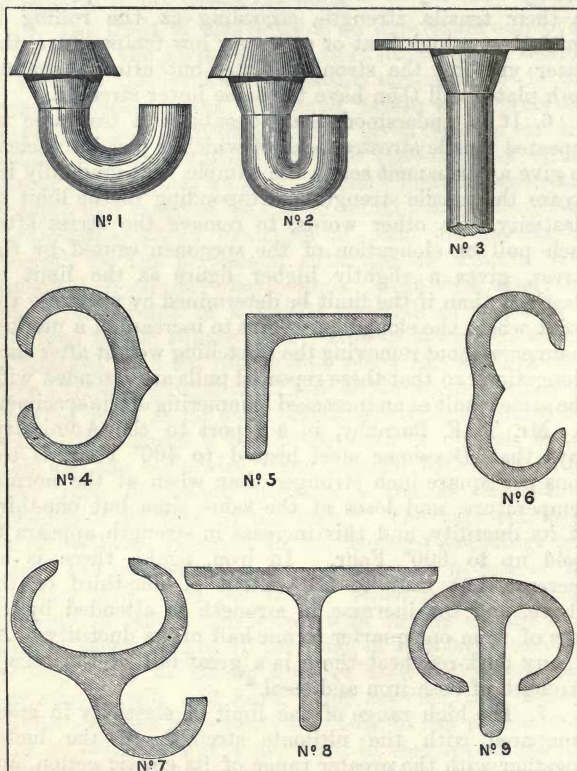
Fig. 3.—Forge Tests of the Malleability and Ductility of Iron and Steel.
