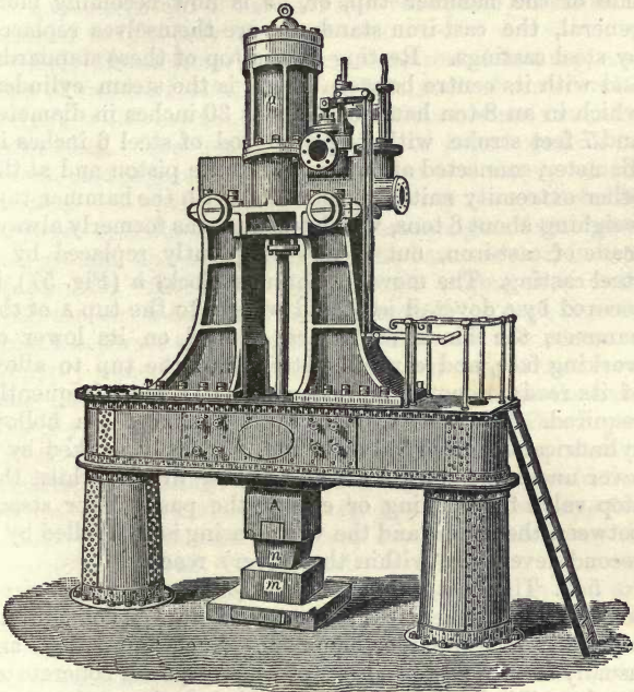
Fig. 57.—Double acting Steam Hammer for general forging purposes.
