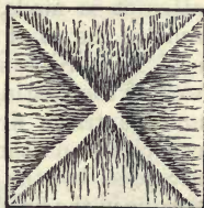
Fig. 32. — Arrangement of Crystals in a Square Flat Plate of Cast-iron.
