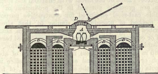
Fig. 85.—Longitudinal Section of the Siemens Regenerative Crucible Steel-melting Furnace.
