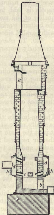
Fig. 35.—Sectional Elevation of Foundry Cupola.
