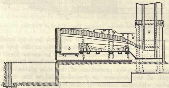
Fig. 43.—Vertical Longitudinal Section of the Puddling Furnace.
