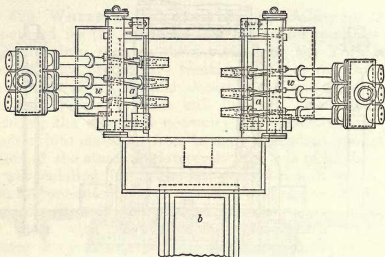
Fig. 41.—Plan of the Refinery and of the Mould for the Refined Metal.
