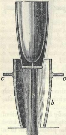
Fig. 6.—Form of Crucible on Withdrawal from the Flask.
