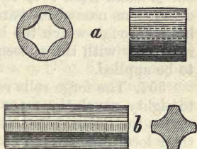
Fig. 62.—Coupling Box and Breaking Spindle for connecting the Rolls, and the Rolls with the Pinions, &c.
