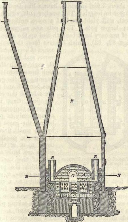
Fig. 82.—Sectional Elevation of the Cementation Furnace.
