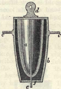
Fig. 5. — Flask and Plug for crucible-making.
