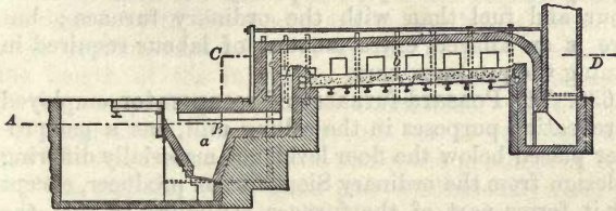
Fig. 80.—Sectional Elevation of the Bicheroux Reheating Furnace.
