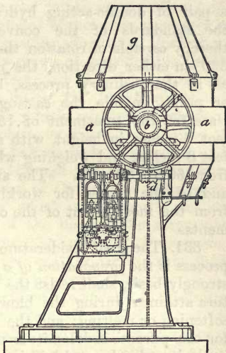
Fig. 94.—10-ton Converter employed in the Basic Bessemer Process.*
