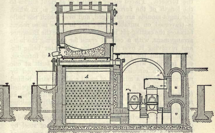
Fig. 87.—Cross Section of the Siemens Steel-Melting Furnace.
