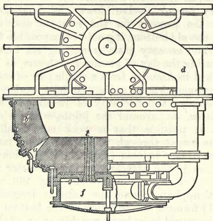
Fig. 91.—Lower Portion of Bessemer Converter showing Holley's Movable Bottom.
