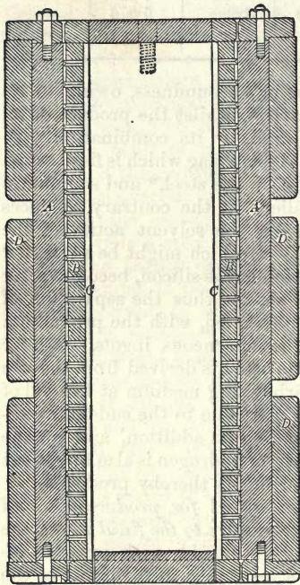
Fig. 96.—Vertical Section of the Mould employed in the Compression of Steel whilst in its Fluid State.
