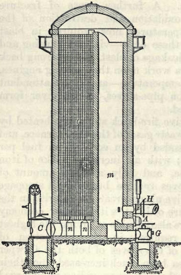
Fig. 25.—Sectional Elevation of the Cowper Hot-blast Stove.
