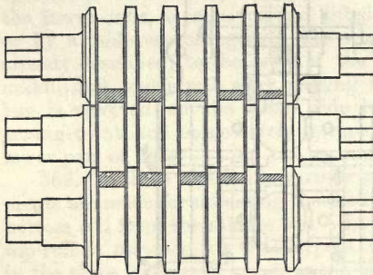
Fig.64.—Three High Rolls for Merchant Iron.
