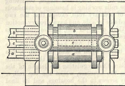
Fig. 52.—Plan of Squeezer for Puddled Balls.
