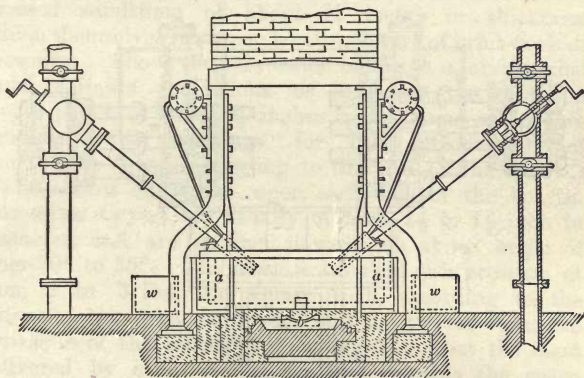
Fig. 40.—Elevation of the Refinery for converting Grey into White Iron.
