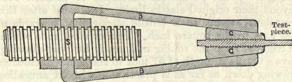
Fig. 2.—One Form of the Bridle and Grip for holding the Test-pieces in the Testing Machine. (p.352).
