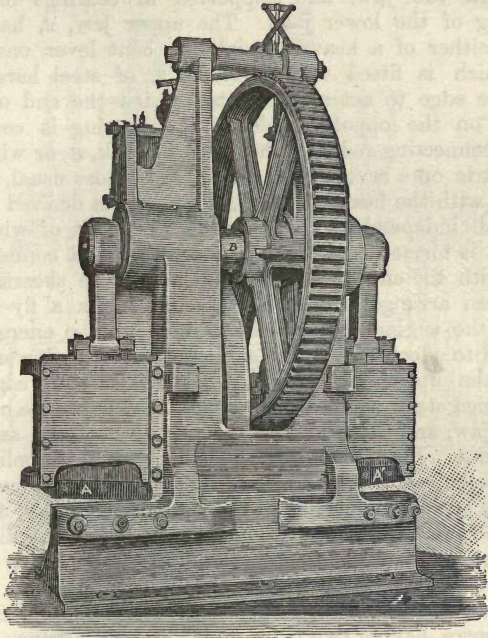
Fig. 68.—Shears for cutting up Puddled Bars and Slabs.
