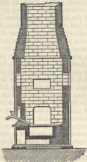
Fig. 39.—Elevation of Charcoal Finery.
