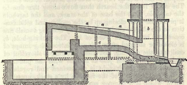
Fig. 72.—Vertical Section of Reheating or Balling Furnace.
