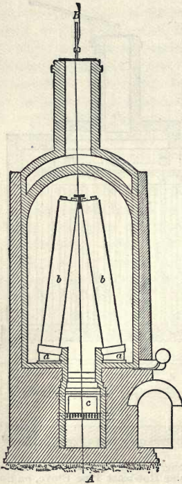
Fig. 21.—Transverse Vertical Section of Rectangular Hot-blast Pipe Stove.
