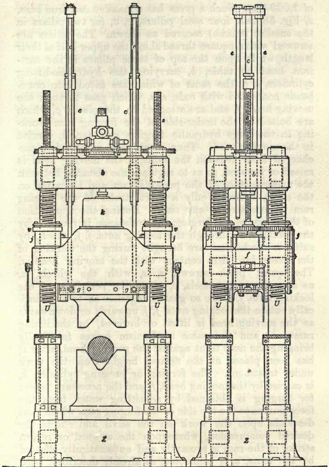
Fig. 58.—Front and End Elevation of Sir J. Whitworth and Co.'s Hydraulic Forging Press.
