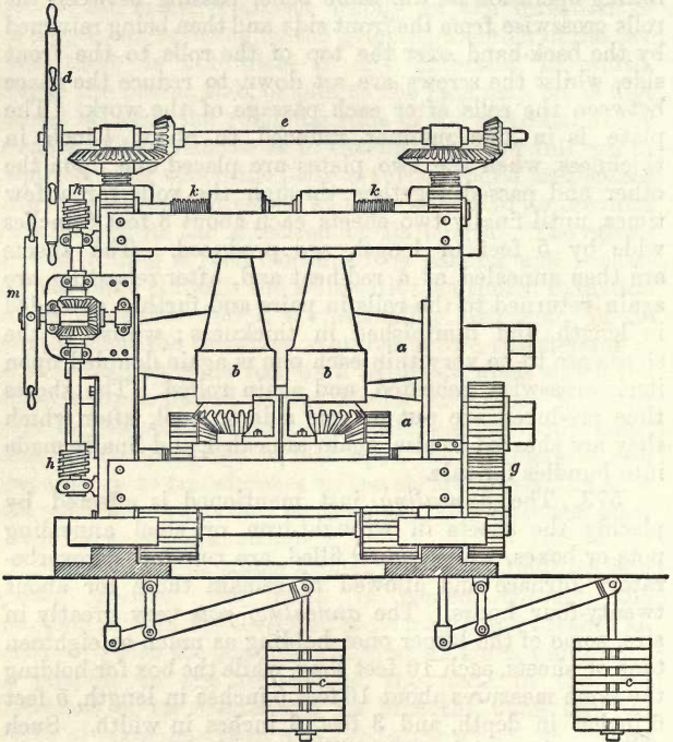
Fig. 66.—Universal or Belgian Rolling Mill.
