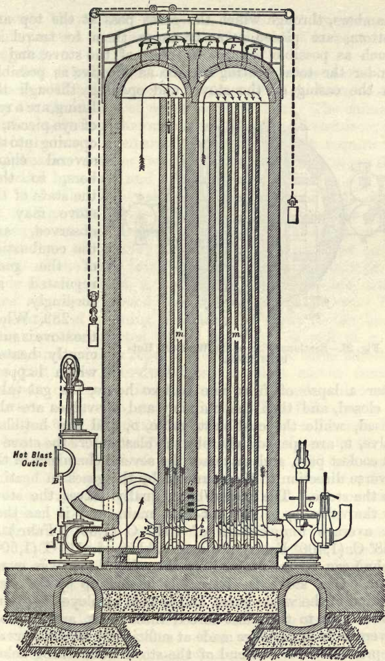
Fig. 27.—Sectional Elevation of the Whitwell Hot-blast Stove.
