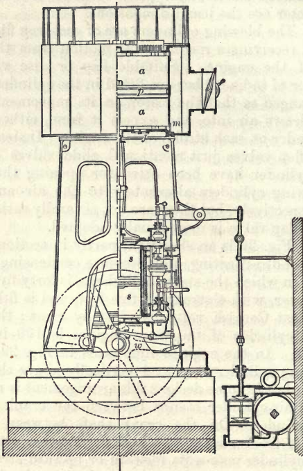
Fig. 29.—Elevation partly in Section of Blowing Engine.
