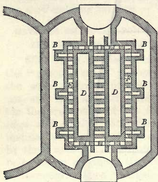
Fig. 83.—Plan of Cementation Furnace on line M, N, Fig. 82.
