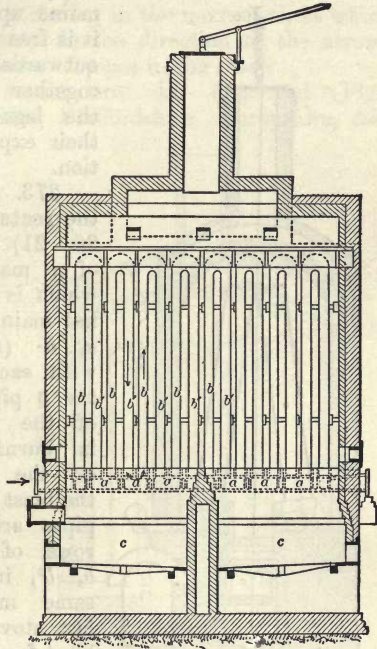
Fig. 20.—Longitudinal Vertical Section of Rectangular Hot-blast Pipe Stove, on line A B, Fig. 21.
