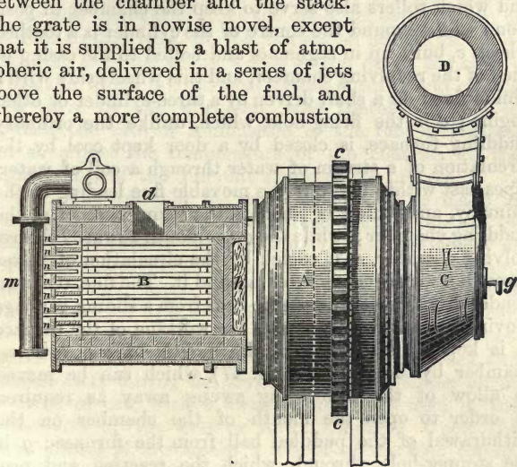
Fig. 48.—Plan of the Danks Revolving Puddling Furnace, half in Section.
