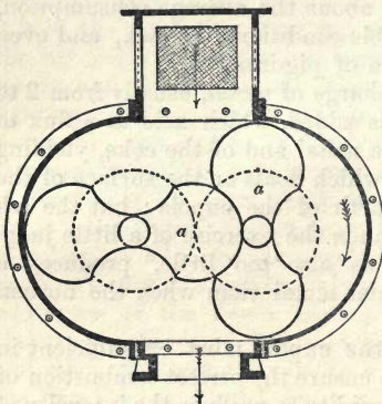
Fig. 36.—Transverse Section of the Roots Blower.
