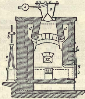
Fig. 76.—Vertical Section on line A, B, Fig. 77, of the Brook and Wilson Gas Producer.
