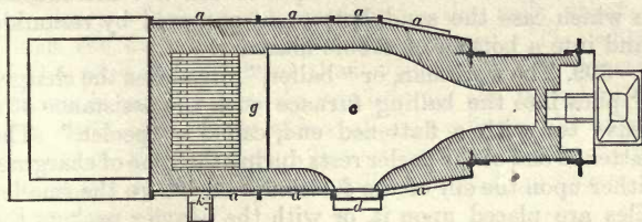
Fig. 73.—Plan of Bed of Reheating or Balling Furnace.
