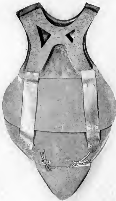
Fig. 197. Light body armor. Inner view of laminated breastplate. A heavy cushion of sponge rubber lines the uppermost plate
