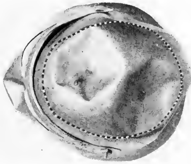
Fig. 169. Experimental helmet model No. 8. Result of test by pistol bullet at 800 f. s. Outline of head within helmet is shown by dotted line. This helmet bears marks of six testing bullets
