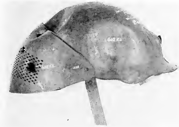
Fig. 116. Belgian helmet. Result of tests
