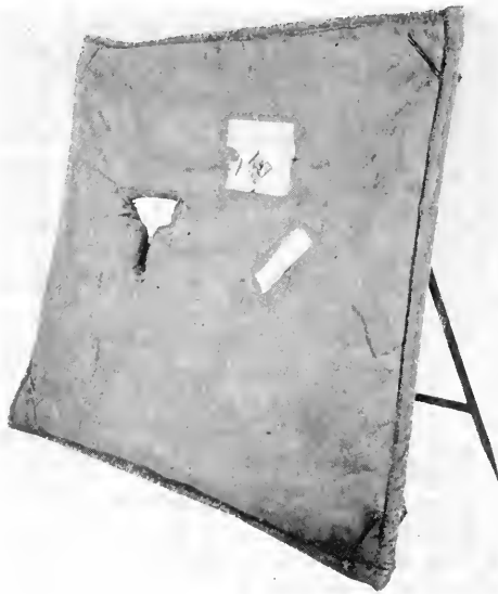
Fig. 136. Belgian trench shield. American manufacture
