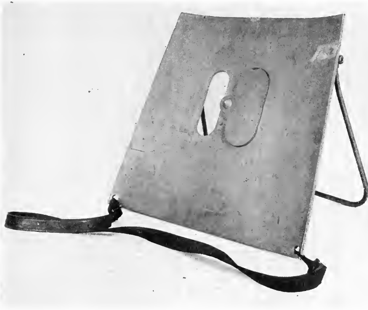
Fig. 137. Russian trench shield. American manufacture
