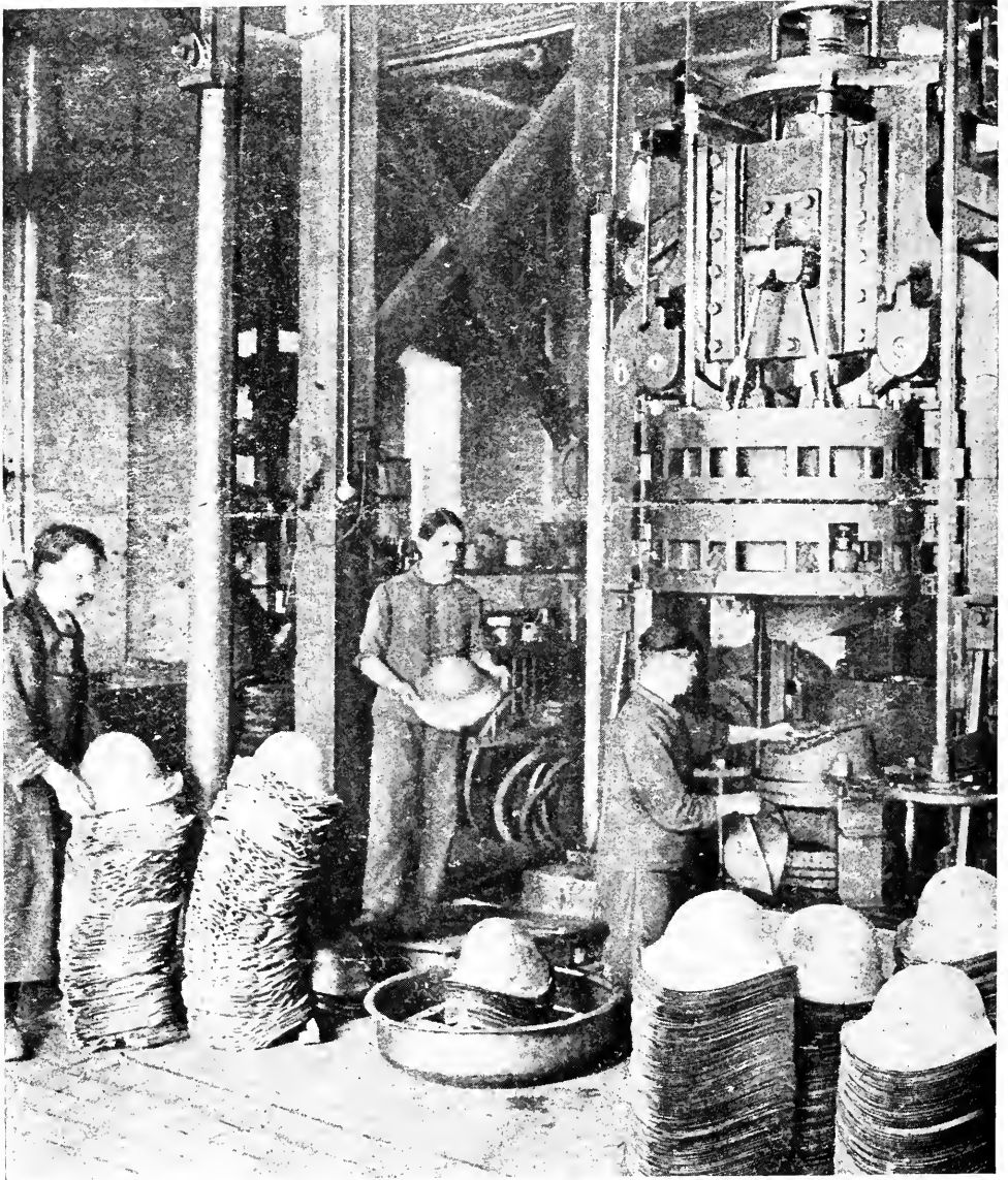
Fig. 126. Swiss standard helmet in process of manufacture
