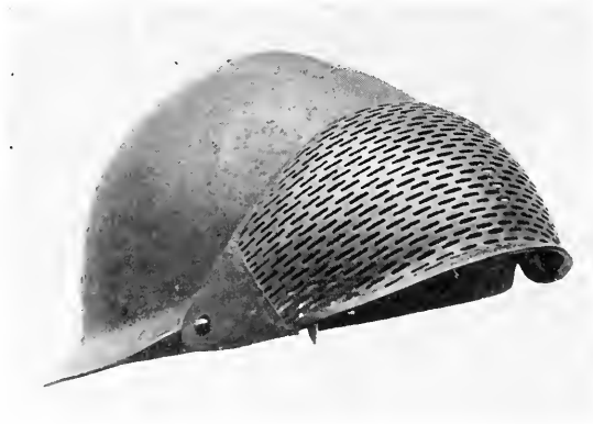
Fig. 46. Dunand helmet model, 1918, in ballistic metal
