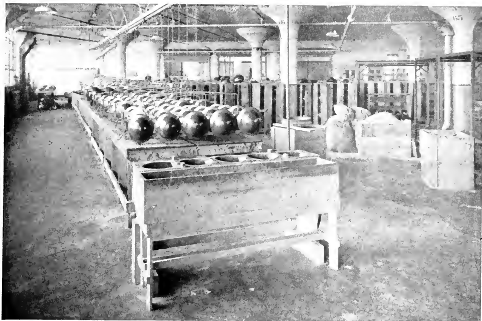
Fig. 154. British-American helmet. Assembling. Freshly painted helmets about to be given a coating of sawdust in the sprinkling box shown in the foreground
