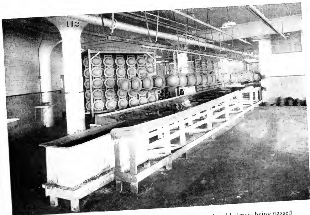
Fig. 152. British-American helmet. Assembling. The helmets are shown arranged in rows on metal racks, front and back, ready to be immersed in the paint trough shown in right of picture. (Ford Mfg. Co., Philadelphia)
