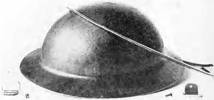
Fig. 146. Manufacture of British-American helmet. Helmet shell, metal rim, chin-strap loops and rivets ready to be put together
