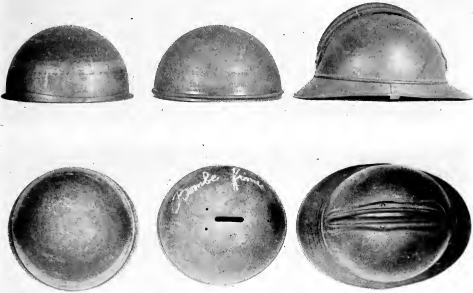
Fig. 24. Three stages in making French helmet, 1916
