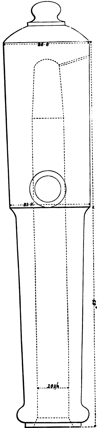
FIG. 89.—Russian 120-pounder. Scale, \frac{1}{8} in. to 1 ft.
