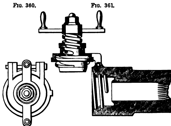
Screw breech-loader.
