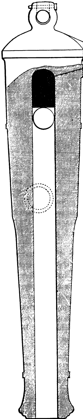
FIG. 87.—British 68-pounder (8-in.) 95 cwt. Scale, \frac{1}{8} in. to 1 foot.
