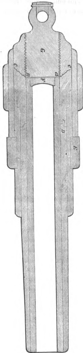
FIG. 177.—Armstrong 10½-in. muzzle-loader. Scale, ½ in. to 1 ft.
