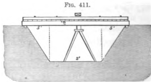
Fig. 411. Bridge of oak, 12 inches scantling, 24 feet span.
