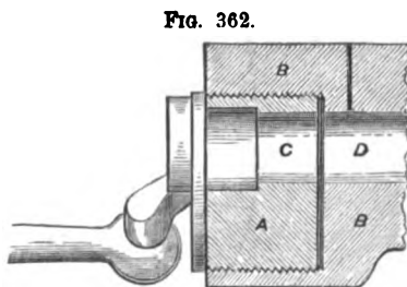
Clay's breech-loader.
