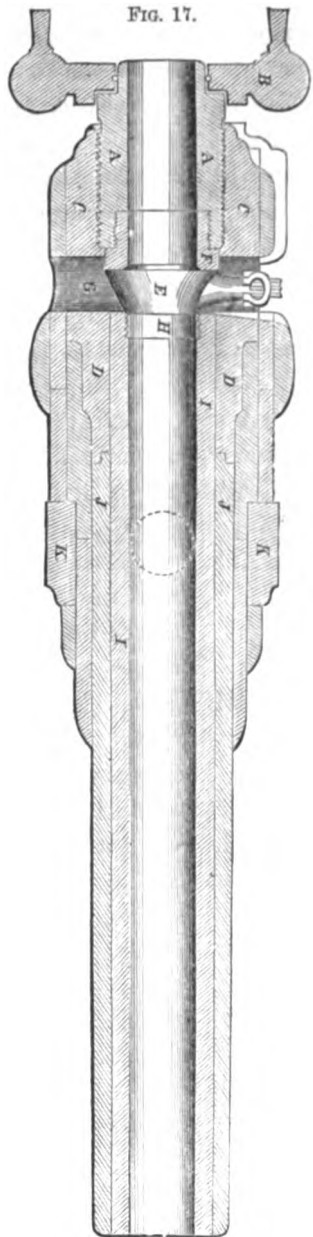
Armstrong 110-pounder. \frac{1}{10} in. to 1 ft.
