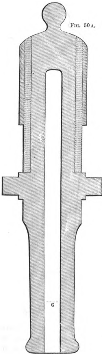
Armstrong cast-iron 70-pounder of 1860. Scale \frac{1}{10} in. to 1 ft.
