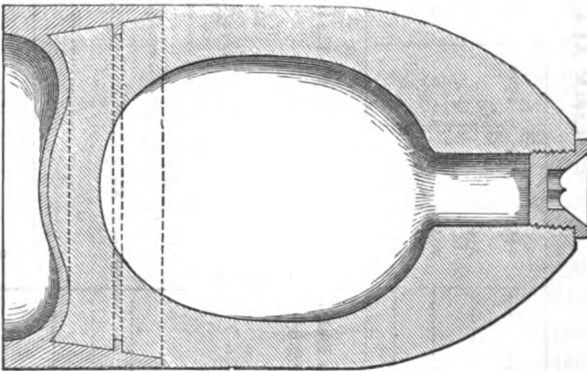
Jeffery's shell.
