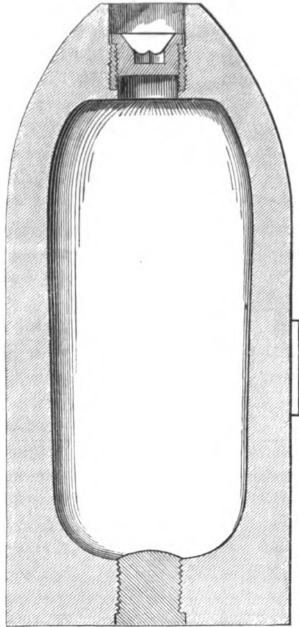
French shell.
