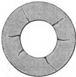
Fig. 136. Cylinder burst by internal pressure.
