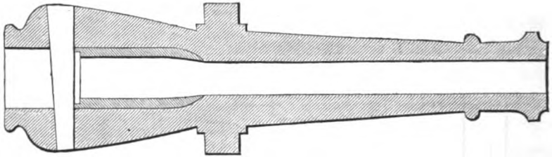
Cavalli breech-loader.
