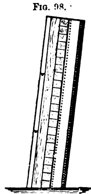
The Warrior target. Scale, \frac{1}{4} in. to 1 ft.
