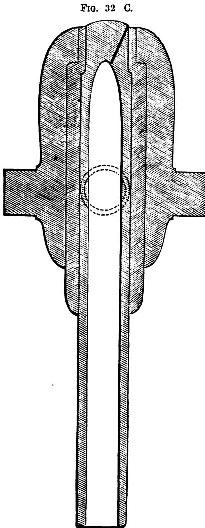
Blakely's 9-inch rifle. Low steel bore, hooped by high steel and cast iron. Scale, \frac{1}{16} in. to 1 ft.
