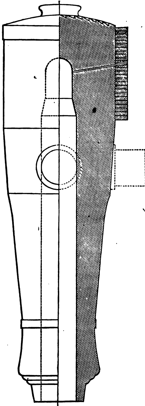
The Dumford 12-in. gun, hooped. Scale, \frac{1}{4} in. to 1 foot.
