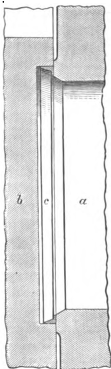
Krupp's gas-check.
