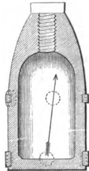
Beaulieu's, or first French service rifle shot.
