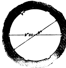
FIGS. 248 to 251.—Shunt rifling of Russian 9-in. gun. Scale, 1½ in. to 1 ft.
