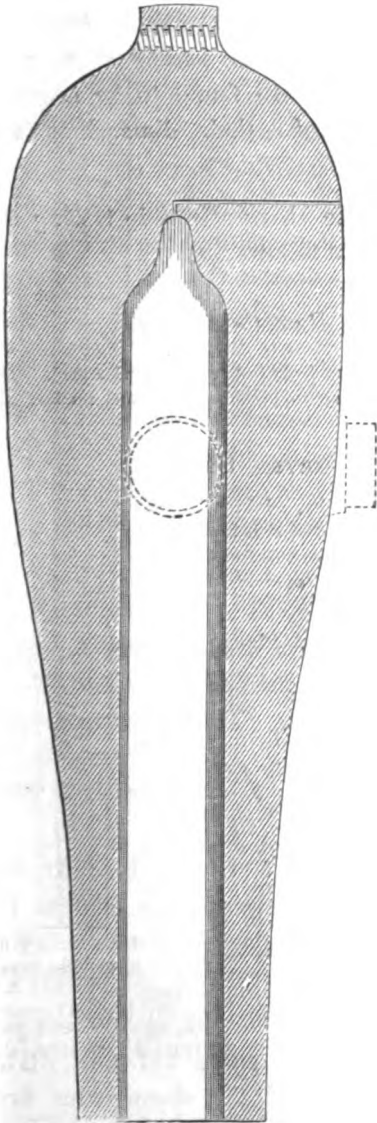
U. S. Navy 15-in. gun. Scale, \frac{1}{4} in. to 1 ft.
