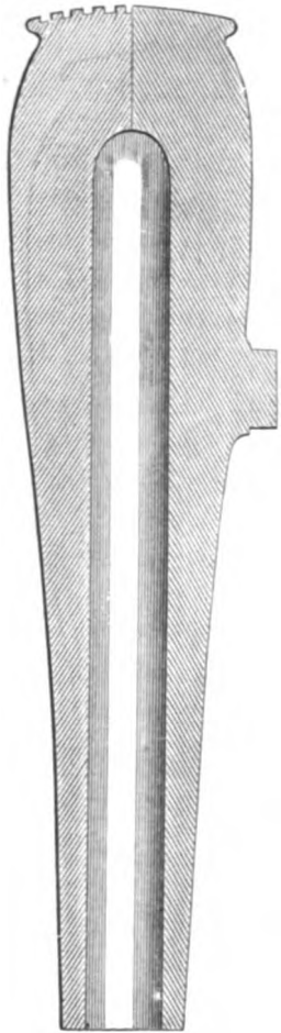
U. S. Army 10-in. Columbiad. Scale, \frac{1}{8} in. to 1 ft.
