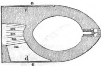
Section of James shell
