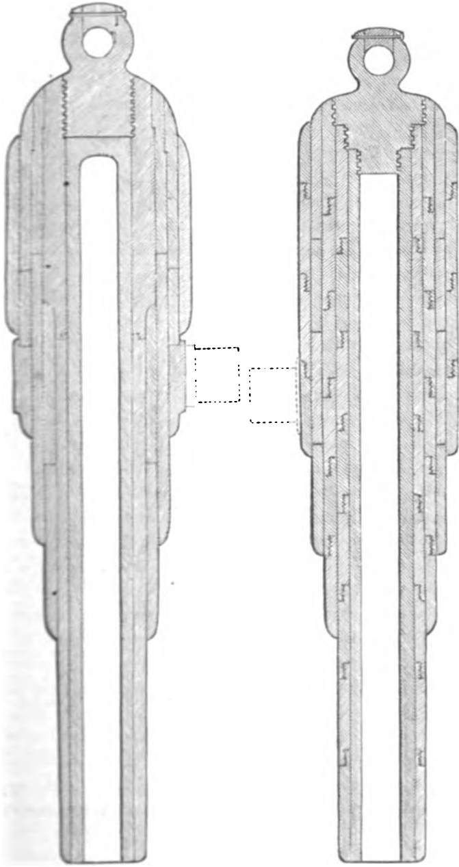
FIG. 27. 7-in. gun as built at Wadsworth and refired for Mr. Whitworth. Scale \frac{1}{16} in. to 1 ft.
