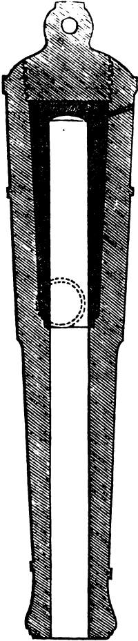
68-pounder, strengthened by Parsons's internal tube. Scale, \frac{1}{8} in. to 1 ft.
