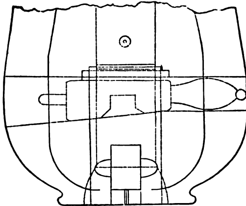
Cavalli breech-loader.
