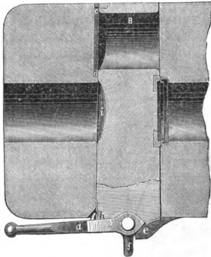
Broadwell's breech-loader.
