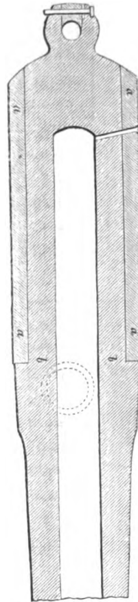
Armstrong hooped cast-iron naval gun. Scale, \frac{1}{16} in. to 1 ft.
