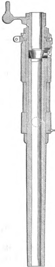
Armstrong 12-pounder. \frac{1}{8} in. to 1 ft.
