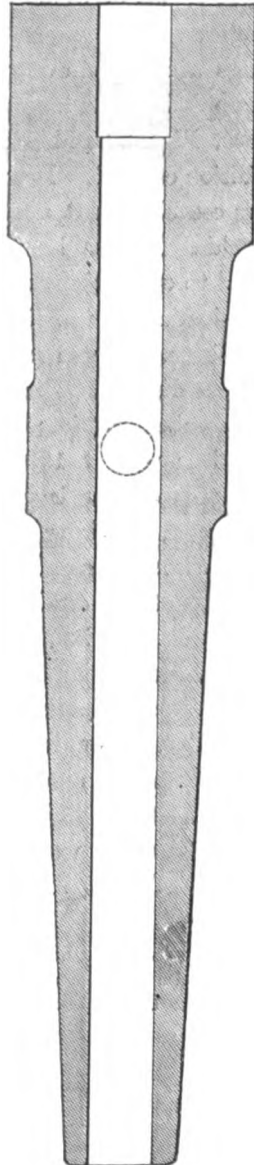
FIG. 69.—Section of Krupp's 9-inch solid steel gun in the Exhibition of 1862. Scale, \frac{7}{8} in. to 1 ft.
