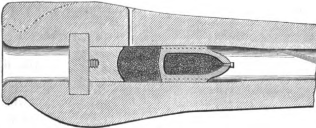
Cavalli rifled breech-loader.
