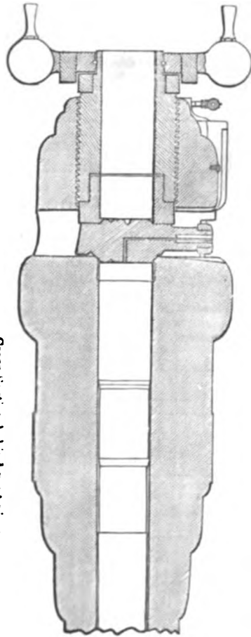
FIG. 18. Section of breech of 110-pounder—scale 1/4 in. to 1 ft.
