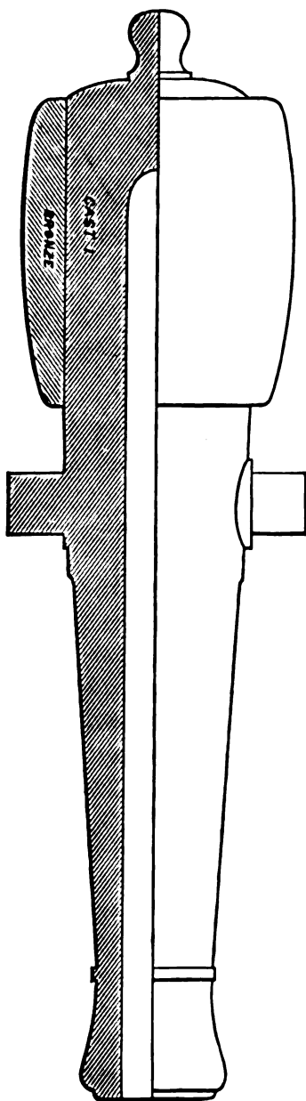
FIG. 59.—Atwater's bronze reinforce. 100-pounder. Scale \frac{1}{8} in. to 1 ft.
