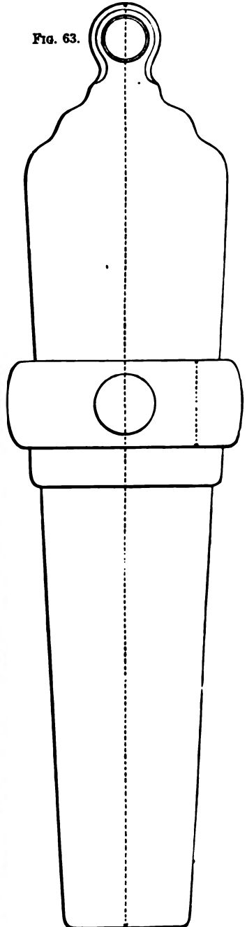
FIGS. 62, 63.—The Horsfall wrought-iron solid-forged 13-in. gun. Scale, 1/2 in to 1 ft.
