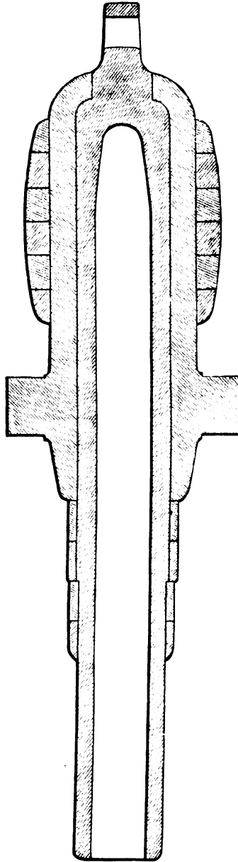
FIG. 32 D. Blakely's steel 8-inch 200-pounder. Scale, ⅓ in. to 1 ft.
