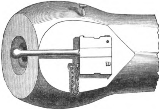
Breech of Krupp 110-pounder.
