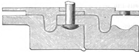
Section of the armor of the Galena (built of wood). \frac{1}{2} size.
