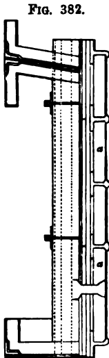
Section of Mr. Scott Russell's target. Scale, \frac{1}{4} in. to 1 ft.
