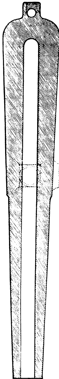
FIG. 71.—Krupp's 9-inch gun for Russia. Scale, \frac{1}{2} in. to 1 ft.
