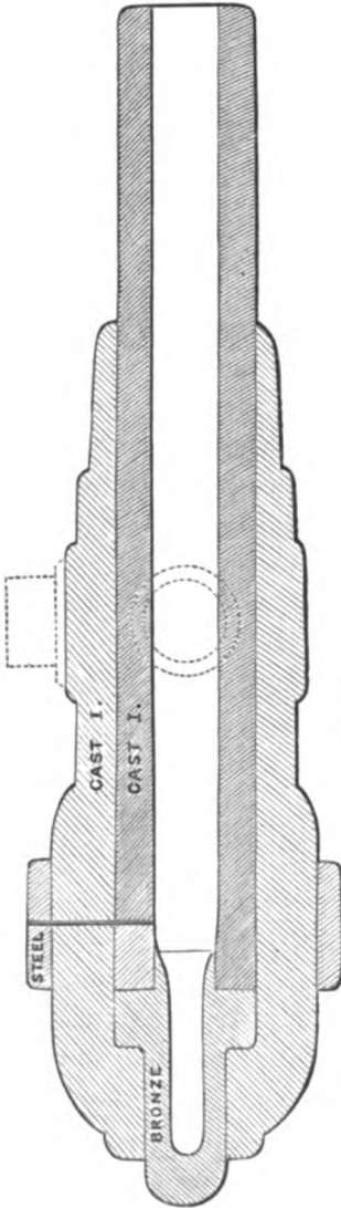
FIG. 34.—Blakely 900-pdr. ( 12\frac{1}{2} in.) rifle, sent to Charleston. Scale, \frac{1}{8} in. to 1 ft. FIG. 35.—Blakely 11-in. rifled gun for Russia, \frac{1}{5} in. to 1 ft.
