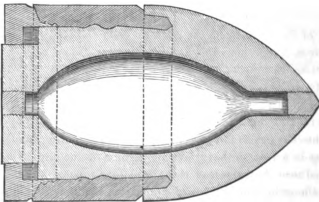
Lynall Thomas's early projectile.
