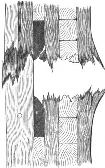
4-in. plate, with wood backing and facing.
