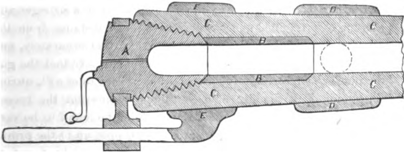
Blakely's breech-loading gun, with internal strengthening tube.
