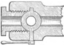
Alger's breech-loader.
