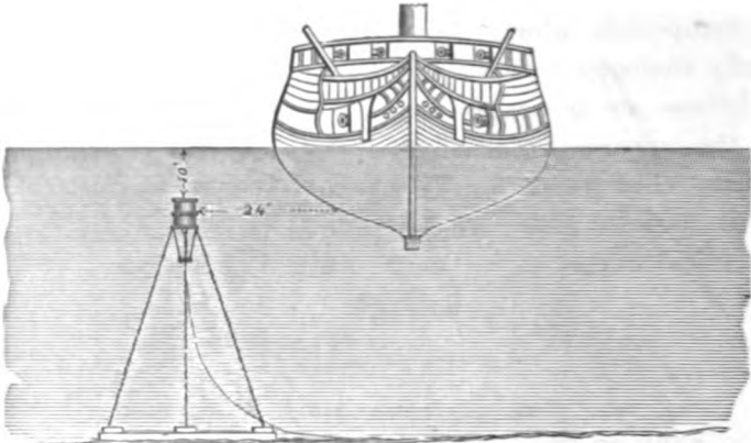
400-lb. gun-cotton torpedo, 24 feet from a ship. Ship blown to pieces.
