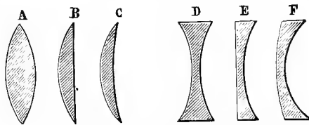
FIG. 375.—DIFFERENT KINDS OF LENSES. (Ganot.)
