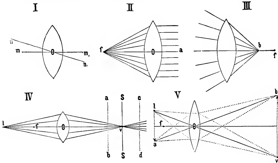
FIG. 374.—ACTION OF A CONVEX LENS ON LIGHT. (Landois.)
