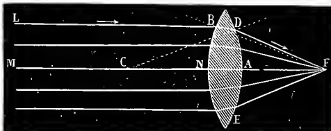
FIG. 372.—DIAGRAM SHOWING REFRACTION BY A DOUBLE CONVEX LENS. ( Ganot. )
