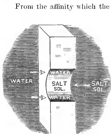
FIG. 39.—DIAGRAM ILLUSTRATING OSMOSIS.
