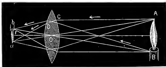
FIG. 378.—DIAGRAM ILLUSTRATING THE FORMATION, BY A DOUBLE CONVEX LENS, OF A SMALLER INVERTED IMAGE. (Ganot.)
