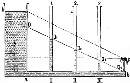
FIG. 214.—ESTIMATION OF PRESSURE OF LIQUID IN A HORIZONTAL OUTFLOW-TUBE CONNECTED WITH A CYLINDRICAL VESSEL FILLED WITH WATER. ( Landois. ) a b, outflow-tube, along which are placed at intervals vertical tubes I, II, and III to estimate the pressure. The line D, D1, D2, D3, D4 indicates the rapidly decreasing pressure.
