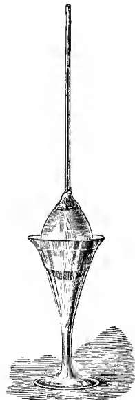
FIG. 40.—EGG PREPARED SO AS TO ILLUSTRATE OSMOTIC ACTION. (Fintl.)
