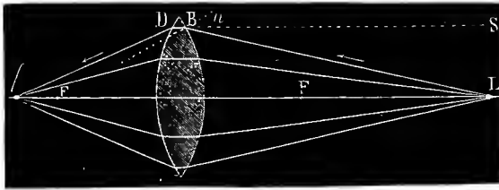
FIG. 373.—DIAGRAM ILLUSTRATING ACTION OF A DOUBLE CONVEX LENS OF HIGH CURVATURE ON DIVERGENT RAYS. ( Ganot .)
