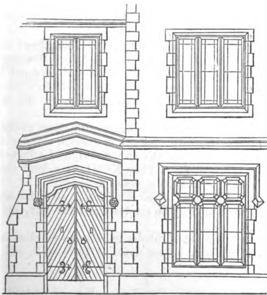
ENLARGED VIEW OF PART OF FRONT ELEVATION IN FIG. 46—SCALE. \frac{1}{4} OF AN INCH TO THE FOOT.
