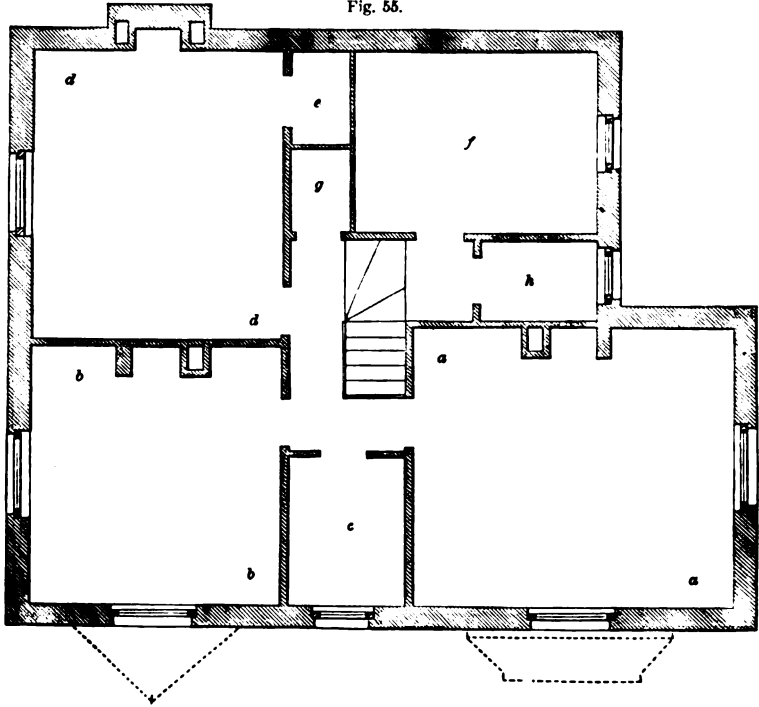
CHAMBER-PLAN OF A SECOND-CLASS FARMHOUSE—SCALE IN FIG. 53.
