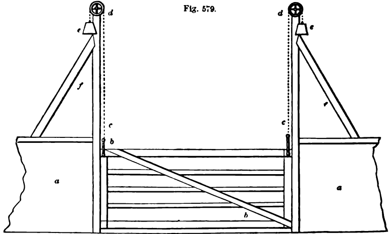
SUSPENDED OR HANGING GATE FOR COURTYARDS—SCALE, \frac{1}{4} INCH TO THE FOOT.
