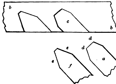
JOINING OF TIMBERS AT OBTUSE ANGLES—SCALE. 1 INCH TO THE FOOT.
