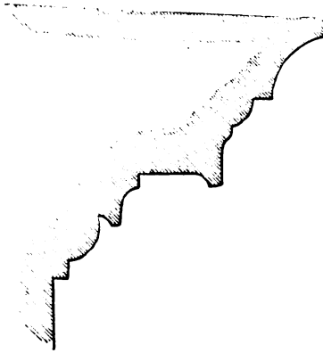
STONE WINDOW CORNICE.—SCALE. 1\frac{1}{4} INCH TO THE FOOT.
