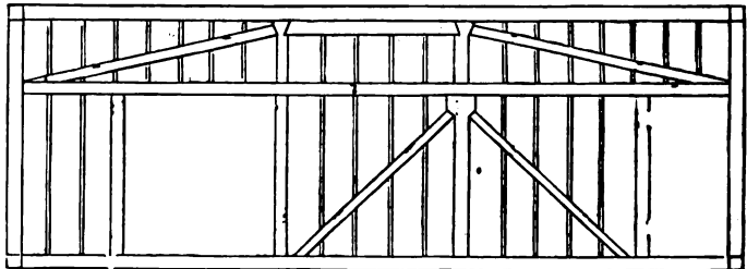
TRUSSED PARTITION—SCALE, \frac{1}{4} INCH TO THE FOOT.
