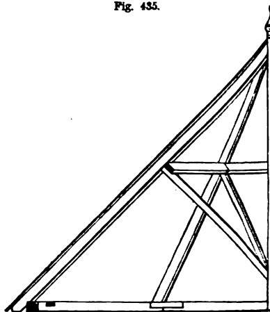
SECTION OF HEXAGONAL ROOF—SCALE, \frac{1}{4} INCH TO THE FOOT.
