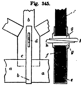
CONNECTION OF KING-POST WITH TIE-BEAM, WITH JOBS AND COLLARS—SCALE, 1/2 INCH TO THE FOOT.
