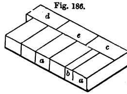
Fig. 186. PLAN OF SECOND COURSE OF 9-INCH WALL —SCALE, ½ INCH TO THE FOOT.
