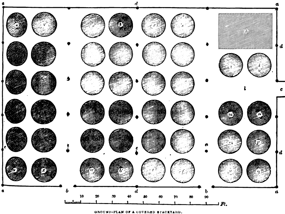
GROUND-PLAN OF A COVERED STACKYARD.
