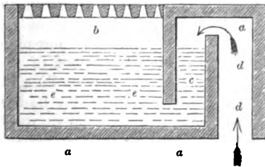
LOWE'S CAST-IRON TRAP.
