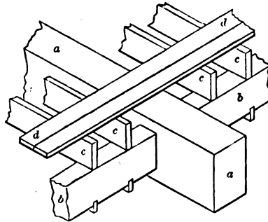
DOUBLE-FRAMED FLOORING—SCALE. 1/4 INCH TO THE FOOT
