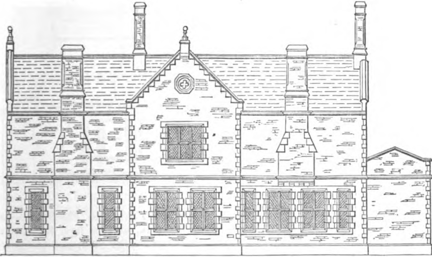
SIDE ELEVATION OF FARMHOUSE, FINISHED TO SHOW STONE-RUBBLE WALLING—SCALE IN PLATE XVIII.
