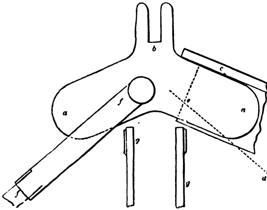
SHOE FOR RAFTERS—SCALE IN FIG. 657.
