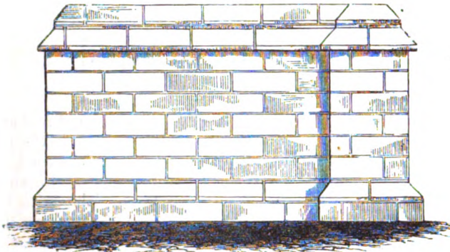
ELEVATION OF DWARF WALL IN ROMAN'S HOLLOW BRICK.
