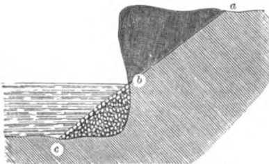
CUTTING OF RIVER-BANKS TO PREVENT WASHING AWAY.
