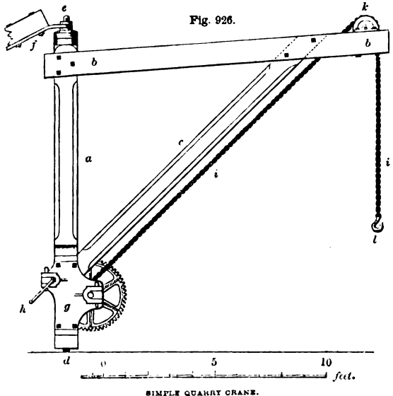
SIMPLE QUARRY CRANE.
