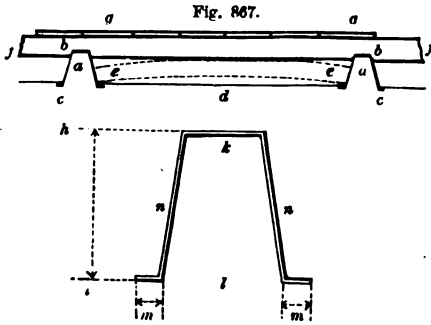
LORE'S SYSTEM OF FIRE-PROOF FLOORING—SCALE, \frac{1}{2} INCH TO THE FOOT.
