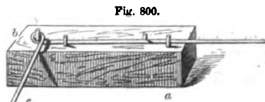
BLOCK FOR MAKING EYES IN WIRES.
