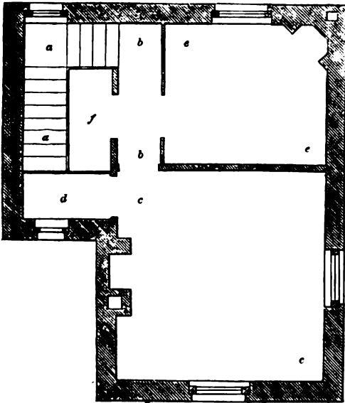
CHAMBER-FLOOR PLAN OF A TWO-STOREYED DETACHED COTTAGE—SCALE IN FIG. 75.
