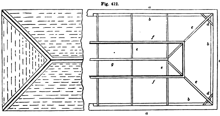
PLAN OF HIPPED-ROOF.
