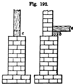
BEARING WALLS.
