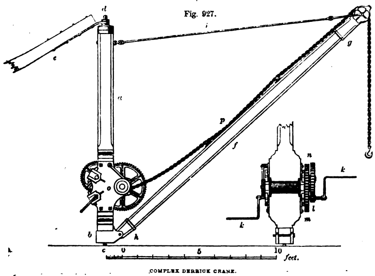
COMPLEX DERRICK CRANE.
