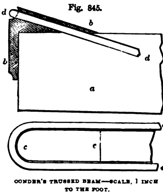
DETAILS OF TRUSSED BEAM—SCALE, 1 INCH TO THE FOOT.
