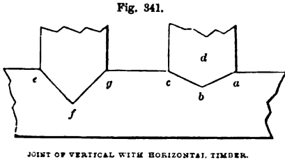
JOINT OF VERTICAL WITH HORIZONTAL TIMBER.
