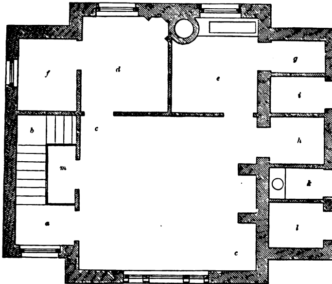
GROUND-PLAN OF A THIRD-CLASS FARMHOUSE—SCALE IN FIG. 67.
