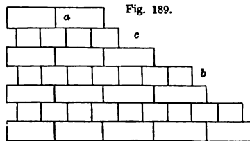
Fig. 189. MODE OF CARRYING UP BRICK COURSES— SCALE, ½ INCH TO THE FOOT.
