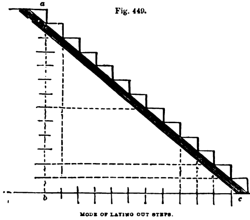
MODE OF LAYING OUT STEPS.
