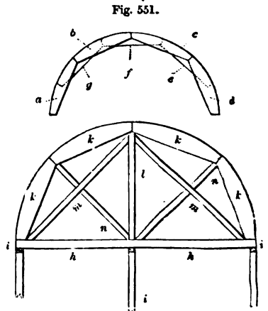
Fig. 551. CENTRES FOR STONE CIRCULAR ARCHES—SCALE, \frac{1}{2} INCH TO THE FOOT.
