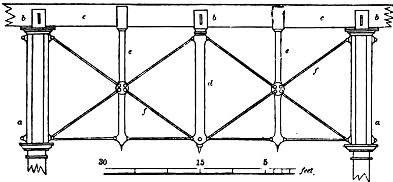
TRUSSED BEAM, OR OPEN GIRDER.
