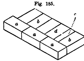
Fig. 185. PLAN OF FIRST COURSE OF 9-INCH WALL IN OLD ENGLISH BOND—SCALE, ½ INCH TO THE FOOT.
