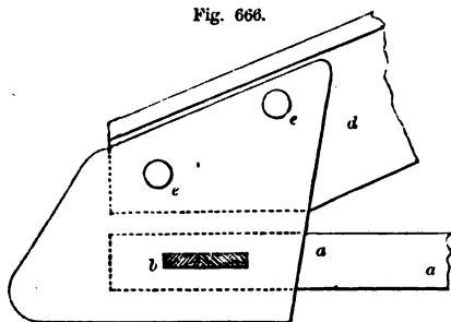
SIDE ELEVATION OF RAFTER-SHOE—SCALE IN FIG. 657.
