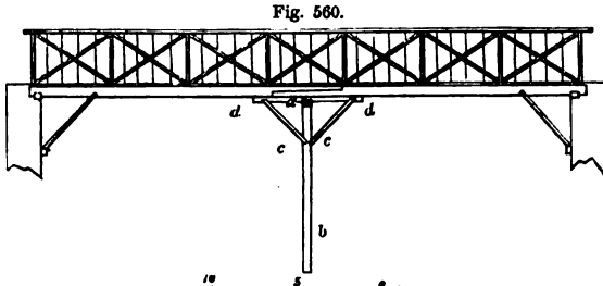
ELEVATION OF BRIDGE OF 32-FOOT SPAN.
