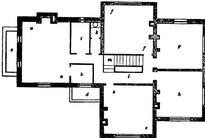
CHAMBER-PLAN OF TUDOR HOUSE—SCALE IN FIG. 41.
