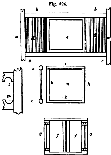
FITTINGS OF HEAD OF STALL WITH FEEDING-PASSAGE—SCALE, 1/4 INCH TO THE FOOT.
