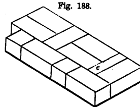
Fig. 188. PLAN OF SECOND COURSE OF 9-INCH WALL, FLEMISH BOND—SCALE, ½ INCH TO THE FOOT
