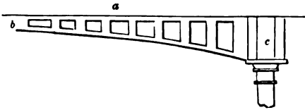
ELEVATION OF CAST-IRON GIRDER FOR SHEDS—SCALE, 1/4 INCH TO THE FOOT.
