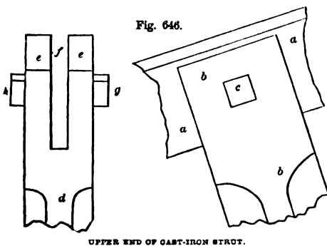
UPPER END OF CAST-IRON STRUT.
