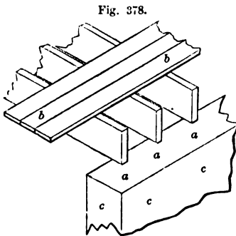
SINGLE FLOORING—SCALE. 1/4 INCH TO THE FOOT.
