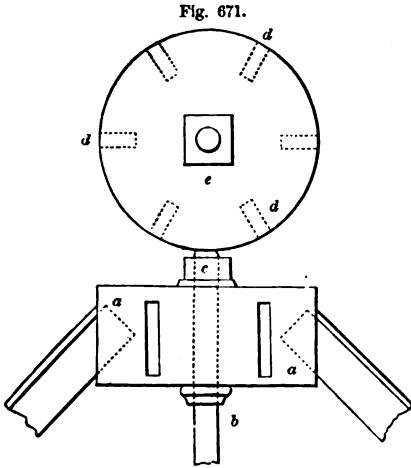
KING-BOLT AND RAFTER-SHOE IN ELEVATION AND PLAN—SCALE, 1 INCH TO THE FOOT.
