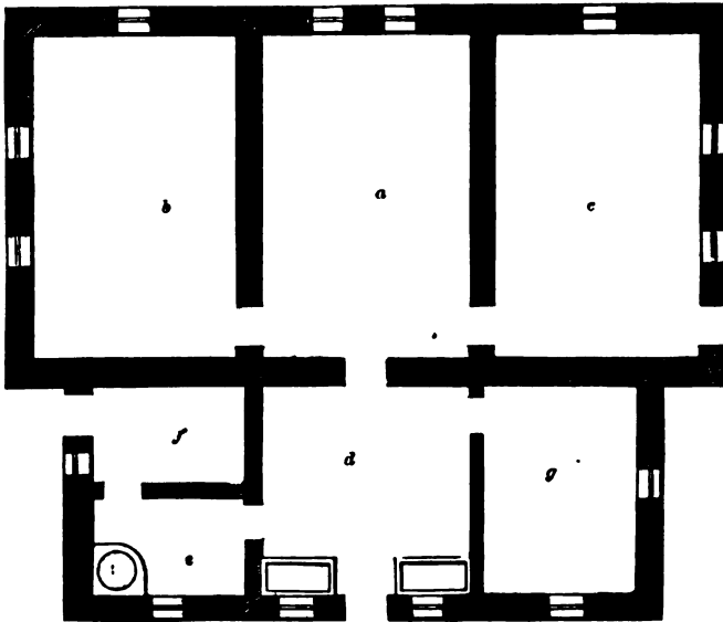
PLAN OF ISOLATED DAIRY—SCALE, \frac{1}{16} INCH TO THE FOOT.
