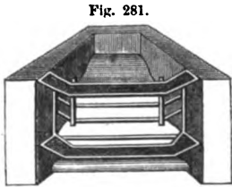
PERSPECTIVE VIEW OF PIERCE'S COIL-TAGE FIRE-LUMP GRATE.
