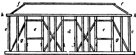
SIDE ELEVATION OF SHED—SCALE, 1/4 INCH TO THE FOOT.
