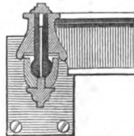
COLLINGS' PATENT SPHERICAL HINGE.
