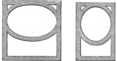
SECTIONS OF DOULTON'S VENTILATING CHIMNEY-TUBE.
