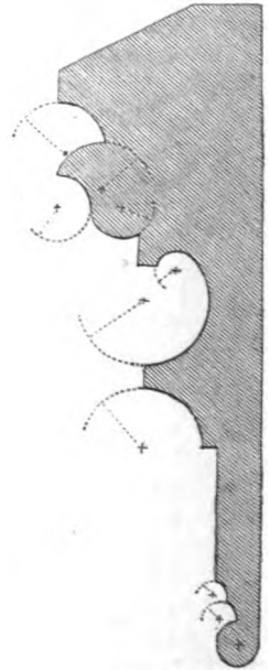
SECTION OF ARCHITRAVES OF HOUSE IN FIG. 23.
