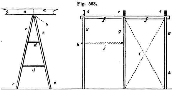
END AND SIDE ELEVATION OF CENTRAL SUPPORT FOR BRIDGE, IN FIG. 560.— SCALE IN FIG. 560.
