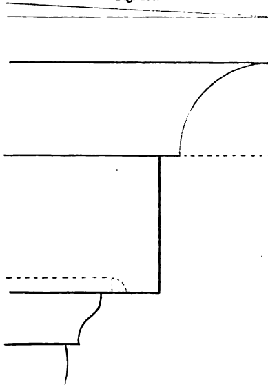
MOULDINGS OF WINDOW CORNICE—SCALE, \frac{1}{2} FULL SIZE.
