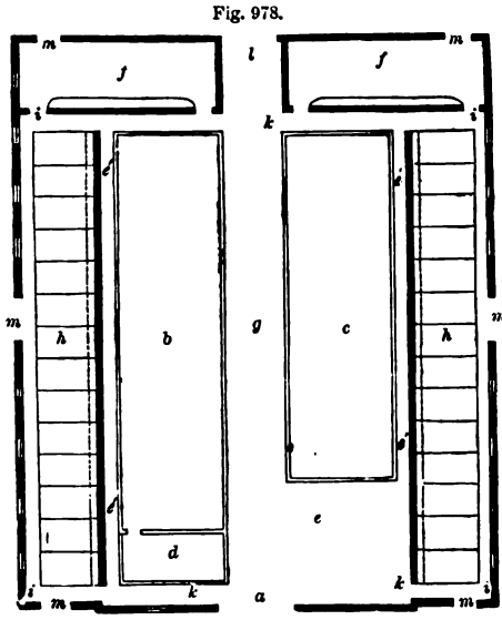
PLAN OF ALLEN'S AMERICAN BARN.
