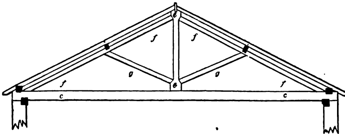
KING-POST ROOF—SCALE IN FIG. 990.
