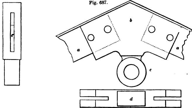
ELEVATIONS AND PLAN OF SHOE FOR UPPER TERMINATION OF RAFTERS—SCALE, 1½ INCH TO THE FOOT.
