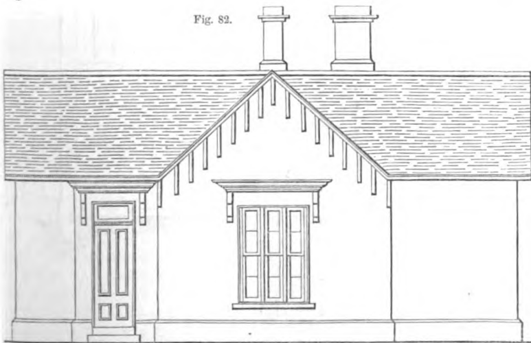
FRONT ELEVATION OF A SINGLE-STOREYED DETACHED COTTAGE—SCALE IN FIG. 81.
