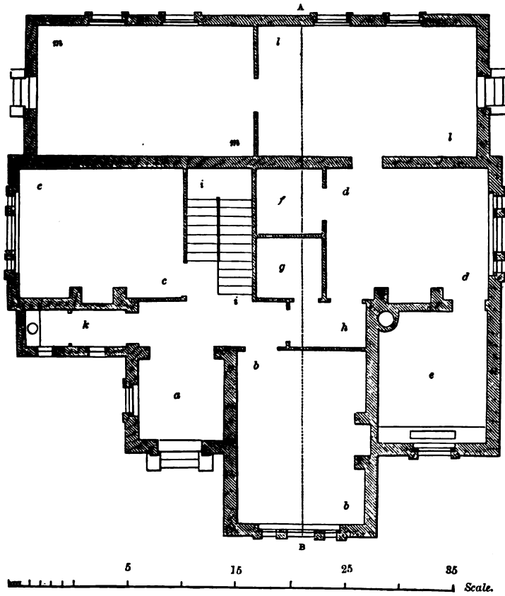
GROUND-PLAN OF FARMHOUSE IN ITALIAN STYLE.
