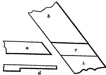
JOINT OF BOTTOM BEAM WITH RAFTER—SCALE, 1/2 INCH TO THE FOOT.
