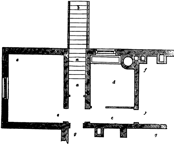
COMPOSITE COTTAGE ADAPTED TO THAT IN FIG. 81.
