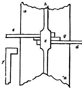
FIXING OF TRUSS-RODS OF CAST-IRON BEAMS—SCALE, \frac{1}{2} INCH TO THE FOOT.
