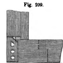
PLAN OF ANGLES FOR DOOR JAMBS IN ALTERNATE COURSES.
