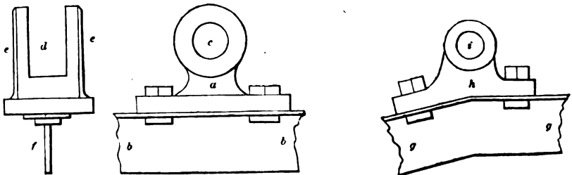
SHOES FOR TIE-RODS—SCALE, 1½ INCH TO THE FOOT.
