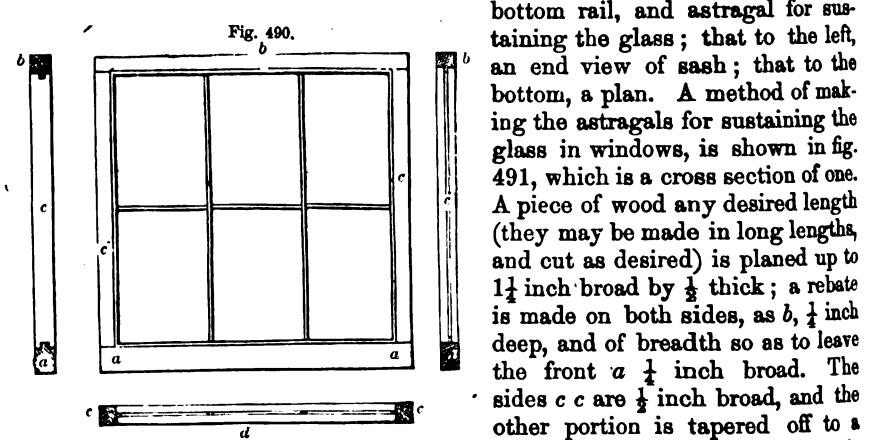
ELEVATION AND SECTION OF SASH-FRAME OF WINDOW.
