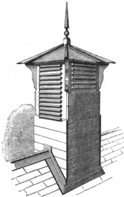
MUIR'S FOUR-POINTS VENTILATOR.
