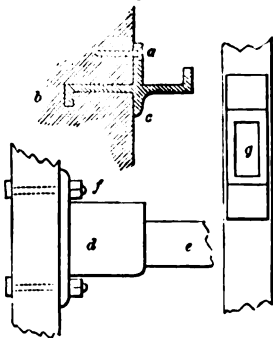
CAST-IRON SHOES FOR "JOISTS," "WALL-PLATES"—SCALE, \frac{1}{2} INCH TO THE FOOT.
