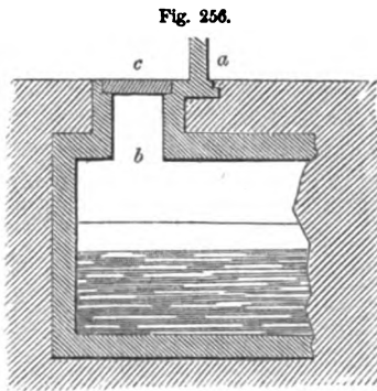
FLEMISH LIQUID-MANURE TANK.
