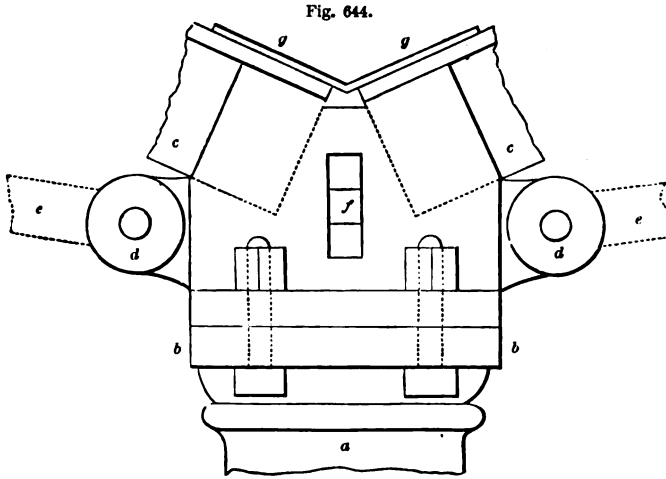
RAFTER-SHOES FOR ROOF IN FIG. 613—SCALE IN FIG. 637.
