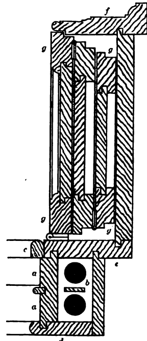
SASH-WINDOW.
