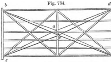
IRON FIELD-GATE ON THE TENSION PRINCIPLE.
