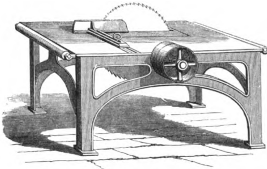
PERSPECTIVE VIEW OF TURNER'S IRON BENCH FOR CIRCULAR SAW.
