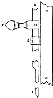
LOWER BOLT OF WINDOW-FASTENING.
