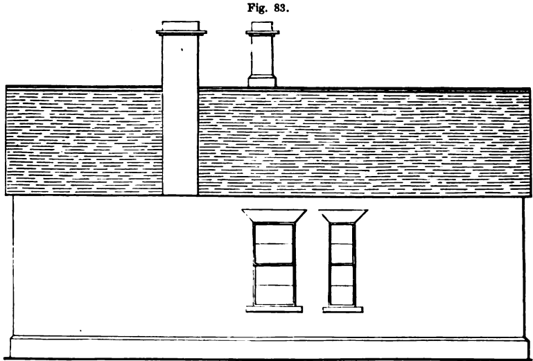
BACK ELEVATION OF A SINGLE-STOREYED DETACHED COTTAGE—SCALE IN FIG. 81.
