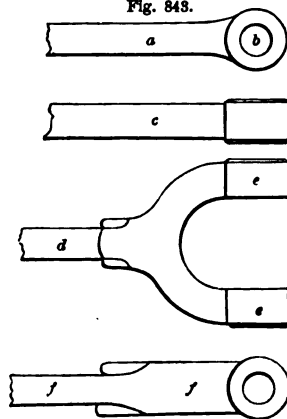
DETAILS OF TRUSS RODS—SCALE, 2 INCHES TO THE FOOT.
