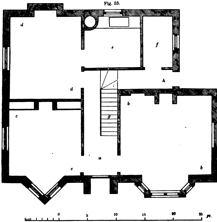
GROUND-PLAN OF A SECOND-CLASS FARMHOUSE.
