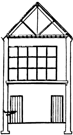
VERTICAL SECTION OF MILK-HOUSE AND CHEESE-ROOM, FIG. 23 AND 24.
