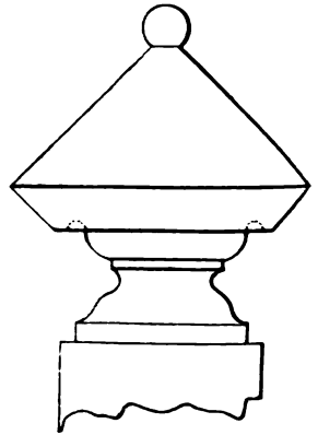
FINIAL—SCALE, \frac{1}{2} FULL SIZE.
