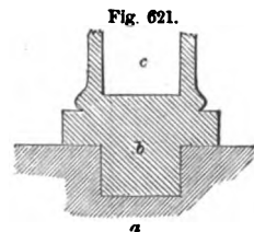
FIXING OF CAST-IRON PILLAR— SCALE, 1 INCH TO THE FOOT.
