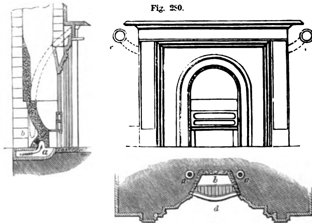
PLAN, ELEVATION, AND SECTION OF PIERCE'S FIRE-LUMP SLOVE-GRATE.
