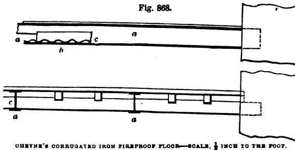
CHEYNE'S CORRUGATED IRON FIRE-PROOF FLOOR—SCALE, \frac{1}{2} INCH TO THE FOOT.
