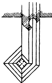
DRIP-STONE.
