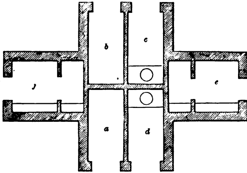
PLAN OF OUTHOUSES FOR DOUBLE-DETACHED COTTAGES—SCALE IN FIG. 133.
