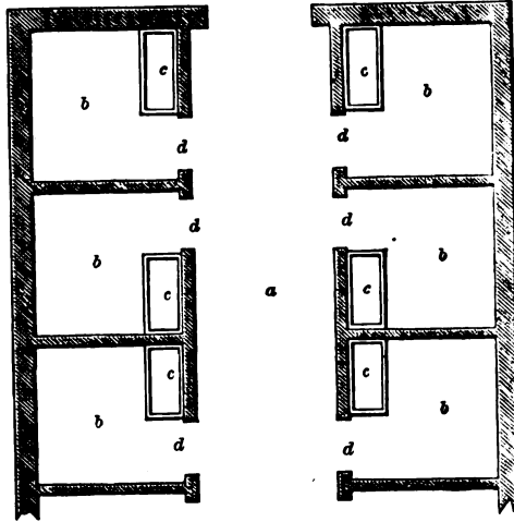
PLAN OF DETACHED PIGSTY—SCALE IN FIG. 944.
