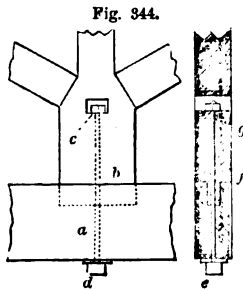
CONNECTION OF KING-POST WITH TIE-BEAM, WITH BOLT—SCALE, 1/2 INCH TO THE FOOT.
