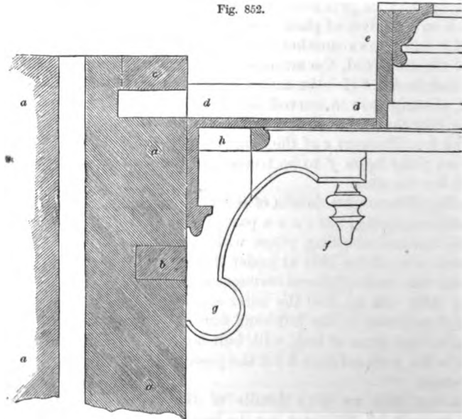
DETAILS OF CORNICE OF FARMHOUSE IN FIG. 56—SCALE, 1 INCH TO THE FOOT.
