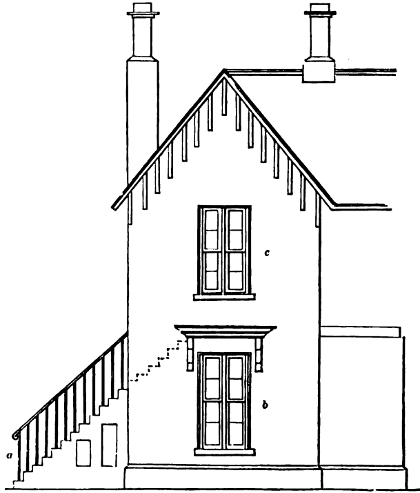
END ELEVATION OF COMPOSITE COTTAGE IN FIGS. 61 AND 121.
