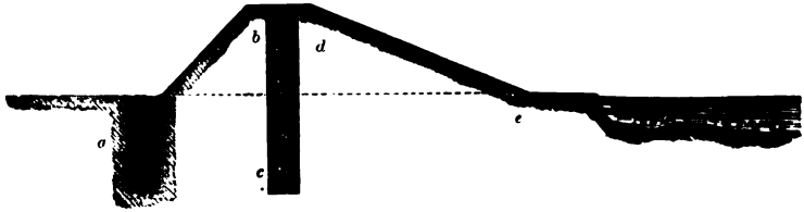
THE MOST EFFECTUAL EMBANKMENT ON A GRAVELLY BOTTOM.
