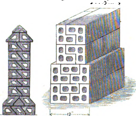
SECTIONS OF 12-INCH HOLLOW WALL.
