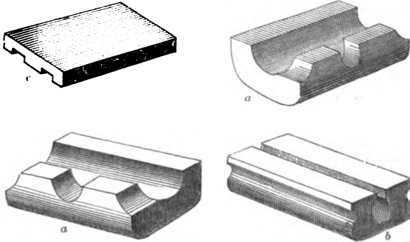
PERSPECTIVE VIEW OF FORBES'S DRAINAGE PAVEMENT-BRICKS.
