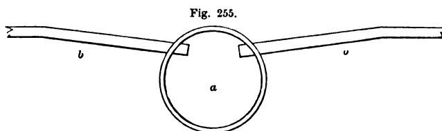
SECTION OF CROSS-CULVERT AND UNDER-DRAINS
