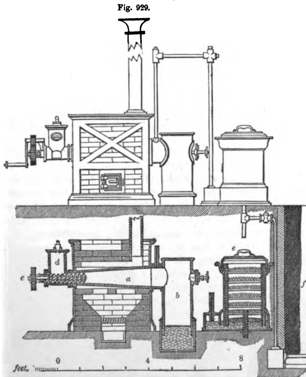
PORTER'S GAS APPARATUS FOR FARM USE.
