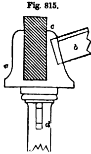
Fig. 815. TERMINATION OF CENTRAL UPRIGHT—SCALE, 1 INCH TO THE FOOT.
