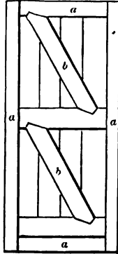
FRAMED AND BRACED DOOR.
