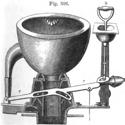
SECTION OF JENNINGS'S WATER-CLOSET—TUBE OPEN.
