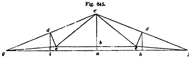
SKELETON OF IRON TRUSS FOR SPAN OF 25 FEET—SCALE IN FIG. 637.
