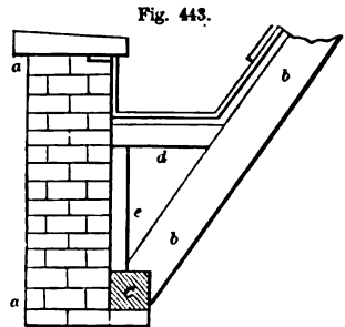
BRIDGED GUTTER—SCALE, 1/2 INCH TO THE FOOT.
