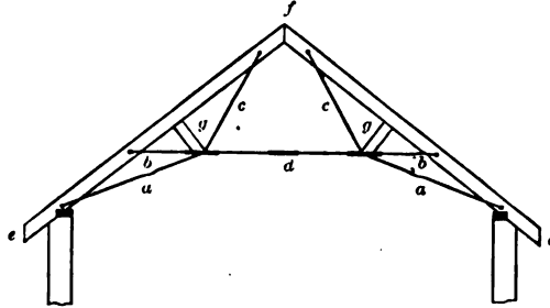
Fig. 818. ROOF TRUSS OF OCTAGONAL SHED—SCALE, 1/4 INCH TO THE FOOT.
