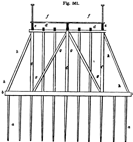
ELEVATION OF MID-PIER FOR BRIDGE IN FIG. 560.
