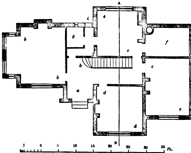
GROUND-PLAN OF FARMHOUSE IN TUDOR-GOTHIC STYLE.
