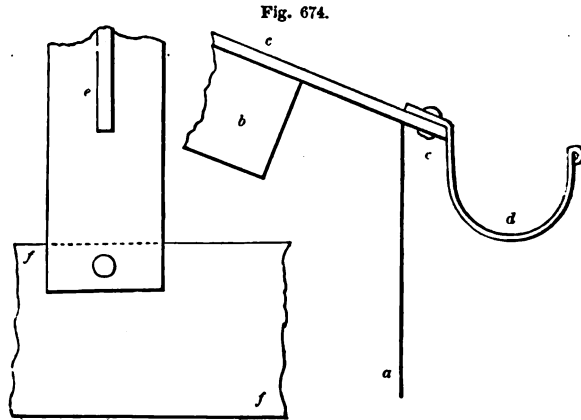
GUTTER OF IRON ROOF—SCALE IN FIG. 657.
