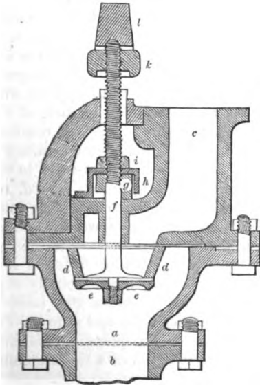
WHEATON AND SMITH'S HYDRANT
