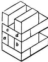
DEARN'S HOLLOW 9-INCH WALL—SCALE, \frac{1}{4} INCH TO THE FOOT.
