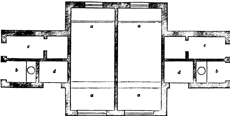
SECOND ALTERNATIVE PLAN OF OUTHOUSES FOR DOUBLE COTTAGES—SCALE IN FIG. 133.
