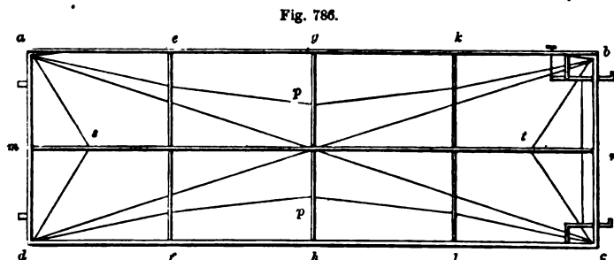
ELEMENTS OF THE BRACING OF A WIRE FIELD-GATE.
