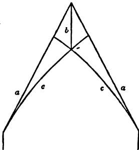
SKELTON OF TRUSS FOR A LAMINATED RIB ROOF, 32-FOOT SPAN.
