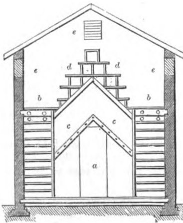
SECTION OF AMERICAN POULTRY-HOUSE—SCALE IN FIG. 986.
