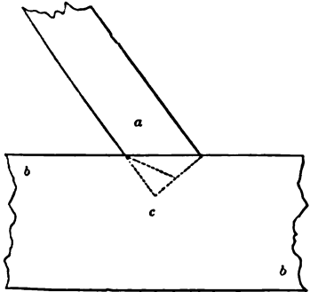
JOINT OF RAFTER WITH TIE-BEAM—SCALE, 1 INCH TO THE FOOT.
