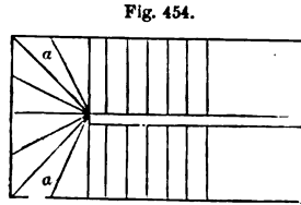
PLAN OF STAIRCASE WITH RETURN.
