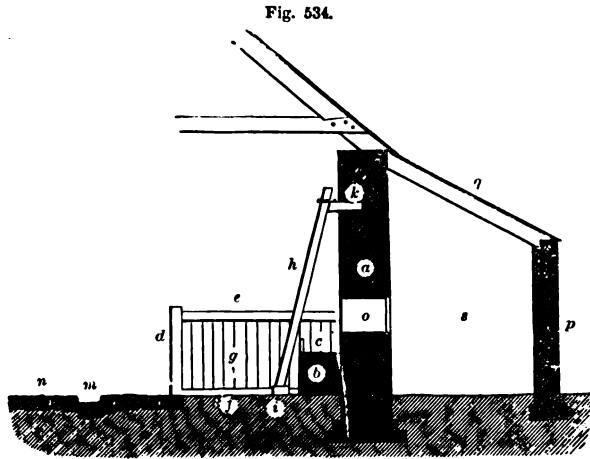
BYRE TRAVIS, MANGER, STAKE, AND TURNIP-STORE.
