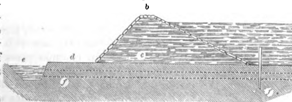
PROTECTION BY SEA EMBANKMENT.
