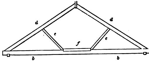
TIE-BEAM ROOF.
