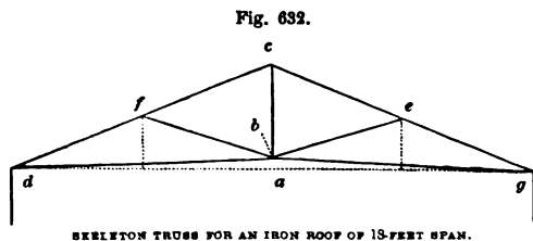
SKELTON TRUSS FOR AN IRON ROOF OF 18-FOOT SPAN.
