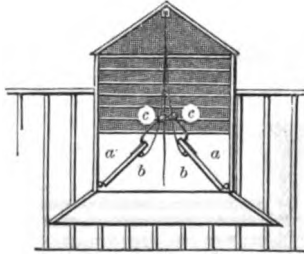
SECTION OF FERGUSON'S VENTILATOR.
