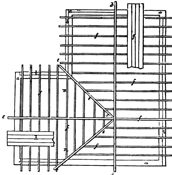
TIMBER OF A ROOF MEETING AT RIGHT ANGLES (PLAN)—SCALE, \frac{1}{2} INCH TO THE FOOT.
