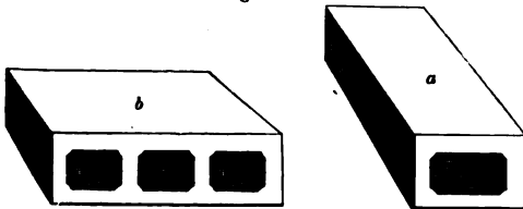
NORTON AND BORRIE'S HOLLOW BRICKS.
