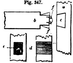
DOVETAIL JOINT—SCALE \frac{1}{2} INCH TO THE FOOT.
