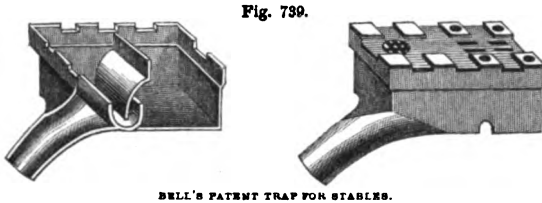
BELL'S PATENT TRAP FOR STABLES.
