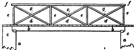
BEAM-BRIDGE FOR 15-FOOT SPAN—SCALE, ¼ INCH TO THE FOOT.
