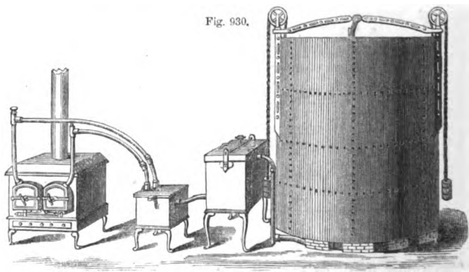
PERSPECTIVE VIEW OF MESSRS BRIDGES AND ADCHRY'S GAS-MAKING APPARATUS.
