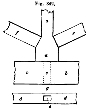
CONNECTION OF KING-POST WITH TIE-BEAM —SCALE, 1/2 INCH TO THE FOOT.
