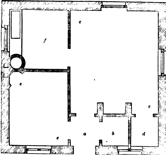
GROUND-PLAN OF A SINGLE-STORYED DETACHED COTTAGE.
