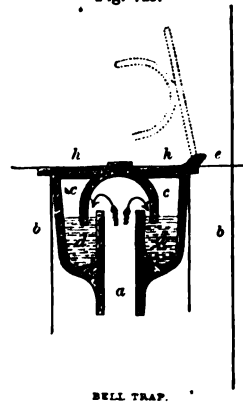
BELL TRAP.
