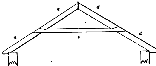
COLLAR-ROOF.
