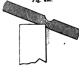
GUTTERS AT ENDS OF RAFTERS.
