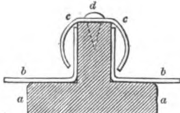
ATTACHING SHEETS OF ZINC TO WROUGHT-IRON RAFTERS.
