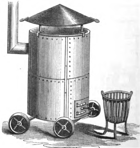
PERSPECTIVE VIEW OF ASPHALT CALDRON AND GRATE.
