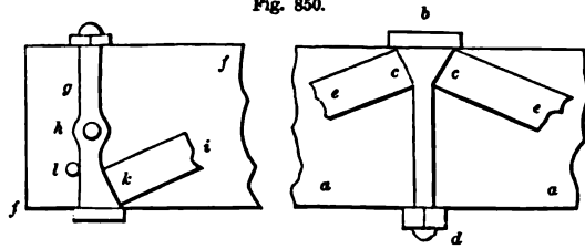
DETAILS OF KING-POST TRUSSED BEAM—SCALE, \frac{3}{4} INCH TO THE FOOT.
