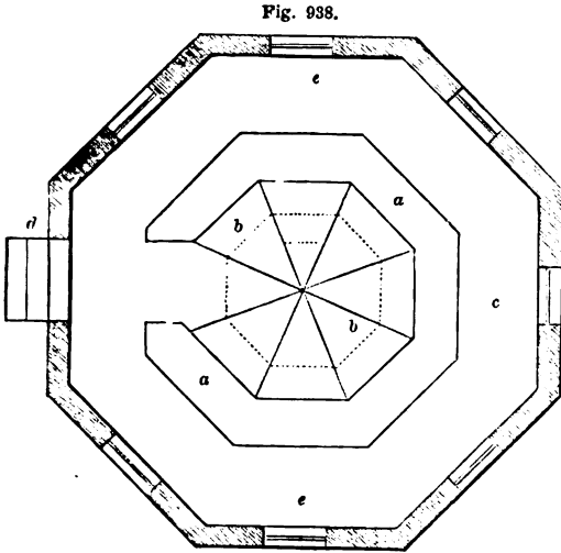
PLAN OF POULTRY-HOUSE—SCALE. \frac{1}{4} INCH TO THE FOOT.
