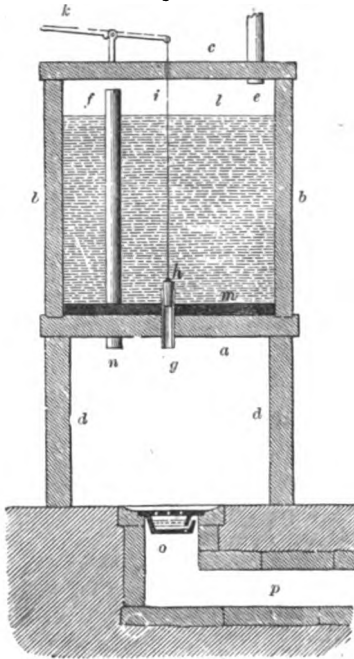
A RAIN-WATER CISTERNS.
