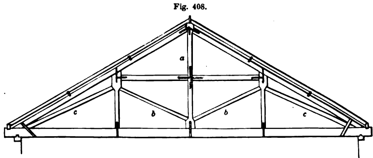
TRUSS FOR A 30-FOOT SPAN—SCALE, \frac{1}{4} INCH TO THE FOOT.
