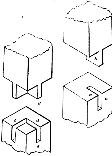
JOINT TO RESIST VERTICAL COMPRESSION— SCALE, 1 INCH TO THE FOOT.
