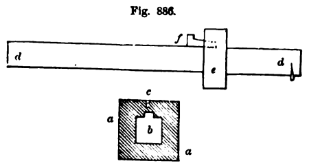
ELEVATION AND SECTION OF GAUGE—SCALE, \frac{1}{2} INCH TO THE INCH
