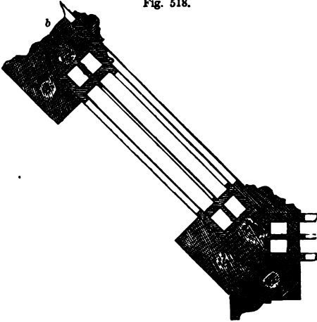
PLAN OF BAY WINDOW, CHAMBER FLOOR, IN FIG. 68—SCALE IN FIG. 516.
