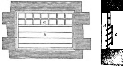
ORDINARY WINDOW AND SECTION OF SHUTTERS.
