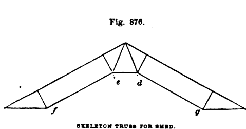
SKELETON TRUSS FOR SHED.
