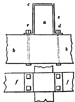
IRON SADDLE FOR JOINING BEAMS CROSSING AT RIGHT ANGLES—SCALE, \frac{1}{2} INCH TO THE FOOT.
