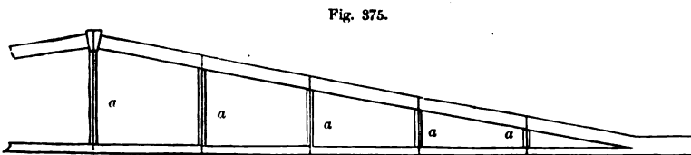
BOW-AND-STRING RAFTER—SCALE, 1/4 INCH TO THE FOOT.
