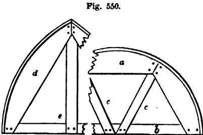
Fig. 550. CENTERINGS FOR GOTHIC AND SEMICIRCULAR ARCHES— SCALE, \frac{1}{2} INCH TO THE FOOT.
