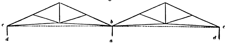
SKELETON TRUSS OF DOUBLE-SPAN ROOF—SCALE IN FIG. 637.
