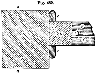
PART SECTION OF SASH-FRAME.
