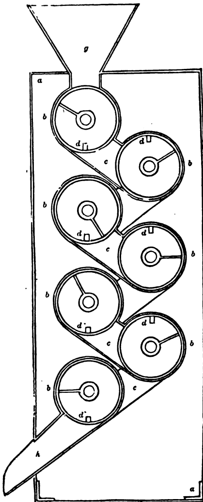
VERTICAL SECTION OF ARCHIMEDEAN SCREW CONVEYOR.
