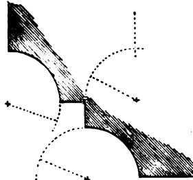
MOULDINGS OF JAMB AND MULLION OF DOORWAY—SCALE, \frac{1}{2} FULL SIZE.
