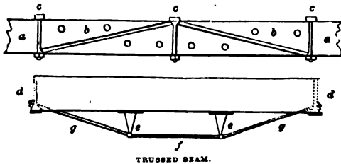
TRUSSED BEAM.
