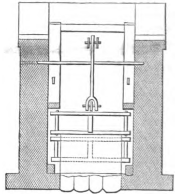
TRANSVERSE SECTION OF SELF-ACTING SLUICE.
