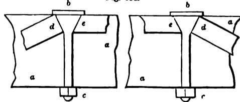
DETAILS OF QUEEN-POST TRUSSED BEAM—SCALE, \frac{3}{4} INCH TO THE FOOT.
