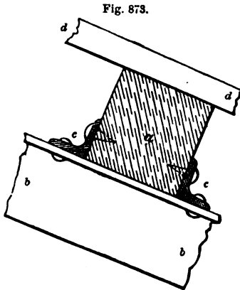
FIG. 873. JUNCTION OF WOODEN PURLINS WITH IRON RAFTERS—SCALE IN FIG. 857.
