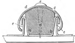
FIXING SHEETS OF ZINC TO WOODROLLS
