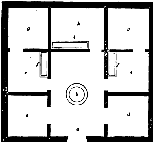
PLAN OF DETACHED PIGGERY—SCALE, 1/2 INCH TO THE FOOT.
