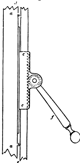
FASTENING FOR FRENCH OR CASEANT WINDOWS—SIDE VIEW.
