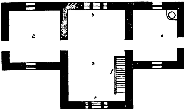
PLAN OF ISOLATED DAIRY—SCALE, \frac{1}{16} INCH TO THE FOOT.
