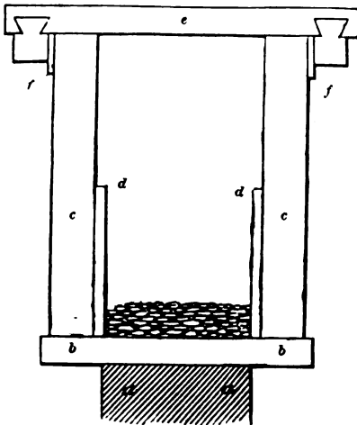
SECTION SHOWING ARRANGEMENT OF PARTS OF MOULD.
