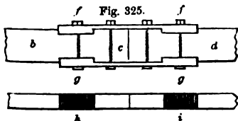
Fig. 325. JOINING TIMBERS IN THE DIRECTION OF THEIR LENGTH—SCALE, \frac{1}{4} INCH TO THE FOOT.
