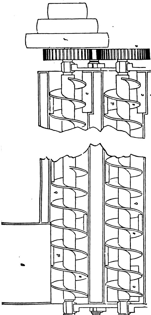
PLAN OF ARCHIMEDEAN SCREW CONVEYOR.
