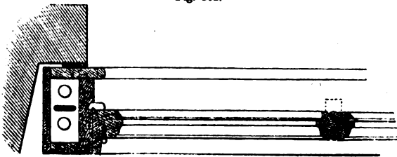
PART HORIZONTAL PLAN OF OAK-HALL WINDOW.
