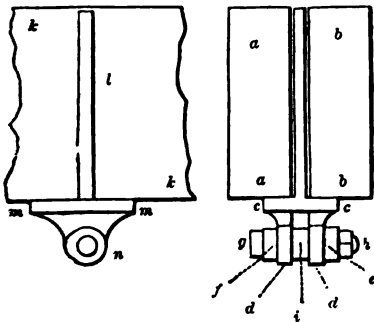
CROSS SECTION AND PART ELEVATION OF FLITCHES OF TRUSSED BEAM IN FIG. 841—SCALE, 1 INCH TO THE FOOT.
