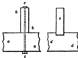
JOINING OF BEAMS CROSSING EACH OTHER AT RIGHT ANGLES—SCALE. 1/2 INCH TO THE FOOT.
