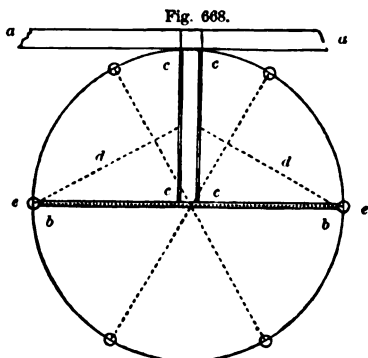
Fig. 668. PLAN OF HORSE-WALK FOR THRASHING-MILL—SCALE, 1/8 INCH TO THE FOOT.
