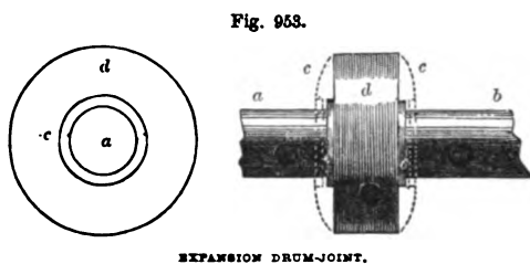
EXPANSION DRUM-JOINT.
