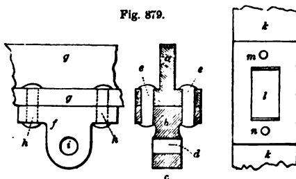
RIVETING STRUTS TO RAFTERS.
