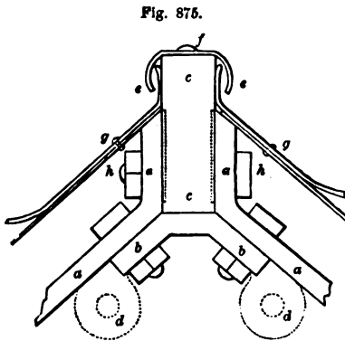
FIG. 875. JOINING RAFTERS OF TRUSS FOR ZINC COVERING.
