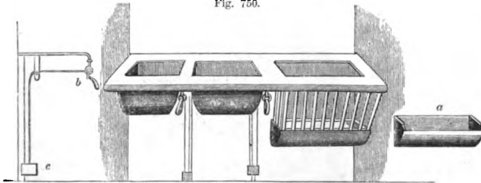
PATENT MANGER, WATER-TROUGH, AND WROUGHT-IRON RACK.
