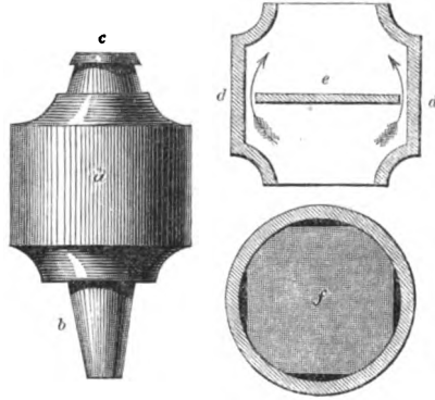
GAS REGULATOR.
