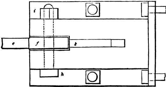
SHOE IN PLAN AND ELEVATION FOR SECURING FEET OF RAFTERS—SCALE IN FIG. 657.
