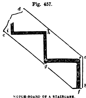
NOTCH-BOARD OF A STAIRCASE.
