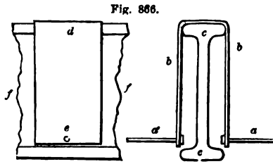
DETAILS OF BEAM—SCALE, 2 INCHES TO THE FOOT.
