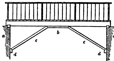
BRIDGE FOR 14-FOOT SPAN, WITH STRUTS—SCALE, ¼ INCH TO THE FOOT.
