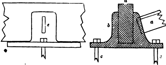
ELEVATION AND SECTION OF SHOE—SCALE, 1 INCH TO THE FOOT.
