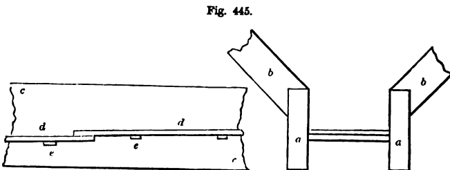
SECTION AND ELEVATION OF VALLEY-GUTTER—SCALE, 1/2 INCH TO THE FOOT.
