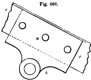
JUNCTION OF BENTS WITH RAFTERS—SCALE, 1½ INCH TO THE FOOT.
