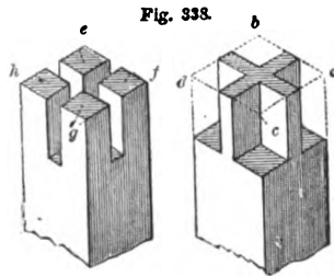
JOINT TO RESIST VERTICAL COMPRESSION— SCALE, 1 INCH TO THE FOOT.
