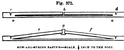
BOW-AND-STRING RAFTER—SCALE, 1/4 INCH TO THE FOOT.
