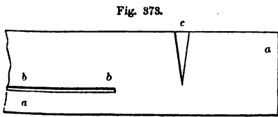
END OF BOW-AND-STRING RAFTER—SCALE, 1/2 INCH TO THE FOOT.
