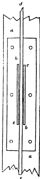
FASTENING OF FRENCH WINDOW—FRONT VIEW.
