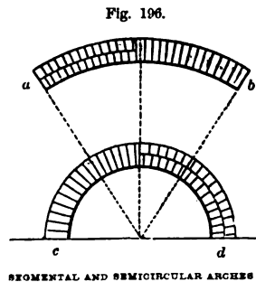
SEGMENTAL AND SEMICIRCULAR ARCHES
