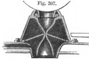
JENNINGS'S WATER-CLOSET—TUBE CLOSED.
