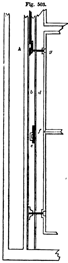
PART ELEVATION OF SHAW'S PATENT WINDOW.
