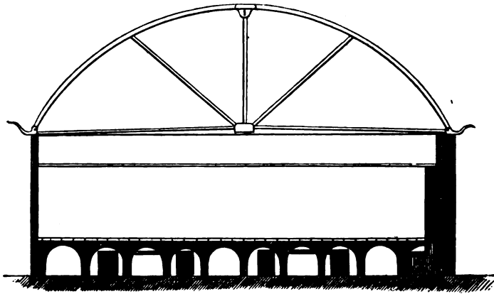
VERTICAL SECTION OF HANDS' DRYING SHEDS.
