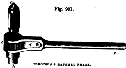
IBBOTSON'S RATCHET BRACE.
