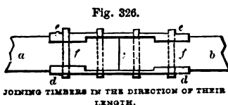
Fig. 326. JOINING TIMBERS IN THE DIRECTION OF THEIR LENGTH.
