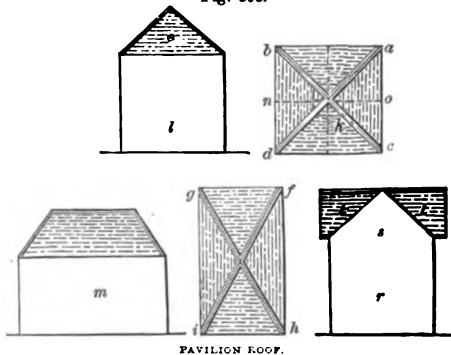
PAVILION ROOF.
