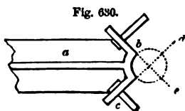
JUNCTION OF FOUR GIRDEES ON CAP OF COLUMN—SCALE, \frac{1}{2} INCH TO THE FOOT.
