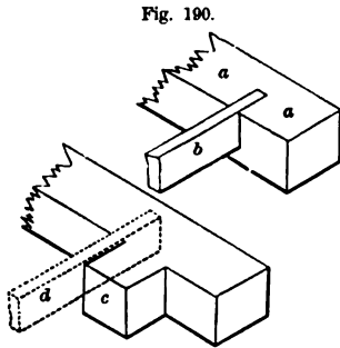
GOOD AND BAD METHODS OF SETTING FLOORING-JOISTS—SCALE, \frac{1}{4} INCH TO THE FOOT.
