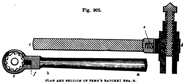
PLAN AND SECTION OF FENN'S RATCHET BRACE.
