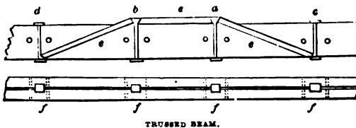
TRUSSED BEAM.
