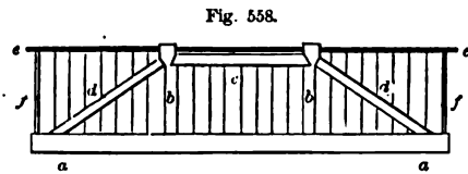
QUEEN-POST TRUSS FOR BRIDGE—SCALE, \frac{1}{4} INCH TO THE FOOT.
