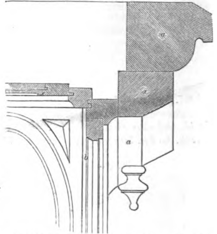
PART VERTICAL SECTION OF BAY WINDOW—SCALE, 1 INCH TO THE FOOT.
