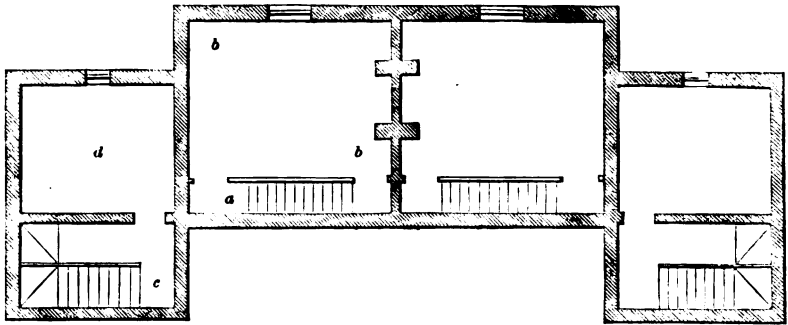
FLOOR-PLAN OF COTTAGES IN FIG. 108.
