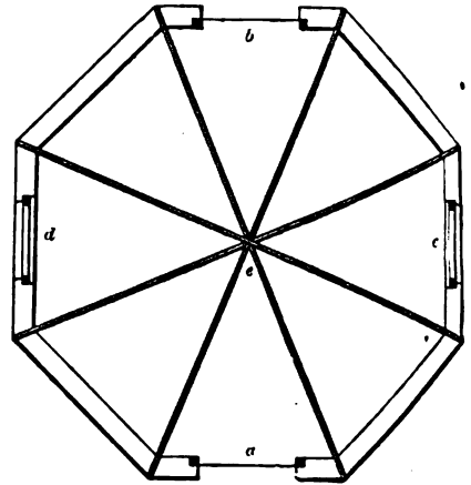
Fig. 817. PLAN OF OCTAGONAL SHED—SCALE, 1/4 INCH TO THE FOOT.
