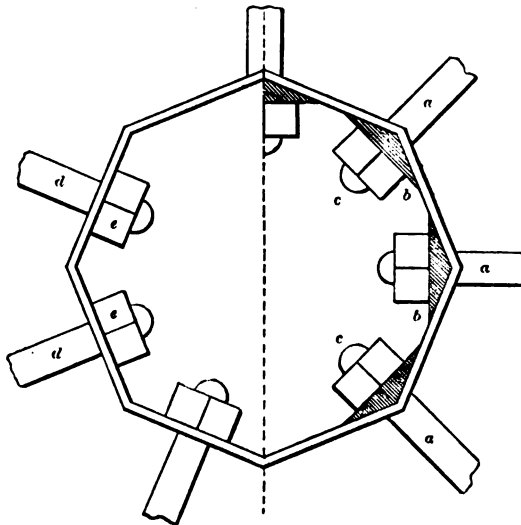
Fig. 819. PLAN OF CENTRAL RING d , FIG. 818—SCALE, 1/4 INCH TO THE FOOT.
