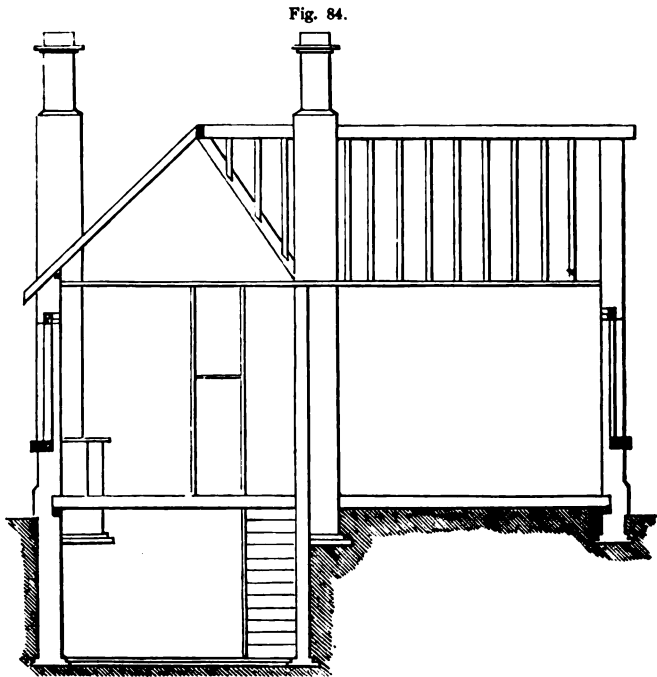
VERTICAL SECTION OF A SINGLE-STOREYED DETACHED COTTAGE—SCALE IN FIG. 81.
