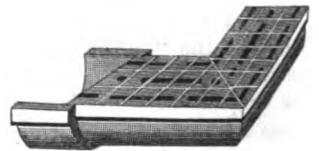
CORNER JUNCTION OF BARION'S STABLE-DRAINS
