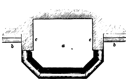
PLAN OF FIRECLAY HEARTH
