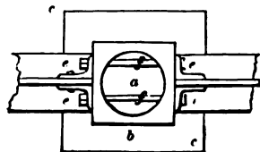
JUNCTION OF WROUGHT-IRON BEAMS IN CAP OF COLUMN—SCALE, 1 INCH TO THE FOOT.
