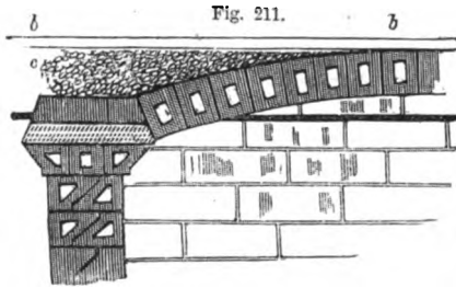
FIRE-PROOF FLOORS AND CEILINGS IN ROBERTS' HOLLOW BRICKS.
