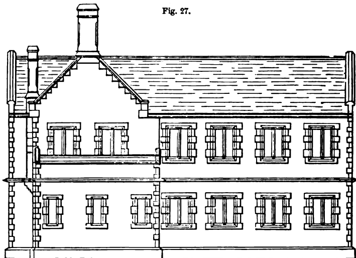
BACK ELEVATION OF FARMHOUSE—SCALE IN PLATE XVIII.
