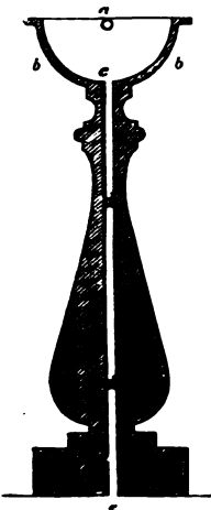
SECTION OF WASH-HAND PORCELAIN BASIN.
