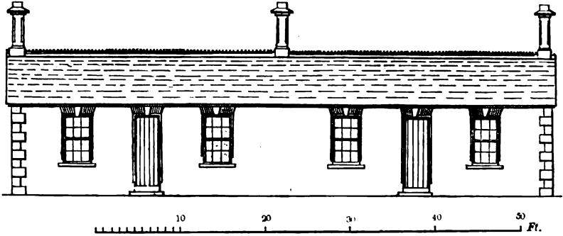
FRONT ELEVATION OF SINGLE-STORYED DOUBLE-DETACHED COTTAGES.
