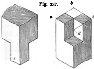
JOINT TO RESIST VERTICAL COMPRESSION— SCALE, 1 INCH TO THE FOOT.
