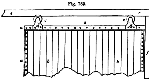
TOP OF SLIDING-GATE OF CORRUGATED IRON—SCALE, \frac{1}{2} INCH TO THE FOOT.
