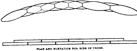
PLAN AND ELEVATION FOR RIBS OF TRUSS.
