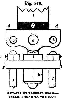
CONDER'S TRUSSED BEAM—SCALE, 1 INCH TO THE FOOT.
