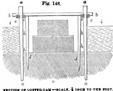
SECTION OF COFFER-DAM—SCALE \frac{1}{2} INCH TO THE FOOT.
