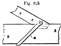
IRON STRAP FOR FOOT OF RAFTER AND TIE-BEAM—SCALE, \frac{1}{2} INCH TO THE FOOT.
