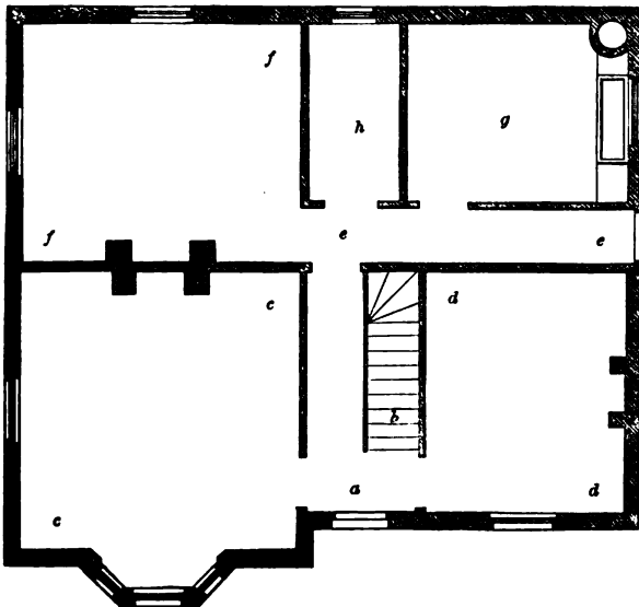
5 10 15 20 Ft. GROUND-PLAN OF A THIRD-CLASS FARMHOUSE.
