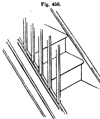
CARRIAGE-BOARD OF A STAIRCASE.
