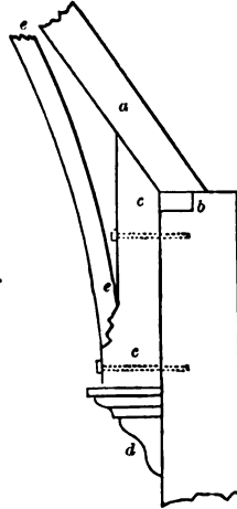
DETAIL OF PART OF ROOF-TRUSS —SCALE. 1/2 INCH TO THE FOOT.
