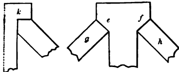
JOINTS OF STRUTS AND RAFTERS WITH HEADS AND FEET OF KING-POSTS AND QUEEN-POSTS—SCALE, 1/2 INCH TO THE FOOT.
