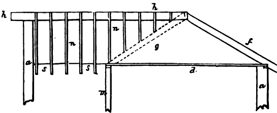
ELEVATION OF ROOF IN FIG. 413—SCALE, \frac{1}{2} INCH TO THE FOOT.
