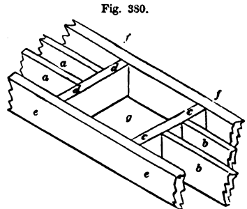
TRIMMING-JOISTS—SCALE 1/4 INCH TO THE FOOT.
