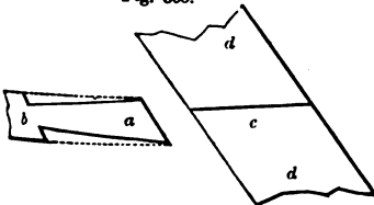
JOINT OF COLLAR-BEAM WITH RAFTER—SCALE, 1/2 INCH TO THE FOOT.
