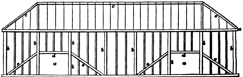
SIDE ELEVATION OF TIMBERS OF SHELTER-SHED.
