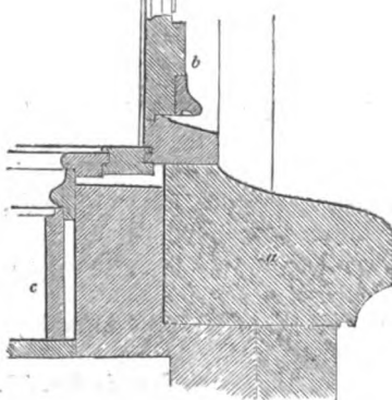
PART SECTION OF BASE OF BAY WINDOW—SCALE, 1 INCH TO THE FOOT.
