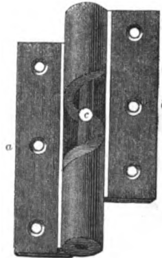
PATENT HINGES FOR SELF-SHUTTING DOORS.
