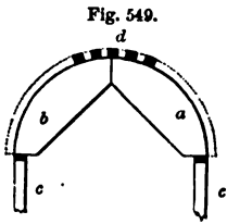
Fig. 549. CENTRE FOR A DOOR ARCH— SCALE, \frac{1}{2} INCH TO THE FOOT.
