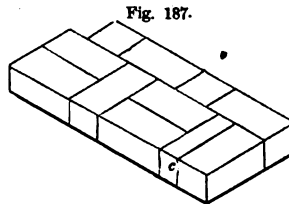
Fig. 187. PLAN OF FIRST COURSE OF 9-INCH WALL IN FLEMISH BOND—SCALE, ½ INCH TO THE FOOT
