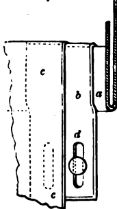
JOINING SHEETS OF ZINC FROM WALL-PLATE TO RIDGE.
