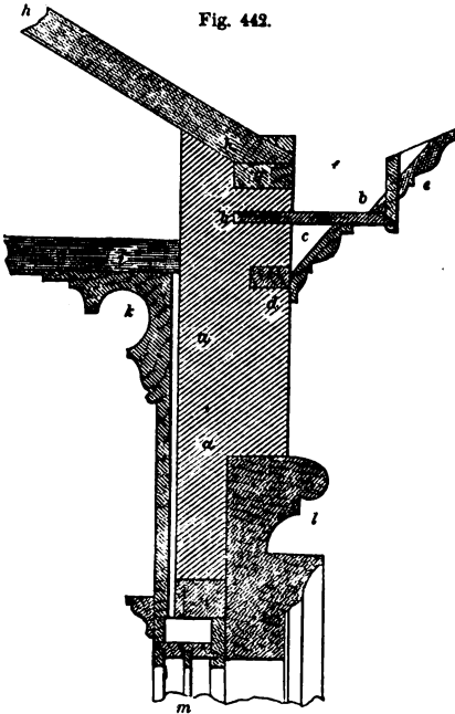
SECTION OF WALL SHOWING GUTTER WITH CANTALIVER—SCALE, 1/2 INCH TO THE FOOT.
