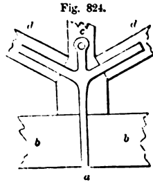
IRON STRAP FOR FOOT OF KING-POST, STRUTS, AND TIE-BEAM—SCALE, \frac{1}{2} INCH TO THE FOOT.
