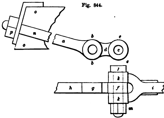
DETAILS OF TRUSS RODS—SCALE, 2 INCHES TO THE FOOT
