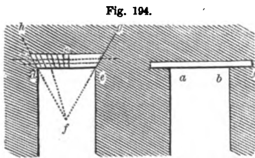
FLAT ARCH AND LINTEL—SCALE, \frac{1}{4} INCH TO THE FOOT.
