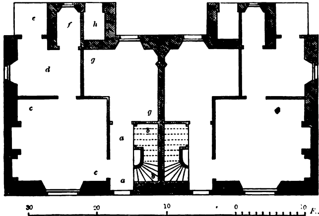
GROUND-PLAN OF TWO-STORYED DOUBLE-DETACHED COTTAGES.
