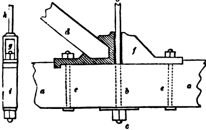
CAST-IRON SHOE FOR THE RECEPTION OF WOODEN STRUTS—SCALE, \frac{1}{2} INCH TO THE FOOT.
