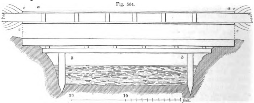
ITALIAN WOODEN AQUEDUCT FOR CONDUCTING WATER OF IRRIGATION OVER RIVERS, RAVINES, &c.
