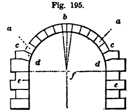
DISPOSITION OF THE PARTS OF AN ARCH —SCALE, \frac{1}{4} INCH TO THE FOOT.
