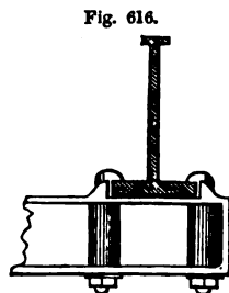
SUSPENSION OF CROSS-BEAMS FROM GIRDERS—SCALE, \frac{1}{4} INCH TO THE FOOT.
