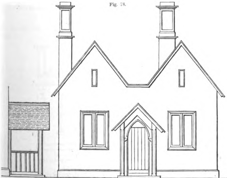
FRONT ELEVATION OF A SINGLE-STORYED DETACHED COTTAGE.
