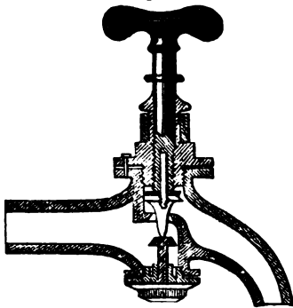
CHRIMES'S WATER-TAP.
