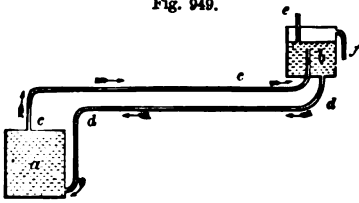
PRINCIPLE OF HOT-WATER SUPPLY.
