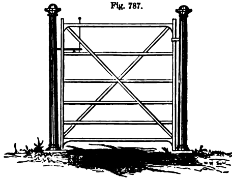
WROUGHT-IRON SIDE-GATE—SCALE, \frac{1}{2} INCH TO THE FOOT.
