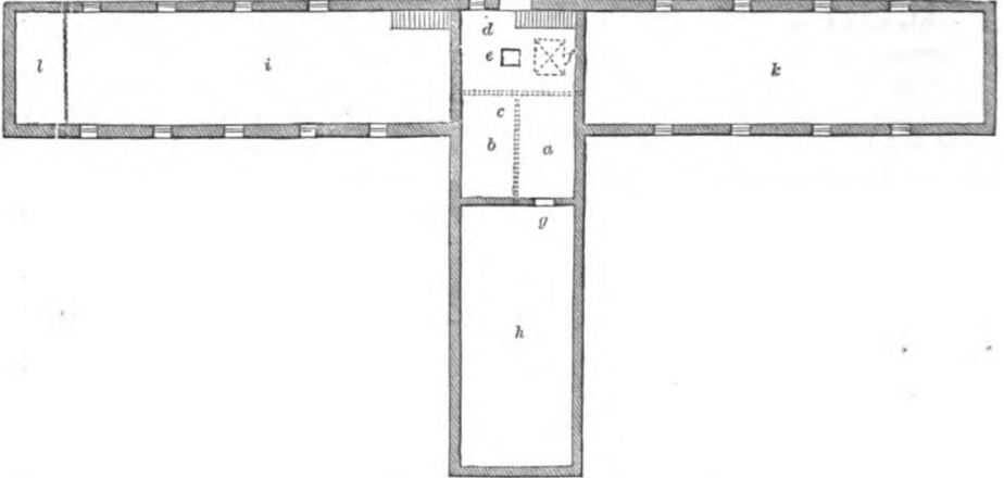
UPPER STORY OF A STEADING FOR SUBURBIAL FARMING WITH ARABLE CULTURE.
