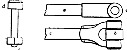
DETAILS OF TIE-RODS—SCALE IN FIG. 637.
