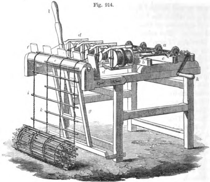
PERSPECTIVE VIEW OF MACPHERSON'S SHEEP-FENCE-MAKING MACHINE.
