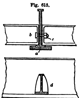
CONNECTION OF CROSS-BEAMS WITH GIRDERS—SCALE, \frac{1}{4} INCH TO THE FOOT.
