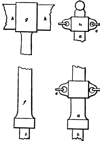
UPRIGHTS FOR SUPPORTING CHAINS AND RAILS.
