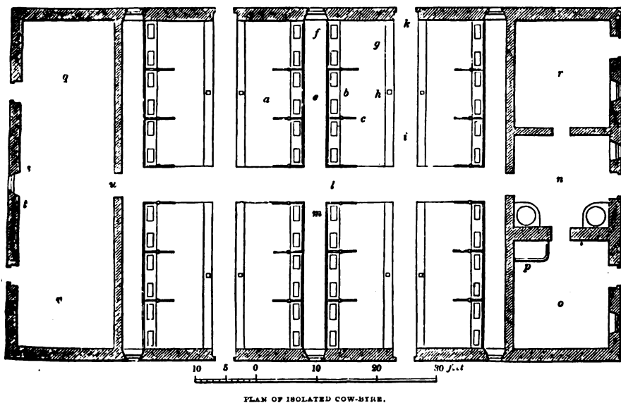
PLAN OF ISOLATED COW-BYRE.
