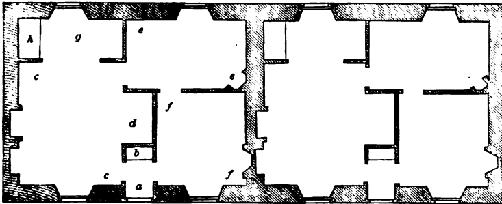
ALTERNATIVE GROUND-PLAN OF SINGLE-STOREYED DOUBLE-DETACHED COTTAGES—SCALE IN FIG. 88.
