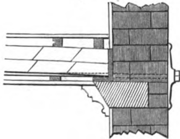
SECTION SHOWING TIE-ROD PASSING UNDER CELLULAR BRICKS—SCALE, \frac{1}{4} INCH TO THE FOOT.
