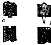
SECTION OF PLANKS FOR MOULD FOR PISE WALLS.
