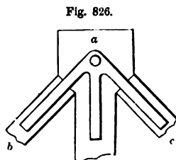
IRON STRAP FOR HEAD OF KING-POST AND BRACES—SCALE, \frac{1}{2} INCH TO THE FOOT.
