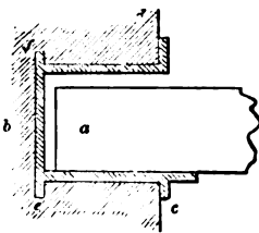
CAST-IRON SHOE FOR RECEIVING END OF GIRDER—SCALE, \frac{1}{2} INCH TO THE FOOT.
