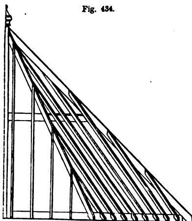
ELEVATION OF HEXAGONAL ROOF—SCALE, \frac{1}{4} INCH TO THE FOOT
