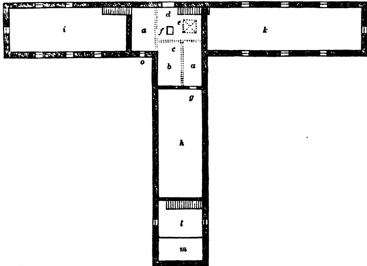
UPPER FLOOR OF A STEADING FOR COARSE FARMING.
