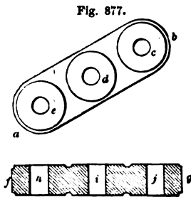
PLATE CONNECTING THE ENDS OF TIE-BOLTS AND STRUTS.
