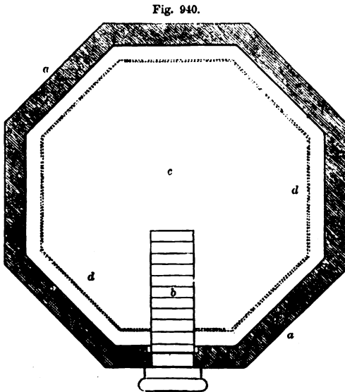
PLAN OF PIGEON HOUSE—SCALE. \frac{1}{4} INCH TO THE FOOT.
