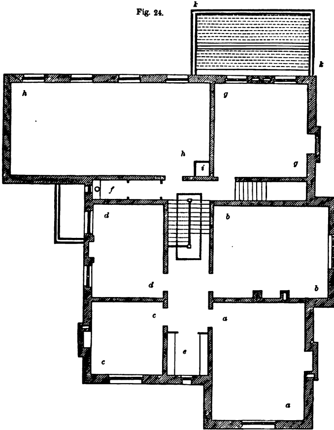
CHAMBER-FLOOR PLAN OF FARMHOUSE—SCALE IN PLATE XVIII.
