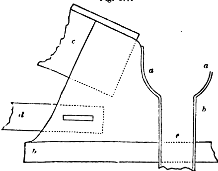
GUTTER FOR DOUBLE-SPAN ROOF—SCALE IN FIG. 657.
