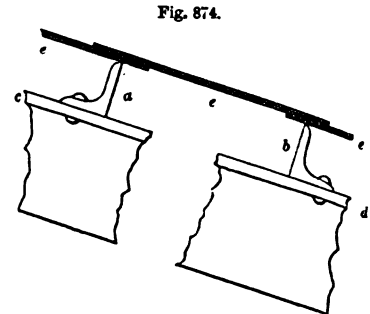
FIG. 874. FIXING OF SLATES WITH IRON ROOF—SCALE IN FIG. 857.
