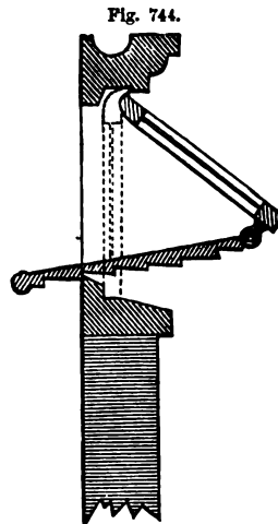
RATCHET-VALVE FOR ADMITTING AIR.
