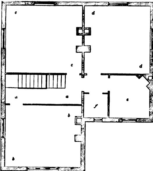
CHAMBER-FLOOR PLAN OF A THIRD-CLASS FARMHOUSE—SCALE, \frac{1}{4} OF AN INCH TO THE FOOT.
