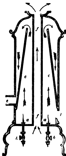
RICKETT'S GAS-STOVE.
