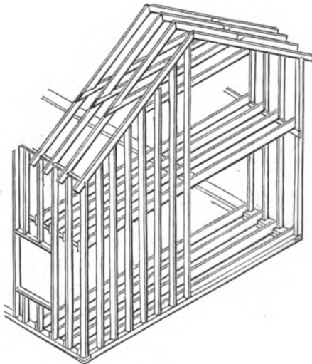
ISOMETRICAL PERSPECTIVE VIEW OF THE BALLOON FRAME.
