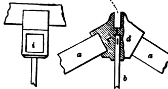
SHOES FOR KING-BOLT HEADS—SCALE, \frac{1}{2} INCH TO THE FOOT.
