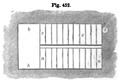
PLAN OF PLATFORM STAIRS—SCALE, 1/4 INCH TO THE FOOT
