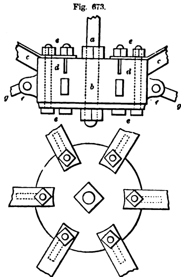
JUNCTION OF KING-BOLT, STRUTS, AND TIE-RODS—SCALE, 1 INCH TO THE FOOT.
