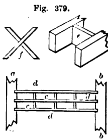
TRUSSING OF FLOORING BEAMS—SCALE. 1/4 INCH TO THE FOOT.
