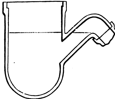
COURT CESSPOOL-TRAP.
