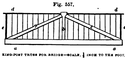
KING-POST TRUSS FOR BRIDGE—SCALE, \frac{1}{4} INCH TO THE FOOT.
