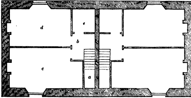
CHAMBER-FLOOR PLAN OF FIG. 99.
