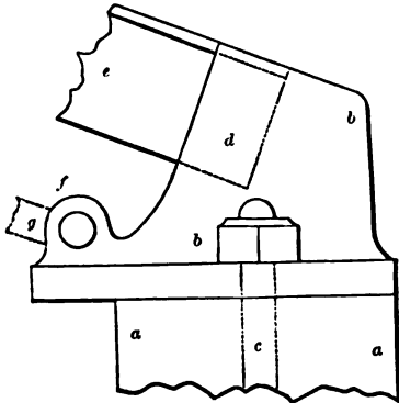
RAFTER-SHOE FOR ROOF IN FIG. 632.—SCALE IN FIG. 637.
