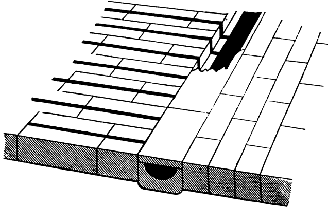
DRAINAGE PAVEMENT-BRICKS IN PERSPECTIVE, WITH GUTTER PARTLY UNCOVERED TO SHOW ITS CONNECTION WITH PAVEMENT.
