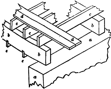
DOUBLE FLOORING—SCALE. 1/4 INCH TO THE FOOT.
