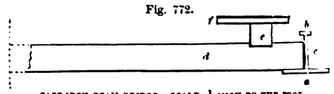
CAST-IRON BEAM BRIDGE—SCALE, 1/4 INCH TO THE FOOT.
