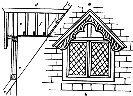
ELEVATION AND SECTION OF DORMER WINDOW—SCALE, \frac{1}{4} INCH TO THE FOOT.
