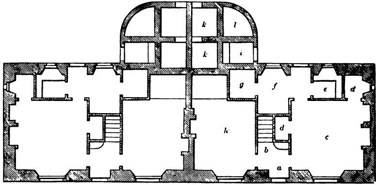
GROUND PLAN OF TWO-STORYED DETACHED COTTAGES.
