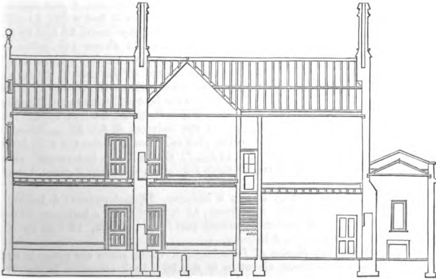
LONGITUDINAL SECTION OF FARMHOUSE IN THE LINE A B, FIG. 23.
