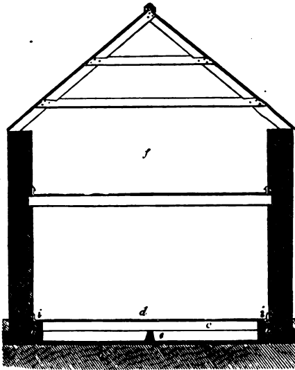
SECTION OF THE CORN-BARN FLOOR.
