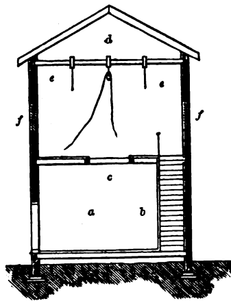
SECTION OF DETACHED SLAUGHTER-HOUSE—SCALE IN FIG. 946.
