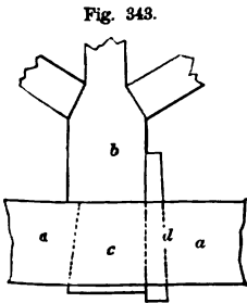
SECTION OF KING-POST WITH TIE-BEAM, WITH WEDGE—SCALE, 1/2 INCH TO THE FOOT.
