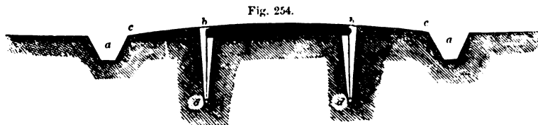
SECTION OF ROAD ON STRONG CLAY SOILS—SCALE, \frac{1}{4} INCH TO THE FOOT.
