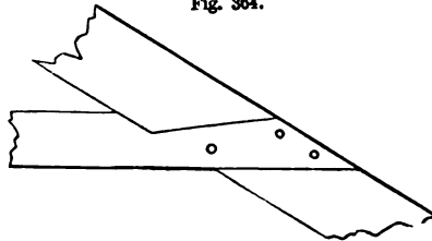
JOINT OF COLLAR WITH RAFTER—SCALE, 1/2 INCH TO THE FOOT.
