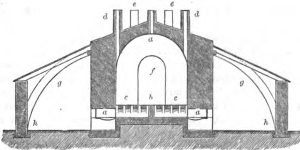
TRANSVERSE VERTICAL SECTION OF DRAIN-TILE KILN.
