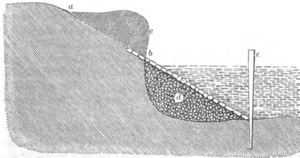
PROTECTION OF SEA-BANKS.
