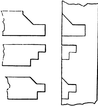
TUBE JOINTS—SCALE, \frac{1}{2} INCH TO THE FOOT.
