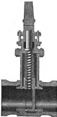
JENNING'S SLUICE-VALVE.
