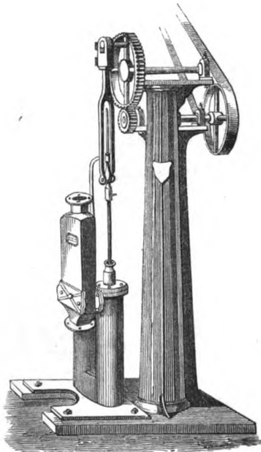
PERSPECTIVE VIEW OF HOLMAN'S DOUBLE-ACTION PUMP
