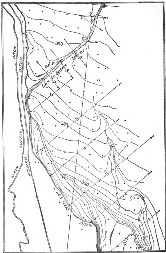
Fig. 10k. Contours of ground water in the Los Angeles river valley, California. (U. S. Geol. Survey.)
