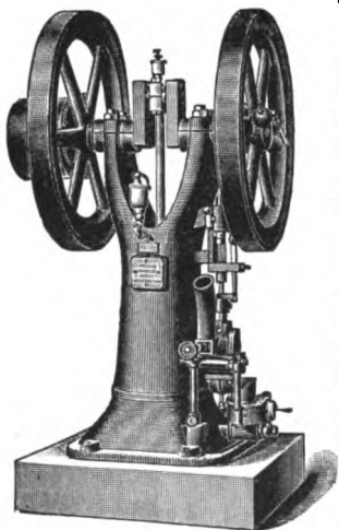
Fig. 77. Webster 2\frac{1}{2} horse-power vertical gasoline engine.
