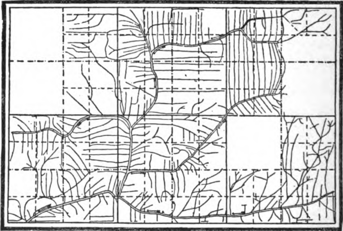
Fig. 151. Plan of drainage of lands of the Illinois Agricultural Company, Rantoul, Illinois. After J. O. Baker. The smallest squares are 40 acres; double lines show open ditches; single lines are tile drains.
