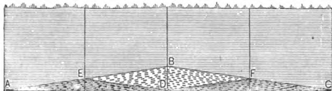
Fig. 139. Diagram of influence of distance between drains on depth of drainage.
