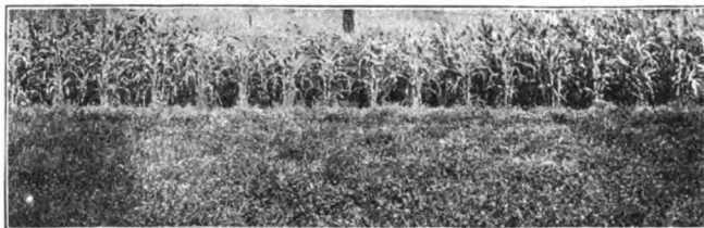
Fig. 25. Difference in growth of corn where there is a difference of 3 per cent of soil moisture in the surface foot.
