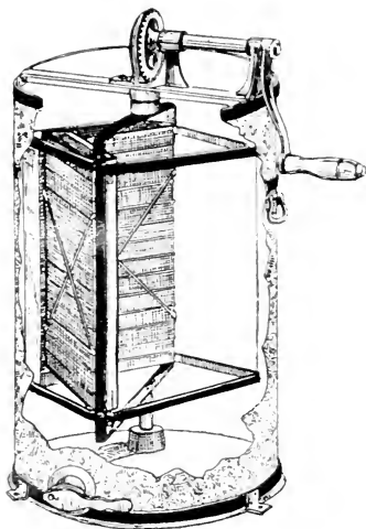
Two-frame reversible Cowan. Pockets in wrong position.
