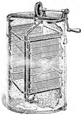
Two-frame reversible Cowan. Pockets in right position.
