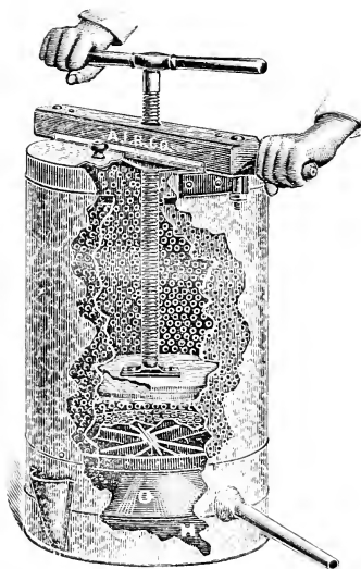
The Root German Steam Wax-Press.
