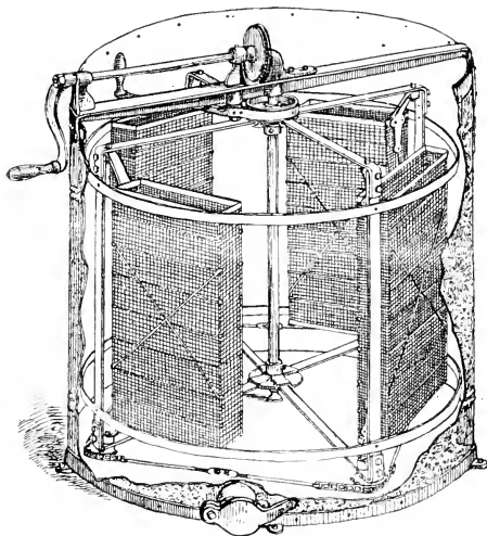
Reel of four-frame reversible Cowan extractor.
