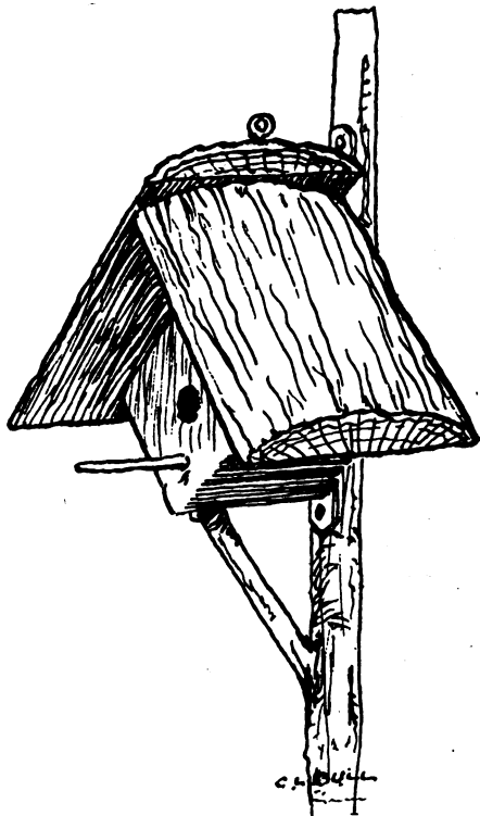
Wren House —Simply a square box (5in.), all dimensions inside measurement, with slab covering, flat on back, but 3 in. overhang in front and 1 in. at sides. One inch hole at center of front; 3 in. perch. We have shown this box on pole but it could be hung from screw eye.
