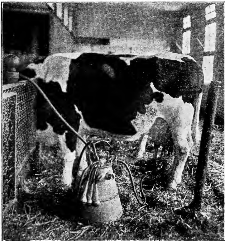
X.—MILKING MACHINE PAIL with one set of teat cups in operation. The pail is divided by a partition which keeps the milk of two cows separately.
