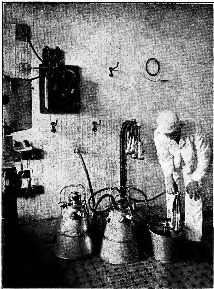
XII.—CLEANING MILKING MACHINE CONNECTIONS.
