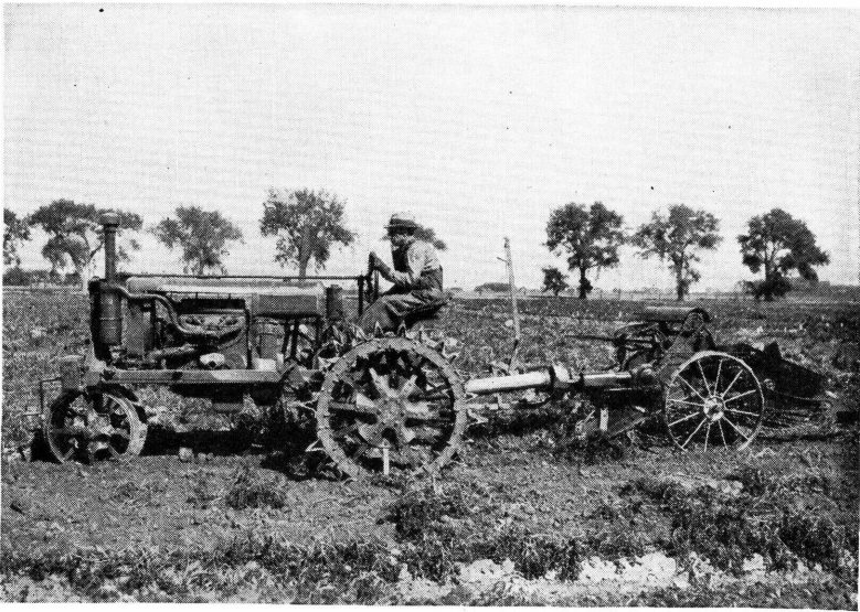
FIGURE 10.—One-row potato digger with a continuous chain.
