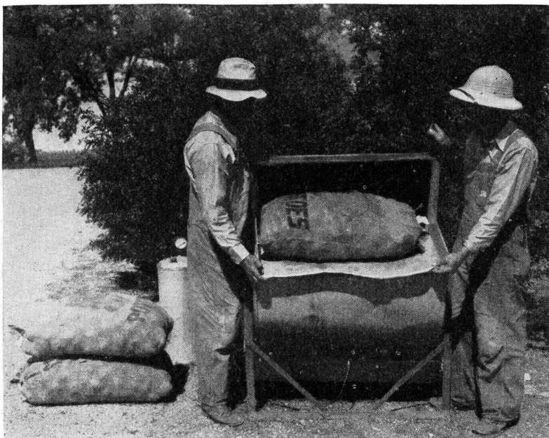
FIGURE 6.—Small outfit for treating potatoes with hot formaldehyde solution on the farm.
