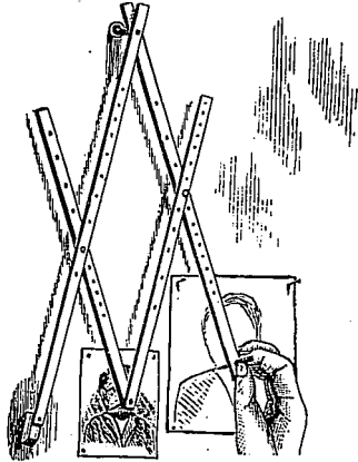
Fig. 42. THE PANTOGRAPH.
