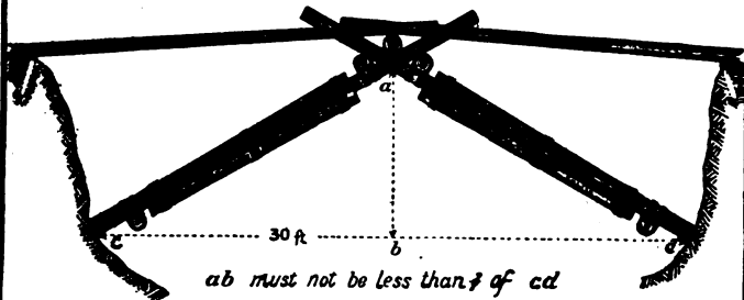
FIG. 4. Single Lock.
