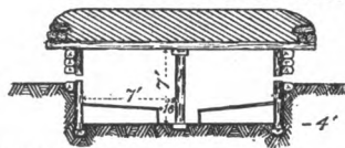
Sunken Block House.
