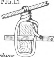
Rack lashing
