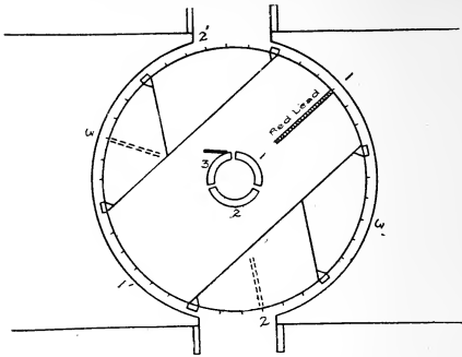
LEFT-HAND DRUM ARMATURE.
