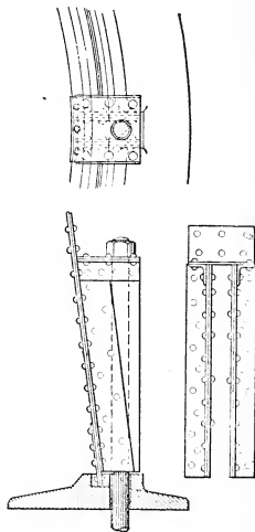
Holding down Bolts and Lugs.
