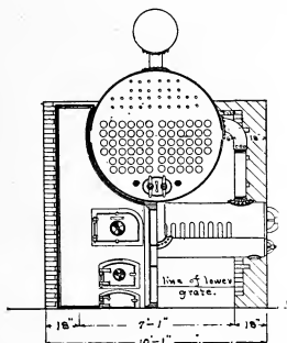
View of the Hawley's Down Draught Furnace.
