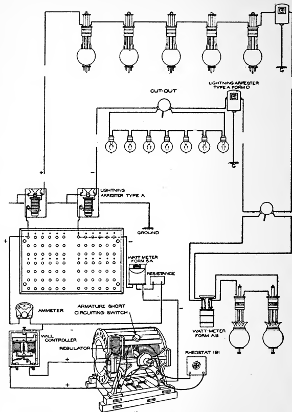
CONNECTIONS FOR ARC LIGHTING SYSTEM.
