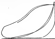
EXTREME LOAD VARIATION INDICATION.
