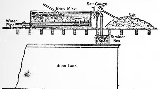
Complete Brine Mixing Arrangement.
