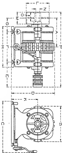
DIMENSIONS.
