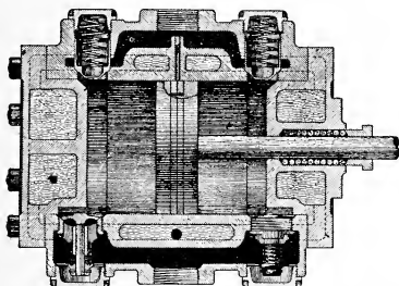
SECTIONAL VIEW OF AIR CYLINDER WITH VERTICAL LIFT VALVES, USED CLASS "E" AND "F" COMPRESSORS.
