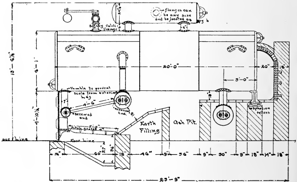
Hawley's Down Draught Furnace.
