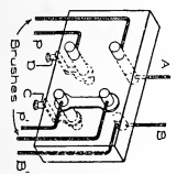
Details of Terminal Board Connections for Form 2 Regulator.
