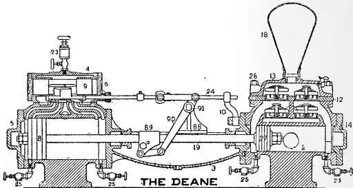
The Deane Pump.
