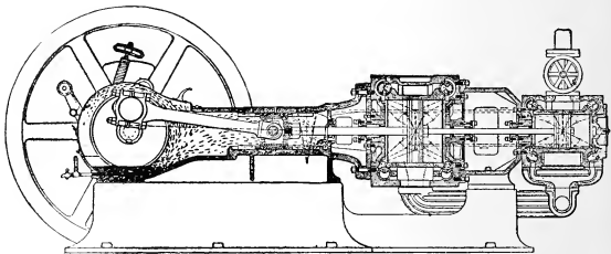
Sectional Elevation of Harrisburg Standard Four-Valve Tandem Compound Engine.
