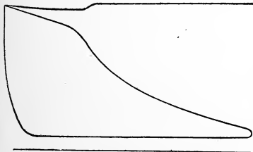
Fig. 12. Steam Chest Card on Forward Stroke.
